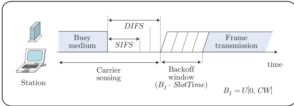
Figure 1.2: CSMA/CA mechanism.
