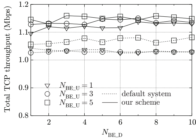
Figure 3.9: Total system throughput of TCP flows ( N_{VO} = 5 , N_{VI\_D} = N_{VI\_U} = 1 ).
