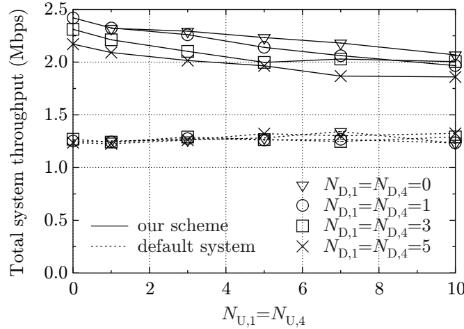
Figure 4.10: Total system throughput of TCP flows.
