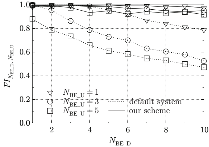
Figure 3.7: Per-flow fairness index FI_{BE,D,BE,U} of TCP flows ( N_{VO} = 5 , N_{VL,D} = N_{VL,U} = 1 ).
