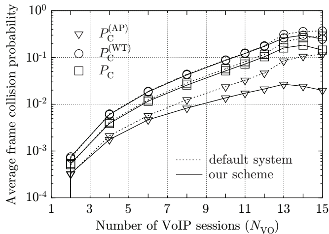
Figure 3.6: Average frame collision probability of VoIP flows.
