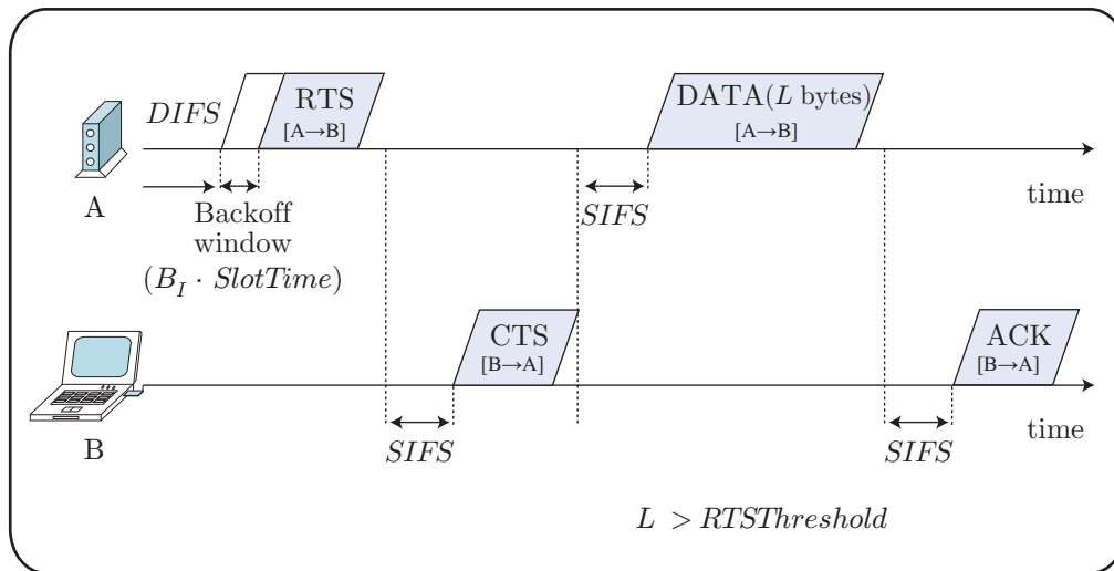
Figure 1.5: RTS/CTS scheme.
