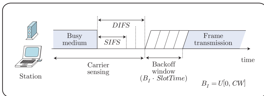
Figure 1.2: CSMA/CA mechanism.
