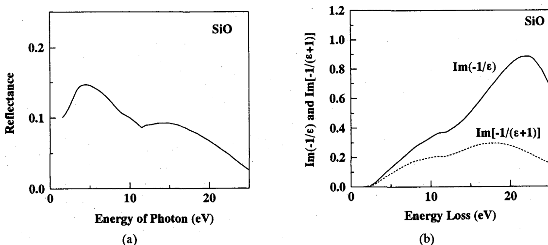
FIG. 3-26. Optical reflectance (a) and optical bulk and surface energy loss functions (b) for \text{SiO} calculated from the optical constant (see Ref. 18). The solid and dotted lines in (b) are the optical bulk and surface energy loss functions [1].
