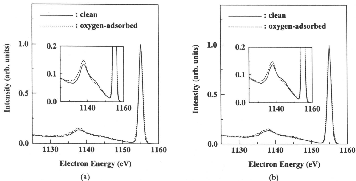
FIG. 3-15. Experimental REELS spectra for the clean (solid line) and oxygen-adsorbed (dotted line) Si (111) surfaces. (a) and (b) are the spectra measured under the conditions (a) and (b), respectively. The intensity is normalized to the no-loss peak [1].
