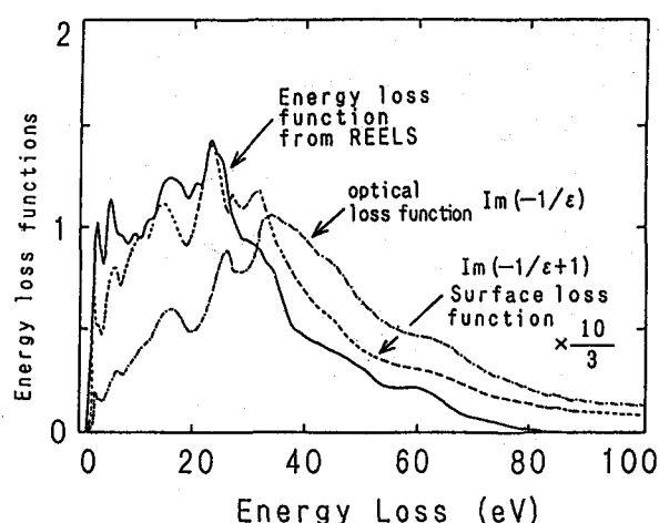
FIG. 1-6. Comparisons of the newly obtained energy loss function for Au obtained from REELS analysis with the optical bulk energy loss function, \text{Im}[-1/\epsilon] , and the surface energy loss function, \text{Im}[-1/(\epsilon+1)] , [19].
