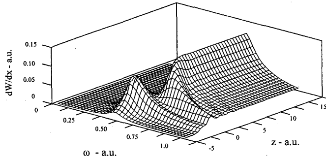
FIG. 5-8. The surface representing energy loss per unit path length by an electron moving parallel with an abruptly terminated metal surface as a function of z and \omega . The conditions assumed are the same as those of FIG. 5-5. The SR Model, together with the Plasmon Pole dielectric function, was used in these calculations. The distribution is smoother and broader than that shown in FIG. 5-5, but there is still a clear separation between the surface plasmon and bulk plasmon structures [15].
