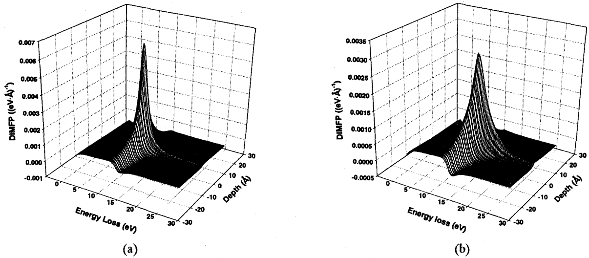
FIG. 5-16. The DIMFPs for an electron having the SR trajectory. (a) the local dielectric function and (b) the HD dielectric function are used to calculate. The DIMFP for positive value of z represents the DIMFP for the reflected electron ( t > 0 ).
