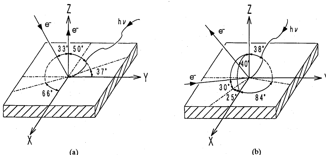
FIG. 3-1. Experimental geometry. (a) The incident angles of the electron and X-ray are 33^\circ and 50^\circ , respectively, from the surface normal. The take-off angle is set at the surface normal direction. (b) The incident angles of electron and X-ray and the take-off angle are 60^\circ , 38^\circ and 40^\circ , respectively, from the surface normal. Geometry (b) is obtained by a rotation of 40^\circ around the Y-axis from geometry (a) [1].
