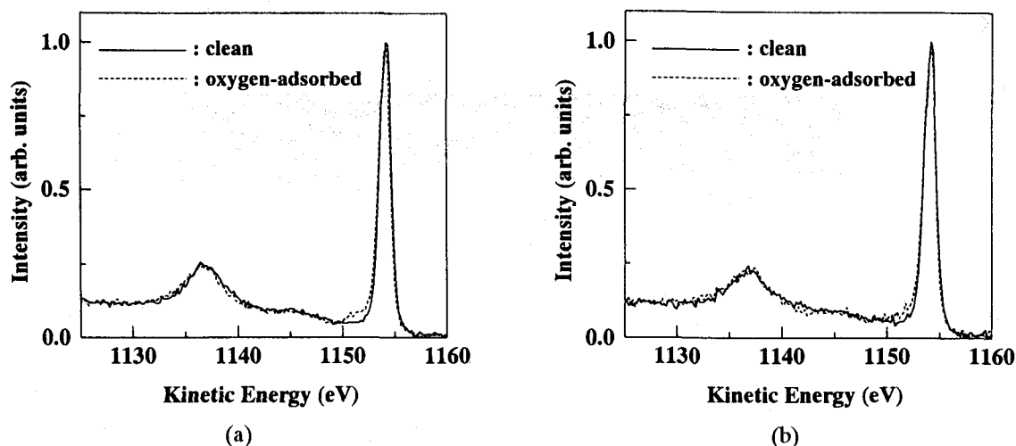
FIG. 3-16. Experimental Si 2p XPS spectra for the clean (solid line) and oxygen-adsorbed (dotted line) Si(111) surfaces. (a) and (b) correspond to the spectra for the experimental geometries (a) and (b), respectively. The constant background has been previously subtracted. The intensity is normalized to the Si 2p photoelectron peak [1].
