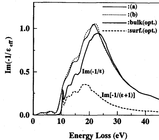
FIG. 3-25. Effective energy loss functions for SiO 2 surface obtained from the measured REELS spectra. The effective energy loss functions for the measurement geometry (a) and (b), are shown by the solid and dotted lines, respectively. The optical bulk and surface energy loss functions calculated from the optical constant (see Ref. 18) are also shown by the thick solid and dotted lines [1].
