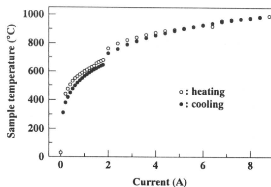
FIG. 3-12. Current dependence of sample temperature.
