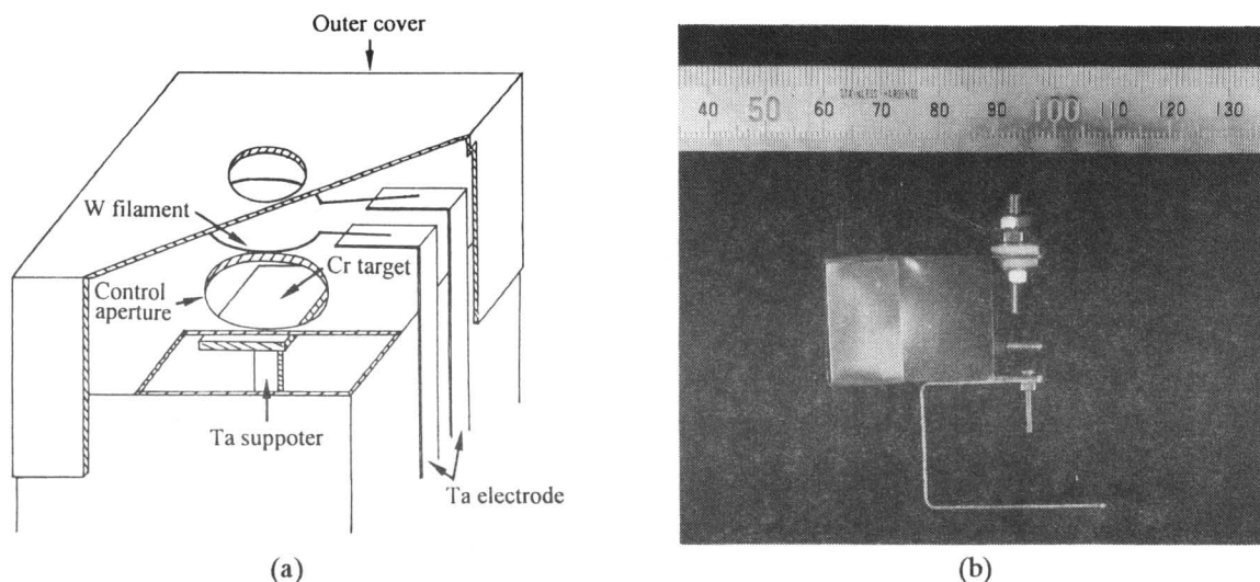
FIG. 3-13. Cr evaporator; (a) schematic illustration and (b) outer view.
