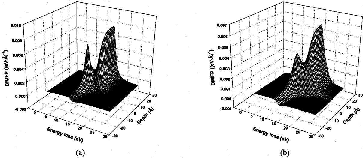
FIG. 5-12. The DIMFPs for an electron having the penetrating trajectory obtained using (a) the local dielectric function and (b) the HD dielectric function.
