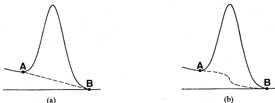
FIG. 1-4. Schematic of the background subtraction method; (a) linear approximation and (b) Shirley method.
