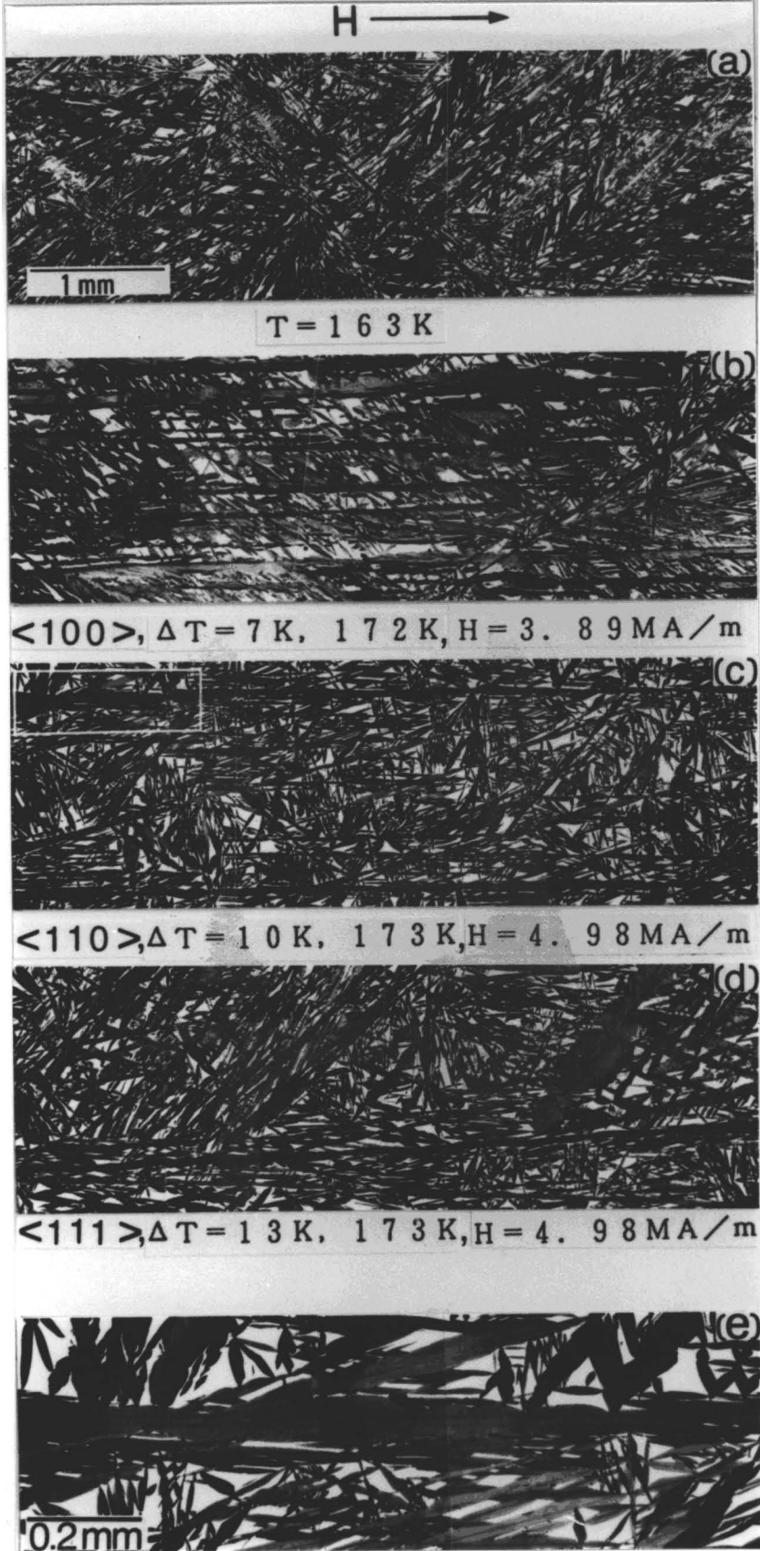
Fig.7 Macroscopic optical micrographs of thermally-induced, (a), and magnetic field-induced ones in three single crystal specimens with \langle 100 \rangle , \langle 110 \rangle and \langle 111 \rangle orientations, (b), (c) and (d). (e) is an enlargement of the framed area of (c). The direction of an applied magnetic field, crystal orientation, transformation temperature, \Delta T and H are indicated in each photograph.
