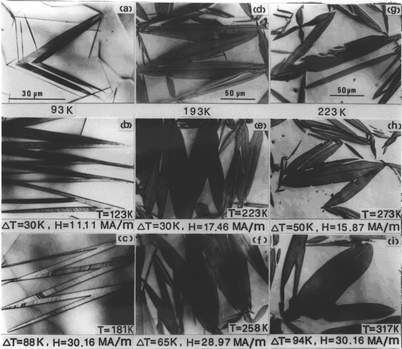
Fig. 5 Optical micrographs of thermally-induced martensites, (a), (d) and (g), and magnetic field-induced ones, (b), (c), (e), (f), (h) and (i). Transformation temperature T, \Delta T and H for the magnetic field-induced martensites are shown in each photograph.
