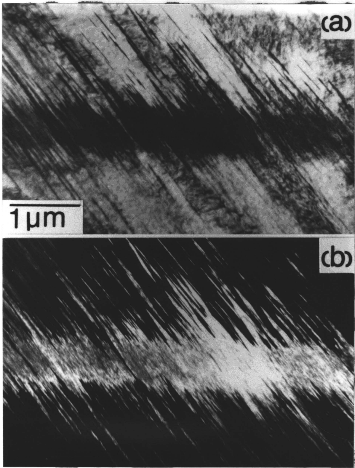
Fig. 9 Electron micrographs of a magnetic field-induced martensite in the Fe-31.7 at% Ni alloy at \Delta T=14K . (a) and (b) are bright and dark field images, respectively.
