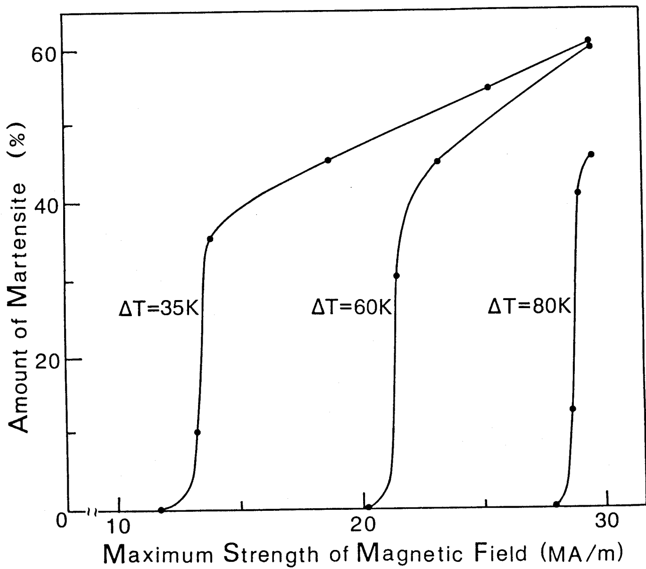
Fig. 4 Calculated amount of magnetic field-induced martensites plotted as a function of maximum strength of pulsed magnetic field.
