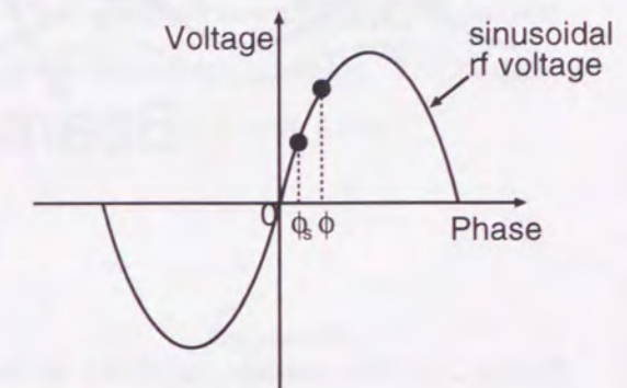
Figure 2.4: The definition of the synchronous phase \phi_s and the phase of arbitrary particle \phi .
