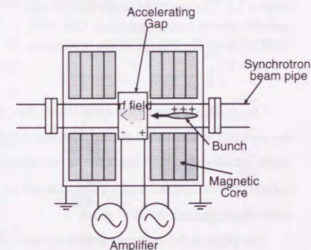
Figure 2.6: The rf cavity resonator loaded with magnetic cores.
