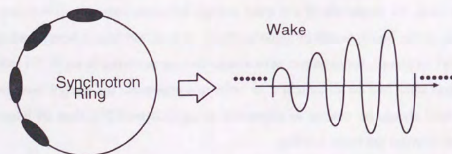
Figure 5.3: The periodic transient beam loading. The amplitude of the wake field are different on each bunch.
