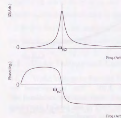
Figure 3.7: The impedance and the phase of the cavity in the series expression loaded with high Q magnetic core
