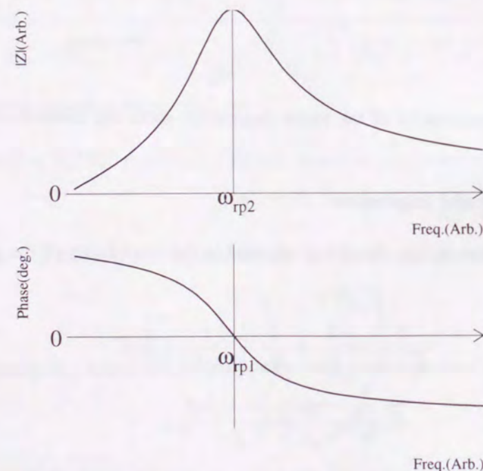
Figure 3.6: The impedance and the phase of the parallel expression.
