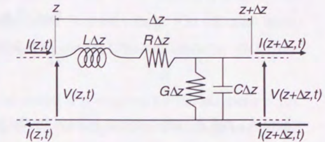
Figure A.1: The distributed constant circuit.
