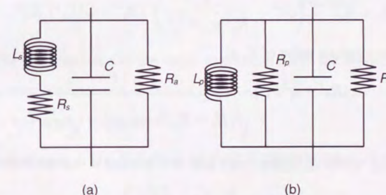
Figure 3.4: The lumped circuit model of the cavity. Parallel expression(a) and series expression(b).
