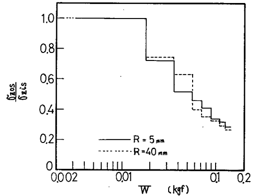
図 1.3.37 W と \sigma_{zos}/\sigma_{zis} の関係 \sigma_s = 1 \mu\text{m} p_m = 500 \text{ kgf/mm}^2 E_1 = E_2 = 21000 \text{ kgf/mm}^2
