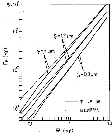
図 2.1.25 \bar{F}_p に関する本理論と自由転がり接触の比較 \beta = 0.05 \text{ mm} p_m = 150 \text{ kgf/mm}^2 n_p = (1.1/\sigma_p)^{1/2} \text{ mm}^{-1} R = 5 \text{ mm} E_1 = 21000 \text{ kgf/mm}^2 E_2 = 10000 \text{ kgf/mm}^2
