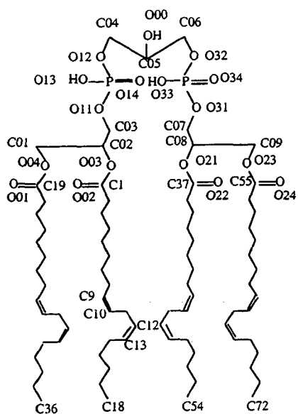
cardiolipin (diphosphatidylglycerol)
