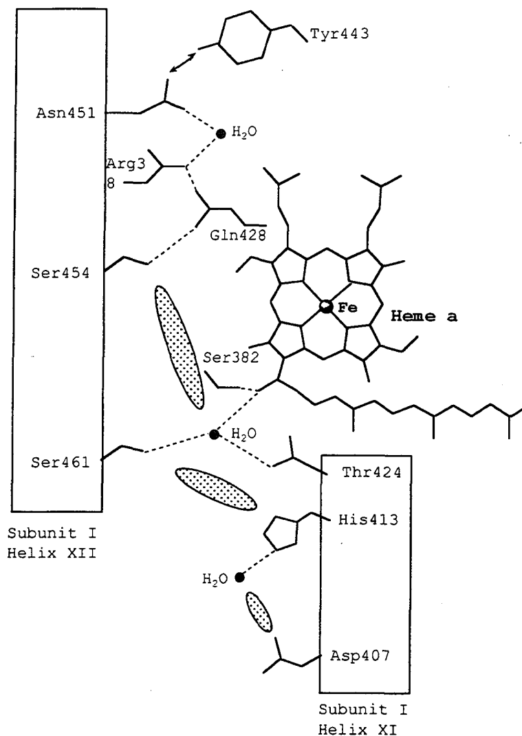
Figure 4.6. Schematic representation of candidates for proton channel.
