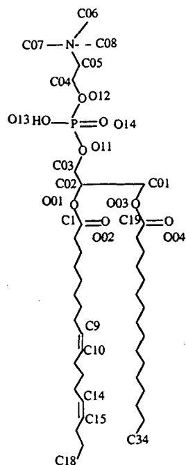
phosphatidylcholine
