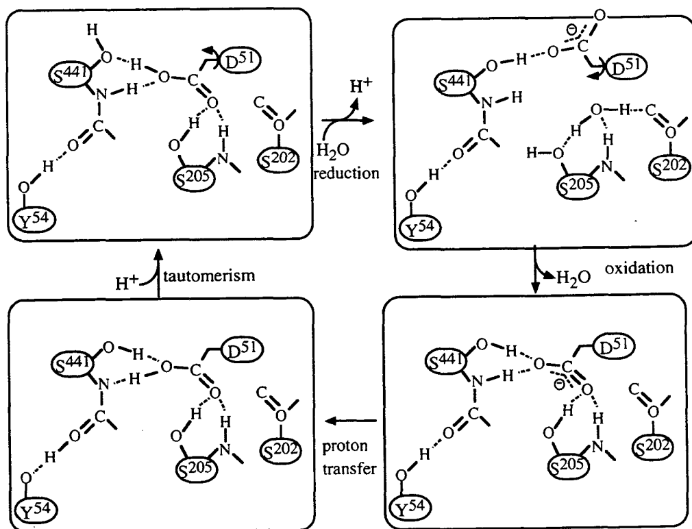
Figure 1.6. Schematic representations of the structure of the proton pumping system and a possible function of Asp51 to the matrix surface.
