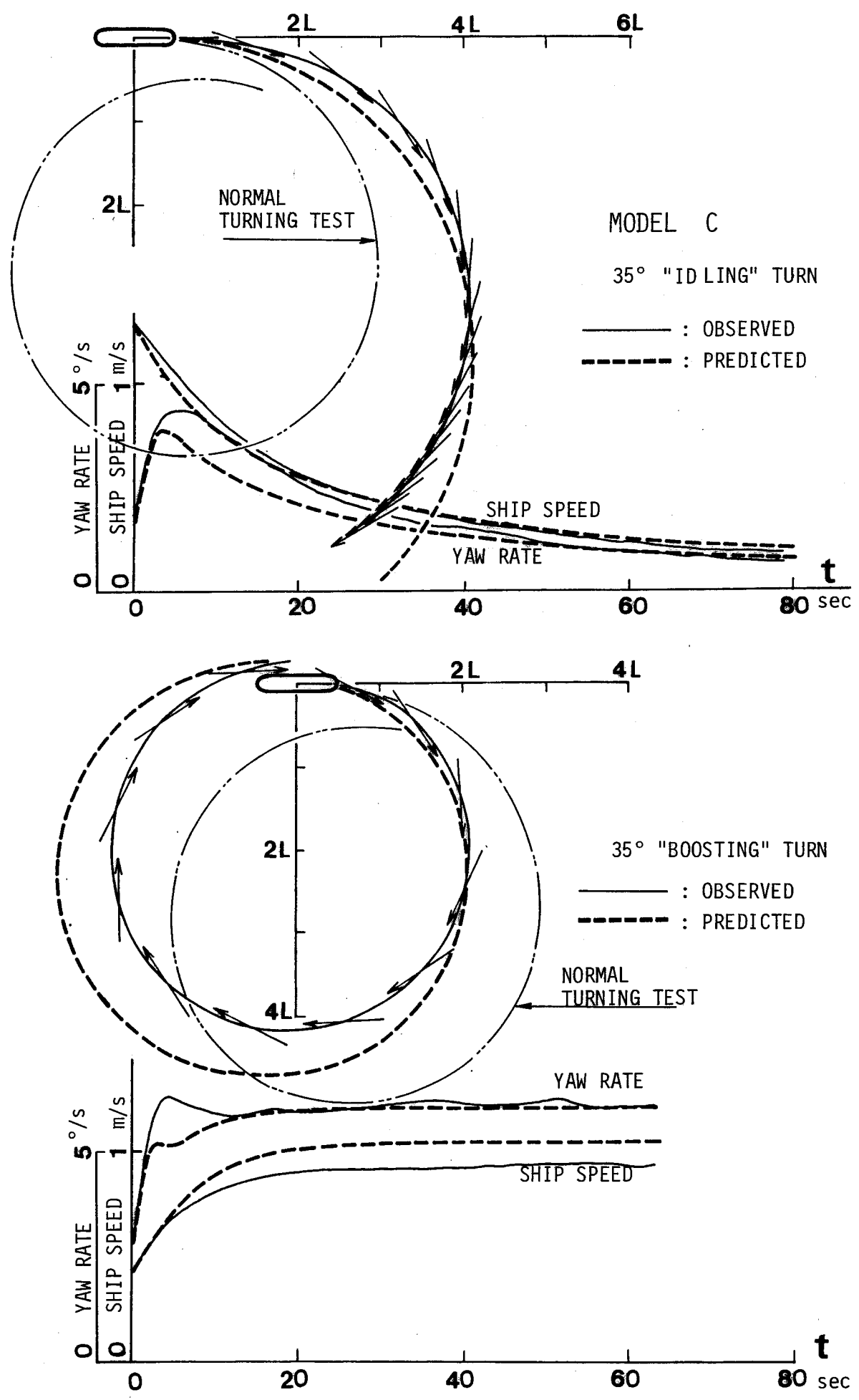
Fig. 4.6 "Idling" and "Boosting" turning tests of model C, observed and predicted.
