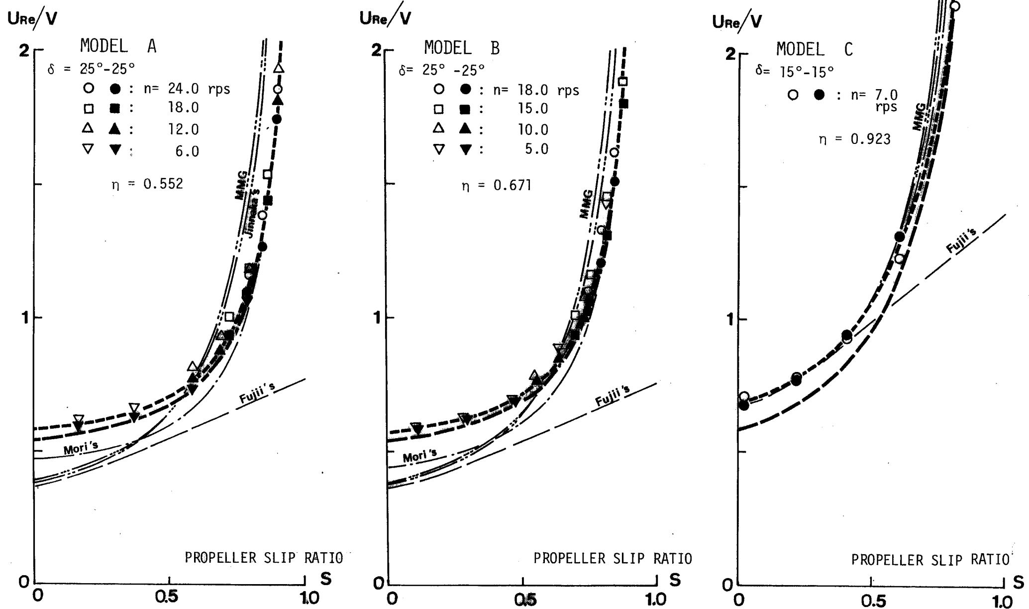
Fig.2.2 Effective rudder inflow velocity, measured and predicted, models A, B and C.
