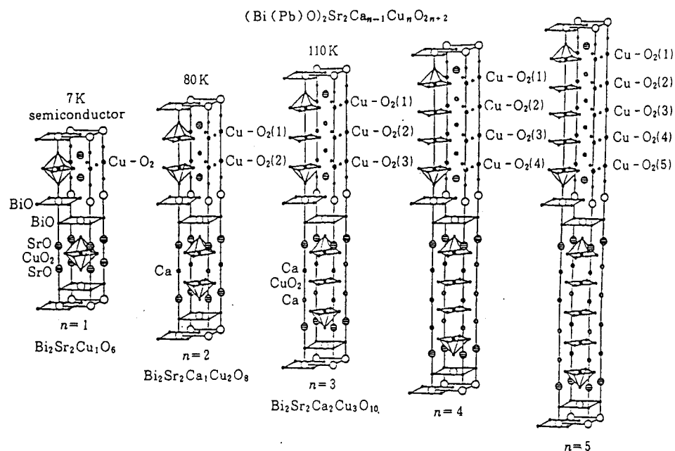
Fig. 4-2-1. The typical crystal structures of Bi 2 Sr 2 Ca n-1 Cu n O 2n+4 .
