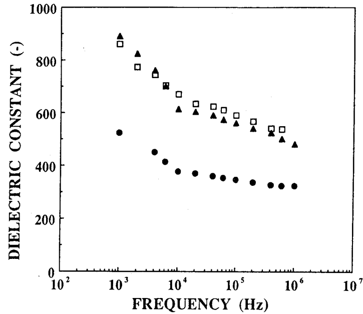
Fig. 5-3-13. (a) Applied frequency dependence of dielectric constant of various BTO/STO superlattices. (total thickness is 2000 Å) ( \bullet ; 1 unit stacking, \blacktriangle ; 2 unit, \square ; 4 unit, \blacksquare ; 25 unit and \triangle ; SBTO solid solution)
