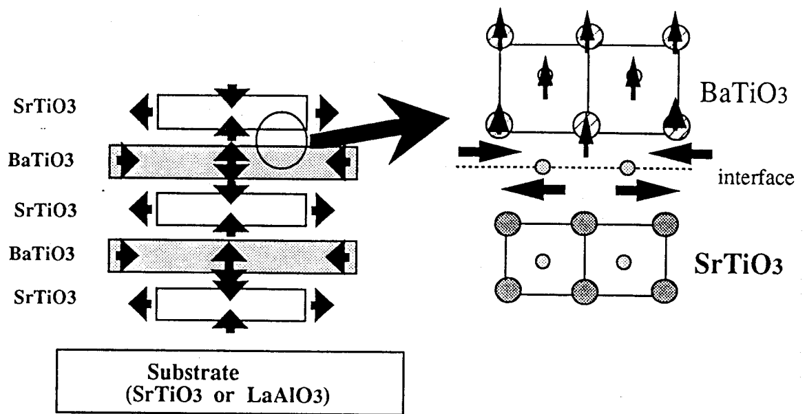
Fig. 5-1-2. A schematic model of strained \text{BaTiO}_3/\text{SrTiO}_3 superlattice.
