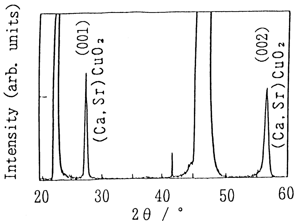
Fig. 4-2-2. X-ray diffraction patterns for the (Ca 0.86 Sr 0.14 )CuO 2 film prepared on the SrTiO 3 substrate.
