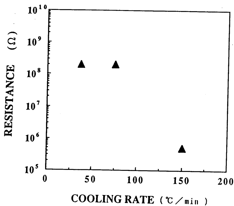
Fig. 8-1-1 (b) Resistance of the \text{PbTiO}_3 films vs cooling rate.
