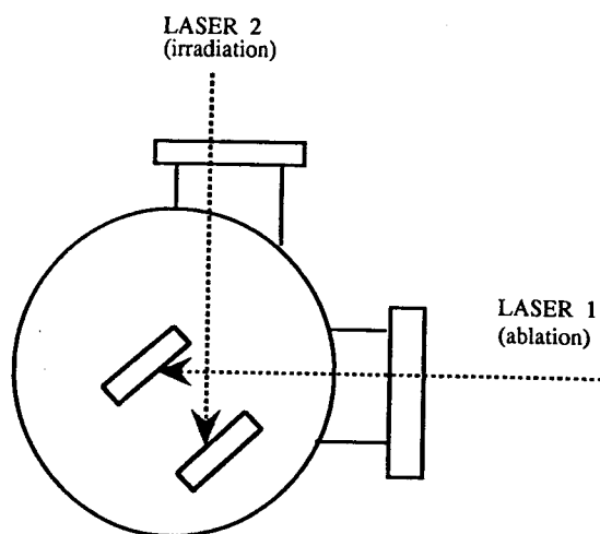
Fig. 3-3-2 schematic image of (a) substrate irradiation and (b) vapor irradiation.
