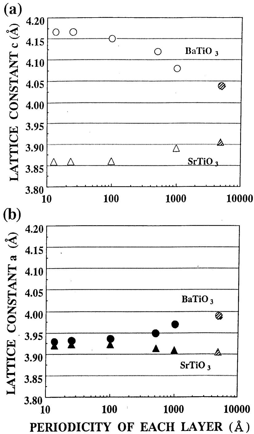
Fig. 5-3-6. Variation of the lattice constant a and c of BTO( \circ , \bullet ) and STO( \triangle , \blacktriangle ) layers in the STO/BTO superlattices against the layer thickness of each stacking periodicity. The total thickness of these superlattices is 2000 Å. Shaded circle and triangle show the lattice constant a and c of single phase film with thickness of 5000 Å.
