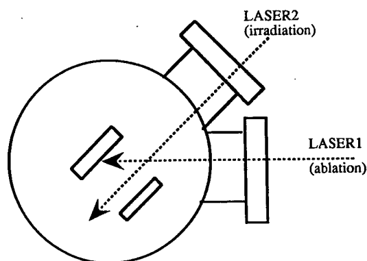
Fig. 3-3-2 schematic image of (a) substrate irradiation and (b) vapor irradiation.
