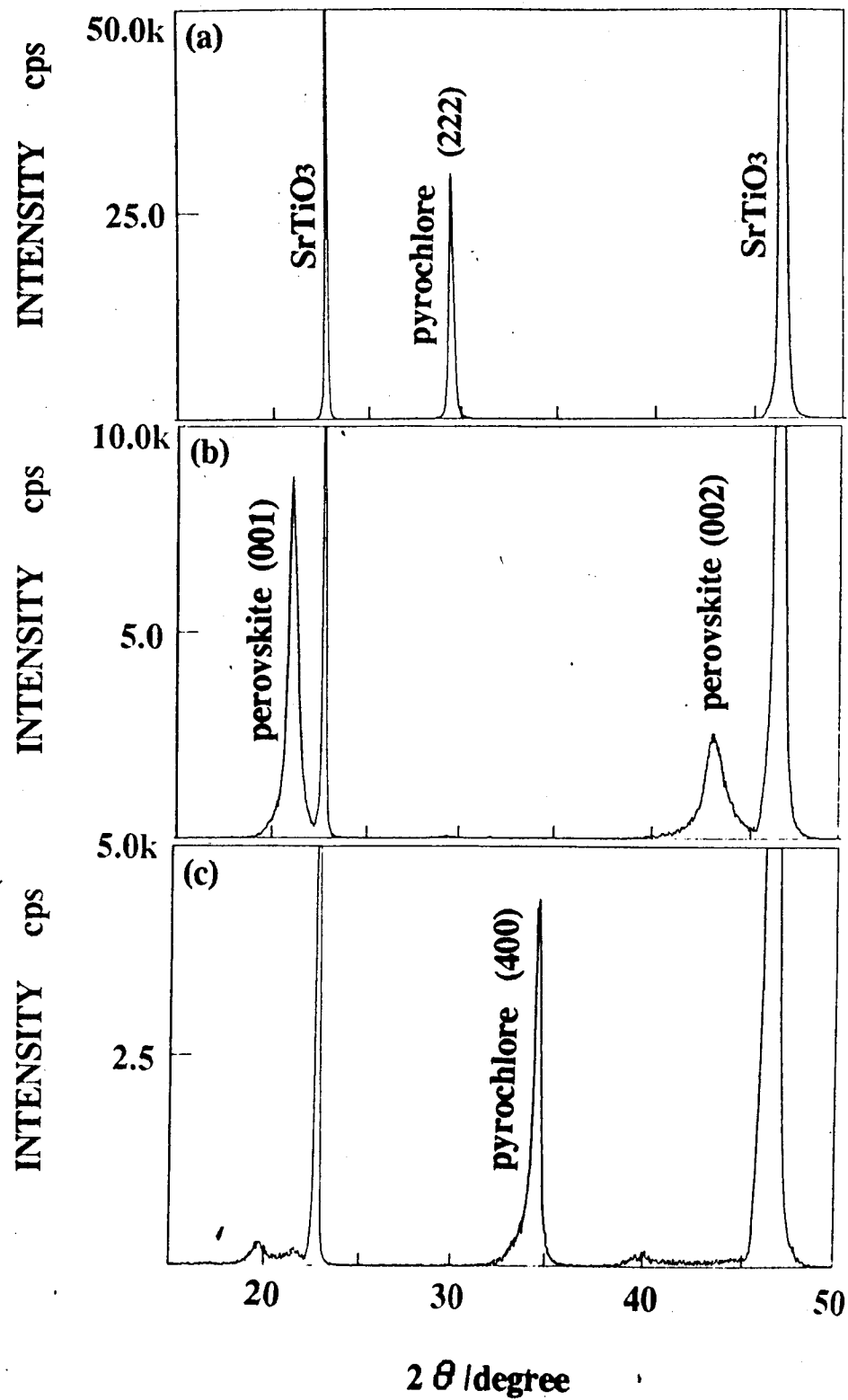
Fig. 3-2-4. X-ray diffraction pattern of \text{PbTiO}_3 films formed at substrate temperature and oxygen pressure of (a) 580°C, 35 mTorr, (b) 490°C, 35mTorr and (c) 400d°C, 50 mTorr.
