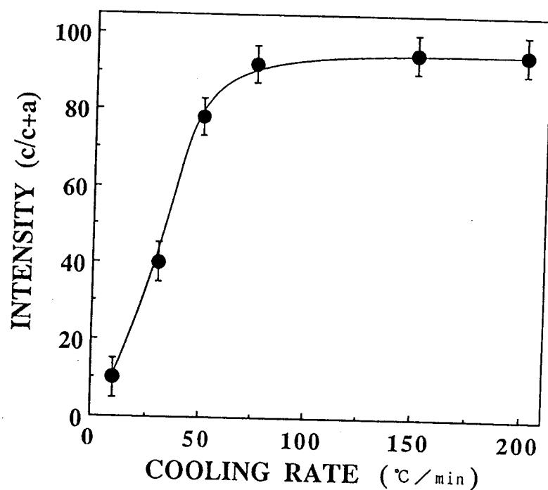
Fig. 8-1-1 (a) c-axis preferred orientation of the \text{PbTiO}_3 films vs cooling rate after contracting the films.
