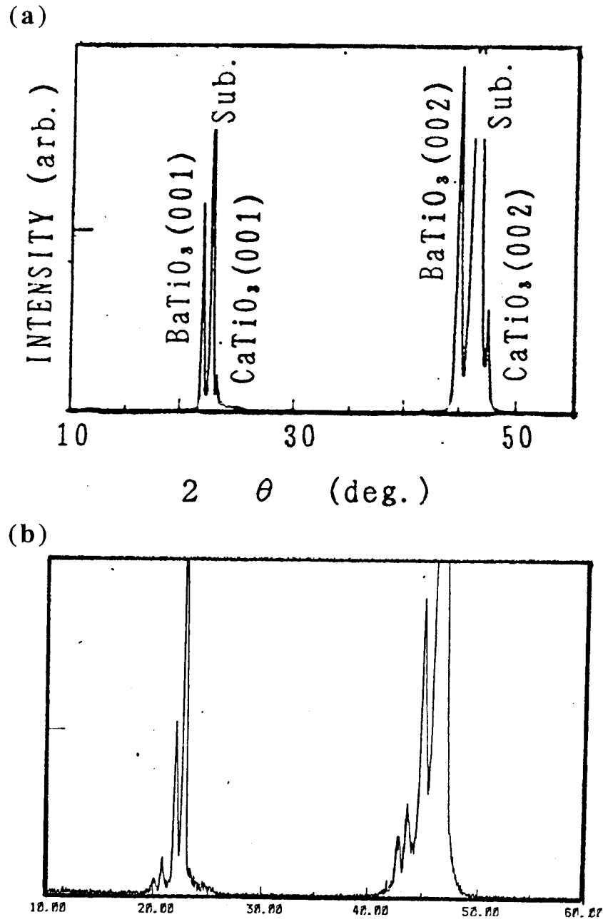
Fig. 5-3-18. (a) X-ray diffraction pattern of \text{CaTiO}_3/\text{BaTiO}_3 superlattice with stacking periodicity of 125 unit cell ( 500 \text{ \AA} ) (b) The X-ray diffraction pattern of observed \text{BTO}(20 \text{ \AA}; 5 \text{ unit cell})/\text{STO}(20 \text{ \AA}) superlattice.
