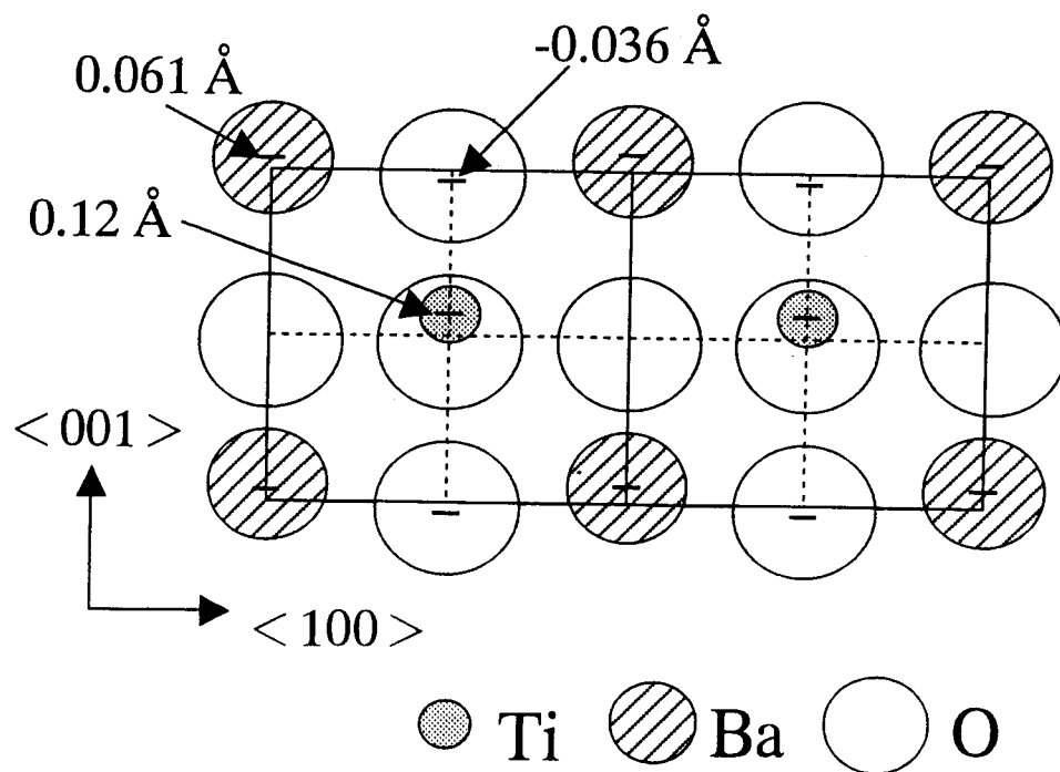
Fig. 5-1-3 Structure of tetragonal \text{BaTiO}_3 projected on (010), showing atomic displacement.
