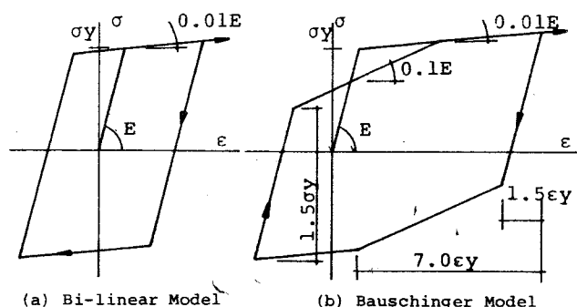
Fig.2-2 Stress-Strain Relations
