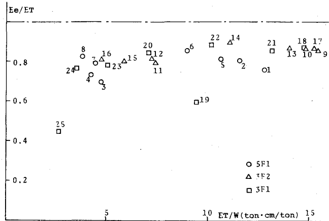
Fig.8-8 ET/W-Ee/ET Relation
