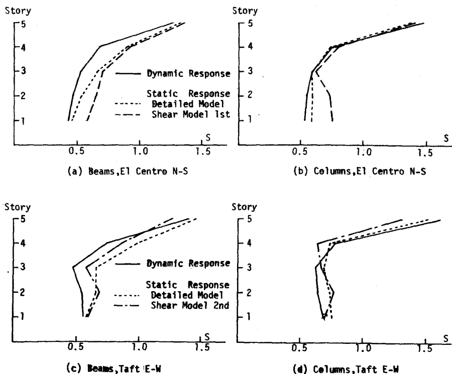
Fig.4-9 Maximum Stress Responses
