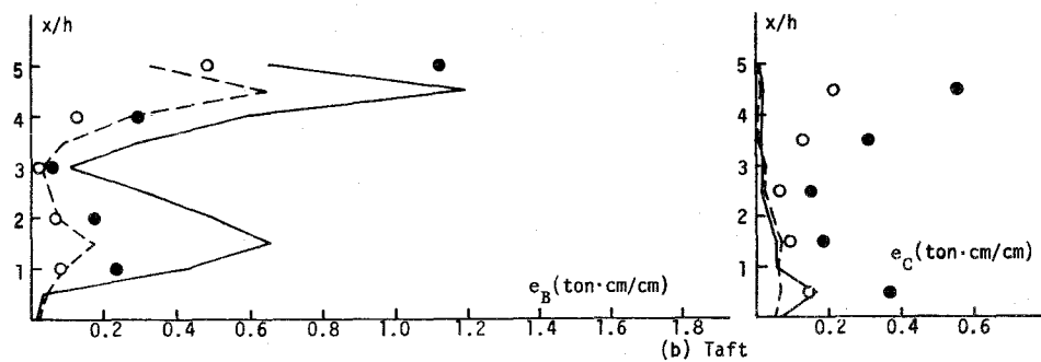
Fig.6-20 Vertical Distribution of Internal Work in 5F1
