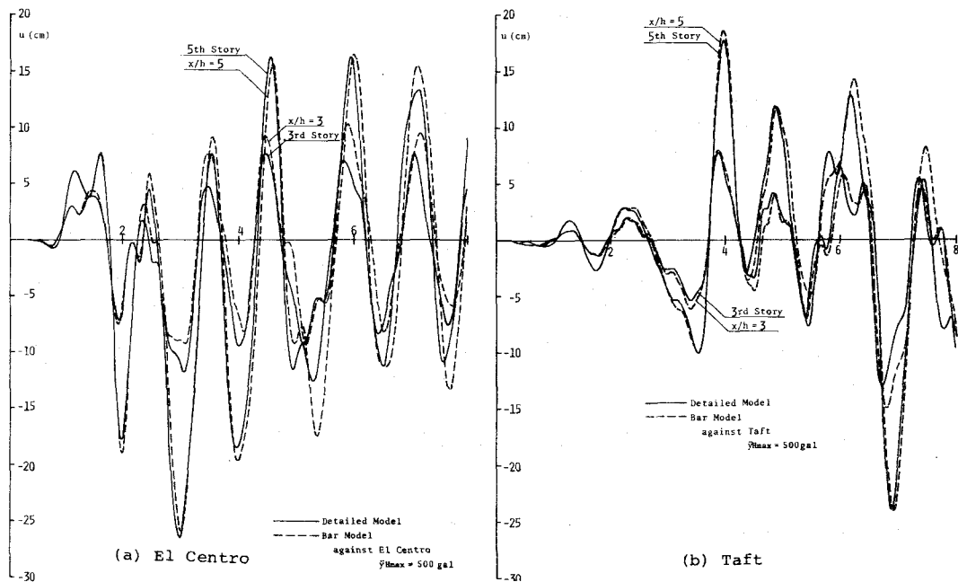
Fig. 6-16 Horizontal Displacement Time Histories
