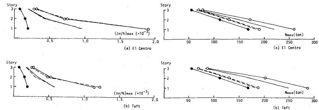
Fig. 5-9 (\Delta v/h)_{\max} and N_{\max} of 3F2
