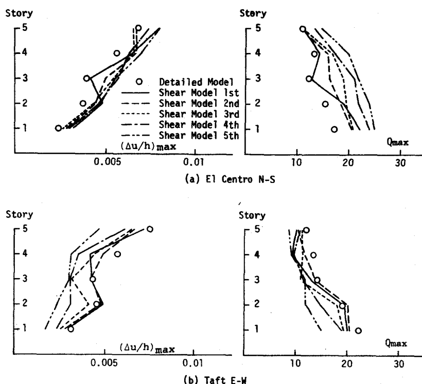
Fig.4-3 Maximum Responses of Elastic Systems
