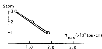
Fig.5-10 (\Delta\theta/h)_{\max} and M_{\max} of 5F1
