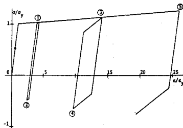
Fig.2-8 Stress-strain Relation of Bauschinger Model
