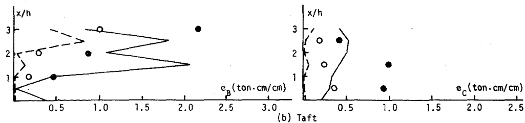
Fig.6-21 Vertical Distribution of Internal Work in 3F2
