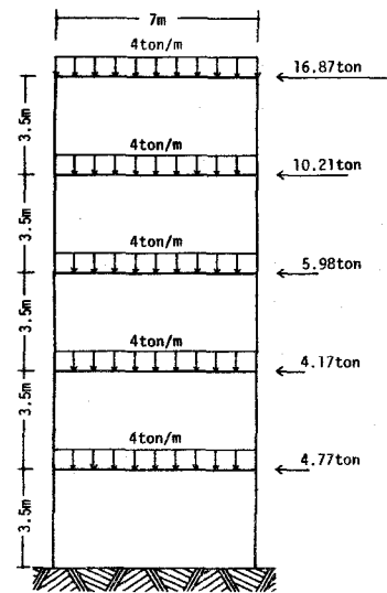
Fig.4-1 Frame Geometry
