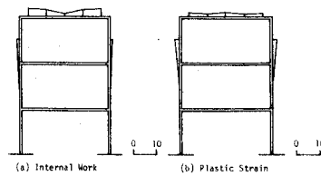
Fig. 5-19 Local Responses of 3F1 for U-D Component of Taft Earthquake ( \dot{y}H_{max}=389gal )
