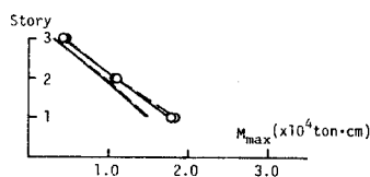
Fig.5-11 (\Delta\theta/h)_{\max} and M_{\max} of 3F1
