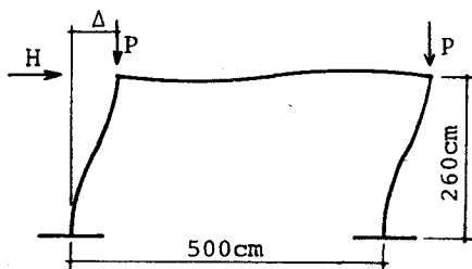
Fig.2-3 Test Frame
