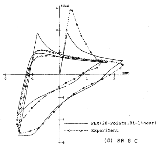
Fig.2-13 Axial Force-Deformation Relations
