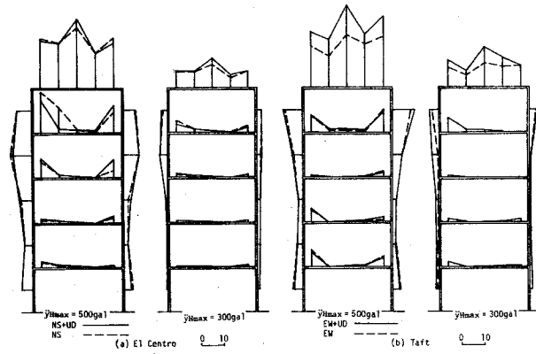
Fig. 5-16 Internal Work Distribution of 5F1
