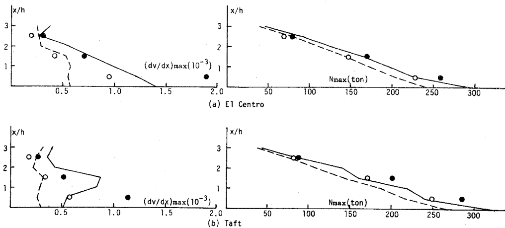
Fig.6-13 (dv/dx)_{\max} and N_{\max} of 3F2
