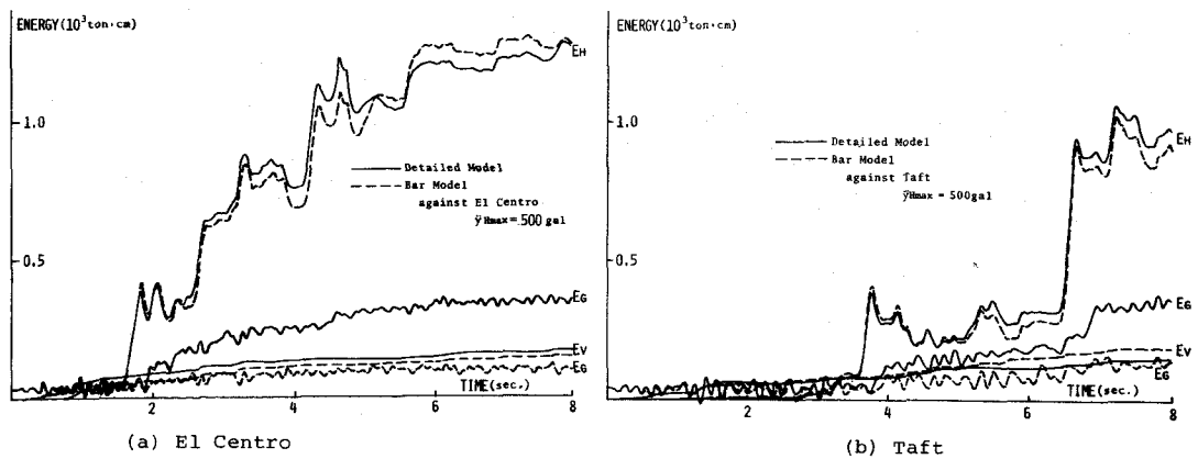
Fig. 6-18 Input Energy Time Histories
