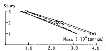
Fig.5-12 (\Delta\theta/h)_{\max} and M_{\max} of 3F2
