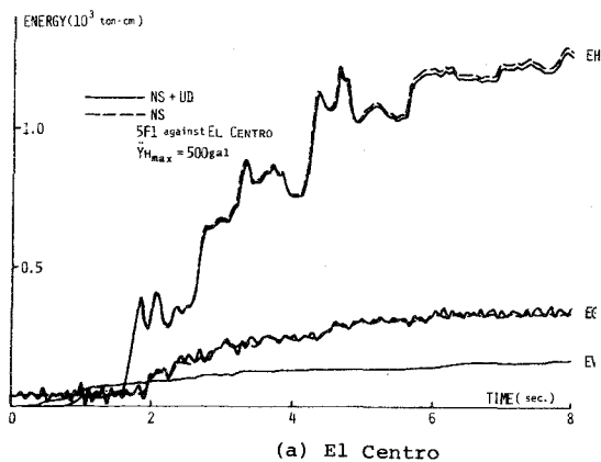
Fig.5-15 Input Energy Time Histories
