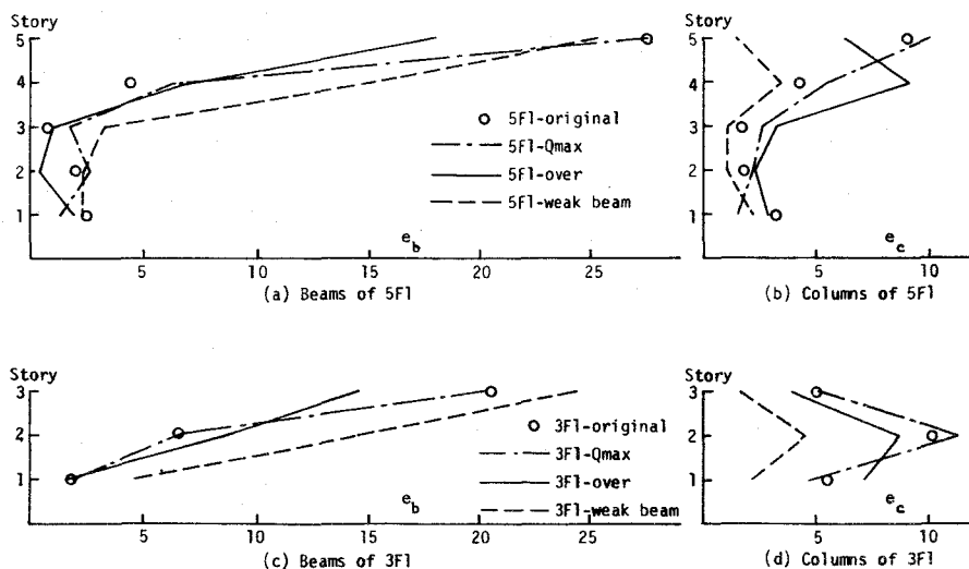
Fig.7-5 Normalized Internal Work Response for Taft
