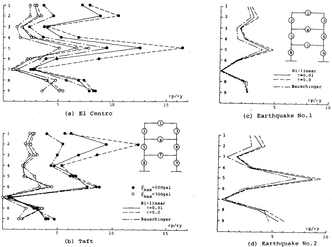
Fig.3-10 Normalized Plastic Strain
