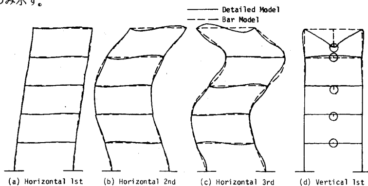
Fig. 6-9 Natural Mode of 5F1
