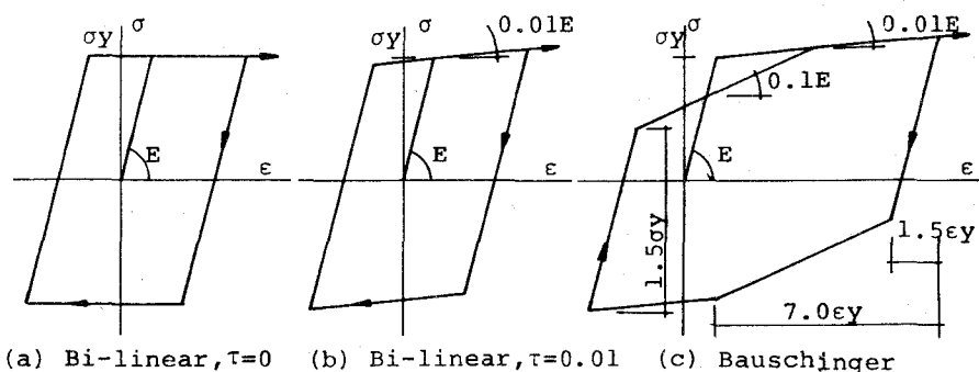
Fig.3-3 Stress-Strain Relations
