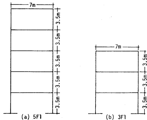
Fig.7-2 Frame Geometry
