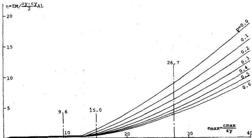
Fig.8-3 \eta - e_{max} Relations of Beams
