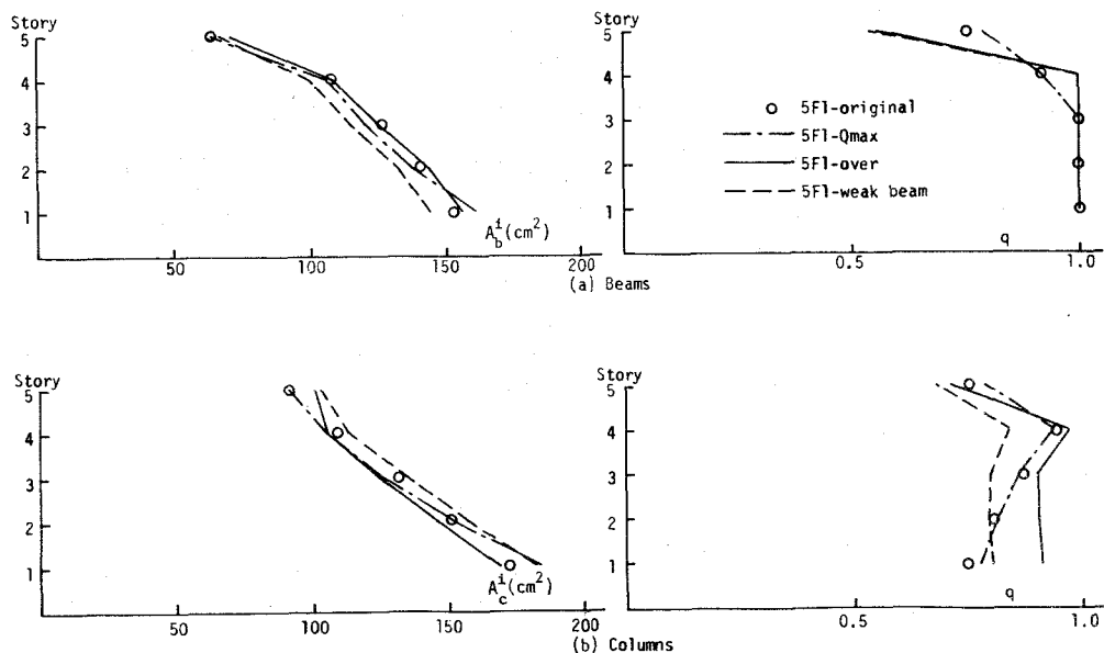
Fig.7-3 Distribution of A^i and q in 5F1
