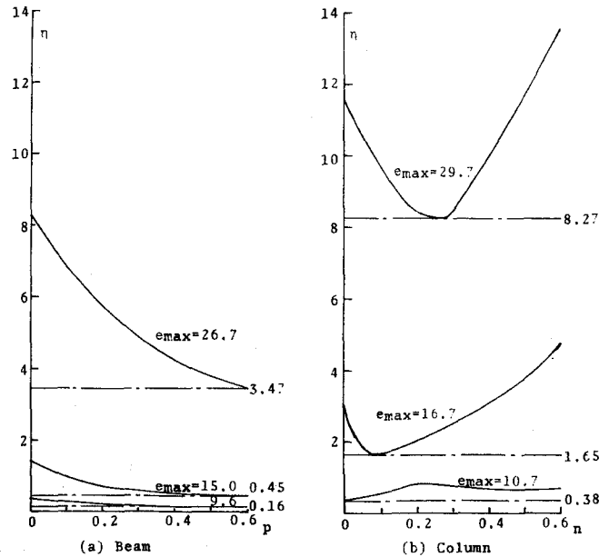
Fig.8-5 Energy Absorption Capacity
