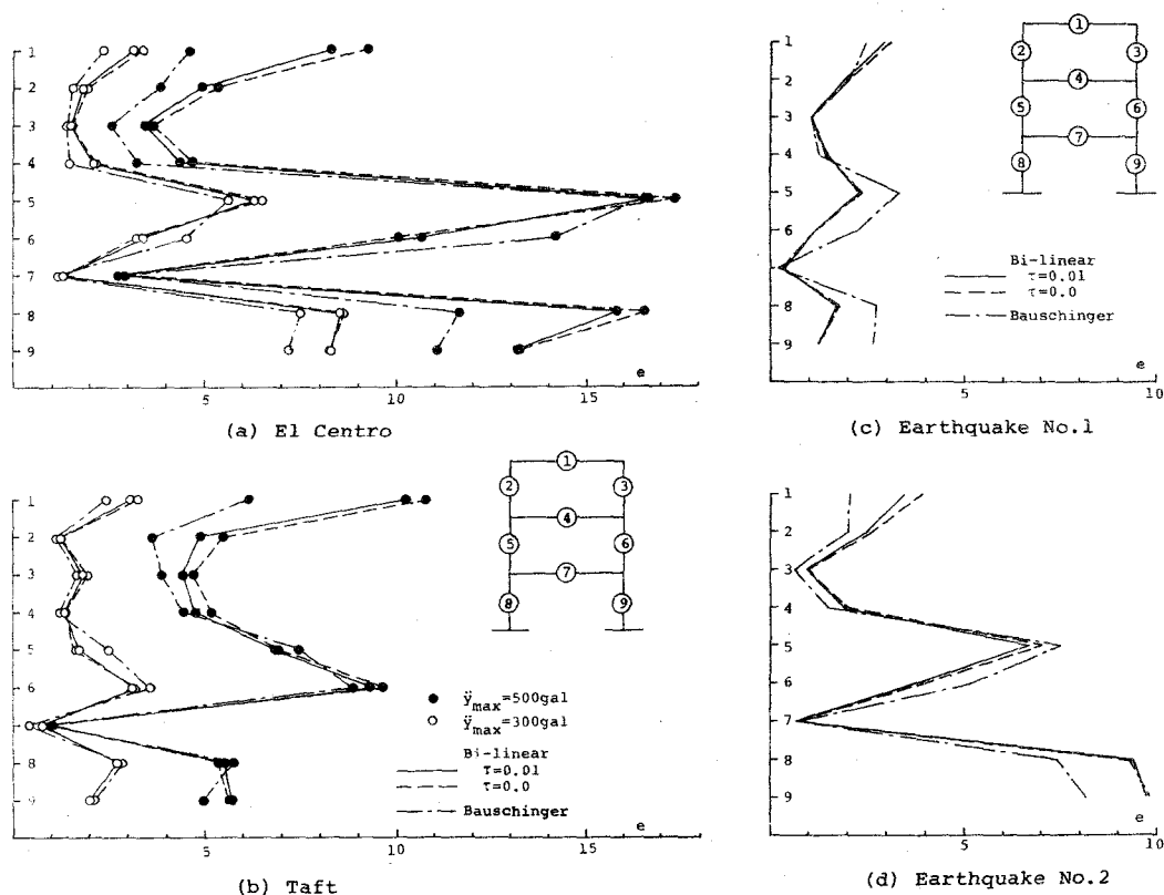
Fig.3-9 Normalized Internal Work
