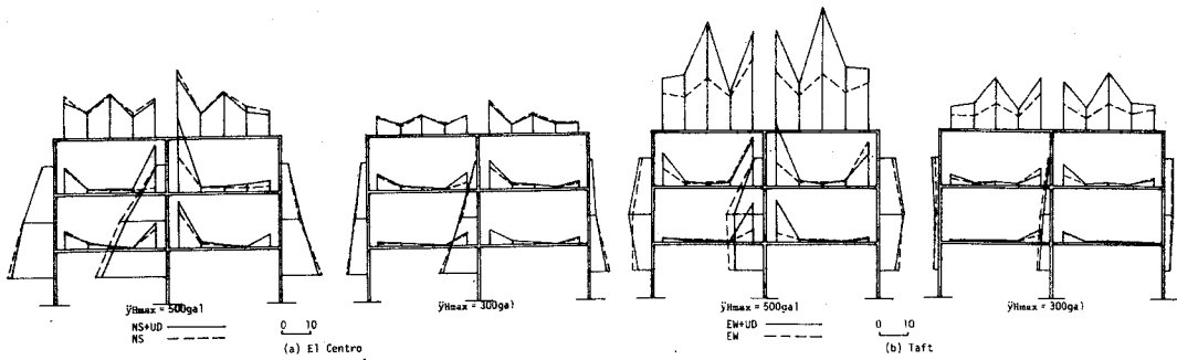
Fig. 5-18 Internal Work Distribution of 3F2
