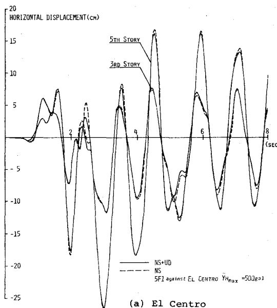
Fig.5-13 Horizontal Displacement Time Histories
