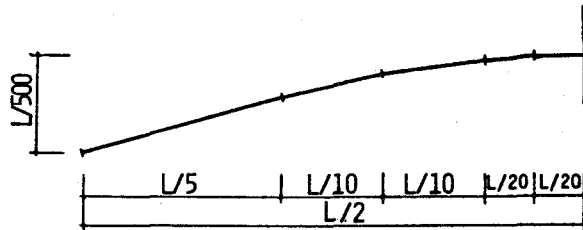
Fig.2-12 Idealized Model for 1-FEM
