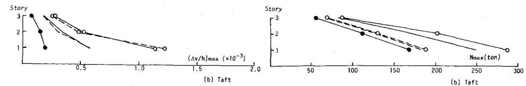
Fig. 5-9 (\Delta v/h)_{\max} and N_{\max} of 3F2
