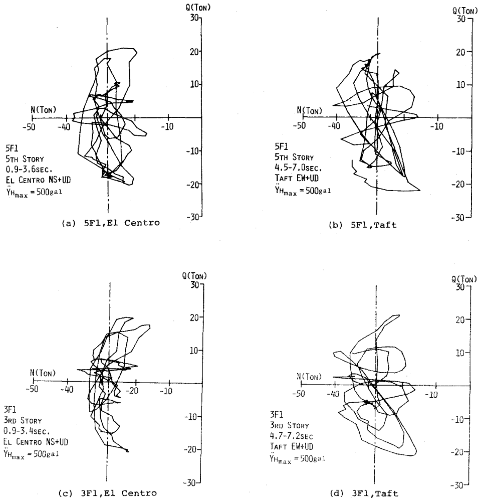
Fig.5-20 N-Q Relations
