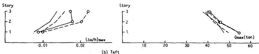
Fig.5-6 (\Delta u/h)_{\max} and Q_{\max} of 3F2
