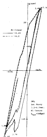
Fig.3-7 Q-( \Delta u/h ) Relations
