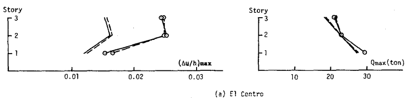
Fig.5-4 (\Delta u/h)_{\max} and Q_{\max} of 5F1
