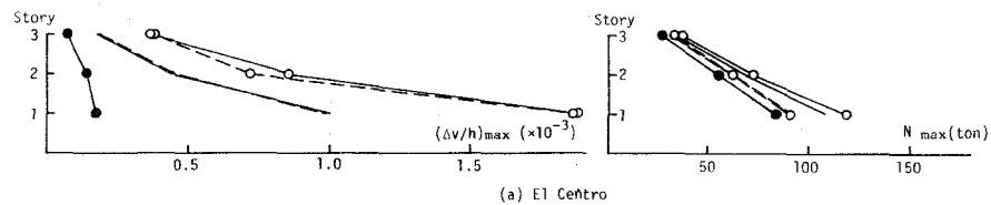
Fig. 5-7 (\Delta v/h)_{\max} and N_{\max} of 5F1
