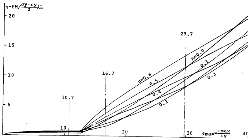
Fig.8-4 \eta - \epsilon_{max} Relations of Columns
