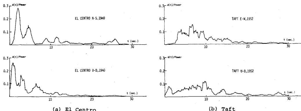
Fig.5-21 Temporal Density of Power
