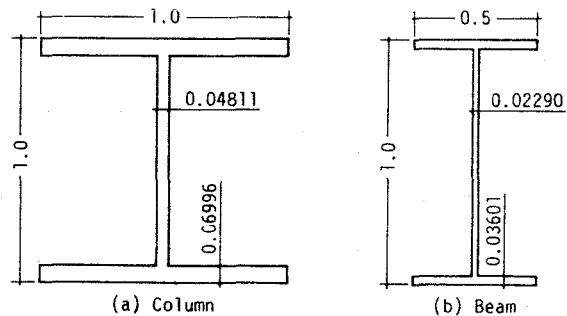
Fig.3-5 Member Size
