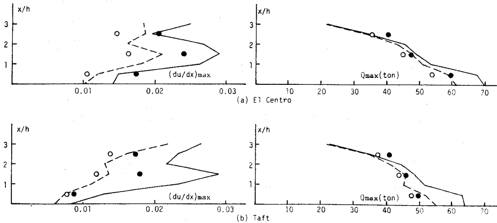
Fig.6-11 (du/dx)_{max} and Q_{max} of 3F2
