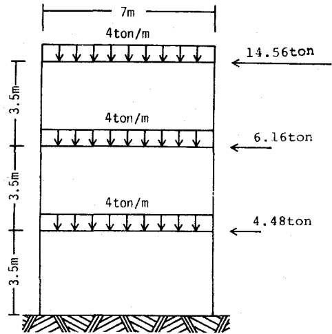
Fig.3-4 Frame Geometry
