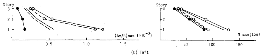
Fig. 5-8 (\Delta v/h)_{\max} and N_{\max} of 3F1
