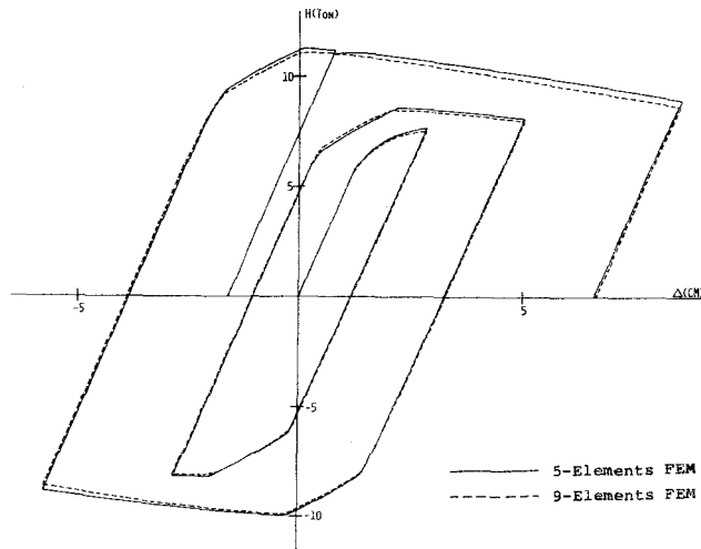
Fig.2-5 Horizontal Force-Displacement Relations
