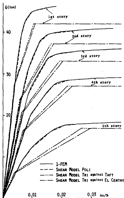
Fig.4-2 One Way Q-( \Delta u/h ) Relations
