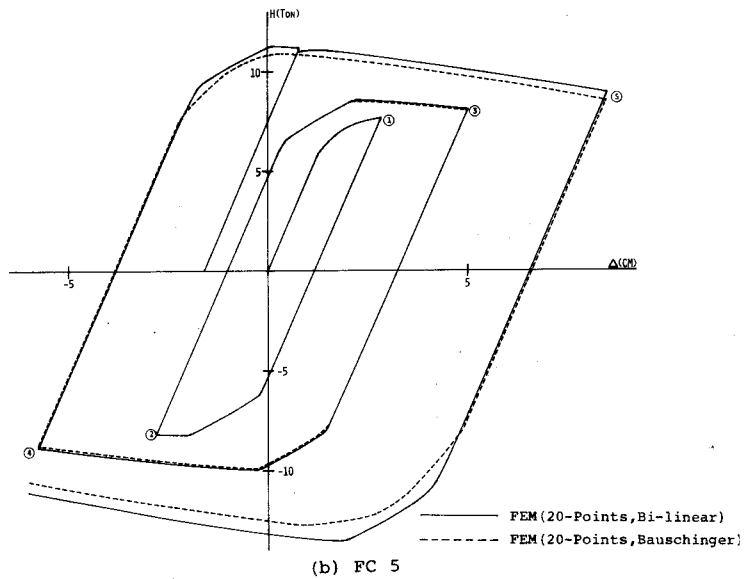
Fig.2-7 Horizontal Force-Displacement Relations
