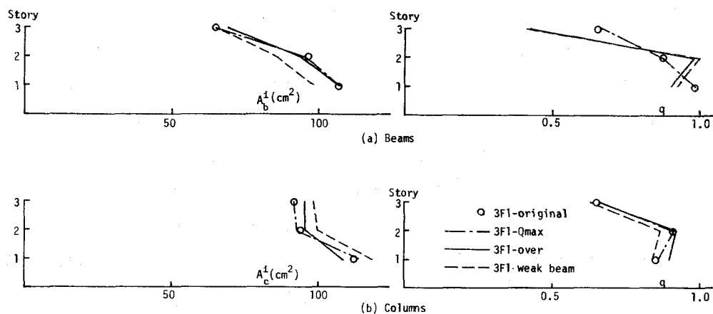
Fig.7-4 Distribution of A^i and q in 3F1
