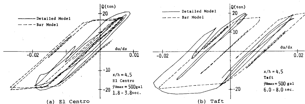
Fig. 6-19 Q-(du/dx) Relations
