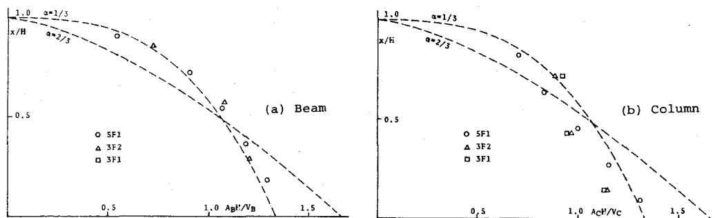
Fig.8-9 Distribution of Cross Sectional Area
