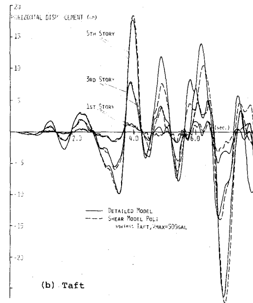
Fig.4-6 Displacement Time Histories
