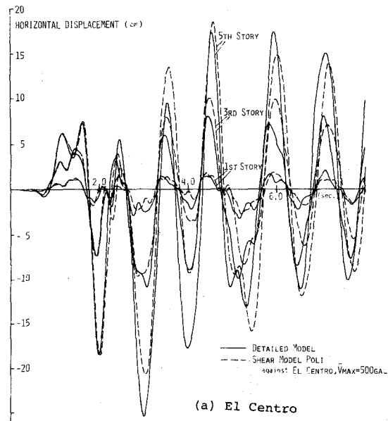
Fig.4-6 Displacement Time Histories
