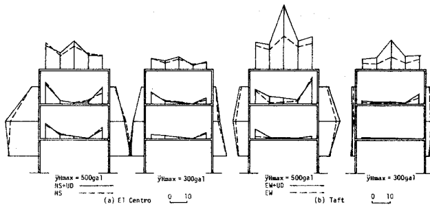
Fig. 5-17 Internal Work Distribution of 3F1
