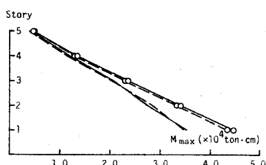
Fig.5-10 (\Delta\theta/h)_{\max} and M_{\max} of 5F1
