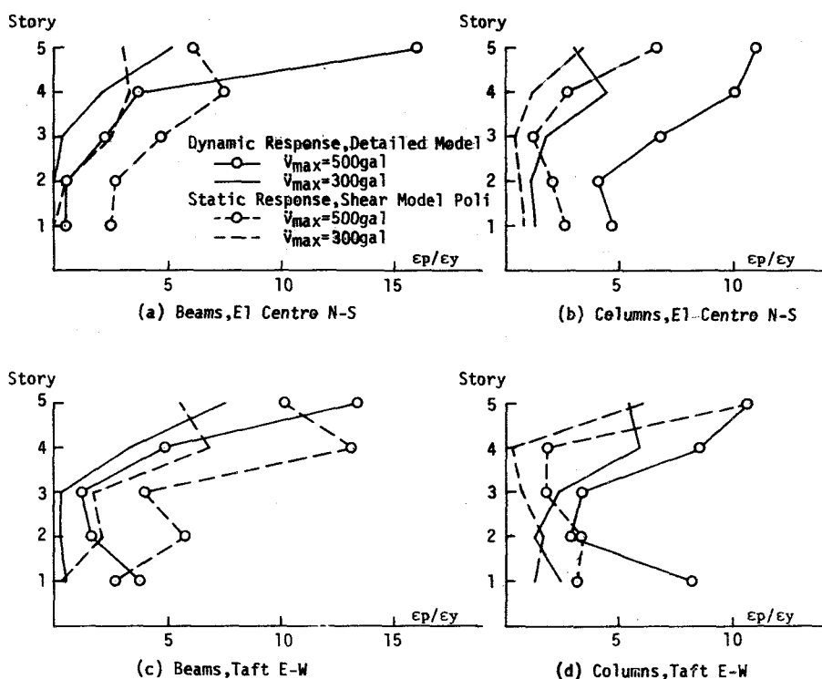
Fig.4-10 Maximum Plastic Strain Responses
