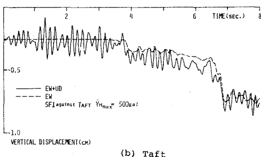
Fig.5-14 Vertical Displacement Time Histories
