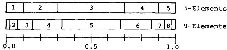
Fig.2-4 Member Division
