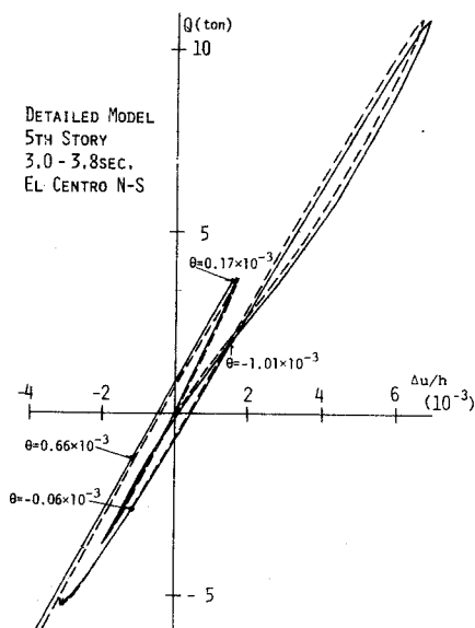
Fig.4-4 Q-( \Delta u/h ) Relation of Elastic System
