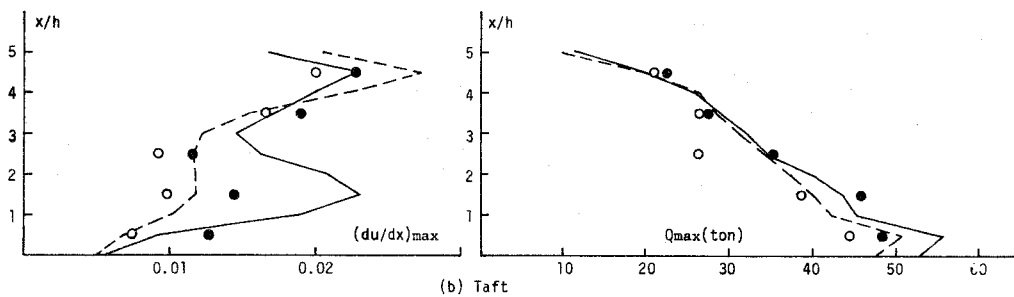
Fig.6-10 (du/dx)_{max} and Q_{max} of 5F1
