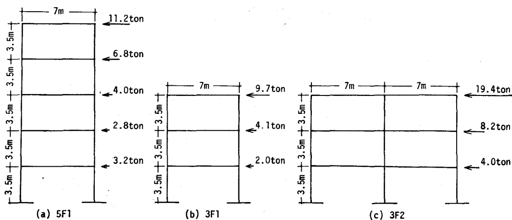
Fig.5-1 Frame Geometry and Seismic Load
