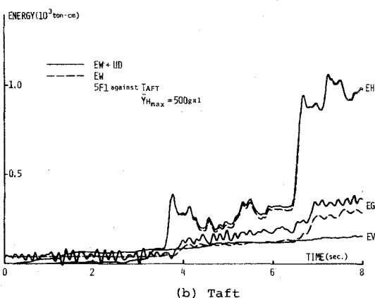
Fig.5-15 Input Energy Time Histories
