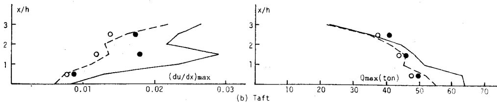
Fig.6-11 (du/dx)_{max} and Q_{max} of 3F2
