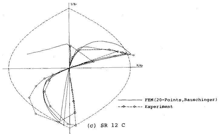
Fig.2-15 Stress Points Trajectory
