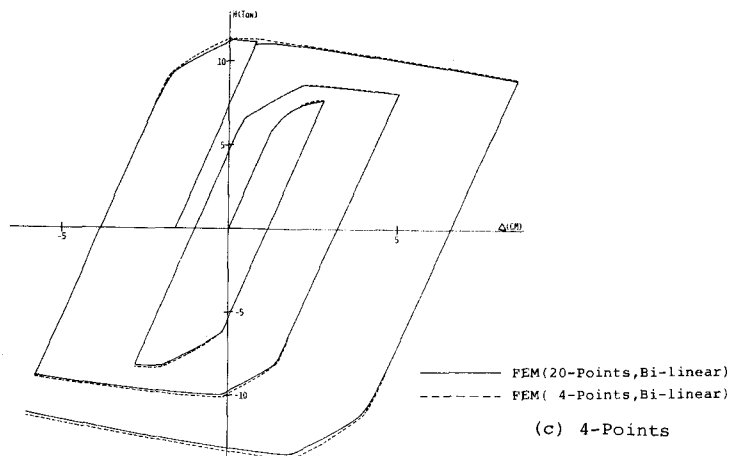
Fig.2-11 Horizontal Force-Displacement Relations of FC 5
