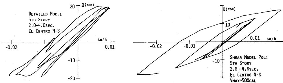
(a) 5th Story for El Centro
