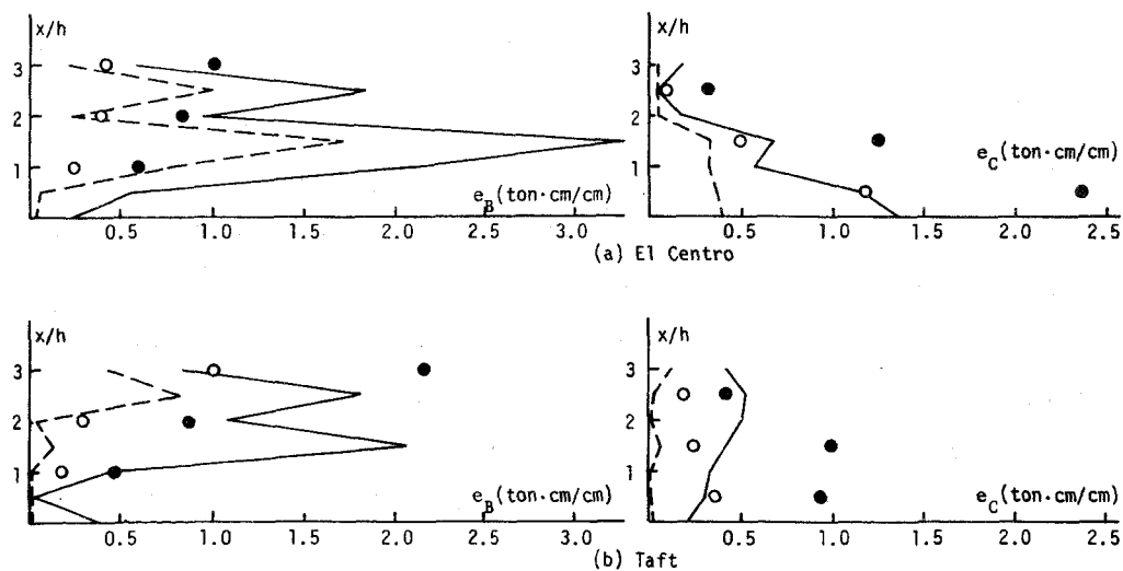
Fig.6-21 Vertical Distribution of Internal Work in 3F2
