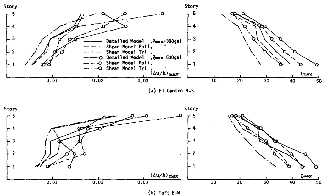
Fig.4-5 Maximum Responses of Elasto-Plastic Systems
