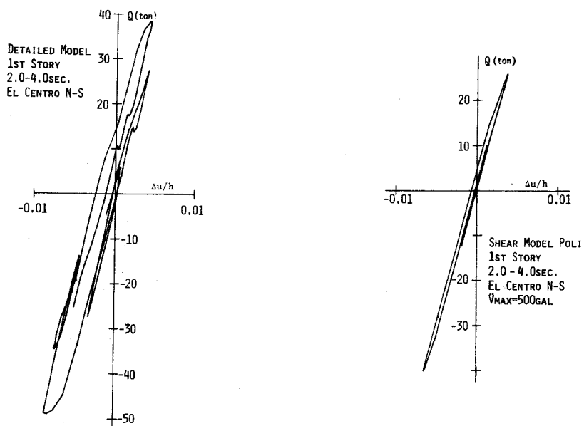
(c) 1st Story for El Centro
