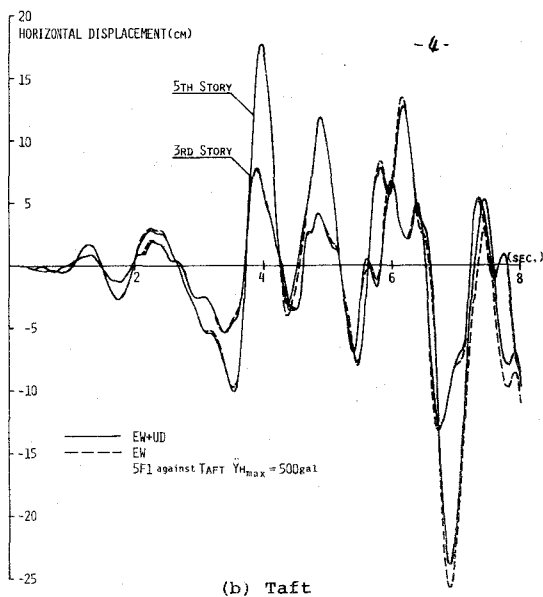
Fig.5-13 Horizontal Displacement Time Histories
