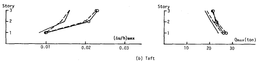
Fig.5-5 (\Delta u/h)_{\max} and Q_{\max} of 3F1
