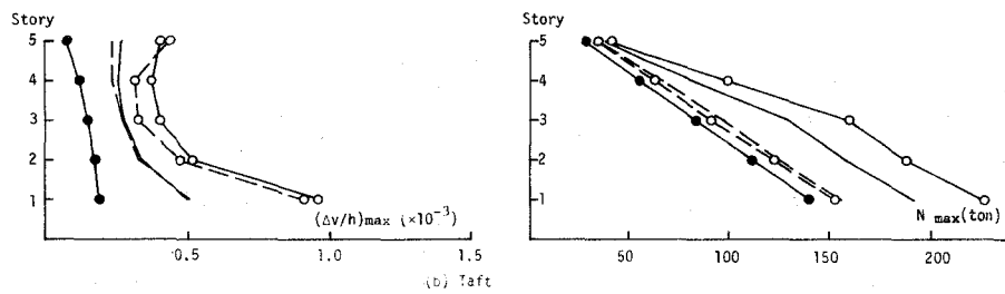
Fig. 5-7 (\Delta v/h)_{\max} and N_{\max} of 5F1
