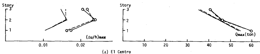
Fig.5-5 (\Delta u/h)_{\max} and Q_{\max} of 3F1
