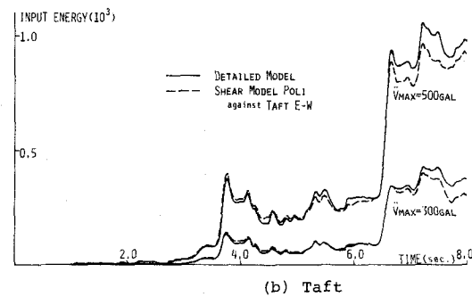
Fig.4-7 Input Energy Time Histories
