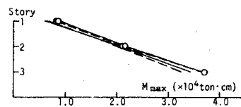
Fig.5-11 (\Delta\theta/h)_{\max} and M_{\max} of 3F1
