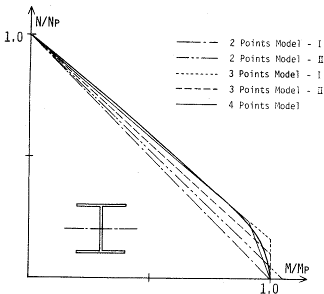
Fig.2-9 Interaction Curve
