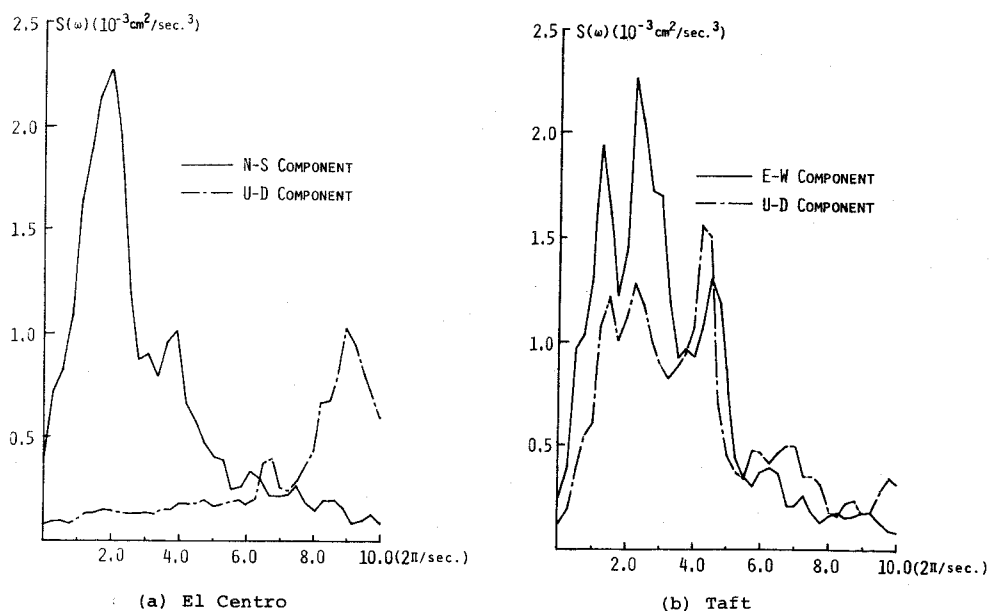
Fig.5-2 Normalized Power Spectral Density
