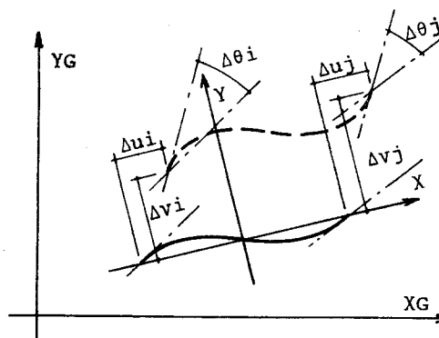
Fig.2-1 Coordinates for an Element
