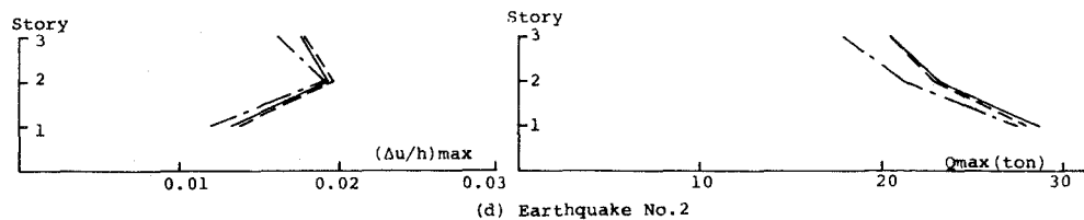
Fig.3-6 (\Delta u/h)_{\max} and Q_{\max}
