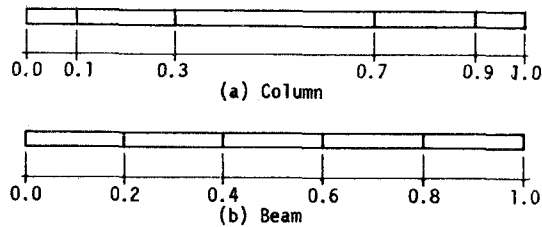
Fig.5-3 Member Division for Analysis
