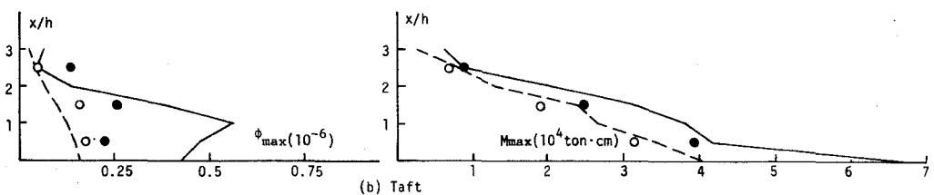
Fig.6-15 \phi_{\max} and M_{\max} of 3F2
