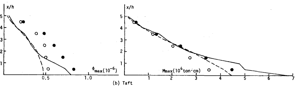
Fig.6-14 \phi_{\max} and M_{\max} of 5F1
