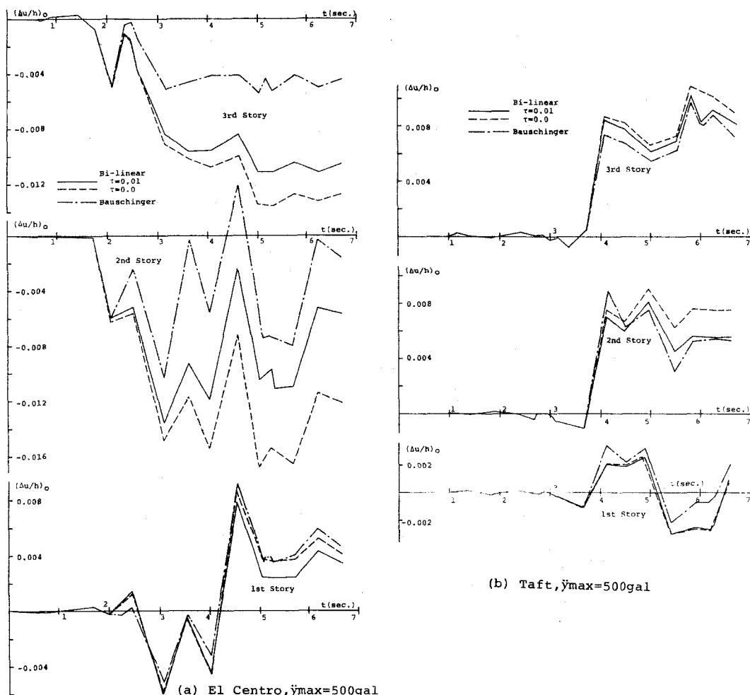
Fig.3-8 (\Delta u/h)_0 Time History
