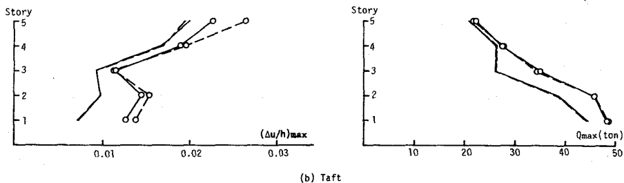
Fig.5-4 (\Delta u/h)_{\max} and Q_{\max} of 5F1
