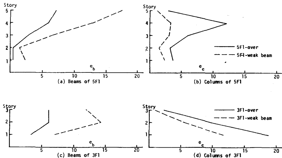
Fig.7-7 Normalized Internal Work Response for El Centro
