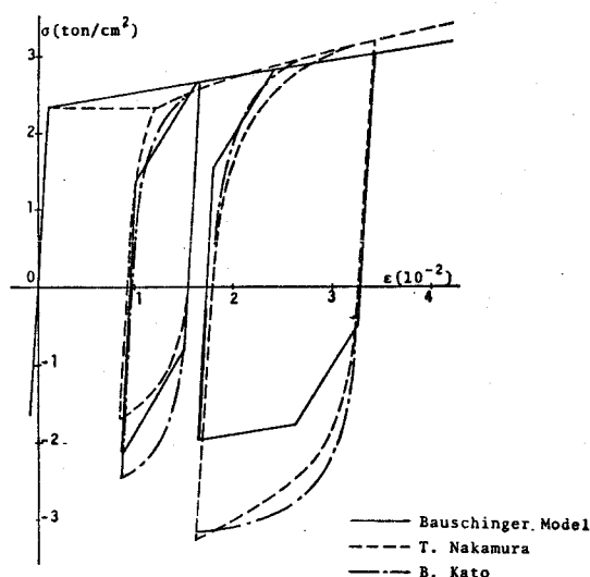
Fig.2-14 Stress-Strain Relations
