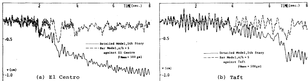
Fig. 6-17 Vertical Displacement Time Histories
