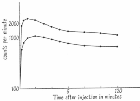
Fig. 1 Counting rate over normal area during first two hours after intravenous injection of ^{32}\text{P}
