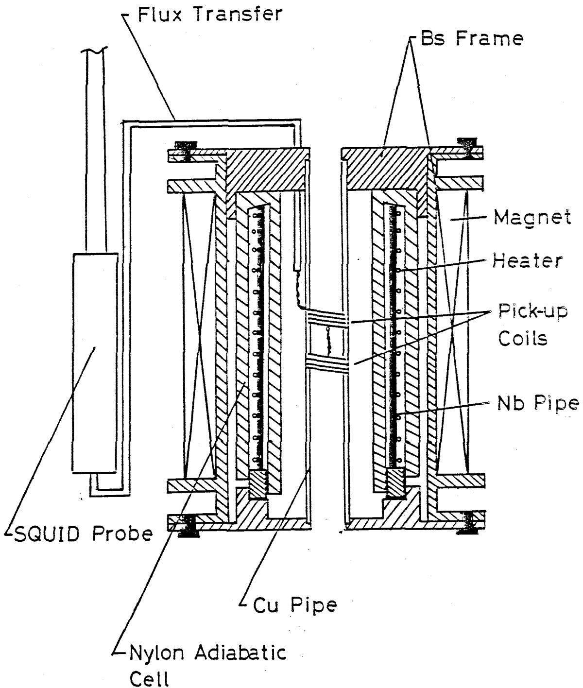
Fig. 3 Main portion of the SQUID magnetometer. The equipment is immersed into liquid He bath.
