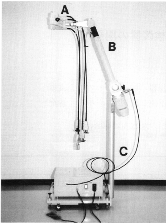
Fig.1 Illustration of our newly-developed equipment for CT-guided biopsy. This equipment is composed of three parts. A: needle holder part B: arm part C: supporting part
