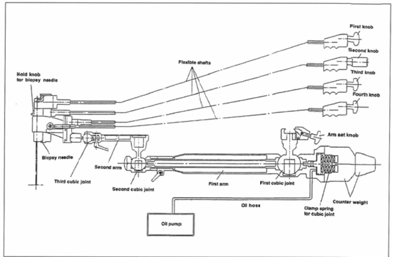
Fig.2 Detailed illustration of the needle holder part and the arm part.
