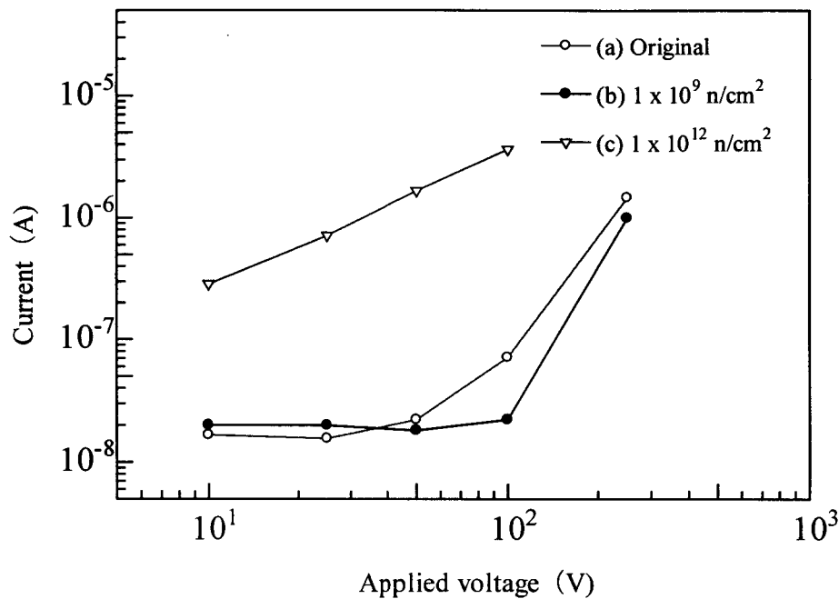
Fig. 5.3 Current-voltage characteristics of the CdTe detectors.
