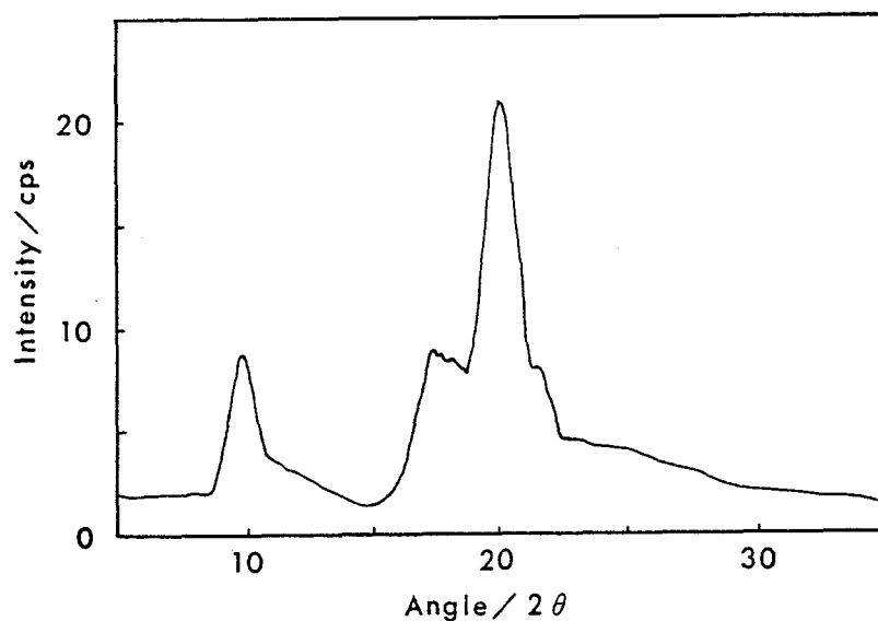
Fig. 12. X-ray diffraction pattern of 5% poly-1-butene gel in toluene formed by quenching rapidly to 0^\circ\text{C} , at 20^\circ\text{C} .
