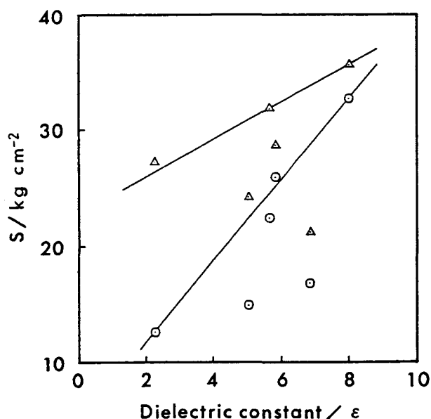
Fig. 2. Plots of the adhesive strength against the electric constant of the solvents as a function of the irradiated time; \circ —: 7 min, \triangle —: 8 min.
