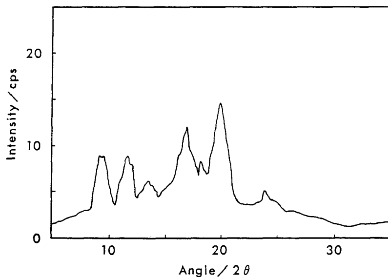
Fig. 13. X-ray diffraction pattern of 5% poly-1-butene gel in toluene formed by quenching rapidly to -195^\circ\text{C} , at 20^\circ\text{C} .
