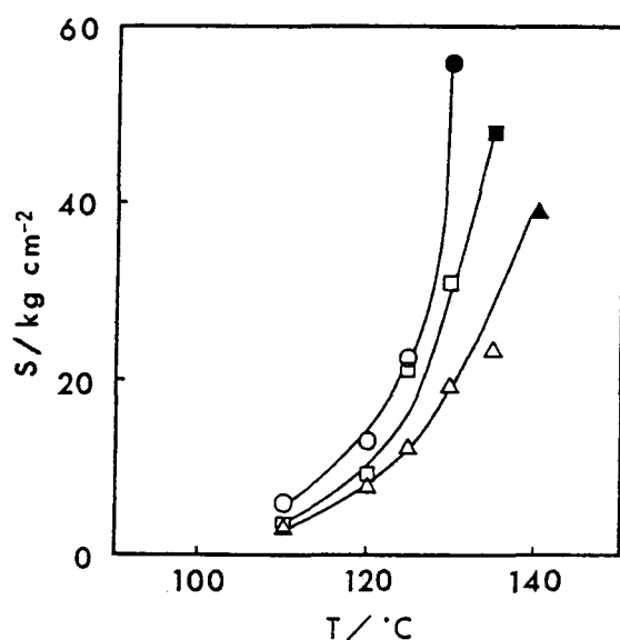
Fig. 1. Effects of the heating temperature on the adhesive strength of various gels in tetralin; -\bigcirc- : PP-1, -\square- : PP-2, -\triangle- : PP-3. Filled symbols represent the results of polypropylene plates themselves giving rise to necking.
