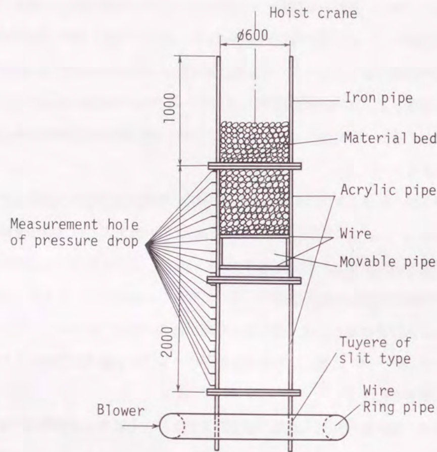
Fig. 2.1 Experimental apparatus.
