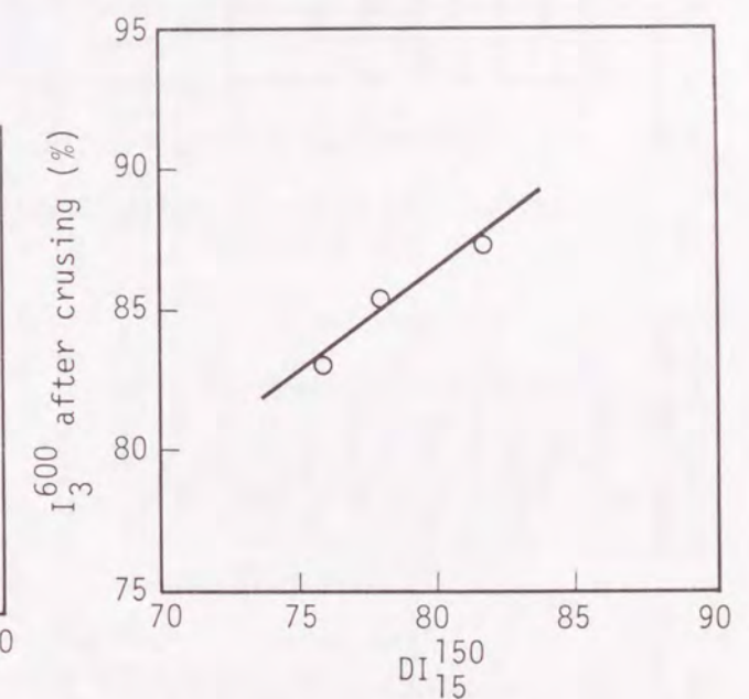
Fig. 6.6 Relationship between coke strength DI_{15}^{150} and I_3^{600}
