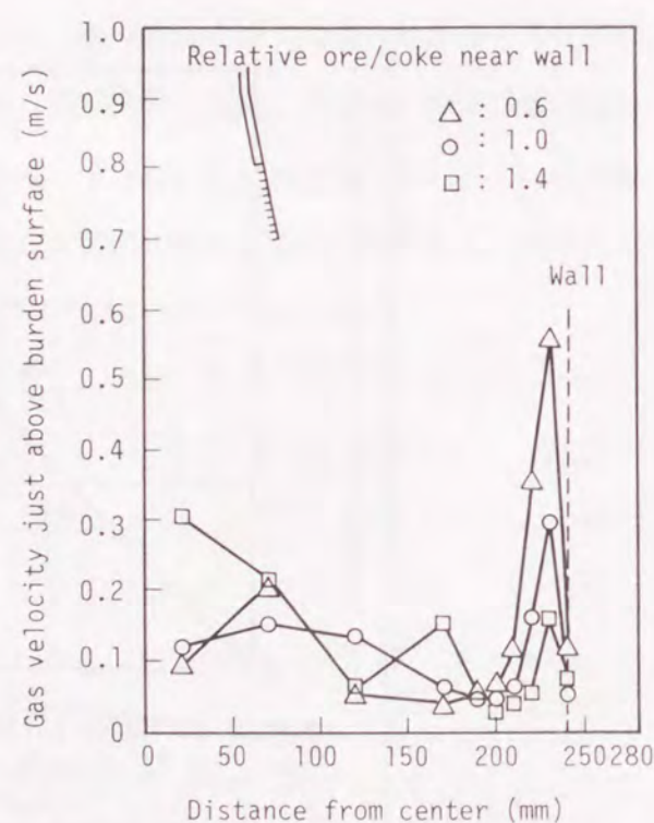
Fig. 5.15 Influence of relative ore/coke near wall (95mm from wall) on gas velocity distribution just above burden surface in case of rugged wall profile and small ore ( d_p: 0.5 \sim 1.0\text{mm} ) ratio=20%.
