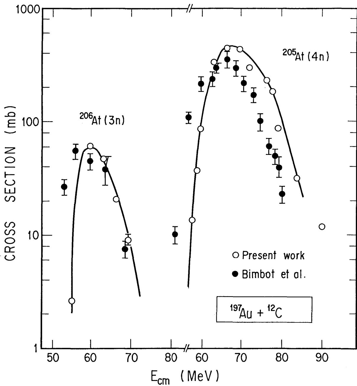
Fig.3.6(a). Excitation functions for At nuclides produced in the xn reactions ( x=3,4 ) induced by ^{12}\text{C} . Absolute errors for the cross sections are within the size of the marks in the figure. The data by Bimbot et al. [28] corrected with the decay properties in [33] are shown as well.
