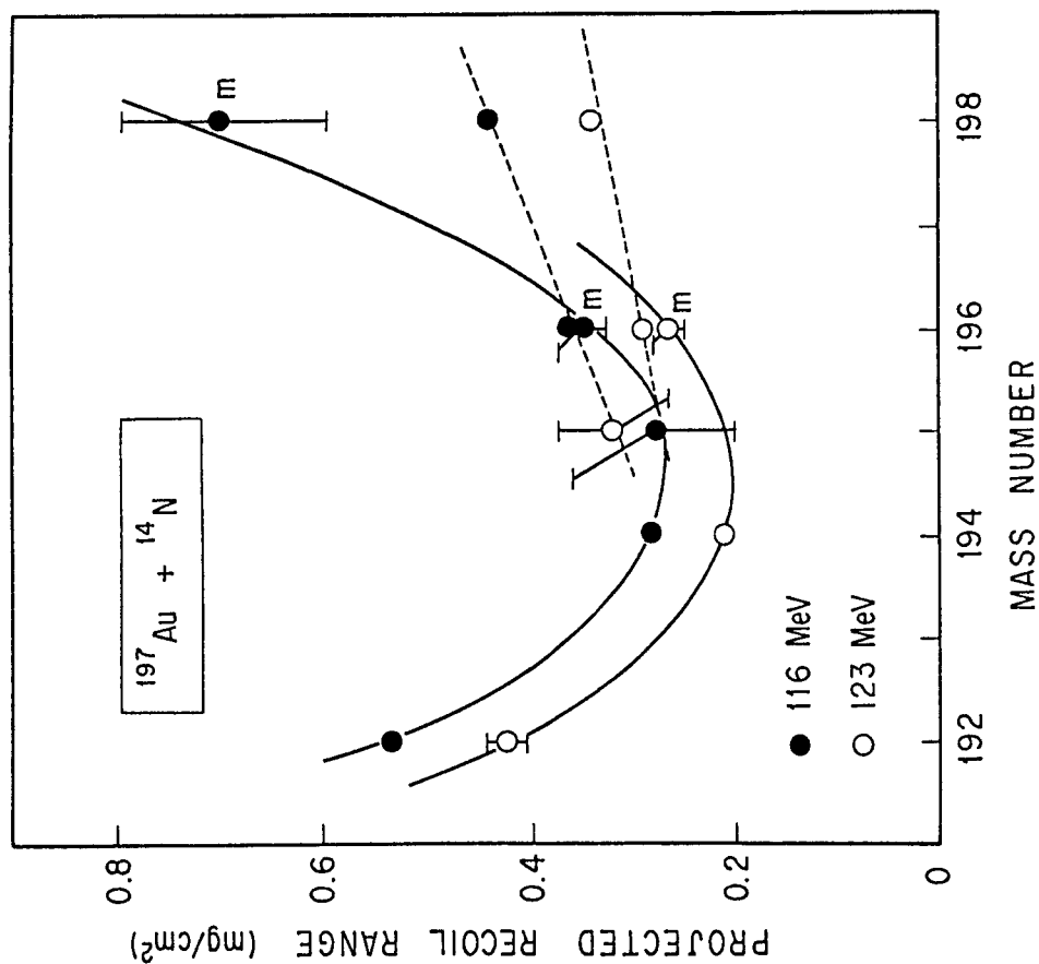
Fig.2.11. Mean projected recoil ranges as a function of mass number of Au nuclides in the ^{14}\text{N} - and ^{12}\text{C} -induced reactions. The bombarding energies were 116MeV and 123MeV for the ^{14}\text{N} -induced reaction and 86MeV, 92MeV, and 114MeV for the ^{12}\text{C} -induced reaction. According to the idea distinguishing products of QET and DIT in 2.4.1, dashed lines through recoil ranges of the isotopes produced by QET and solid lines through those of the isotopes produced by DIT are drawn.
