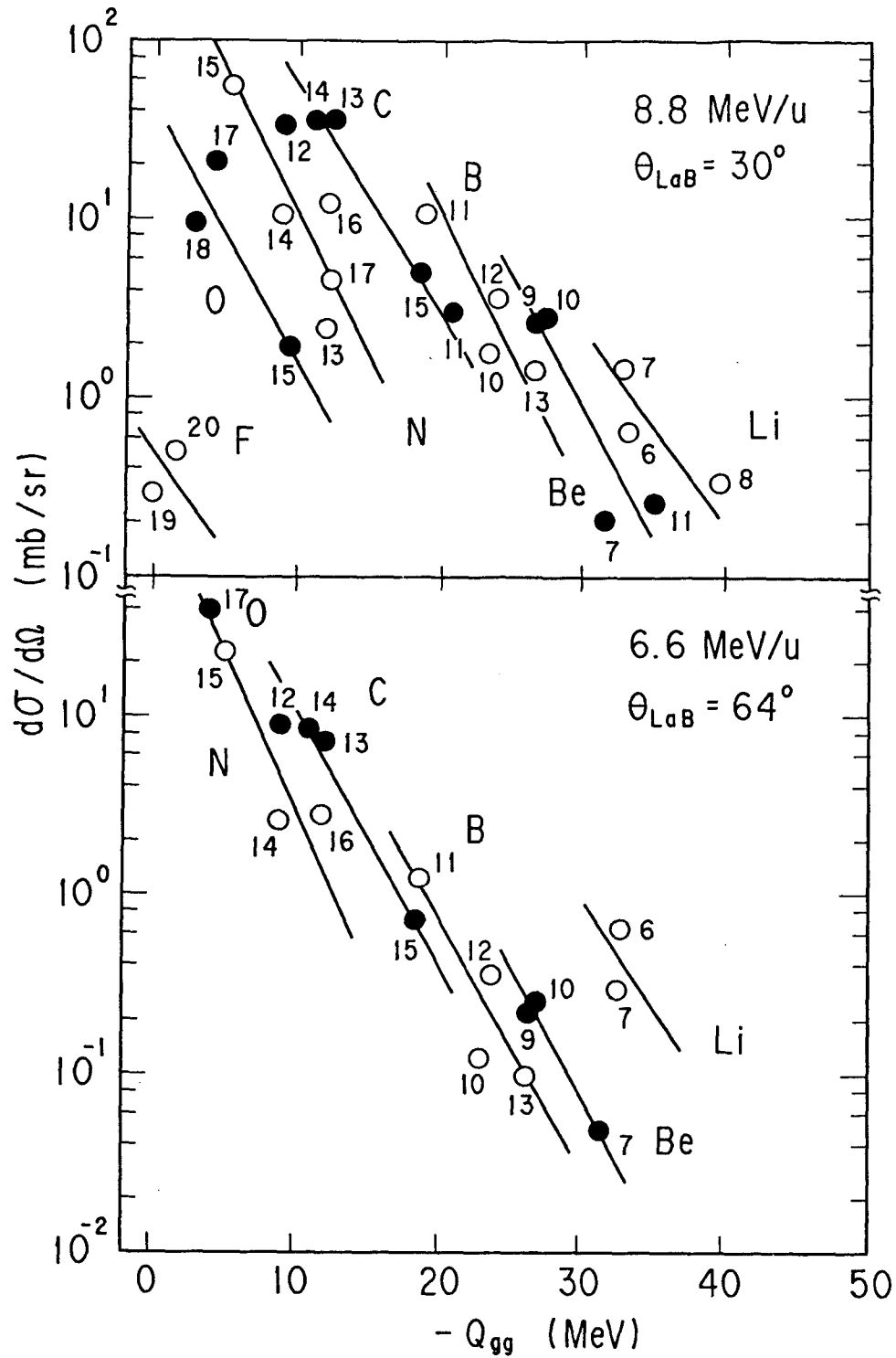
Fig.2.45. Q_{gg} systematics of the isotopic differential cross sections at 30^\circ for the 8.8MeV/u system and at 64^\circ for the 6.6MeV/u system. The straight lines are drawn through the isotopic cross sections.
