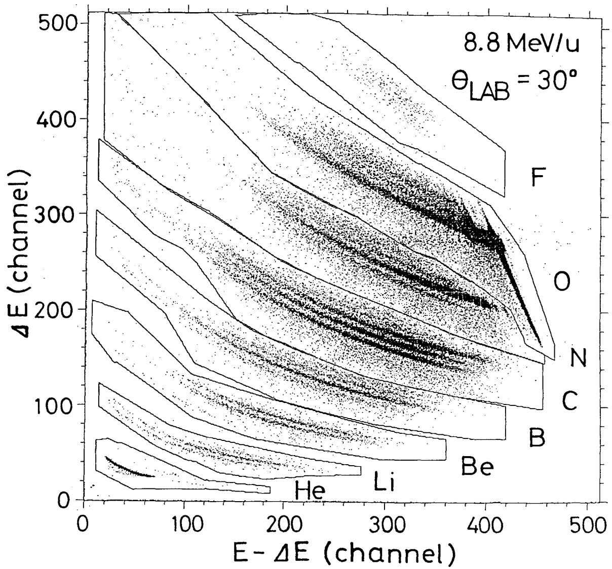
Fig.2.19. A typical (E - \Delta E) - \Delta E map of emitted particles measured at 30^\circ in the laboratory system for the 8.8 MeV/u ^{16}\text{O} -induced reaction.
