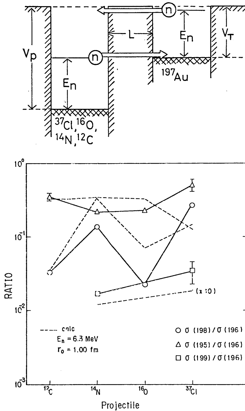
Fig.2.15. Cross section ratios of the quasi-elastic transfer products. Solid lines are drawn through the experimental values, while dashed lines represent the values calculated with a extended tunneling model. The model is illustrated schematically in the top. See text for the parameters E_n and r_0 .
