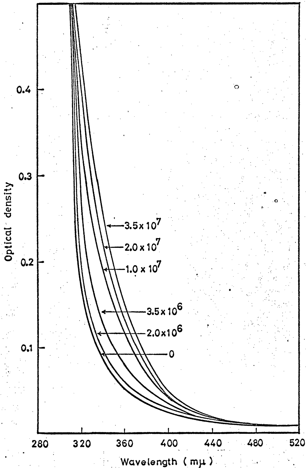
Fig. 4.2.6 Optical density of celluloid film irradiated with ^{60}\text{Co} \gamma -rays as function of UV wavelength Doses are in rad.
