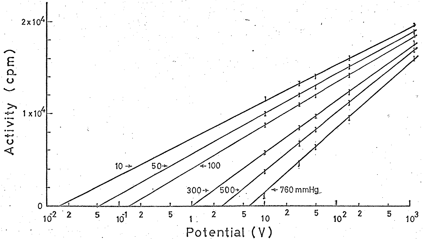
Fig. 3.3 Variations of deposited activity of ^{208}\text{Tl} according to applied potential, with pressure as parameter (source(+), target(-), and interval 2 cm)
