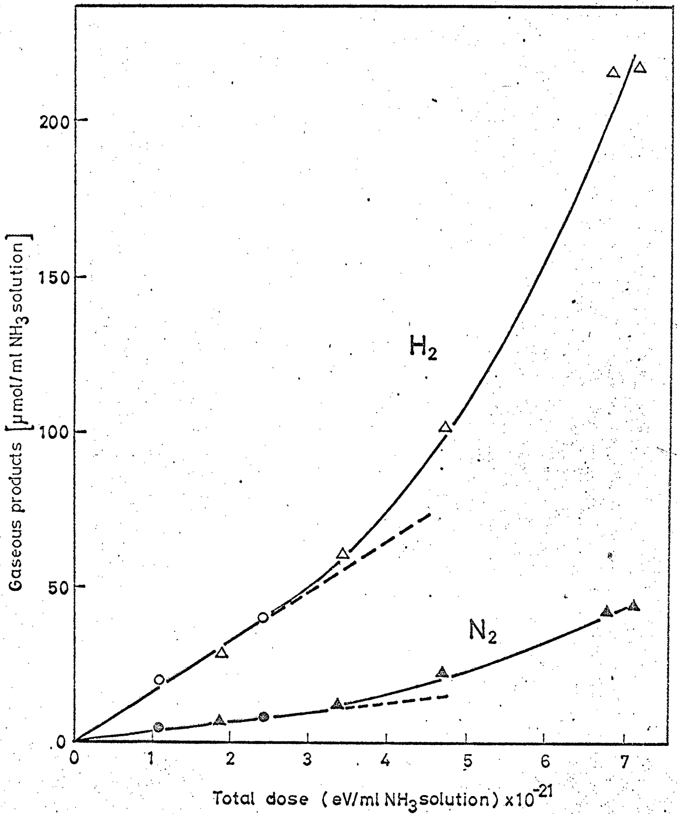
Fig. 5.3 Yields of gaseous products from 15 M ammonium hydroxide without additive (○) and with NH 4 BF 4 (△) in the Slant ○, △: H 2 ●, ▲: N 2
