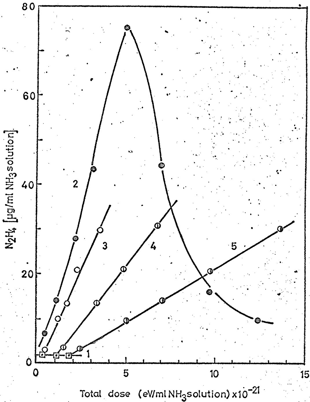
Fig. 5.2 Effect of ^{10}B(n,\alpha)^7Li reaction on 15 M ammonium hydroxide solution
