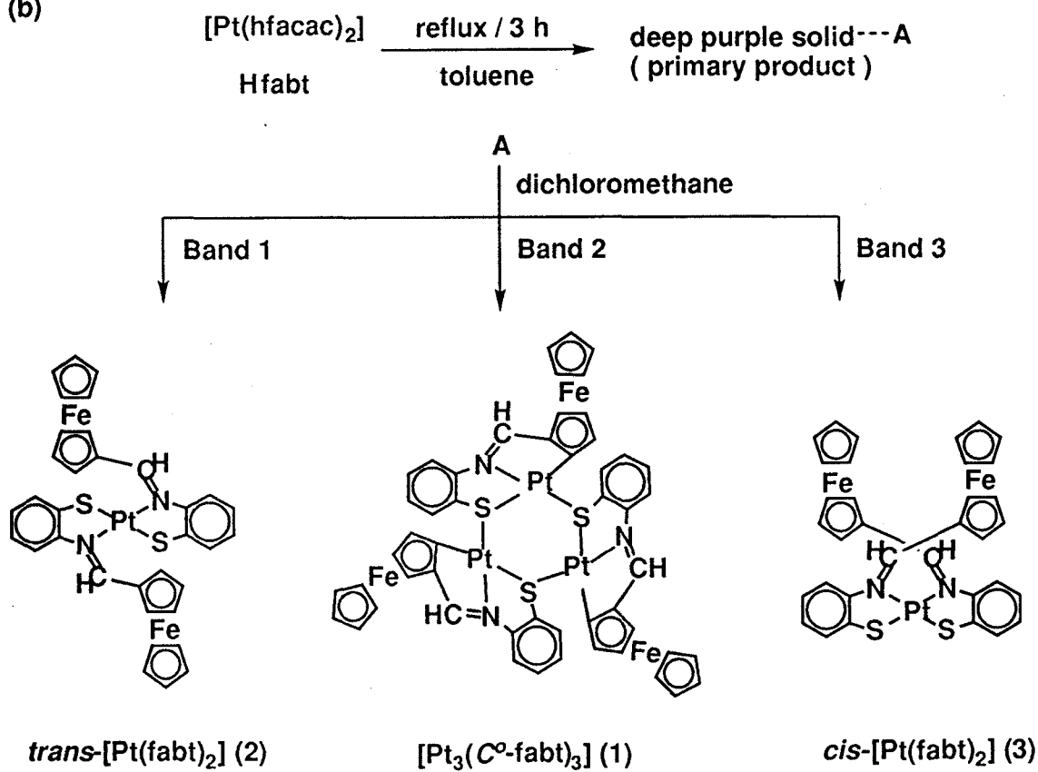
Scheme 2. The reaction of [\text{Pt}(\text{hfacac})_2] with Hfabt (a) in 1:1 (b) in 1:2 stoichiometry ratio.
