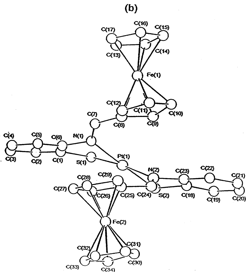
Fig. 3. Molecular structures of 3 (a) top view, (b) side view.
