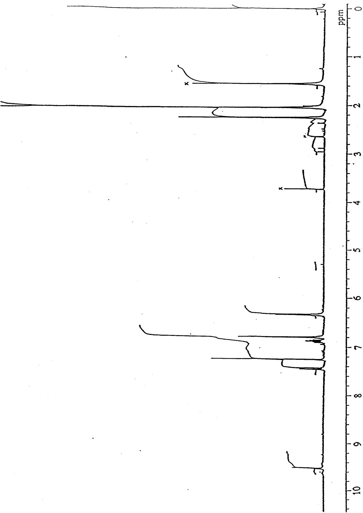
Fig. 3. ^1\text{H} NMR spectrum of 2 in \text{CDCl}_3 solution.
