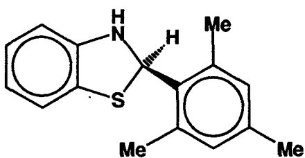
2-(2,4,6-trimethylphenyl)benzothiazoline H2,4,6Me-phbt
