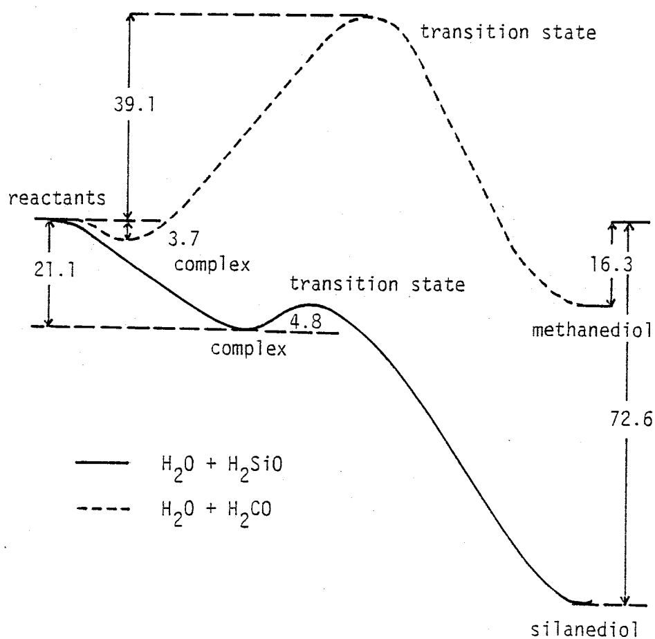
Figure 7. Energy profiles(kcal/mol) at the MP3/6-31G* level at the H 2 O + H 2 SiO(full line) and H 2 O + H 2 CO(dotted line) reactions.'
