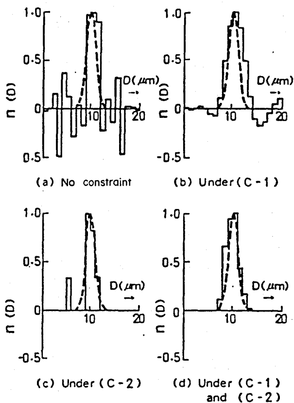
図4. 3 (C. 1), (C. 2) の条件を付加した効果
