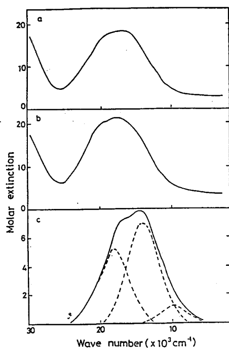
Fig. 3-3 Optical absorption spectra of chromium ions in soda silicate slags containing 0.5mol % \text{Cr}_2\text{O}_3 produced in CO gas.
