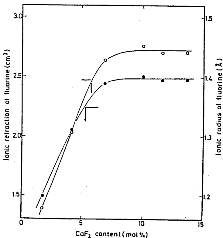
Fig. 4-7 Dependence of ionic refraction of fluorine in x\text{CaF}_2 \cdot (1-x)\text{CaO} \cdot \text{SiO}_2 slags on \text{CaF}_2 content. Dependence of ionic radius determined using the Kordes equation 11 .
