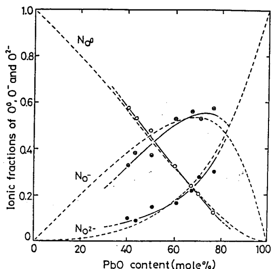
Fig. 2-6 Ionic distributions of three sorts of oxygens in the PbO-SiO_2 slags. The broken lines show the curves calculated using the equations after Kapoor and Froberg with K=0.2 12 .
