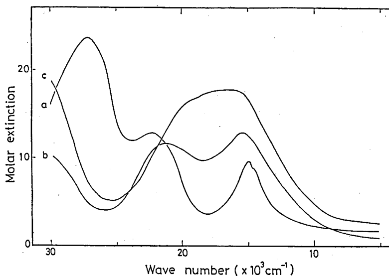
Fig. 3-2 Optical absorption spectra of chromium ions in soda silicate slags with \text{Na}_2\text{O}/\text{SiO}_2 = 2/8 and 0.5 mol % \text{Cr}_2\text{O}_3 produced under various partial oxygen pressures.
