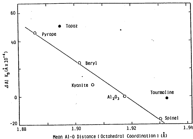
Fig. 1-20 Relation between chemical shift of \Delta Al K_\beta and mean Al-O distance.
