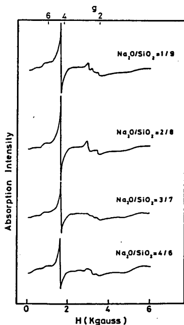
Fig. 5-8 ESR spectra of soda silicate slags with iron and sulphur produced in the \text{CO}/\text{CO}_2 mixed gas with \text{Po}_2 = 10^{-5.1} \text{ atm} . (No. 7, No. 8, No. 9 and No. 10 slags, see Table 5-1)
