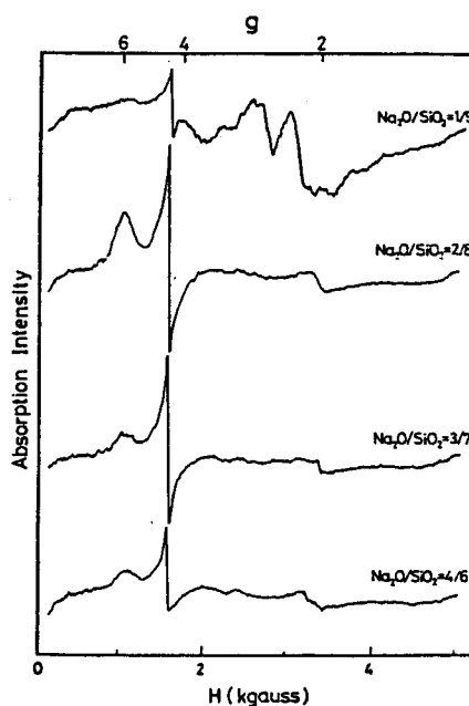
Fig. 5-9 ESR spectra of soda silicate slags with sulphur and iron produced in the \text{CO}/\text{CO}_2 mixed gas with \text{Po}_2 = 10^{-6.7} \text{ atm} .
