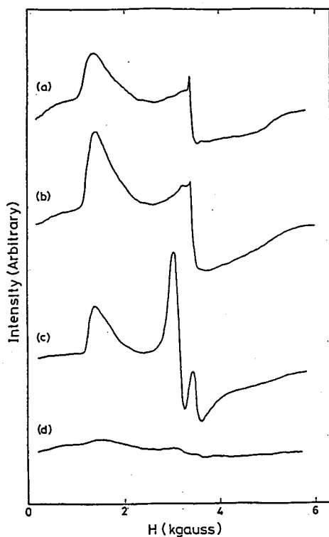
Fig. 3-7 ESR spectra of chromium ions in soda silicate slags with \text{Na}_2\text{O}/\text{SiO}_2=2/8 and 0.5 mol % \text{Cr}_2\text{O}_3 produced under various partial oxygen pressures. a: in air, b: in the mixed gas with \text{CO}/\text{CO}_2=1/100 , c: in the mixed gas with \text{CO}/\text{CO}_2=1 , d: in CO gas.
