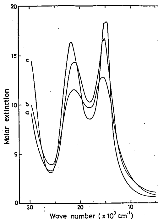
Fig. 3-4 Optical absorption spectra of chromium ions in soda silicate slags containing 0.5mol % \text{Cr}_2\text{O}_3 produced in the mixed gas with CO/CO 2 =1.
