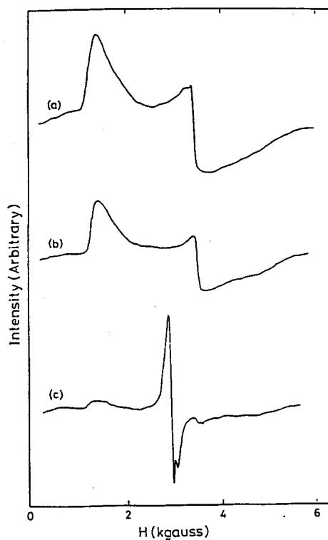
Fig. 3-8 Dependence of ESR spectra on the chromium content in soda silicate slags with \text{Na}_2\text{O}/\text{SiO}_2=2/8 produced in the atmosphere with \text{CO}/\text{CO}_2=1/100 . a: 0.5 mol % \text{Cr}_2\text{O}_3 , b: 0.05 mol % \text{Cr}_2\text{O}_3 , c: 0.005 mol % \text{Cr}_2\text{O}_3 .
