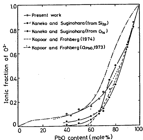
Fig. 2-7 Comparison among distributions of free oxygens determined with various methods. 15,17,18 The activity of \text{PbO} determined theoretically is also shown. 13
