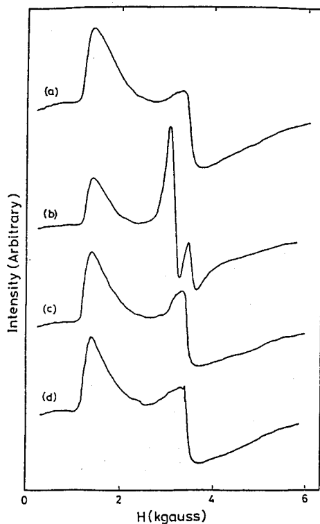
Fig. 3-6 ESR spectra of chromium ions in soda silicate slags with 0.5 mol % \text{Cr}_2\text{O}_3 produced in the mixed gas with \text{CO}/\text{CO}_2 = 1 .
