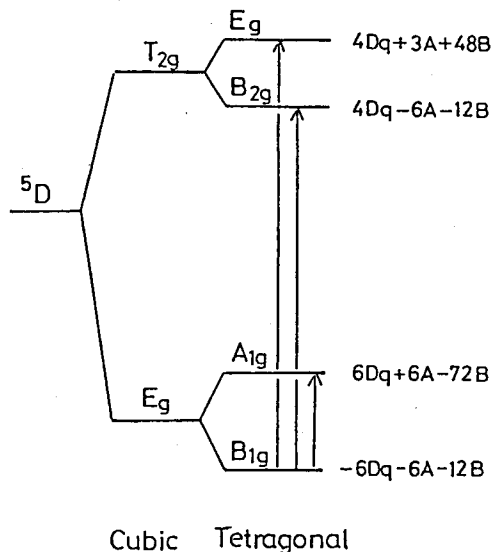
Fig. 3-9 Energy levels of 3d^4 configuration in cubic and tetragonal crystal fields calculated by the point charge model. ( A=2e^2\partial r^2/7a^4 , B=-2e^2\partial r^4/63a^6 , where r is the distance of a 3d electron from the origin, a is the interionic distance, e is the electronic charge and \partial is a small distortion of the octahedron.)
