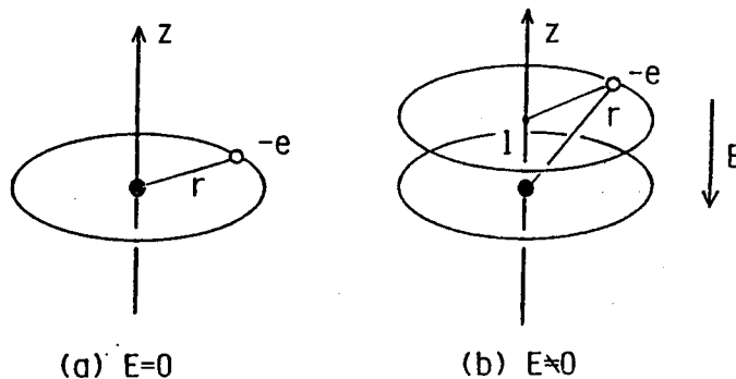
Fig. 1-1 Explanation of polarizability by Bohr model.
