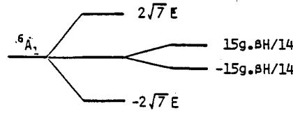
(c) D = 0, E \neq 0, S_z \parallel H
