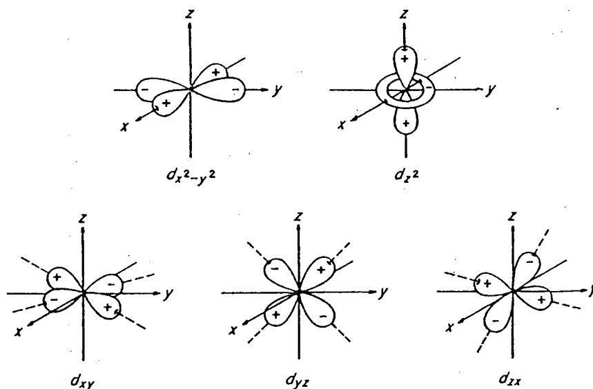
Fig. 1-2 Schematic orbitals of d electrons.
