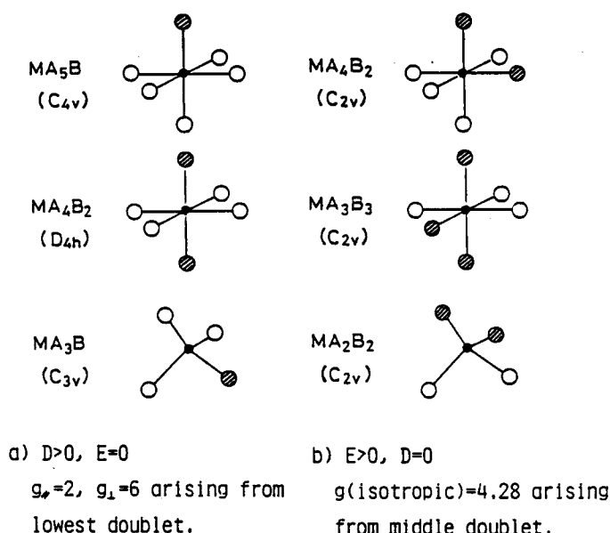
Fig. 5-12 Some environments associated with resonance at g = 6.0 and g = 4.28 . (Symmetry of each complex is shown in each parenthesis.)
