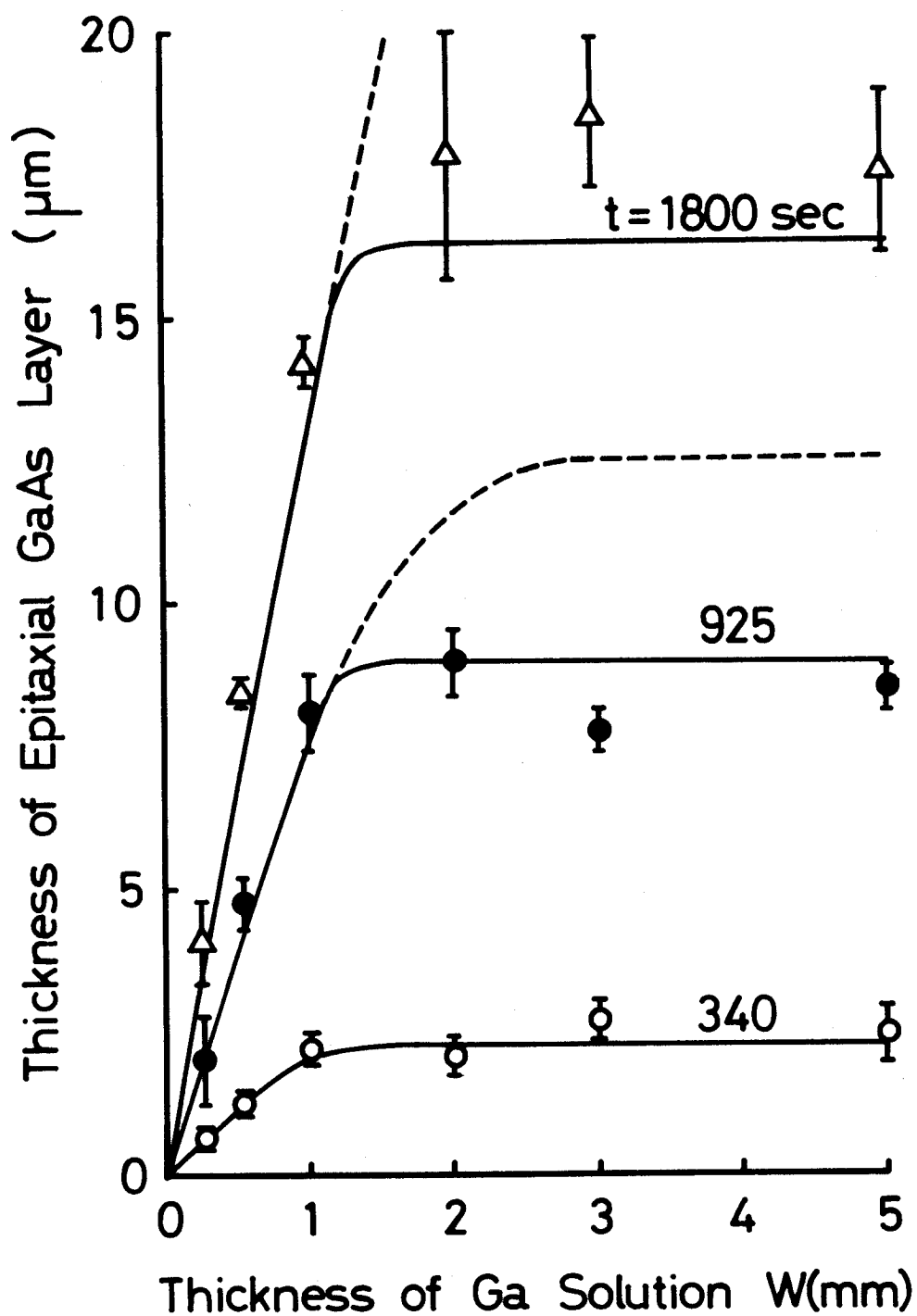
Fig. 4. Thickness of LPE GaAs layer versus thickness of Ga solution for growth durations t of 340, 925, and 1800 sec.
