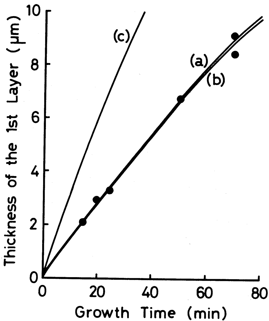
Fig. 16. Thickness of the first layer versus growth time. Solid circles are the experimental data and curves are the calculated results for cases (a) diffusion only with dummy crystal, (b) boundary layer diffusion with dummy crystal, and (c) diffusion only without dummy crystal.
