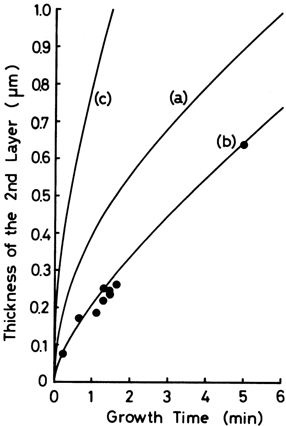
Fig. 17. Thickness of the second layer versus growth time. Solid circles are the experimental data and curves are the calculated results for cases (a) diffusion only with dummy crystal, (b) boundary layer diffusion with dummy crystal, and (c) the conventional method.
