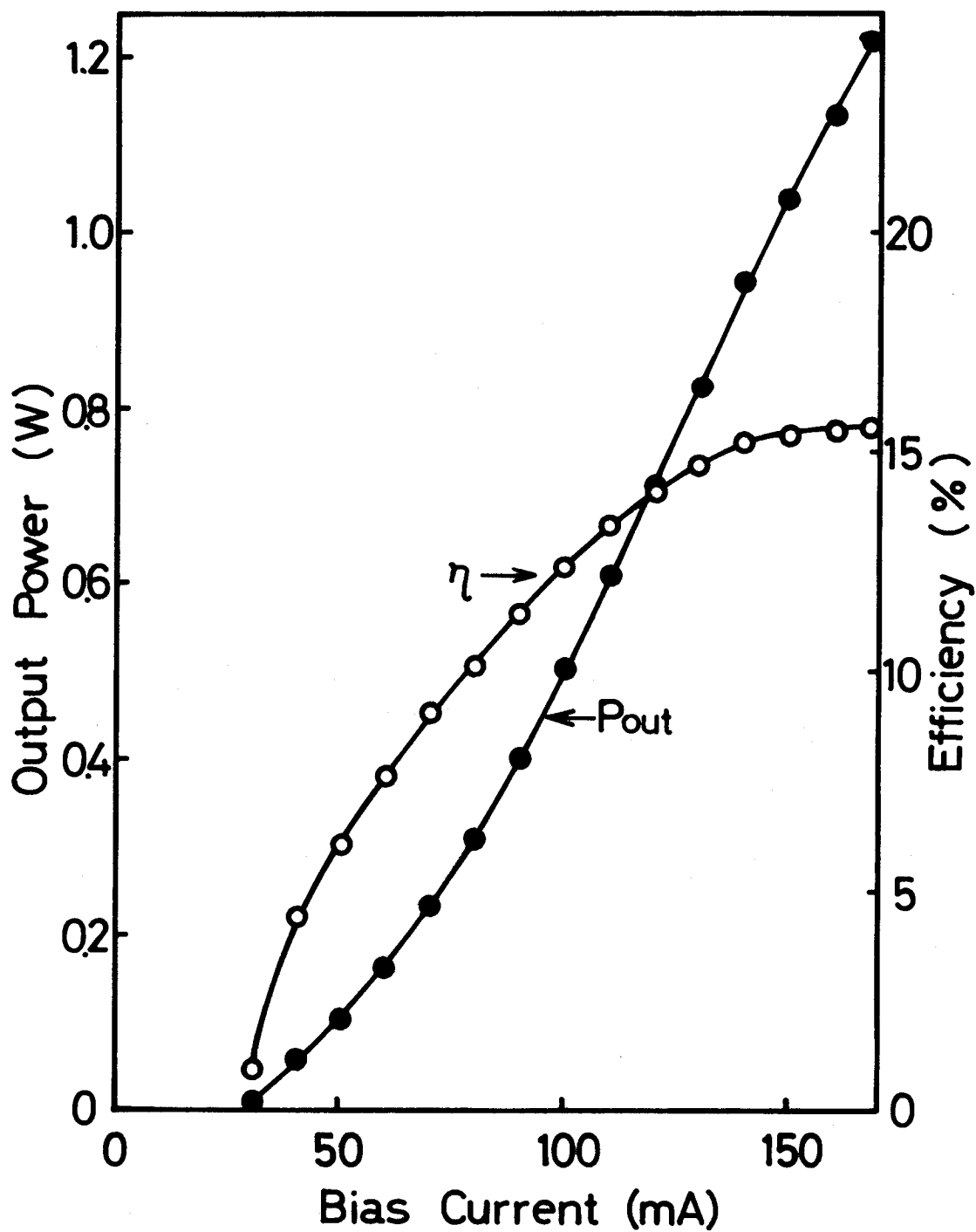
Fig. 31. High frequency characteristics of GaAs DDR IMPATT diode.
