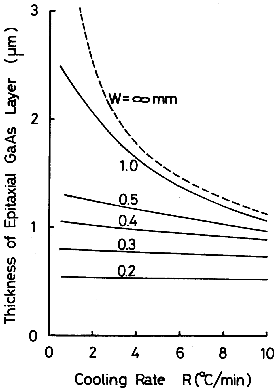
Fig. 5. Thickness of epitaxial GaAs layer versus cooling rate for various thickness W of Ga solution.
