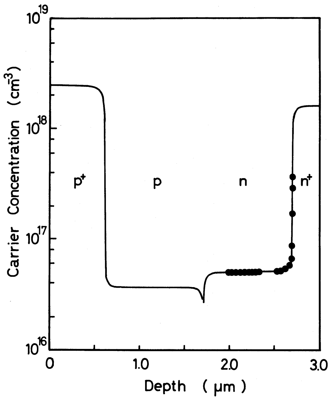
Fig. 30. Carrier concentration profile of the epitaxial layer.
