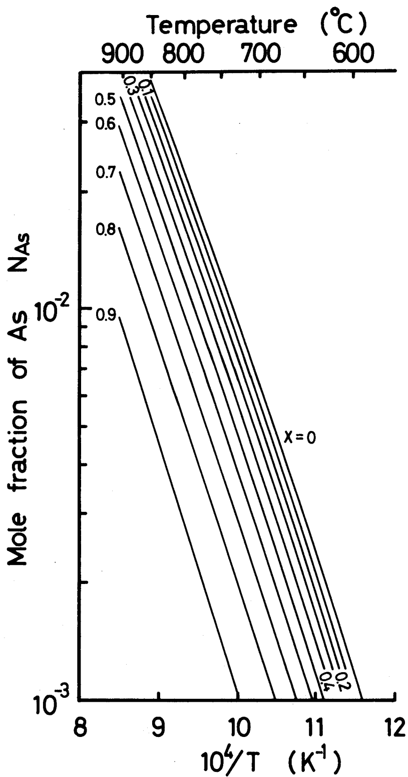
Fig. 18. Temperature dependence of As mole fraction in the saturated Ga solution.
