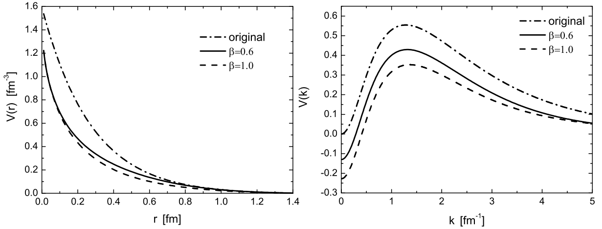
Figure C.4: The spin-spin central part of the pion exchange interaction with and without UCOM for the case \Lambda=700 MeV in coordinate space in the left panel and one in momentum space in the right panel. The dot-dashed curve corresponds to the interaction without UCOM, the solid curve corresponds to UCOM with \beta = 0.6 fm and the dashed curve with \beta = 1 fm.
