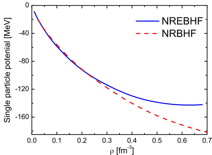
Figure 4.3: The depth U of the single particle potential for symmetric nuclear matter in the NREBHF theory with Bonn B potential. The solid curve represents the single particle potential of the NREBHF theory, while the dashed curve corresponds the results of the NRBHF theory.
