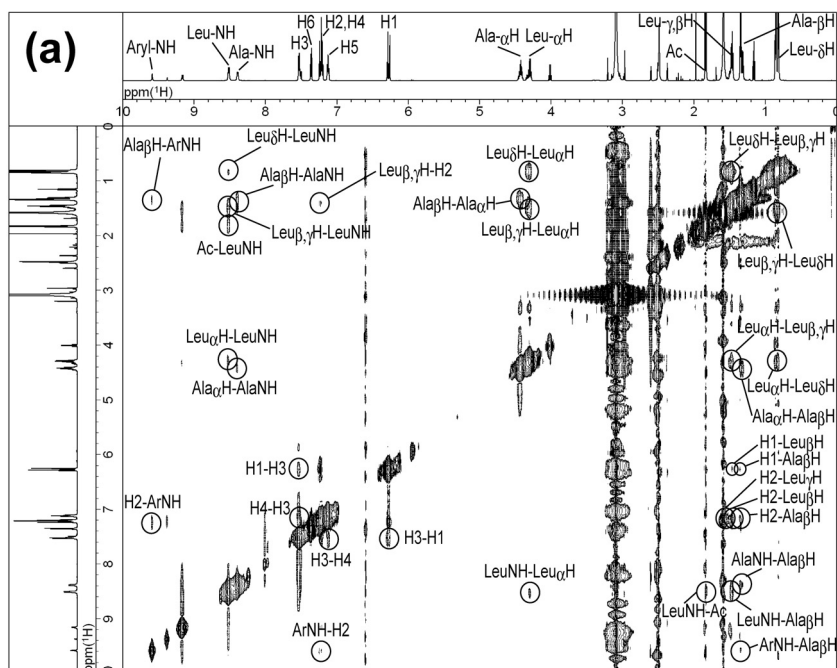
Figure 5a. NOESY spectra of E -6 in DMSO- d 6 solution at 303 K
