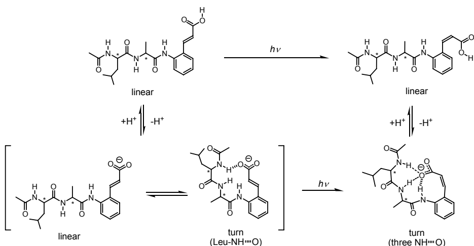
Scheme 4. Proposed conformation changes and photoswitching of intramolecular NH \cdots O hydrogen bond network of E -5/ Z -5 and E -6/ Z -6.
