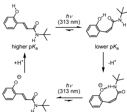
Figure 9. Artificial photocycle of ortho -coumaric acid derivative, which involves protonation and deprotonation process derived by pK_a change owing to photoswitching of an intramolecular NH...O hydrogen bond.
