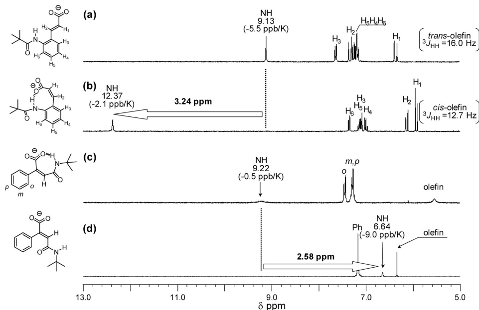
Figure 2. ^1\text{H} NMR spectra changes of isolated ON \rightarrow OFF type carboxylate derivatives c) E -4, d) Z -4, comparing with OFF \rightarrow ON type a) E -1, b) E -2, 5 mM in \text{DMSO}-d_6 at 303 K.
