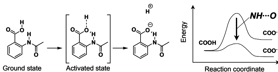
Figure 2. Deprotonation process of carboxylic acid derivative, whose carboxylate and transition state is stabilized by intramolecular \text{NH}\cdots\text{O} hydrogen bond toward carboxylic oxygen from proximate amide \text{NH} .
