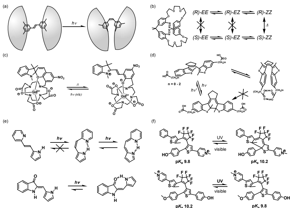
Figure 4. Photoswitching devices. a) stilbene dendrimer, b) chirality control by azobenzene, c) chaperone Gd ion by spiropyran, d) photoreactivity control by OH \cdots O hydrogen bond, e) photoreaction control by NH \cdots O and NH \cdots O hydrogen bond, f) acidity control by diarylethene.
