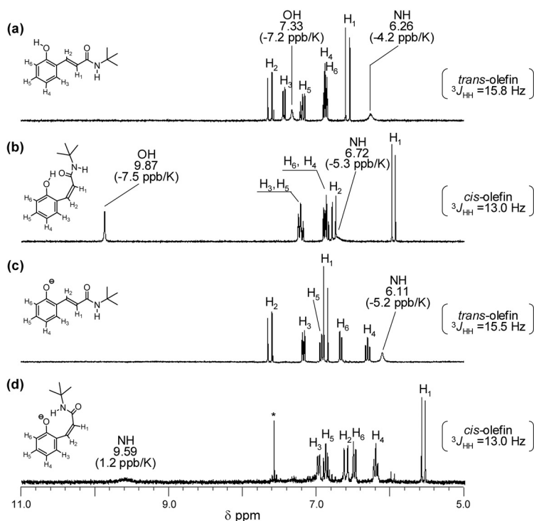
Figure 4. ^1\text{H} NMR spectra of a) E -1, b) Z -1, c) E -2 and d) Z -2, 5 mM in acetonitrile- d_3 at 303 K.
