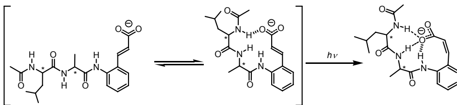
Scheme 3. Intramolecular hydrogen bond formation of E -6 and Z-6.
