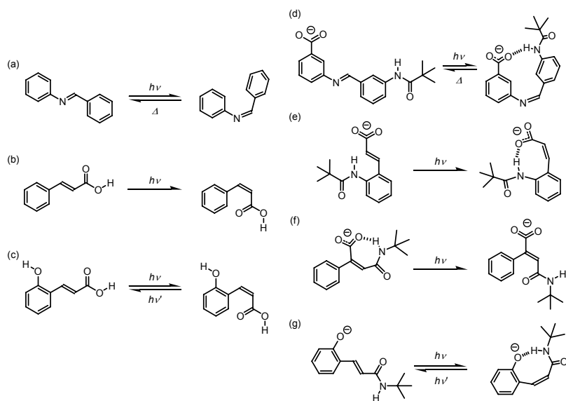
Figure 5. Photoswitching frameworks a) benzylidenedianiline, b) cinnamic acid, c) ortho -coumaric acid, and molecular design of the switching of intramolecular NH \cdots O hydrogen bond d) benzylidenedianiline derivative, e) OFF → ON type cinnamic acid derivative, f) ON → OFF type cinnamic acid derivative, and g) ortho -coumaric acid derivative.
