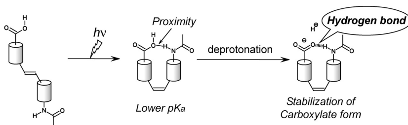
Figure 1. Switching of intramolecular NH\cdots O hydrogen bond by E/Z photoisomerization of olefin moiety.
