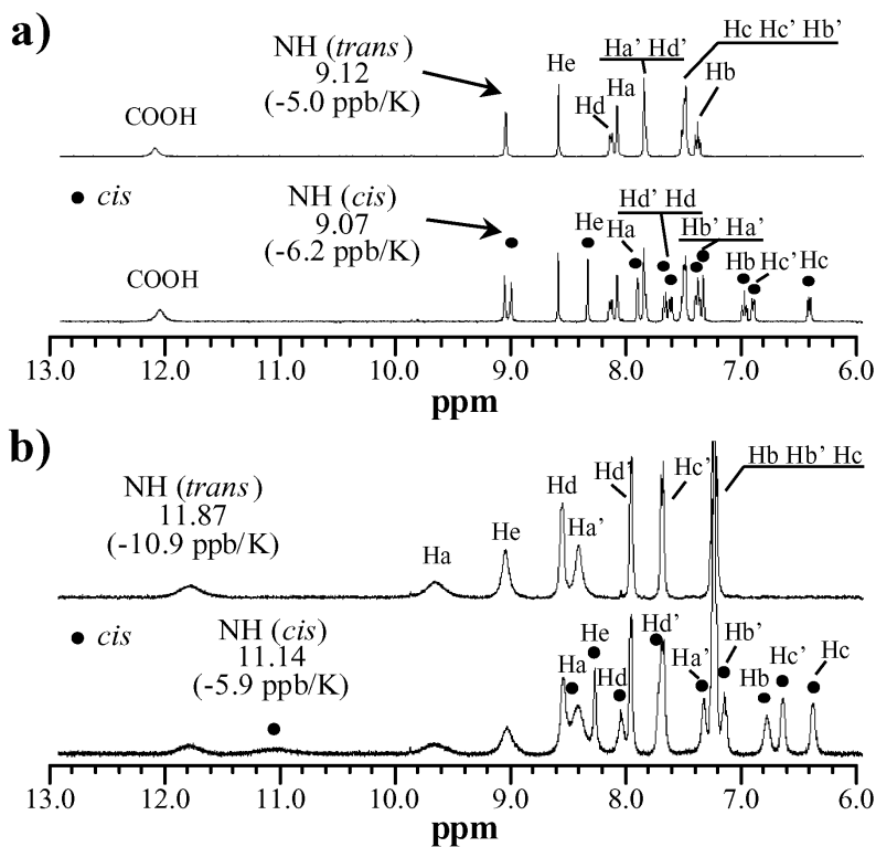
Figure 4. 1 H NMR spectrum change of a) E -1 and b) E -2', by UV irradiation of 313 nm and 365 nm 5 mM in THF- d 8 solution at 183 K. Before irradiation (upside) and after irradiation (downside).
