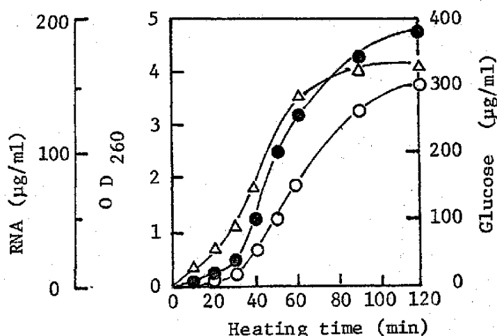
Fig. 1-3. Leakage of intracellular materials from C. utilis cells heated at 55°C in 0.1 M phosphate solution (pH 4.0). Symbols : ○, 260 nm-absorbing materials ; ●, orcinol-positive materials ; △, carbohydrates.
