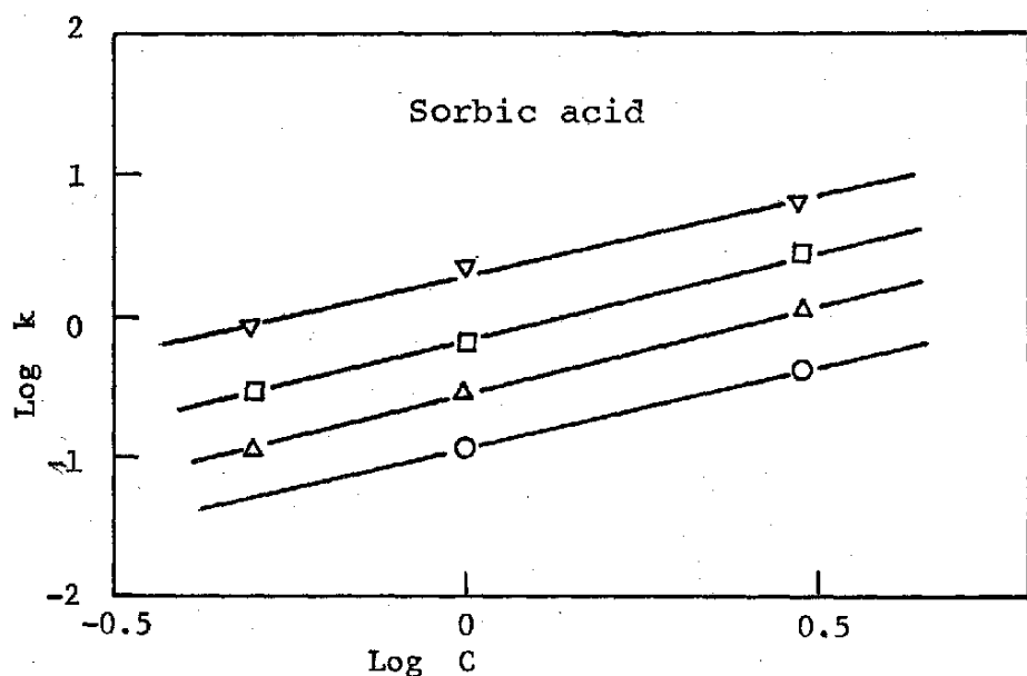
Fig. 6-6. Relationship between the thermal death rate constant and the concentration of sorbic acid. Cells were heated with sorbic acid in 0.05 M phosphate buffer (pH 7.0) at 48 (○), 50 (△), 52 (□) or 54 (▽) °C. Dilution coefficients at above temperatures were 1.15, 1.22, 1.20 and 1.10, respectively.
