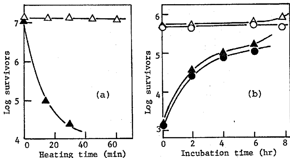
Fig. 1-5. Loss and its recovery of NaCl tolerance of C. utilis cells heated at 45°C in 0.1 M phosphate solution (pH 4.0). (a) Loss of NaCl tolerance. Cells were heated and plated on CPYA ( \Delta ) and CPYA containing 7% NaCl ( \blacktriangle ). (b) Recovery of NaCl tolerance. Cells were heated at 45°C for 15 min, incubated at 30°C in 0.1 M phosphate buffer (pH 5.5) ( \circ , \bullet ) or CPY broth ( \Delta , \blacktriangle ) and then plated on CPYA ( \circ , \Delta ) and CPYA containing 7% NaCl ( \bullet , \blacktriangle ).
