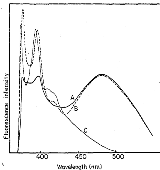
Fig. 1-6. Emission spectra of VPy-MAh alternating copolymer 1 \times 10^{-3} mol/l 2MTHF-THF solution. (A): 300°K, (B): 213°K, (C): 77°K.
