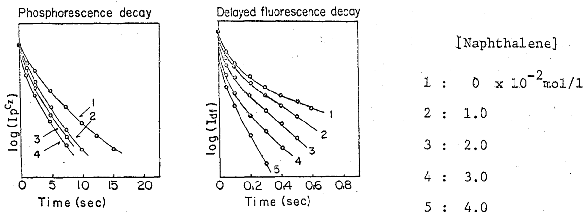
Fig. 2-7. The dependence of delayed emission decays of PVCz/FN on the concentration of naphthalene. [\text{PVCz/FN}] = 1 \times 10^{-3} \text{ mol/l} .
