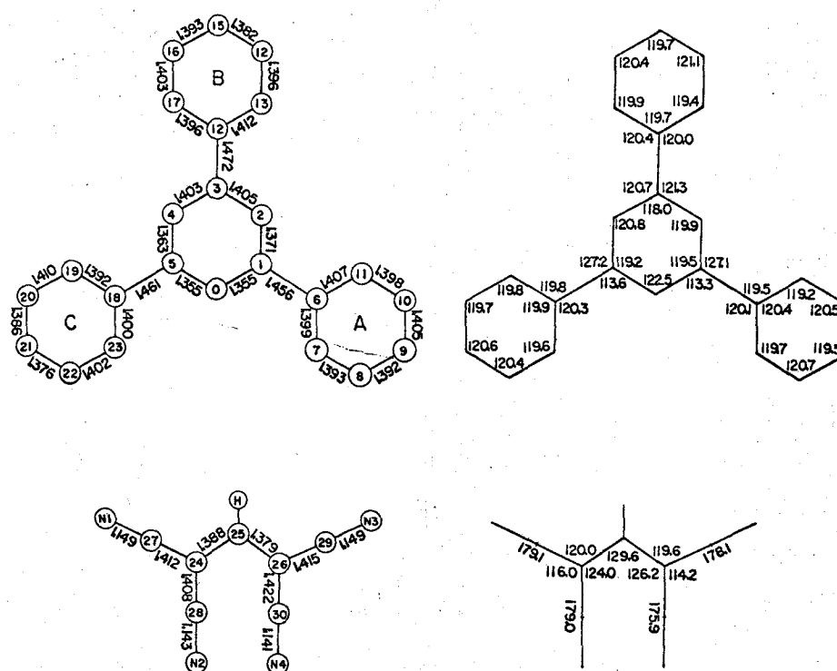
Fig. 4-2. Bond lengths (Å) and bond angles (°) in TPP-TCP salt.
