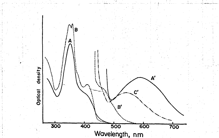
Fig. 1-4. Absorption spectra of TPT-TCP in 2MTHF-toluene (9:1) solution at various temperature.
