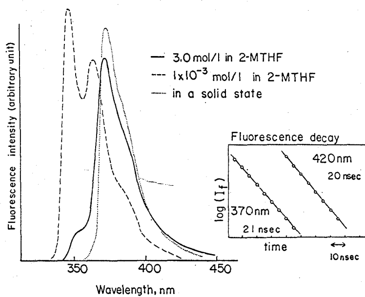
Fig. 1-3. Fluorescence spectra and fluorescence decays of N-ethylcarbazole.
