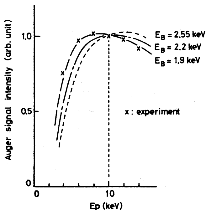
Fig. 4-4 The variation of Auger signal intensity as a function of primary energy for different binding energies of E_B = 2.55 keV (-----), E_B = 2.2 keV (-·-·-·-), and E_B = 1.9 keV(———). All the results (including experimental ones) are normalized at 10 keV.
