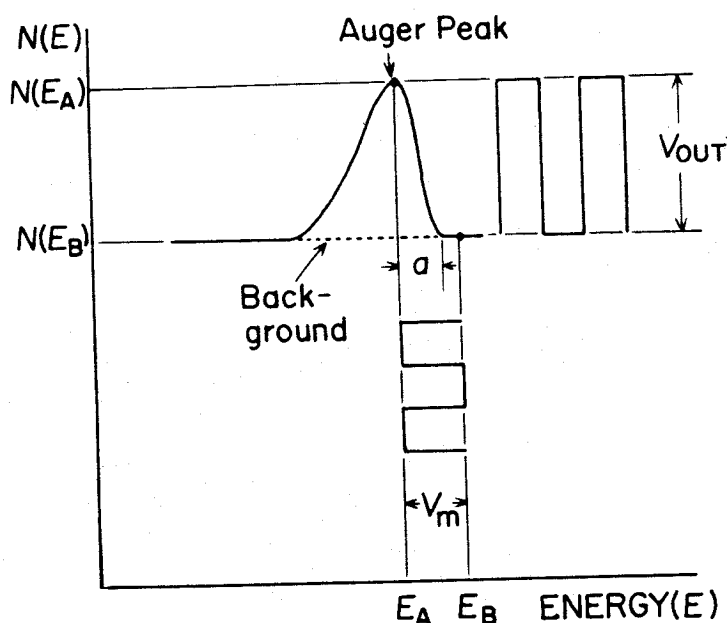
Fig. 2-2 Schematic illustration of square wave modulation. V_m ; amplitude of modulation, E_A ; maximum Auger peak energy, Q ; energy width between the maximum Auger peak and higher energy side of the Auger peak.
