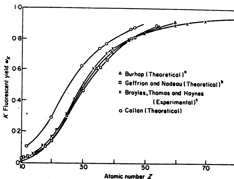
Fig. 1-4 K-shell fluorescence yield as a function of atomic number (Callan 1961)
