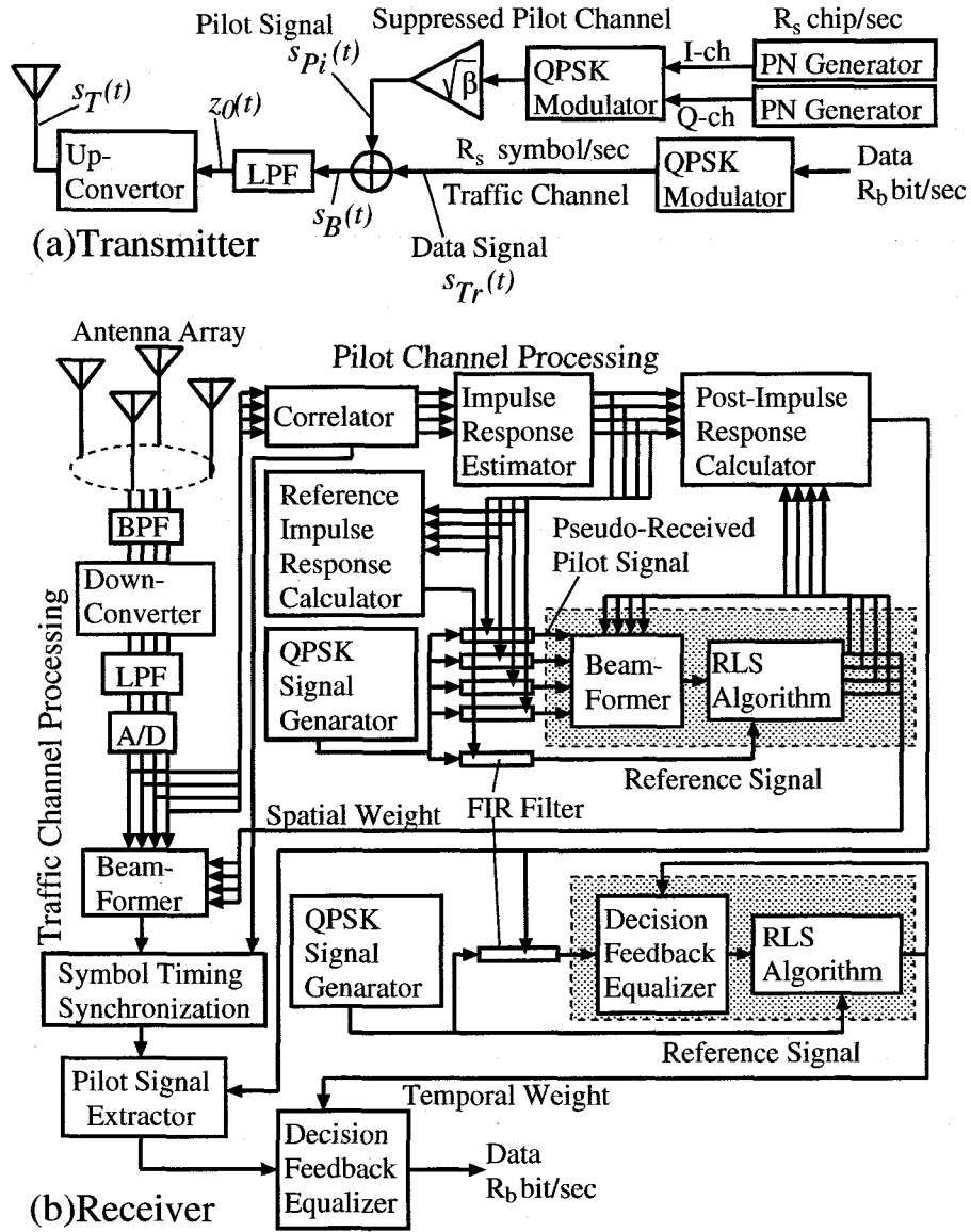
Figure 4.1: Transmitter/Receiver Structure.
