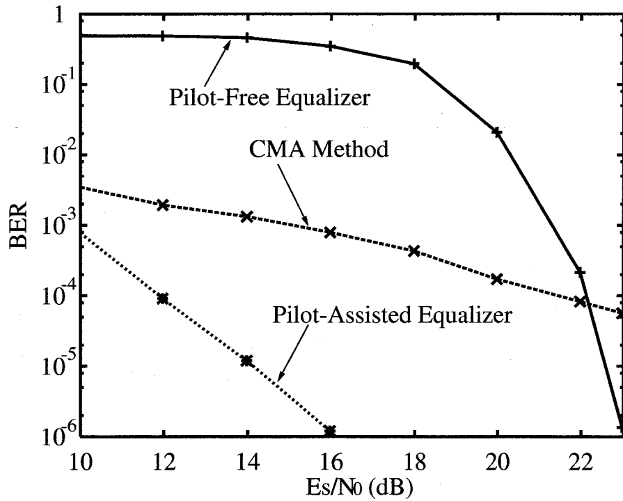
Figure 3.19: BER Performance.
