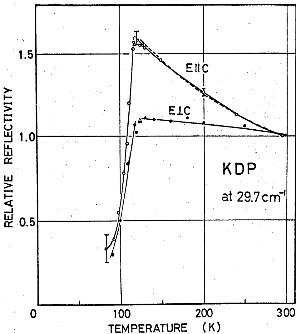
Fig. 4-2 Temperature dependence of polarized reflectivity for KDP at 29.7 cm -1 . The reflectivity is normalized at room temperature. The dashed curve shows the calculated reflectivity by single oscillator model.
