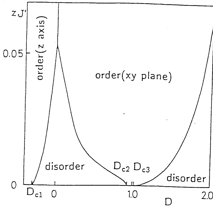
Figure 3.6: Phase diagram obtained with the Hamiltonian; \mathcal{H} = \sum S_i S_{i+1} + D \sum S_i^z{}^2 + J' \sum S_i S_j , where D is the single ion anisotropy and J' is the interchain exchange coupling constant.
