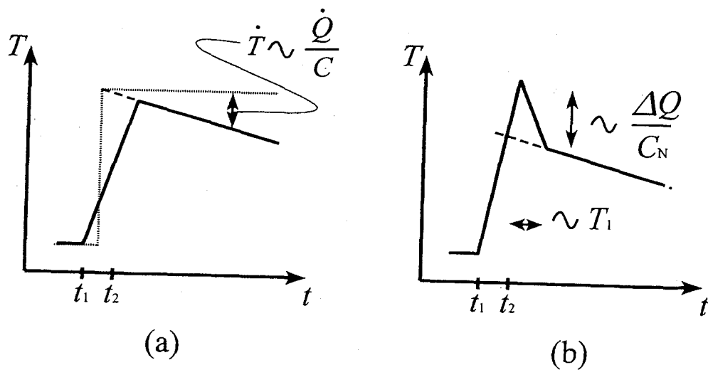
Figure 2.3: Examples of the temperature profile in various configurations. The heat pulse is supplied between t_1 and t_2 . (a) The broken line is the ideal case. In the real system, the heat leak to the thermal bath exists and the temperature profile shows a declination as \dot{T} \sim \dot{Q}/C . (b) In case the nuclear magnetic heat capacity C_N is present, the temperature profile shows an overshoot and, after the duration of the nuclear spin lattice relaxation time T_1 , the system settles down to the thermal equilibrium.
