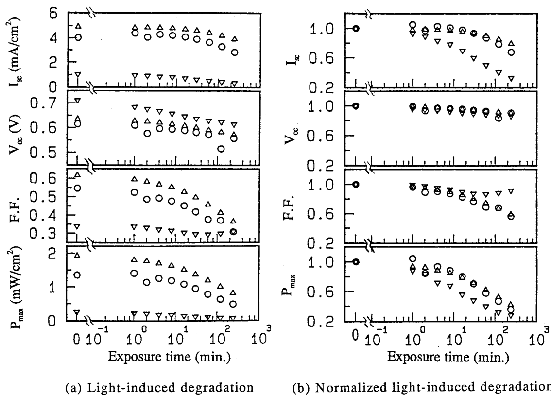
Fig. 5-4-4. Light-induced degradation characteristics under red light of a-SiGe Type P (Δ), Type N (▽) and 1.52 eV constant bandgap cell (○) which is exposed to AM 1.5, 10 suns light [ Original (a) and normalized (b) data] .
