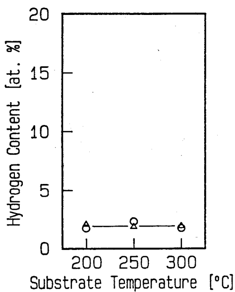
(c) Ge-H bond
