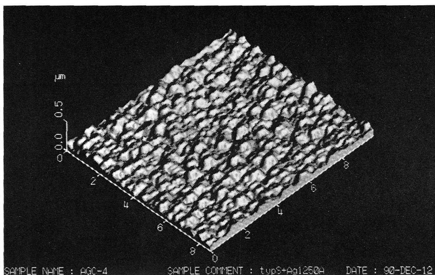
(b) Glass / textured \text{SnO}_2 / Ag (125 nm)
