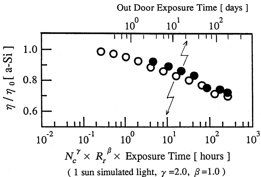
Fig. 4-5-2. Comparison of light-induced degradation characteristics of normalized conversion efficiency ( \eta / \eta_0 ) in a-Si solar cells under 1 sun simulated light ( \bigcirc ) and under outdoor exposure ( \bullet ). Bias voltage is maximum output voltages in both cases.
