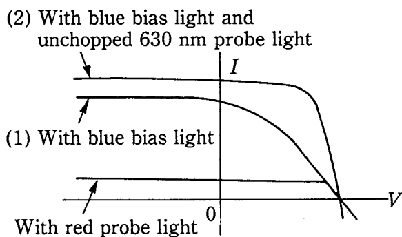
(b) I - V characteristics
