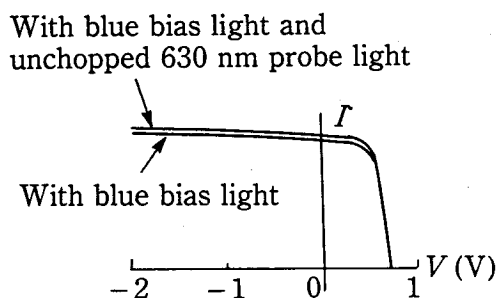
(b) I - V characteristics
