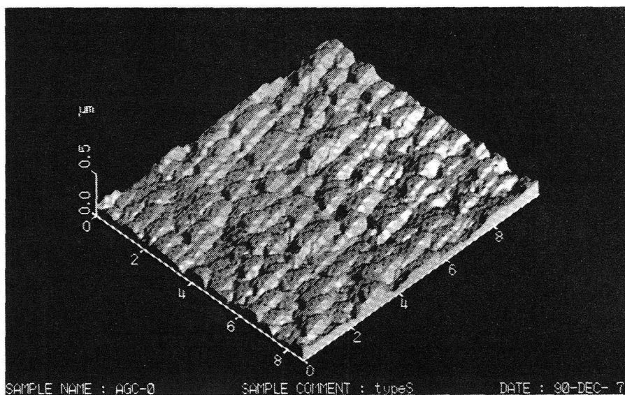
(a) Glass / textured \text{SnO}_2
