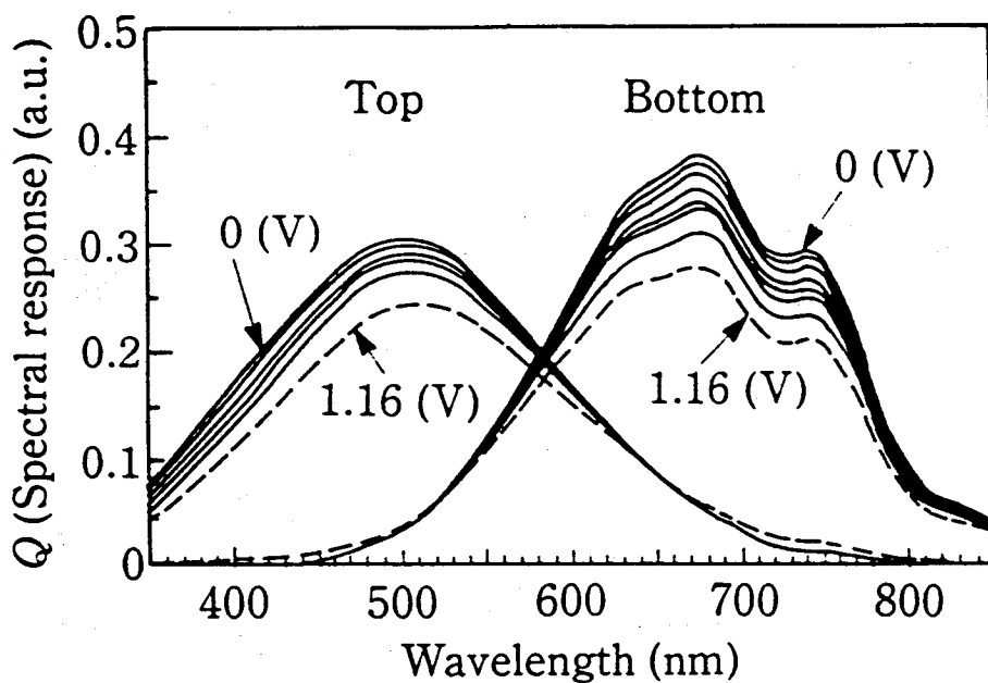
Fig. 3-3-5. Spectral response dependence for each component cell in a stacked cell on external bias voltage.
