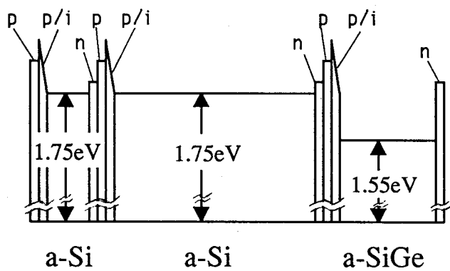
(b) Bandgap profile
