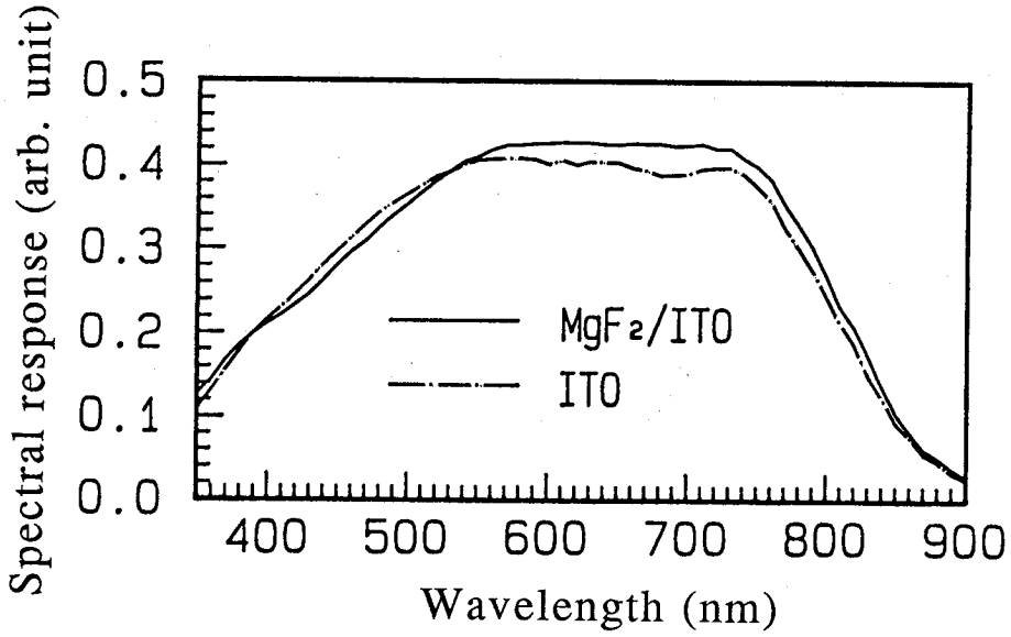
(b) Spectral response
