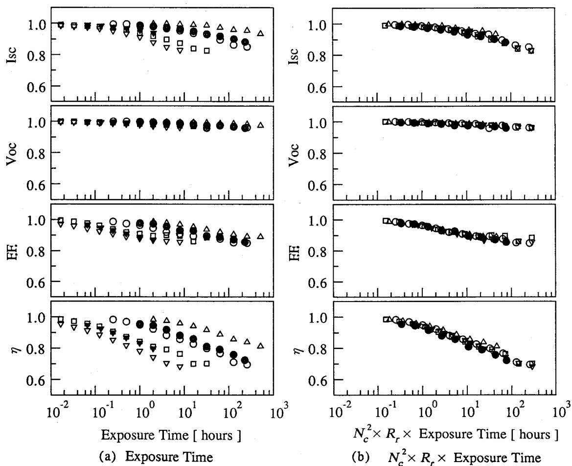
Fig. 4-3-4 Light-induced degradation characteristics of normalized I_{sc} , V_{oc} , FF, and \eta for a-Si solar cell as a function of exposure time t (a), and N_c^2 R_f t (b) for various light intensities and bias voltages. Symbols are the same as those in Figs. 4-3-1 and 4-3-2.
