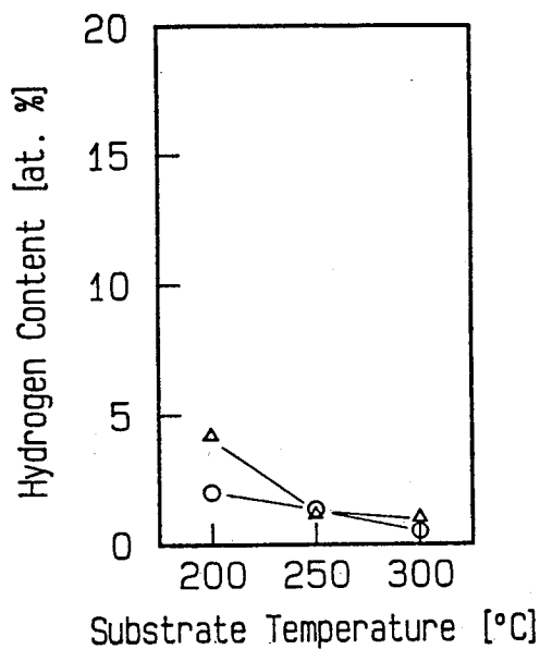
(b) Si-H 2 bond
