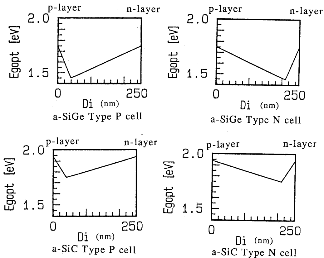
Fig. 5-5-2. Bandgap profiles of a-SiGe cells (Type P, N) and a-SiC cells (Type P, N). ( E_{\text{gopt}} : Optical bandgap )
