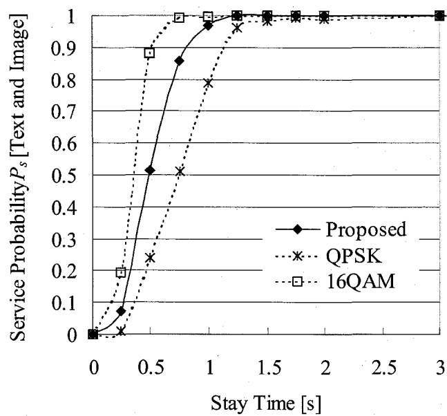
(a) Channel CNR=35[dB]
