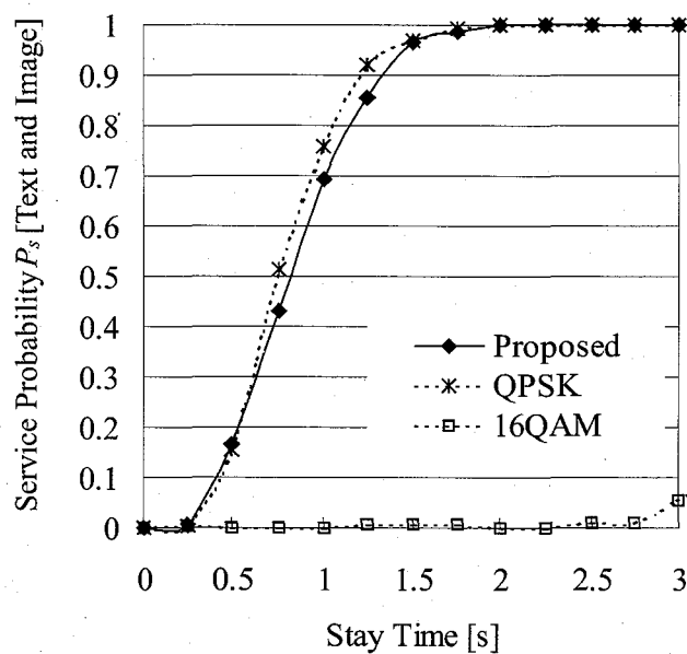
(b) Channel CNR=20[dB]
