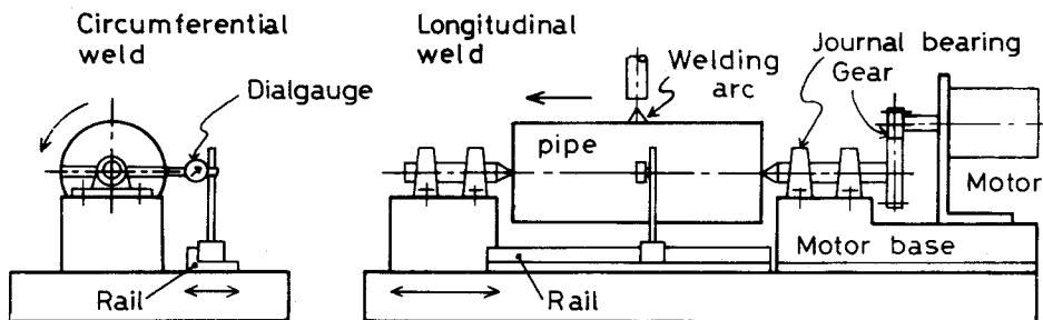
Experimental apparatus
