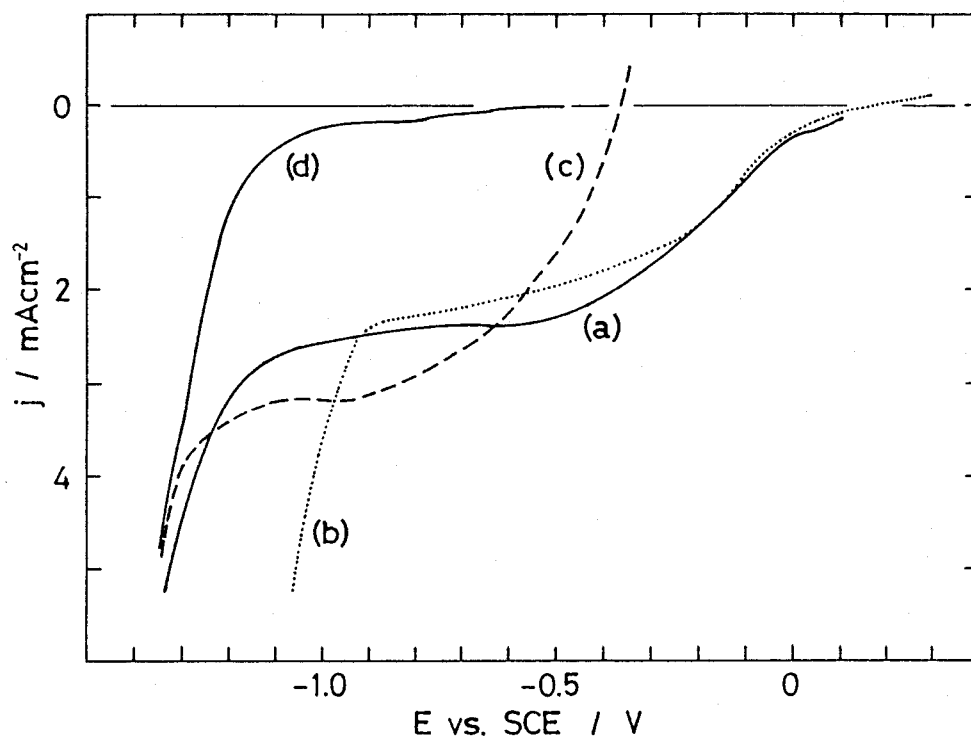
Fig. 4 Current density( j )-potential( E ) curves for \text{Co}_x\text{N} (a), Pt (b) and Co (c) electrodes in \text{O}_2 -saturated 0.5 \text{ M Na}_2\text{SO}_4 (pH 6.0) and that for \text{Co}_x\text{N} (d) in deoxygenated 0.5 \text{ M Na}_2\text{SO}_4 . The scan rate was 20 \text{ mV/s} .
