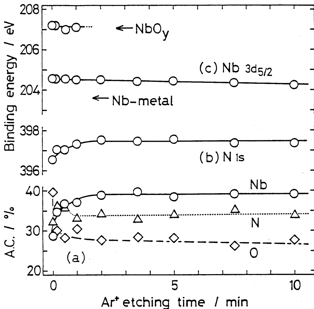
Fig. 4 Relative atomic concentrations (A.C.) for an \text{NbN}_x film the same as shown in Fig. 3 (a) and (b) as a function of the \text{Ar}^+ -ion etching time, together with the binding energies for the \text{N } 1s and the \text{Nb } 3d_{5/2} peaks with the \text{C } 1s peak taken as the energy standard.
