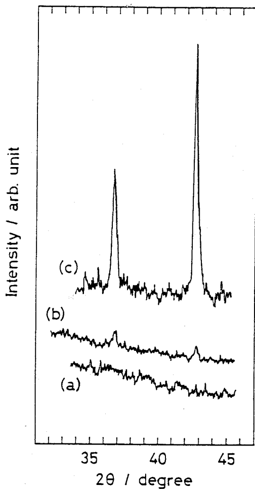
Fig. 1 X-ray diffraction (XRD) patterns; (a) for a \text{TiN}_x film ( 0.70\text{ }\mu\text{m} thick) sputter-deposited on a quartz plate, (b) after thermal treatment at 1000^\circ\text{C} for 20 min under a nitrogen atmosphere, and (c) for crystalline TiN (cubic) powder.
