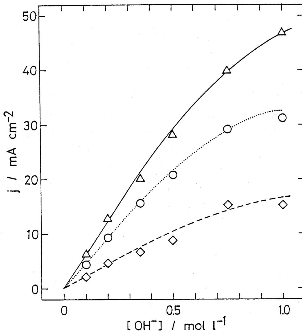
Fig. 10 Dependence of oxygen evolution current densities in the \text{ZrN}_x electrode on the \text{OH}^- concentrations at fixed overpotentials, \eta = 0.8 V (solid line), 0.7 V (dotted line) and 0.6 V (broken line). The solutions are prepared by mixing 1.0 M NaOH and 0.5 M \text{Na}_2\text{SO}_4 solutions.
