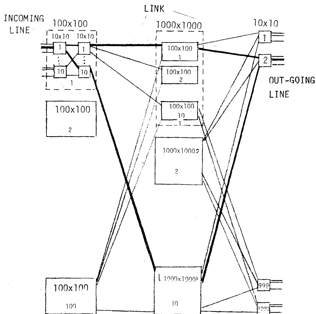
(a) SPACE DIVISION SWITCH NETWORK
