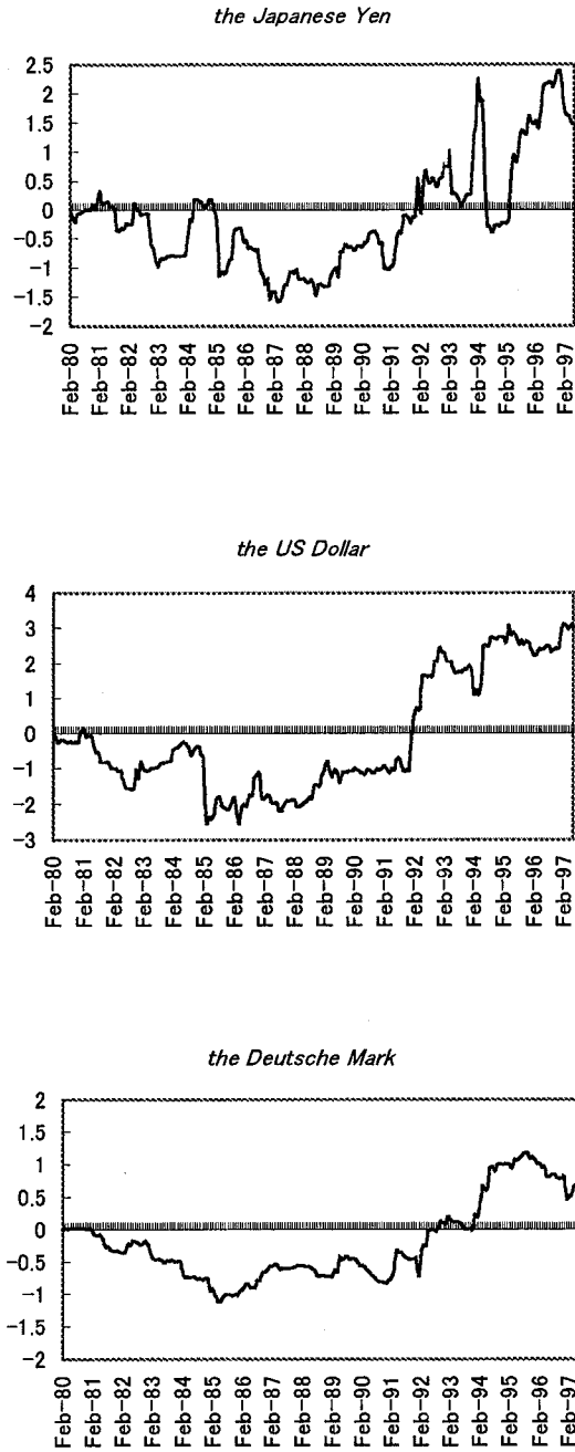
Figure A3.4. The Malaysian Ringgit: Test Statistics for the Variation of the Estimated Weights of Major Currencies
