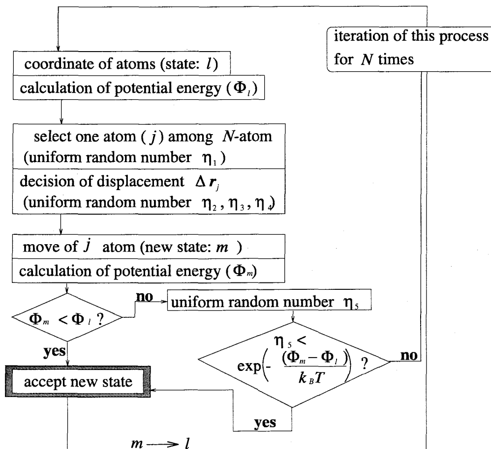
Fig. 2.4 Flow-chart of Metropolis method
