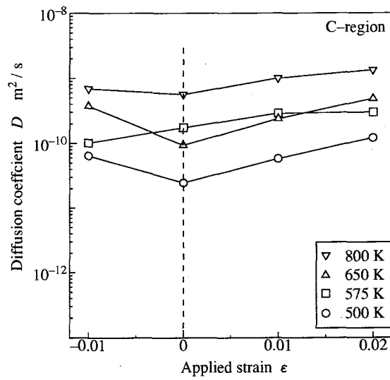
(a) C-region
