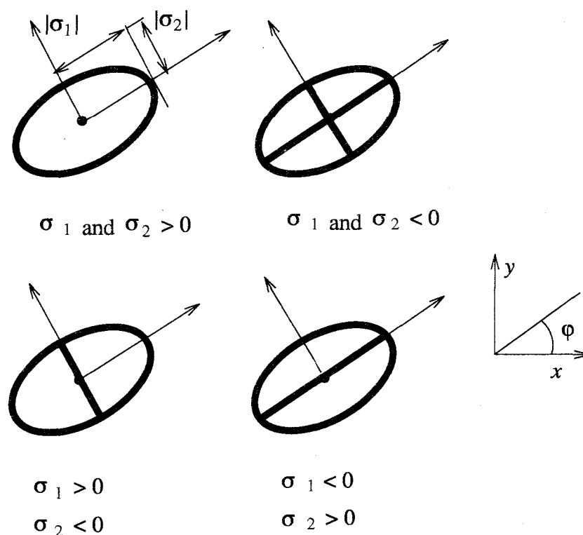
Fig. 6.4 Elliptic circle for visualization of principal stress of atom
