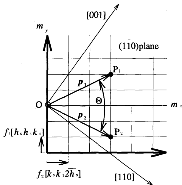
Fig. 2.26 Geometrical relation between crystallographic planes meeting at the grain boundary in [1\bar{1}0] A.T.G.B.
