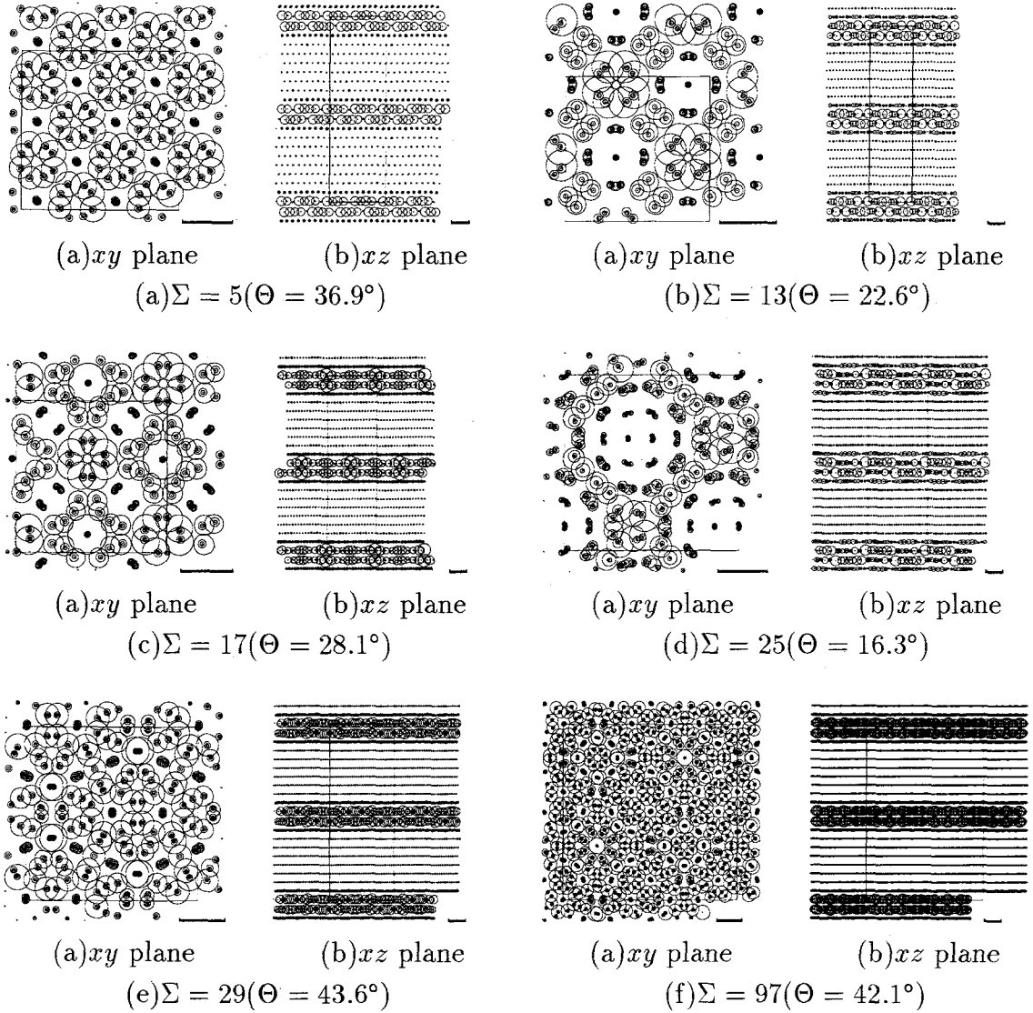
Fig. 2.20 Atomic configuration and energy distribution of [100] twist grain boundaries (Energy level of each atom is shown by circle centered at its position. Radius of the circle corresponds to the energy level. For each grain boundary, projections on (a) xy plane and (b) xz plane are shown. Length of line segment at the lower right of each figure corresponds to -4.3 \times 10^{-19} \text{J} . See Fig.2.15.)
