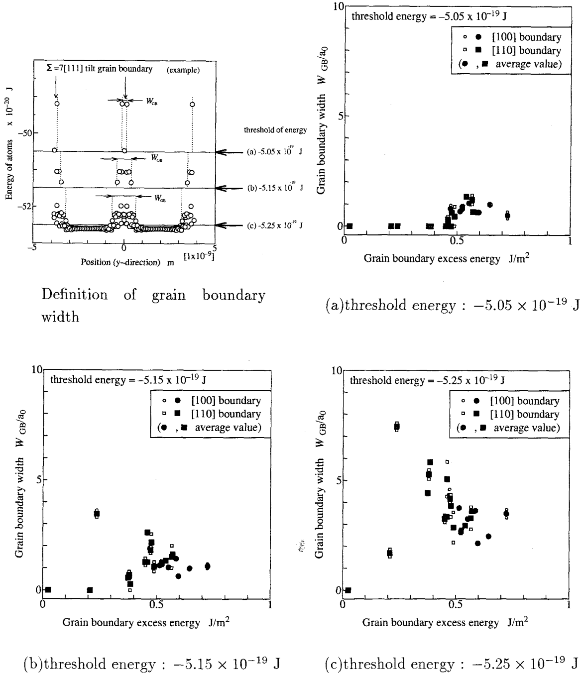
Fig. 2.24 Relation between grain boundary energy and thickness of grain boundaries ( W_{GB} ) (for three threshold energies)
