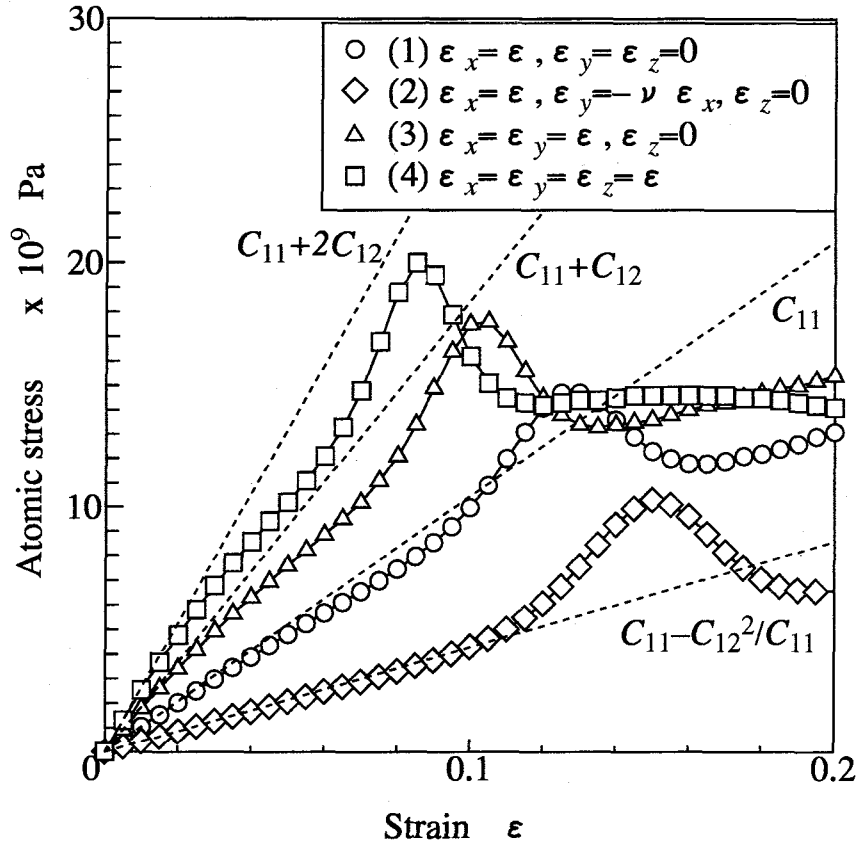
Fig. 3.6 Stress-strain curves for various constrained conditions
