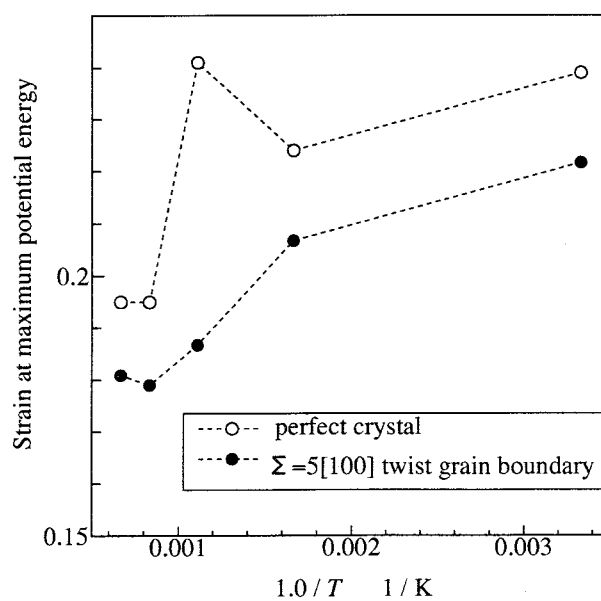
Fig. 4.10 Temperature dependence of total strain at maximum potential energy
