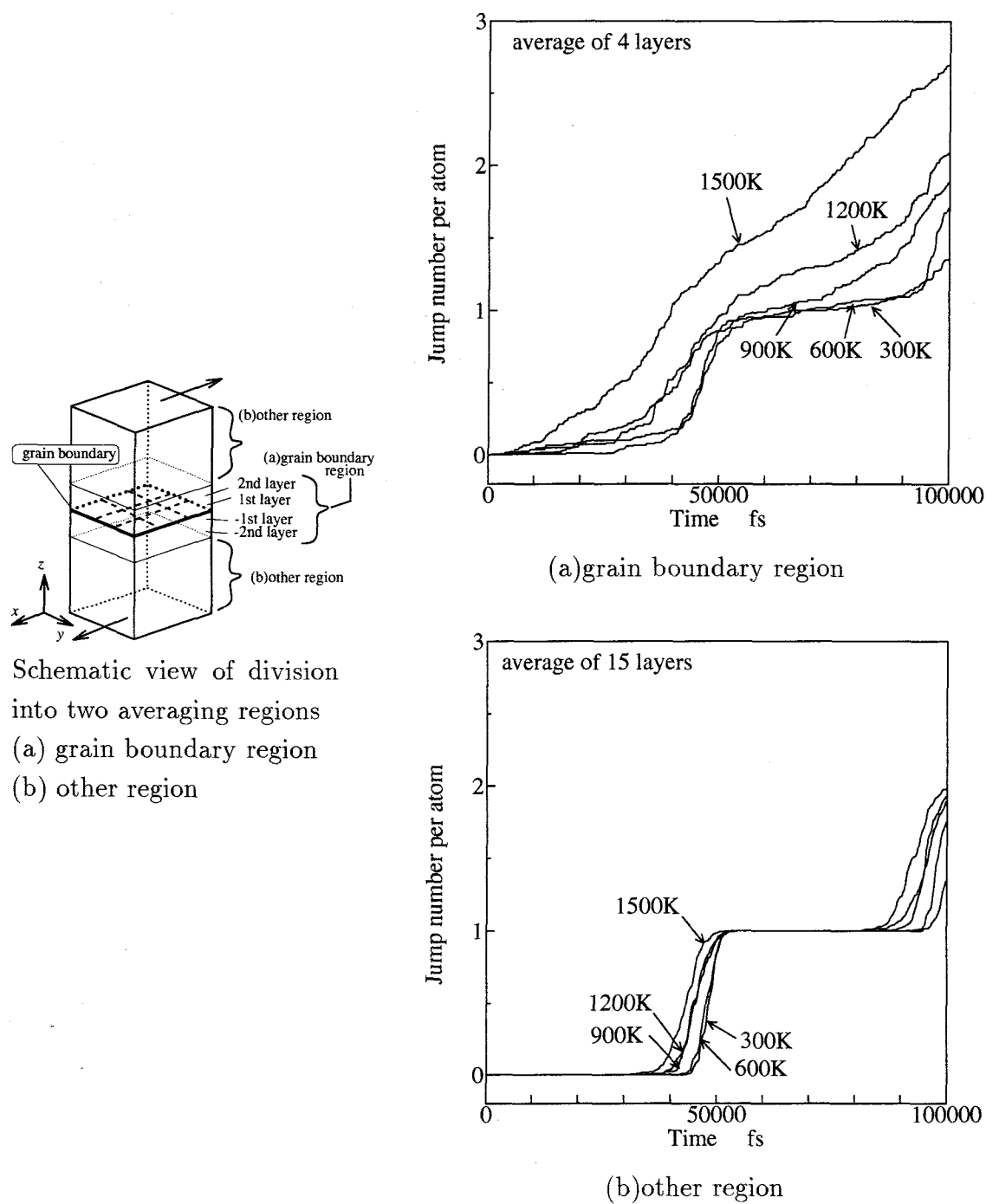
Fig. 4.16 Transition of cumulative jump number during shear loading
