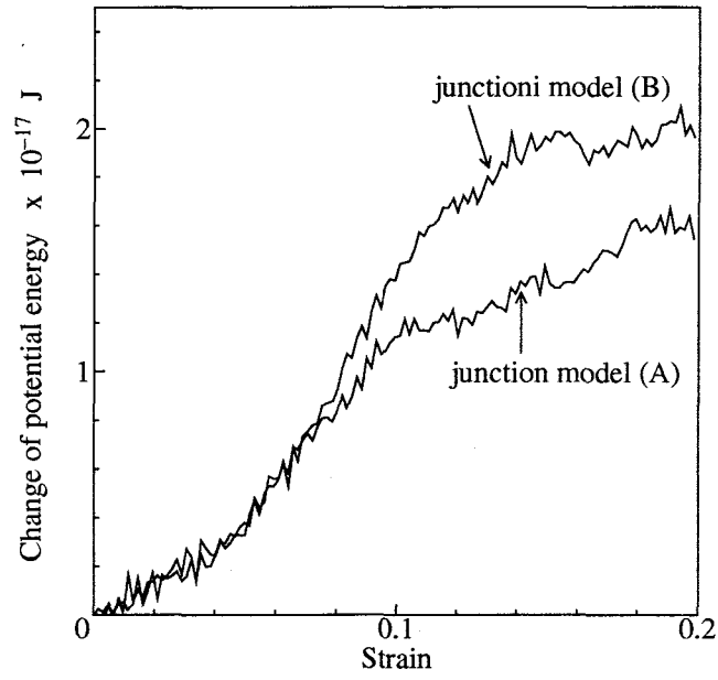
Fig. 6.32 Transition of total potential energy of two junction models
