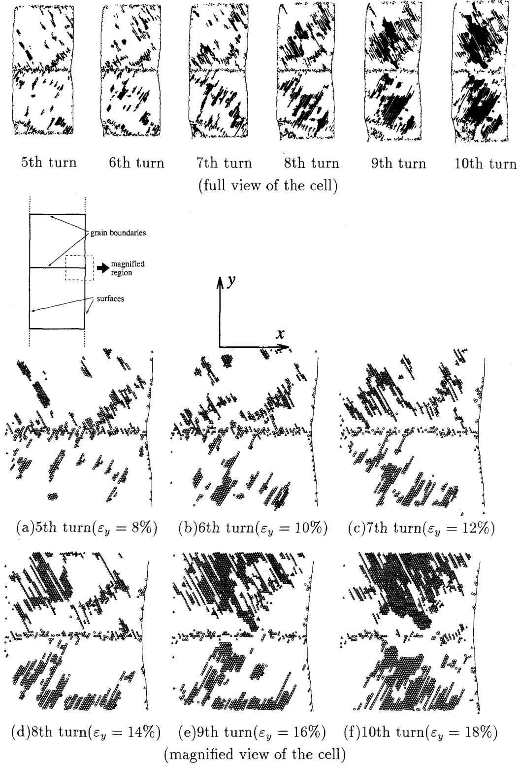
Fig. 6.19 Distribution of atomic shear stress \tau_i^{xy} being larger than a specific value in case (II) (Only atoms with \tau_i^{xy} > 1\text{GPa} ( \bigcirc ) or with \tau_i^{xy} < -1\text{GPa} ( \triangle ) are displayed.)
