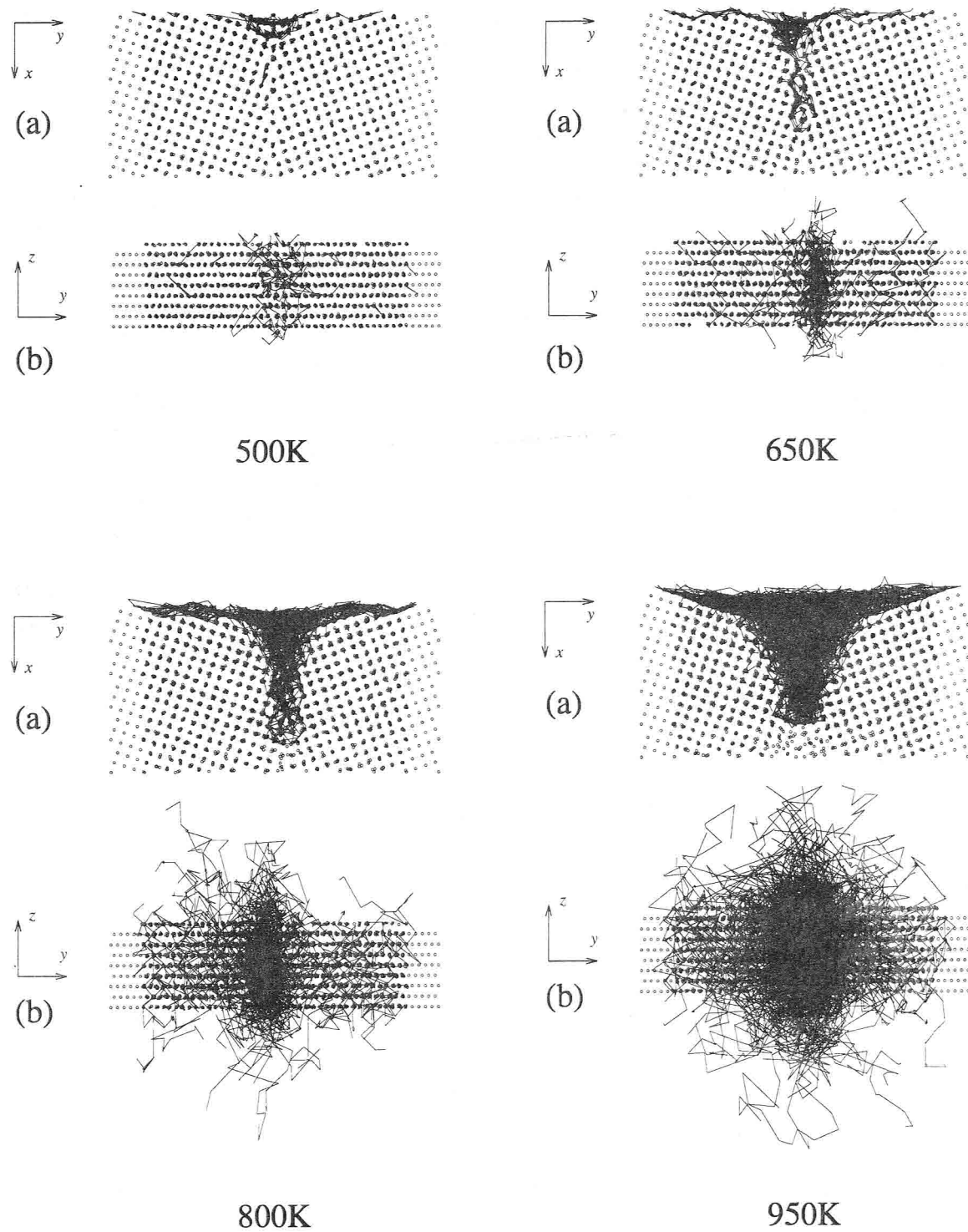
Fig. 5.4 Trajectory of atoms(projection on (a) xy plane and (b) yz plane)
