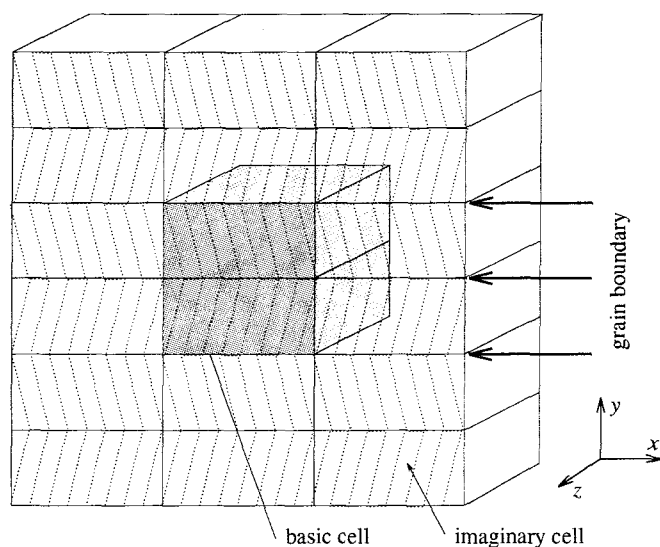
Fig. 2.3 Super-cell method for grain boundary simulation
