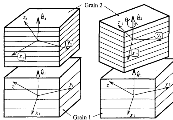
Fig. 2.11 General grain boundary
