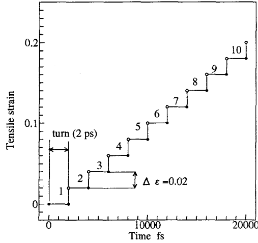
Fig. 6.6 Diagram of stepwise strain loading and definition of turn
