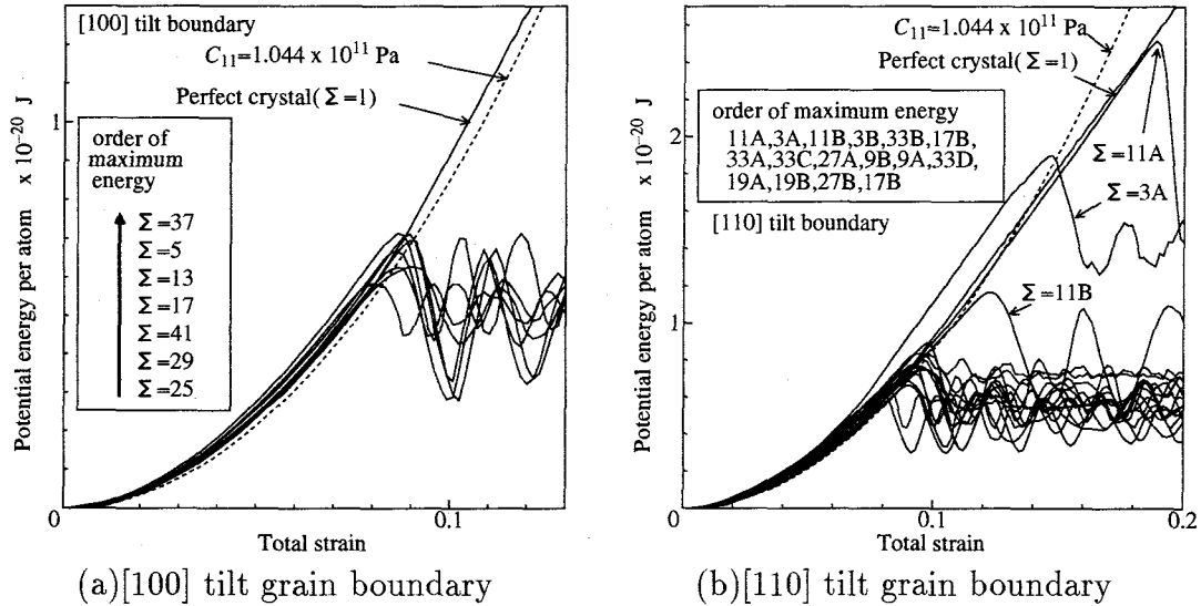
Fig. 3.11 Transition of potential energy per atom (range of horizontal axis and vertical axis is different in each figure)
