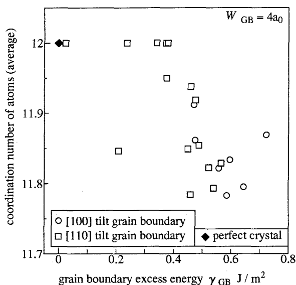
Fig. 2.25 Grain boundary energy vs. coordination number averaged over atoms in grain boundary region
