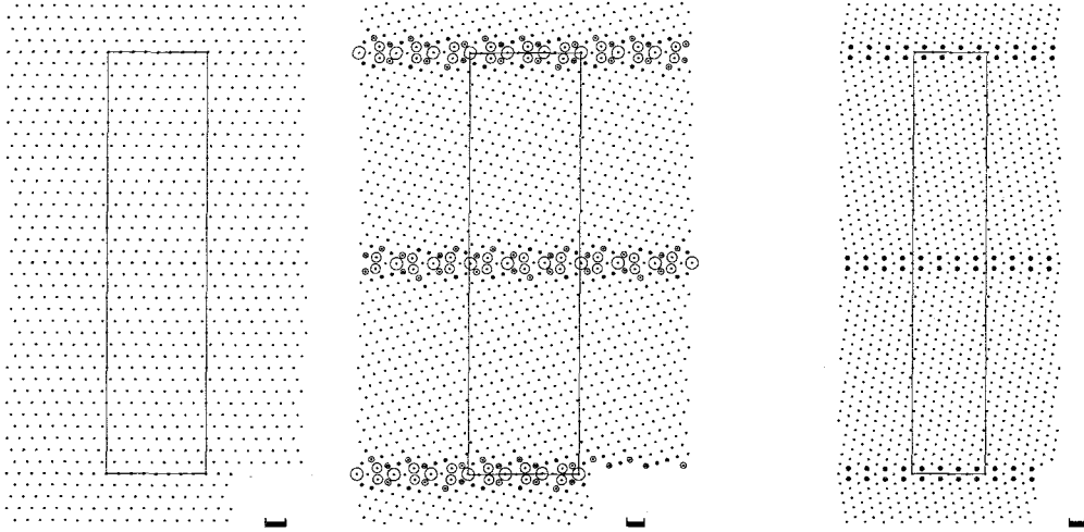
(a) \Sigma = 3[110](A)(109.5^\circ) (b) \Sigma = 9[110](A)(141.5^\circ) (c) \Sigma = 11[110](A)(50.5^\circ)
