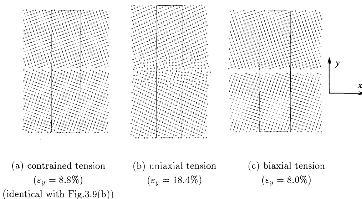
Fig. 3.20 Atomic configurations after fracture in three different tensile conditions (Projections on xy plane are shown. Small circles indicate atoms and a rectangle shows basic calculation cell.)
