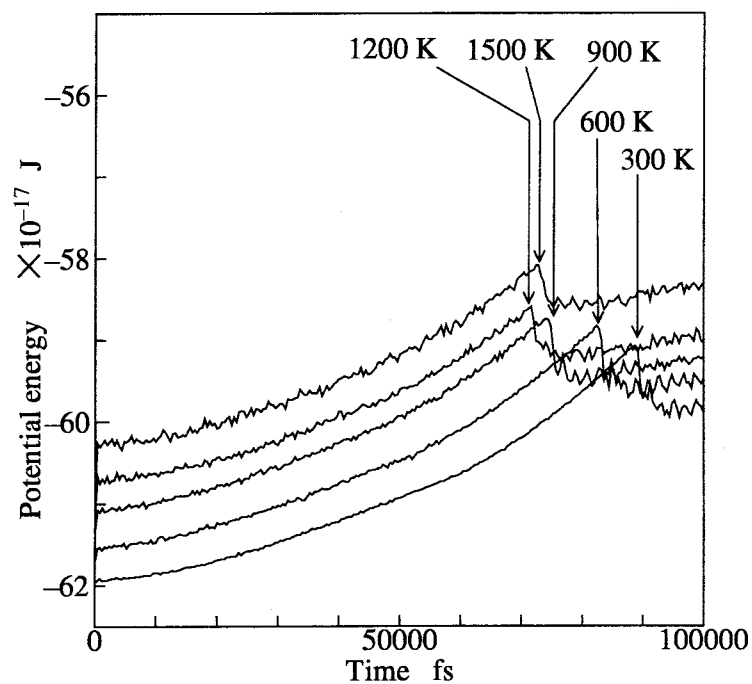
Fig. 4.9 Transition of total potential energy during tensile loading
