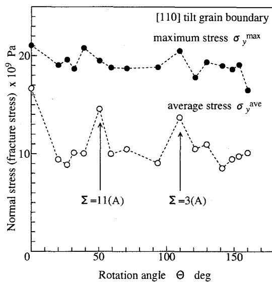
(b) [110] tilt grain boundary
