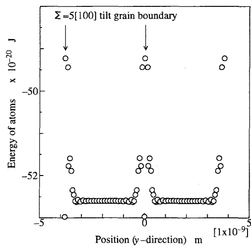
(b) \Sigma = 5[100] tilt grain boundary
