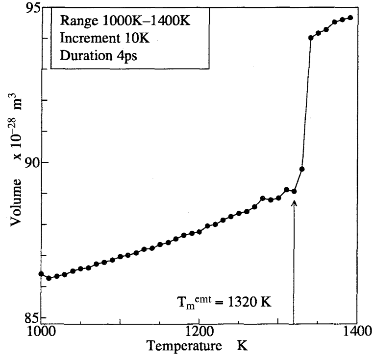
Fig. 2.9 Temperature vs. volume relation obtained by Parrinello-Rahman method under temperature control
