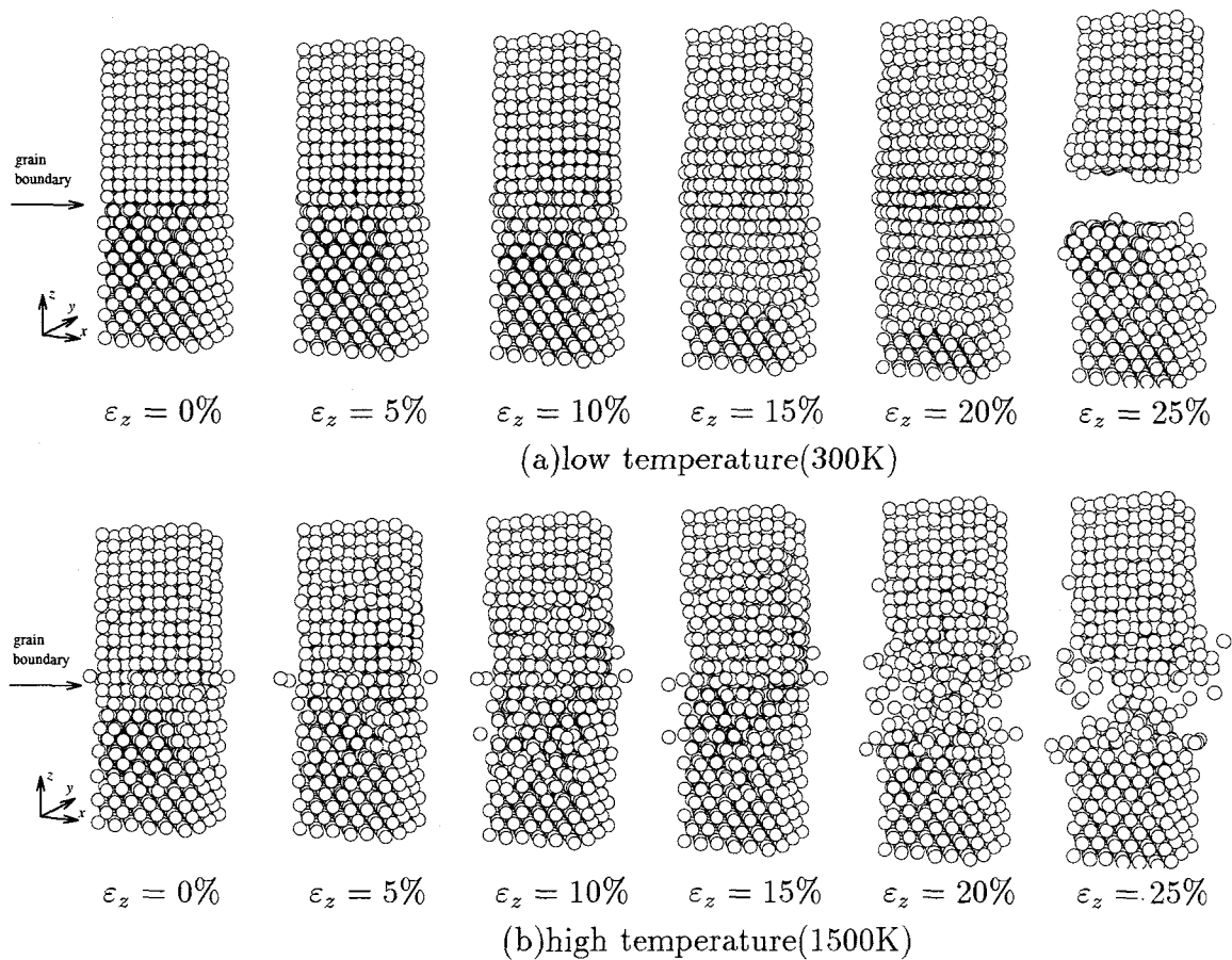
Fig. 4.11 Atomic configuration during tensile loading
