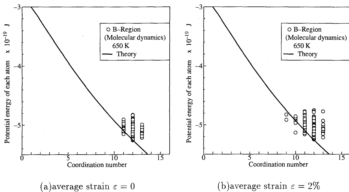
Fig. 5.21 Coordination number vs. potential energy of individual atoms in B-region
