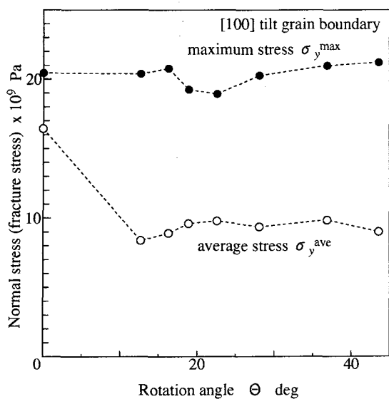
(a) [100] tilt grain boundary
