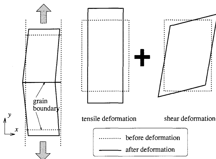
Fig. 6.10 Schematic view of deformation mode of free surface model
