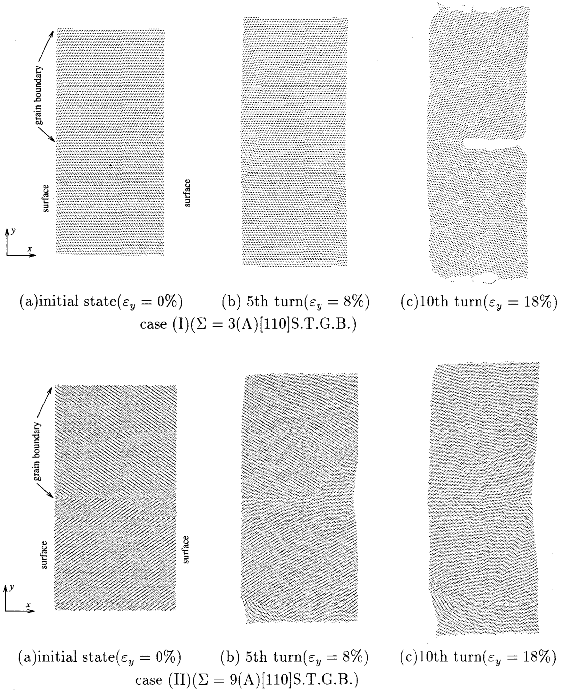
Fig. 6.11 Atomic configuration during loading(case (I),(II); projection on xy plane)
