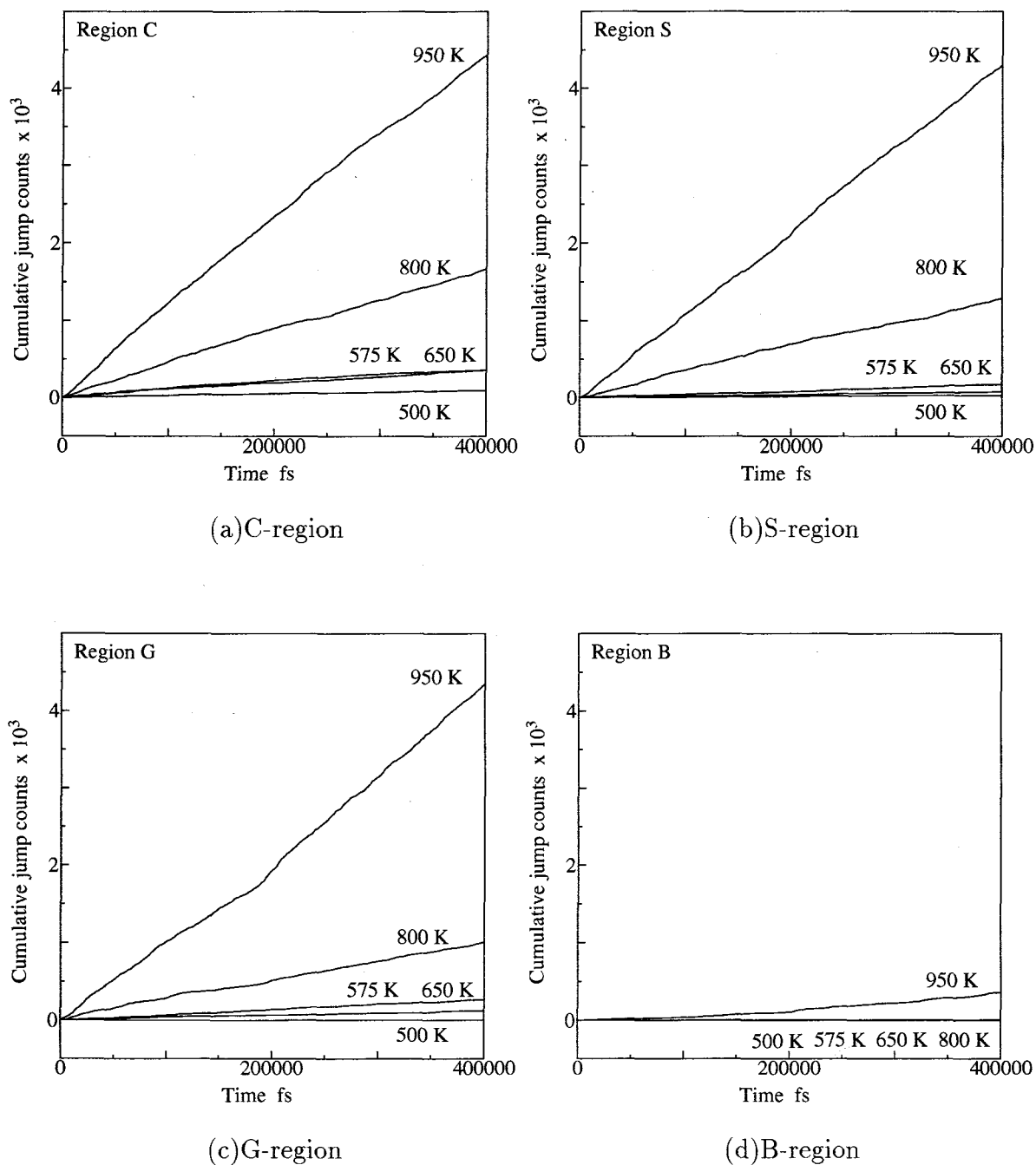
Fig. 5.8 Regional dependence of cumulative counts of jump
