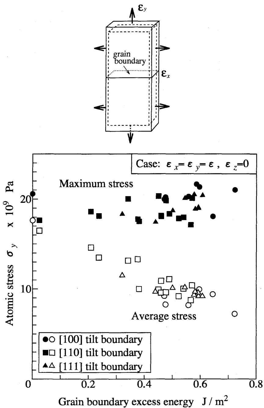
Fig. 3.22 Relation between grain boundary energy and fracture stress(side constraint is case (c) in Fig.3.8)
