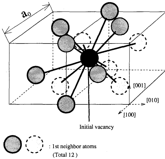
Fig. 4.7 Vacancy migration from 1st neighbor site (f.c.c. structure)
