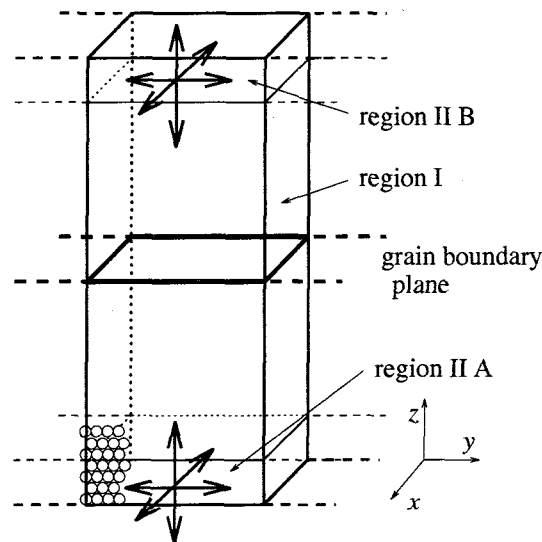
Fig. 2.2 Lutsko's method for grain boundary simulation (4)
