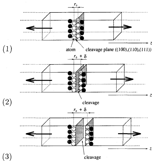
Fig. 3.2 Schematic picture of cleavage procedure((1)→(2)→(3))
