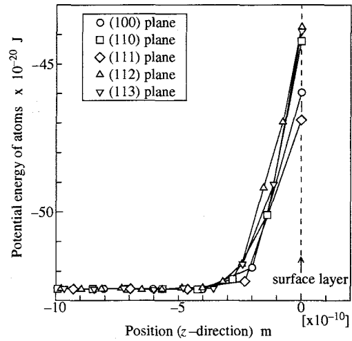
Fig. 2.6 Potential energy distribution of atom near the surface
