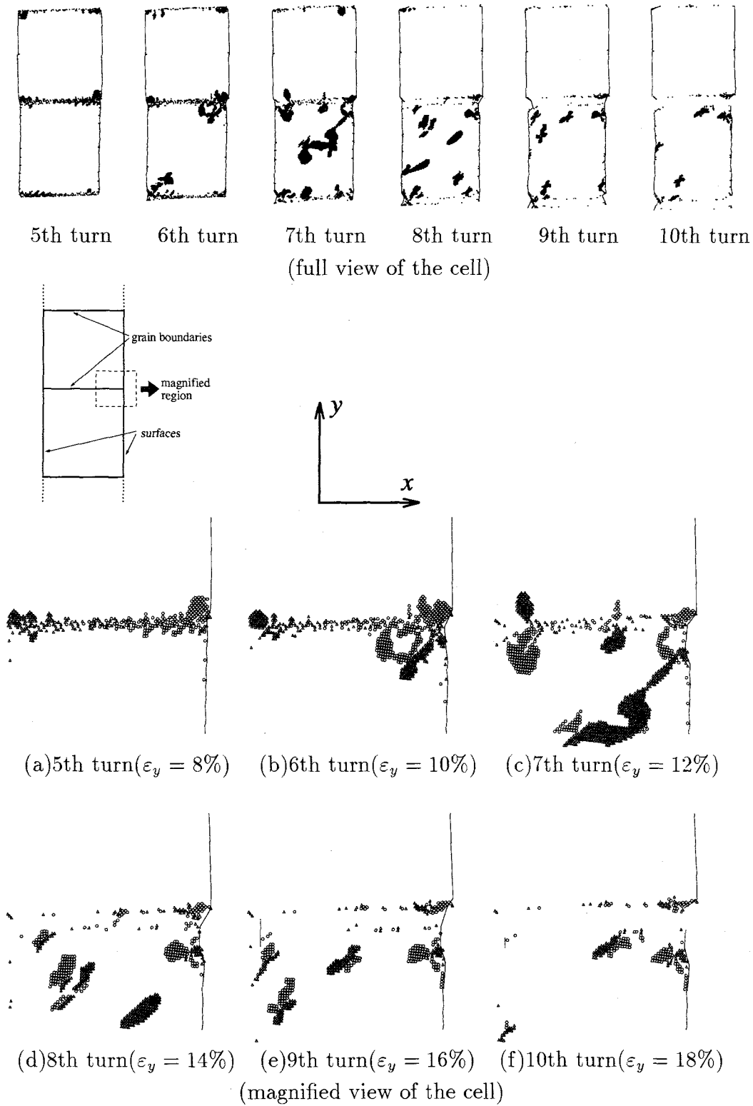
Fig. 6.21 Distribution of atomic shear stress \tau_i^{xy} being larger than a specific value in case (VI) (Only atoms with \tau_i^{xy} > 1\text{GPa} (○) or with \tau_i^{xy} < -1\text{GPa} (△) are displayed.)
