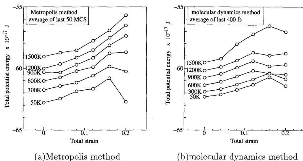
Fig. 4.20 Dependence of total potential energy on initial strain (For Metropolis simulation (a), potential energy is averaged from 4950 to 5000 MCS. For MD simulation (b), it is averaged from 19.6ps to 20.0ps.)
