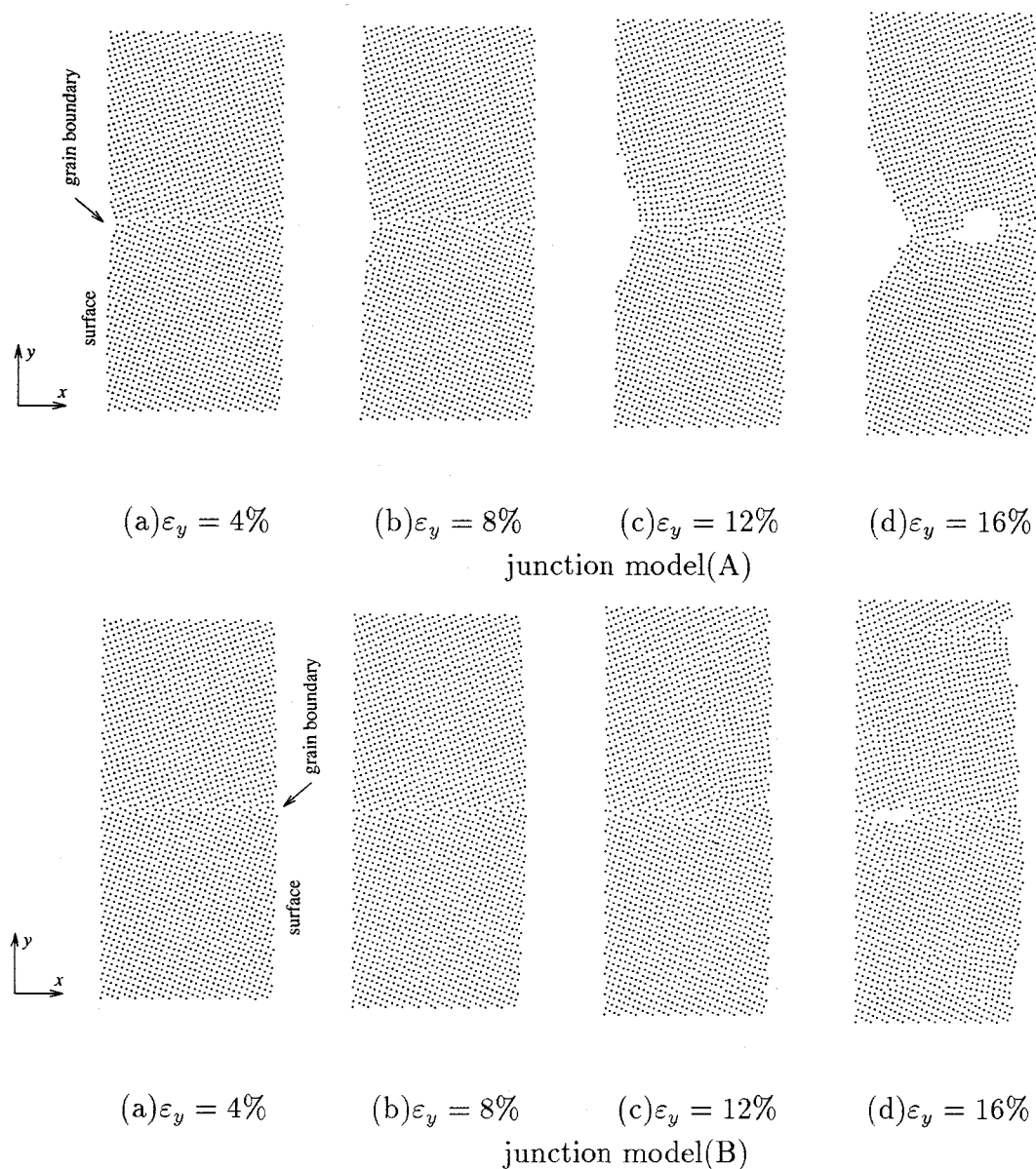
Fig. 6.31 Transition of atomic configuration during loading (projection on xy plane)
