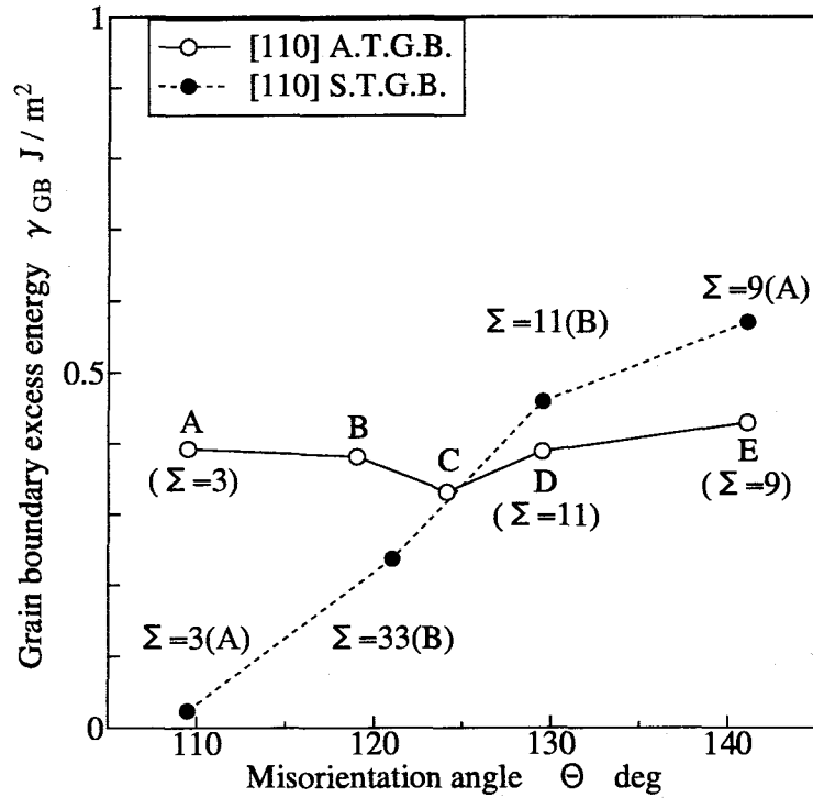
Fig. 2.28 Grain boundary energy vs. misorientation angle (range of misorientation angle \Theta = 109.47 \sim 141.06^\circ )
