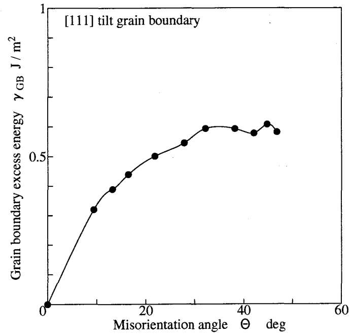
(a)[111] tilt grain boundary
