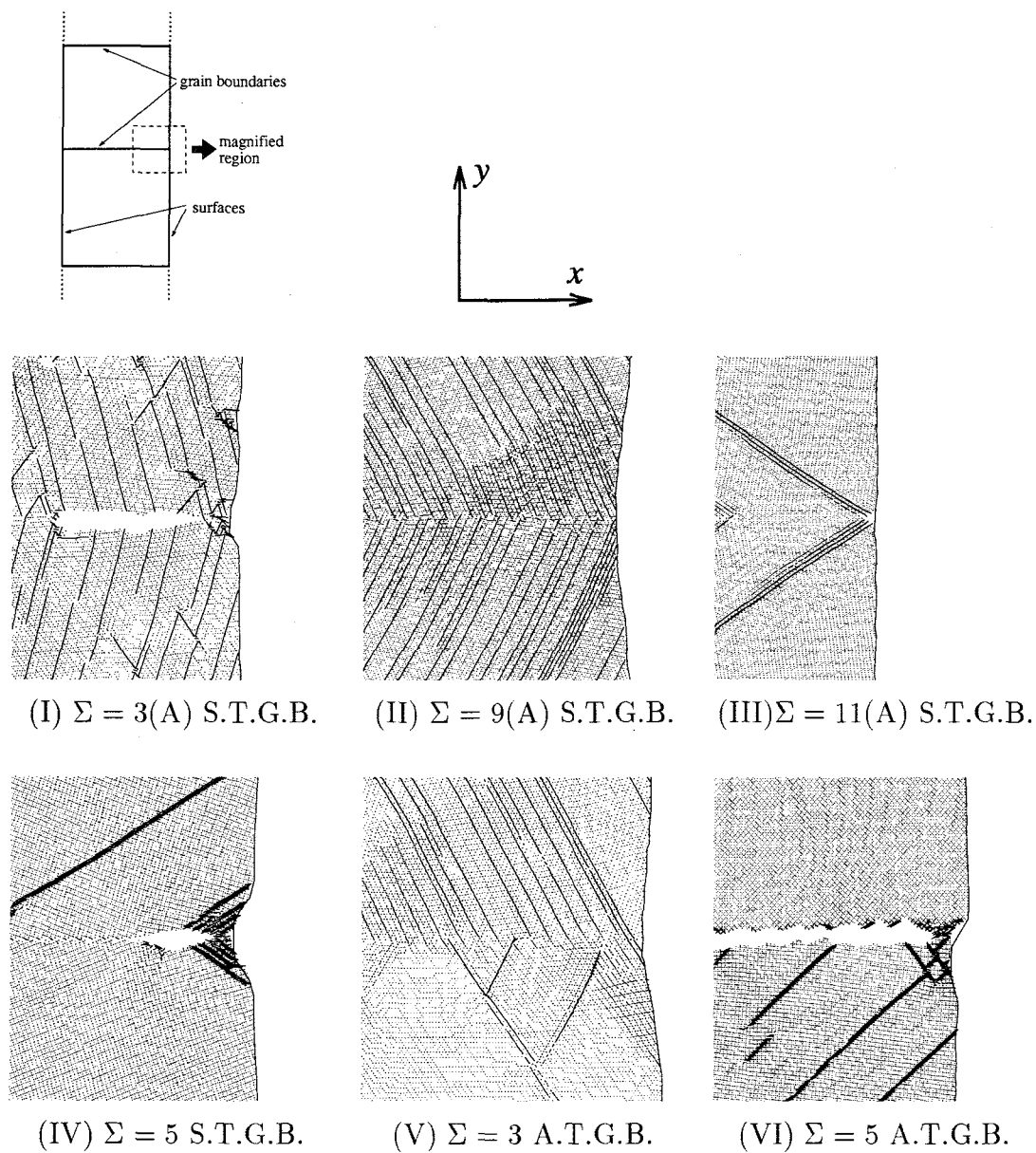
Fig. 6.28 Relative displacement of atoms from the initial state to 8th turn ( \varepsilon_y = 14\% ) (All u_{ij} are displayed. Region near the junction point is magnified. Surface is shown by solid curve.)
