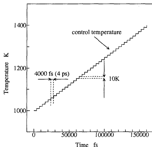
Fig. 2.8 Diagram of temperature control used for simulation of melting
