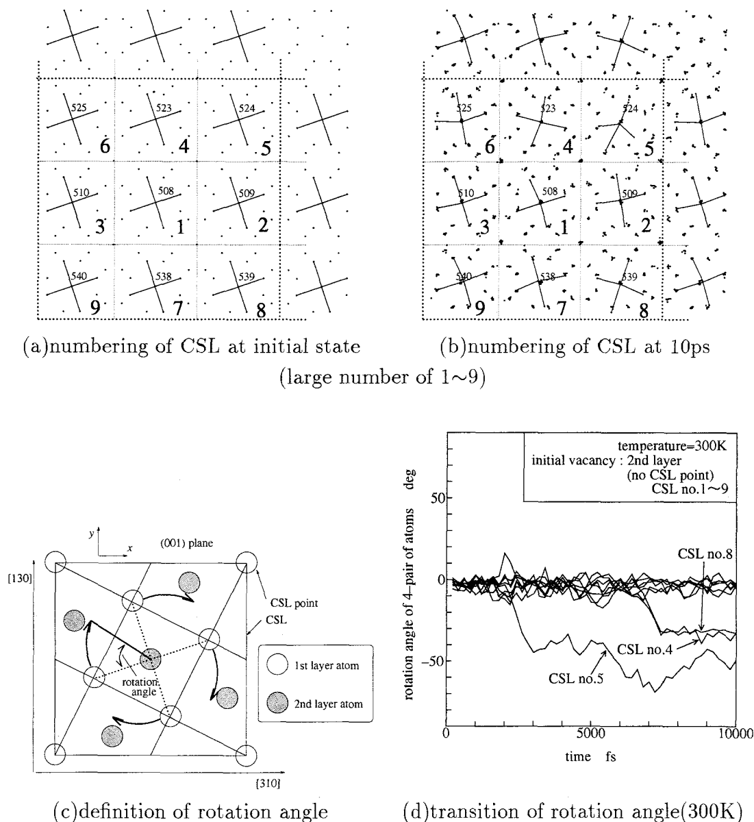
Fig. 4.6 Group rotation involving four atoms around CSL points
