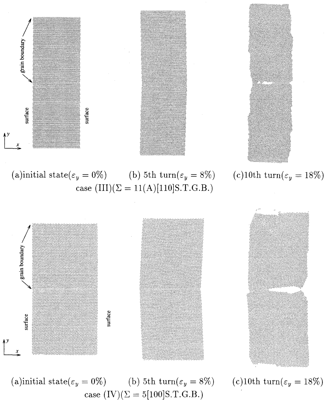
Fig. 6.12 Atomic configuration during loading(case (III),(IV); projection on xy plane)
