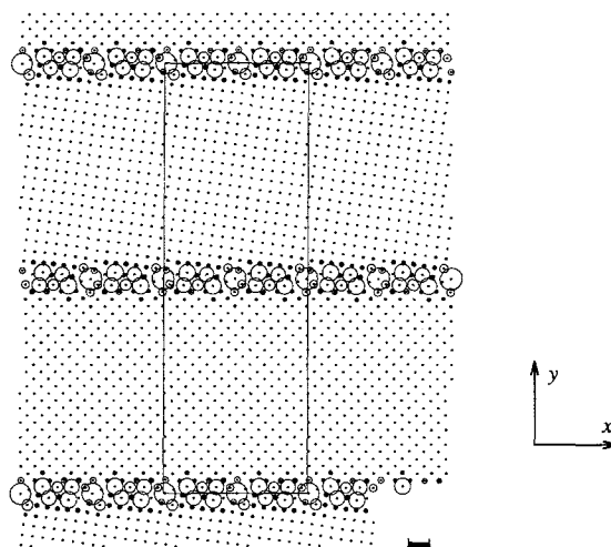
Fig. 2.30 Atomic configuration and energy distribution of \Sigma = 5[100] A.T.G.B. (Energy level of each atom is shown by circle centered at its position. Radius of the circle corresponds to energy level. Length of line segment at the lower right of figure corresponds to -4.3 \times 10^{-19} \text{J} . See Fig.2.15.)
