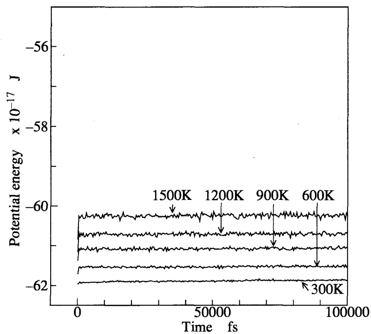
Fig. 4.14 Transition of total potential energy during shear loading
