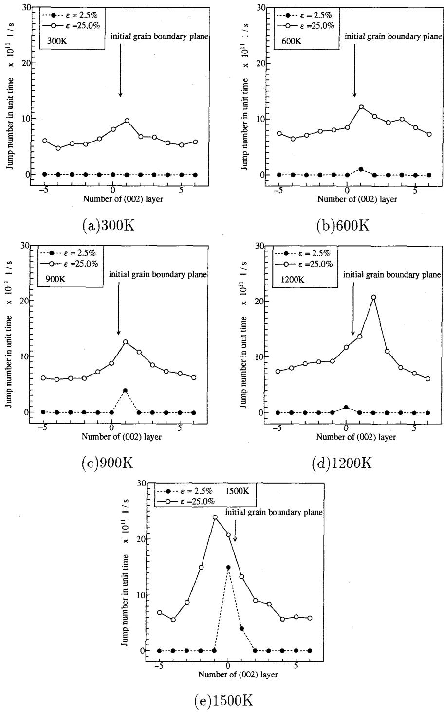
Fig. 4.12 Distribution of jump number along z direction during tensile loading
