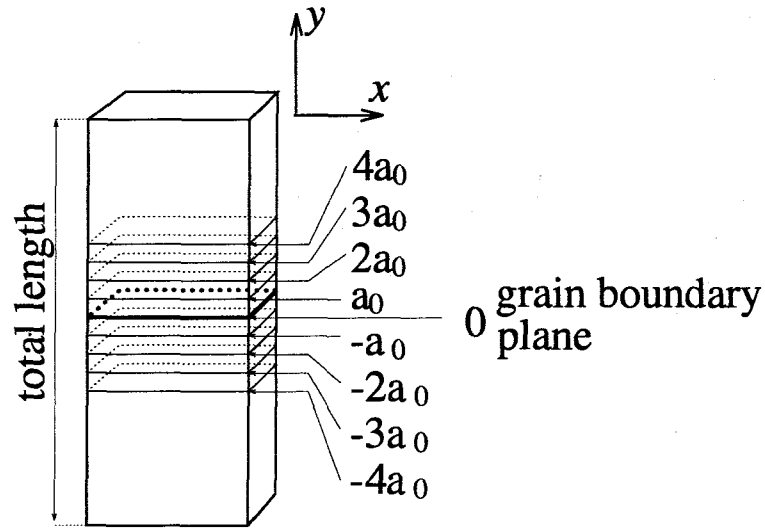
Fig. 3.16 Slabs with various thickness containing a grain boundary
