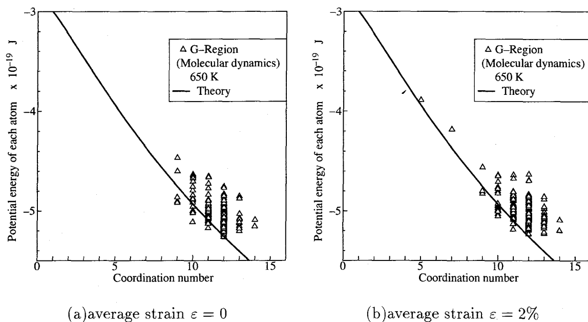
Fig. 5.20 Coordination number vs. potential energy of individual atoms in G-region
