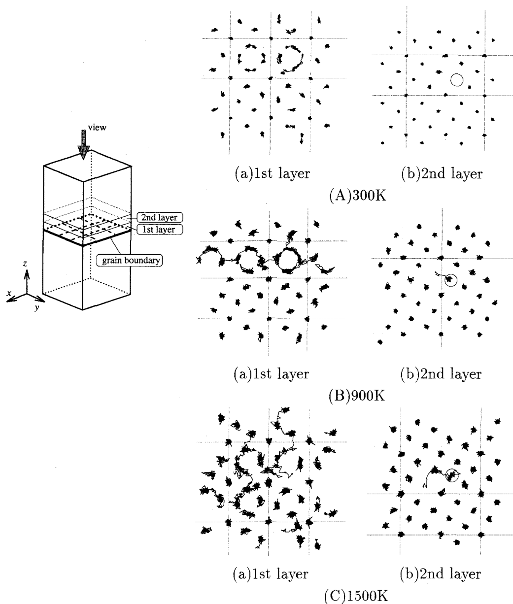
Fig. 4.5 Trajectory of atoms in 1st and 2nd layer defined in Fig.4.2. (Projections on xy plane(parallel to the grain boundary plane) are shown. Large circle indicates the position of initial vacancy and dotted lines denote the outline of CSL.)
