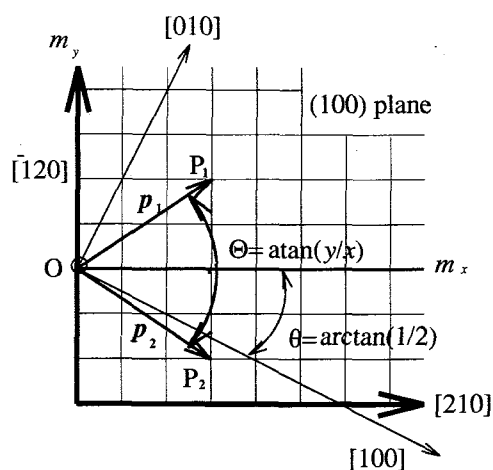
Fig. 2.29 Geometrical relation between crystallographic planes meeting at the grain boundary in [100] A.T.G.B. (case: \xi = 2 )
