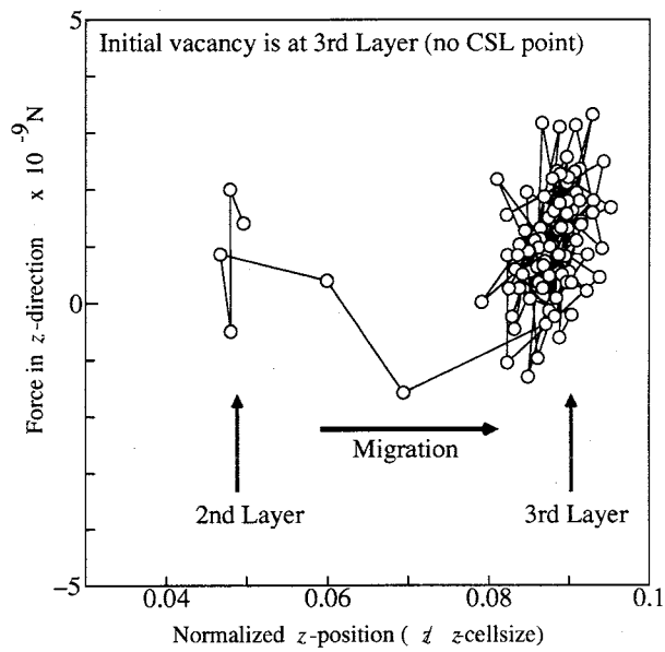
Fig. 4.4 Relation between displacement and force of an atom during jump motion
