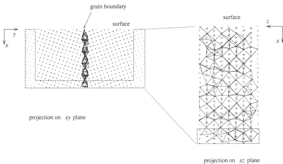
Fig. 5.6 Possible paths of atomic migration near the grain boundary (Line segments connecting atoms have the length less than 1st neighbor distance.)
