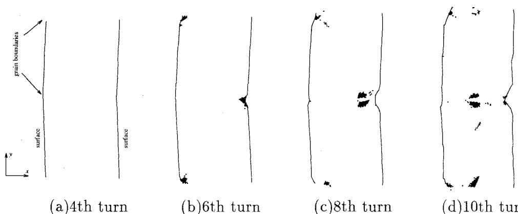
Fig. 6.24 Atoms having square displacement with the magnitude being larger than a specific threshold during one turn (case(IV))
