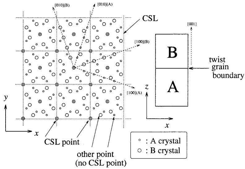
Fig. 4.3 Location of CSL points in \Sigma = 5[100] twist grain boundary
