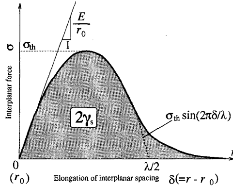
Fig. 3.1 Stress-spacing relation in cleavage process and its approximation by sine curve
