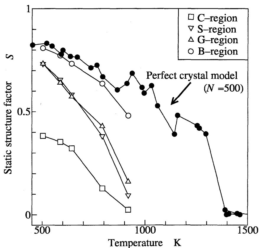
Fig. 5.7 Instantaneous static structure factor S
