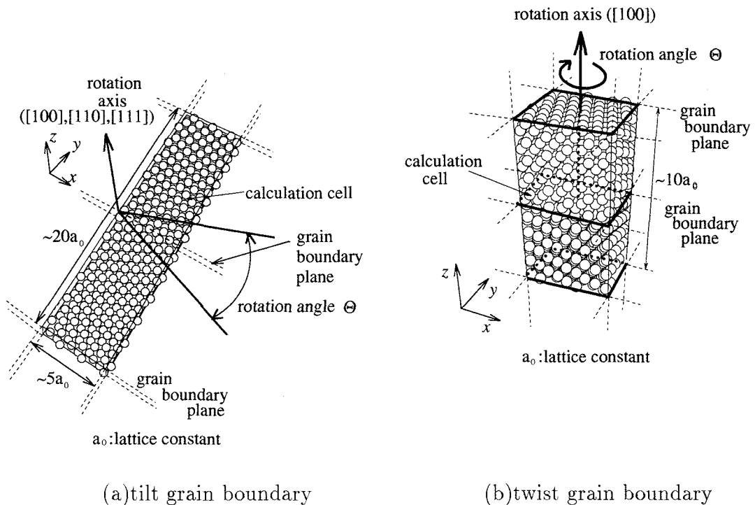
Fig. 2.13 Grain boundary models
