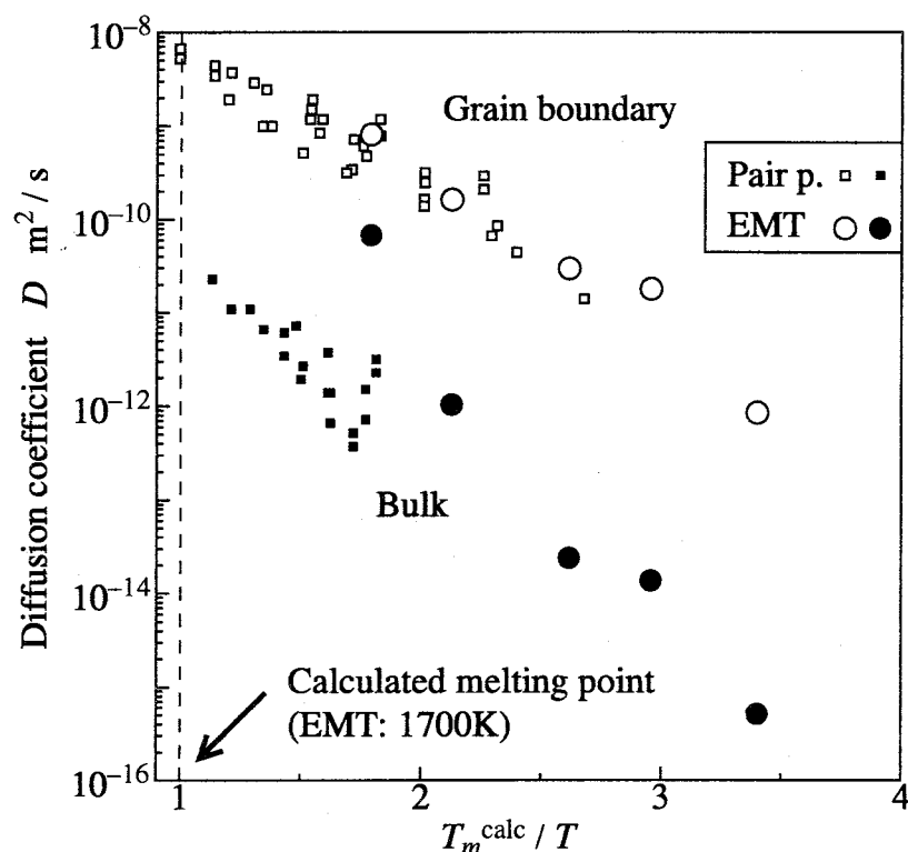
Fig. 5.14 Comparison of diffusion coefficient calculated by EMT(○, ●) with by pair-wise potential (□, ■) (10)
