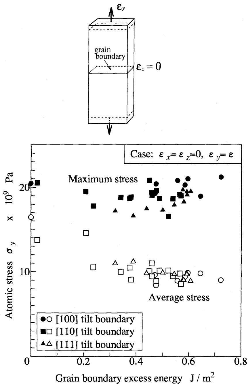
Fig. 3.15 Relation between grain boundary energy and fracture stress(case (a) in Fig.3.8)
