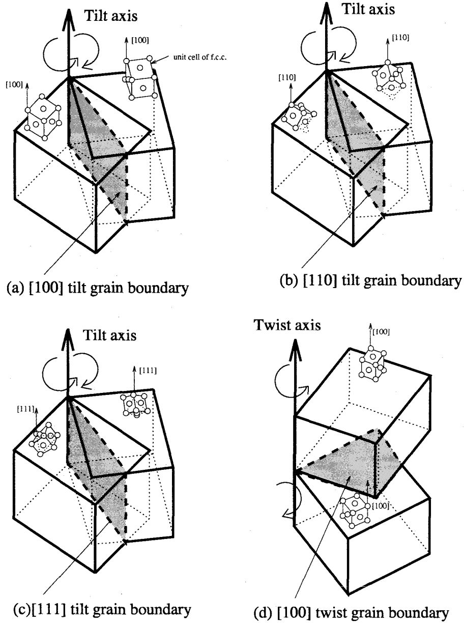
Fig. 2.12 Tilt and twist grain boundaries ((a)[100] tilt, (b)[110] tilt, (c)[111] tilt, (d)[100]twist)
