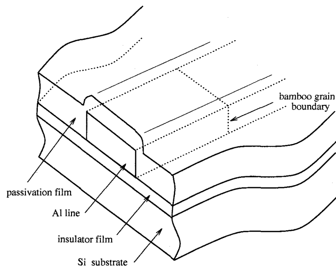
Fig. 5.1 Aluminum line in LSI
