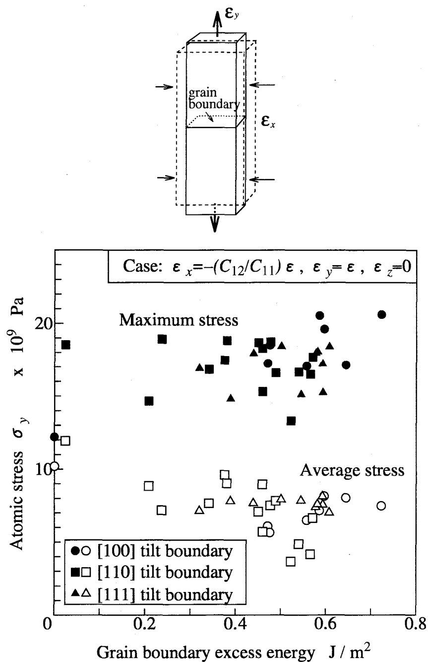
Fig. 3.21 Relation between grain boundary energy and fracture stress (side constraint is case (b) in Fig.3.8)
