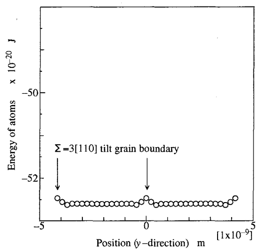
(a) \Sigma = 3(A)[110] tilt grain boundary
