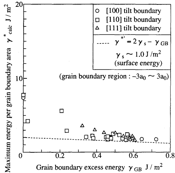
Fig. 3.19 Fracture energy estimated by MD calculation ( \gamma_{\text{calc}}^* is calculated with respect to atoms near the grain boundary)
