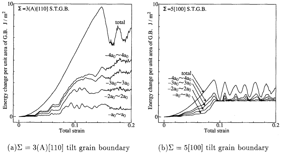
Fig. 3.17 Transition of potential energy contained in each slab defined in Fig.3.16
