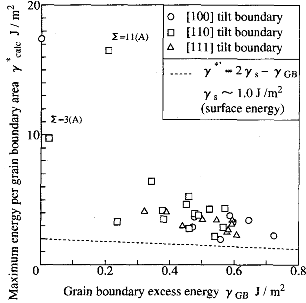
Fig. 3.18 Fracture energy estimated by MD calculation ( \gamma_{\text{calc}}^* is calculated with respect to all atoms in cell)
