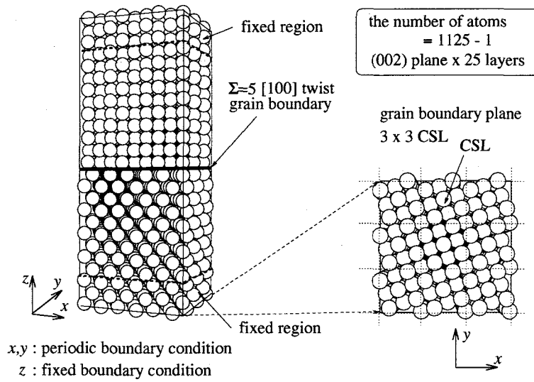
Fig. 4.1 \Sigma = 5[100] twist grain boundary model
