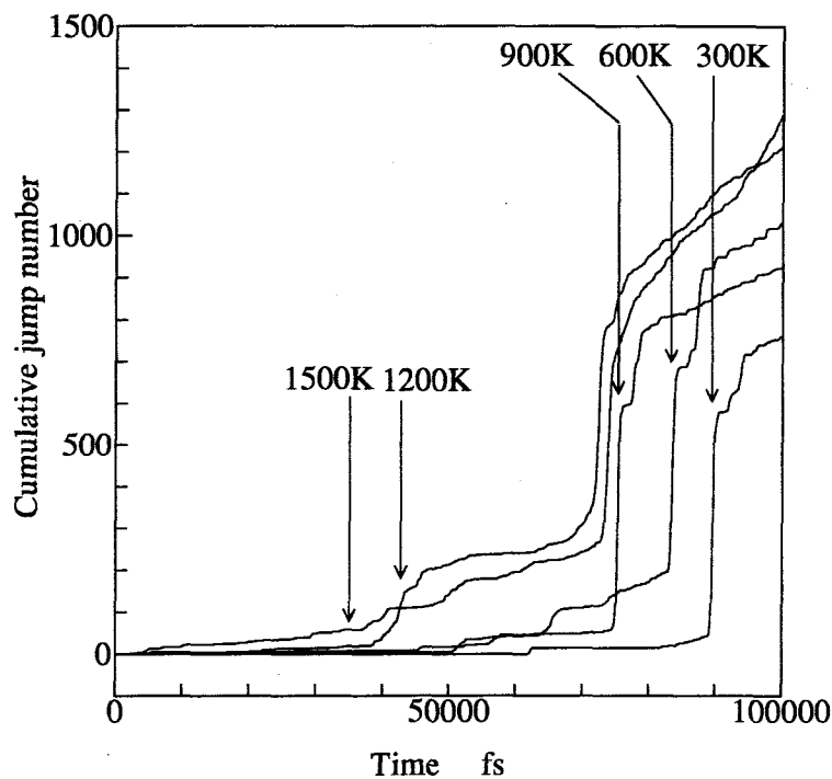
Fig. 4.13 Transition of cumulative jump number during tensile loading
