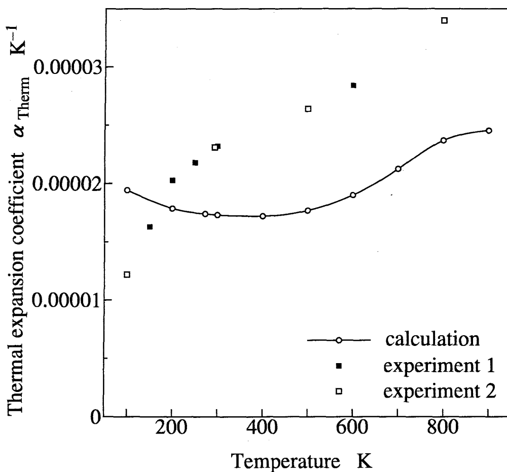
Fig. 2.7 Thermal expansion coefficient (with experimental data 1 (39) , 2 (40) )
