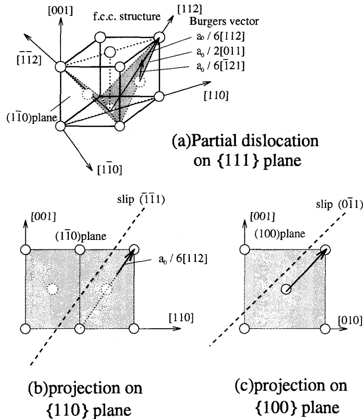
Fig. 6.26 Explanation of slip plane and Burgers vector in f.c.c. lattice
