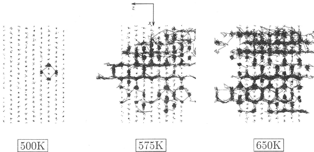
Fig. 5.5 Trajectory of atoms initially in G-region (projection on xz plane)
