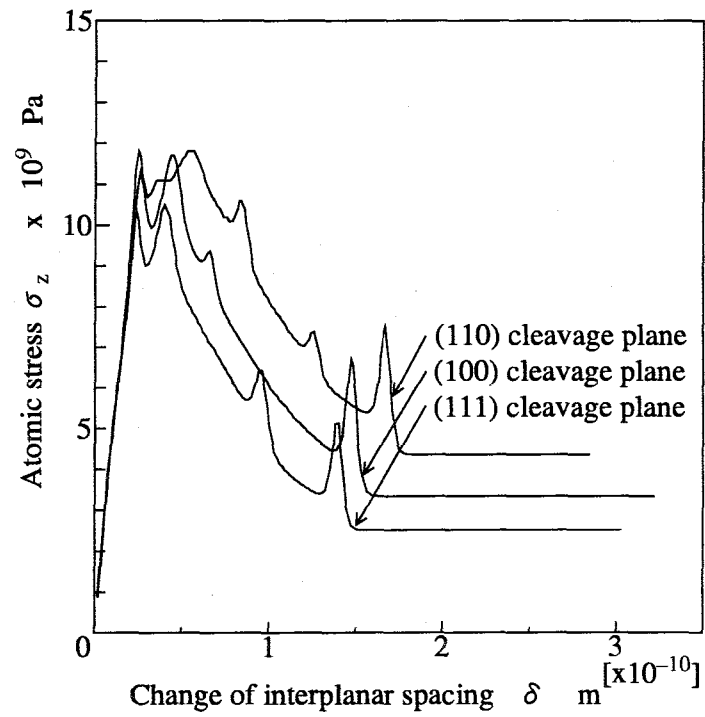
Fig. 3.4 Relation between interplanar spacing and normal stress ( \sigma_z ) of atom (for three cleavage planes)
