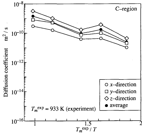
(a)C-region
