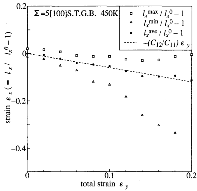
Fig. 6.33 Transition of maximum, minimum and average strain in x direction (junction model(A)(450K))
