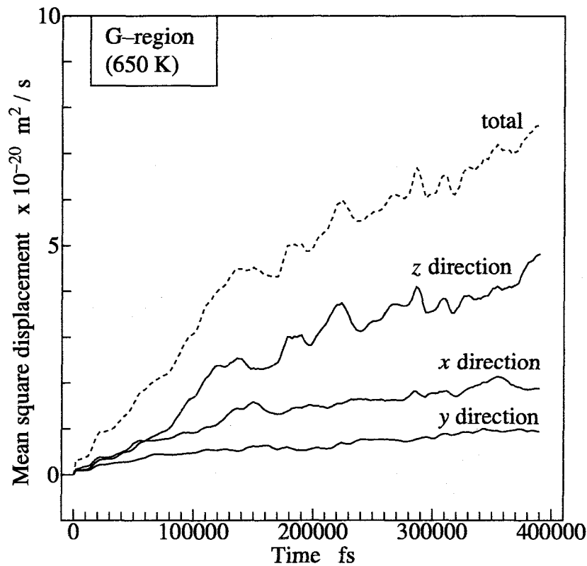
Fig. 5.11 Directional dependence of MSD in G-region (650K)
