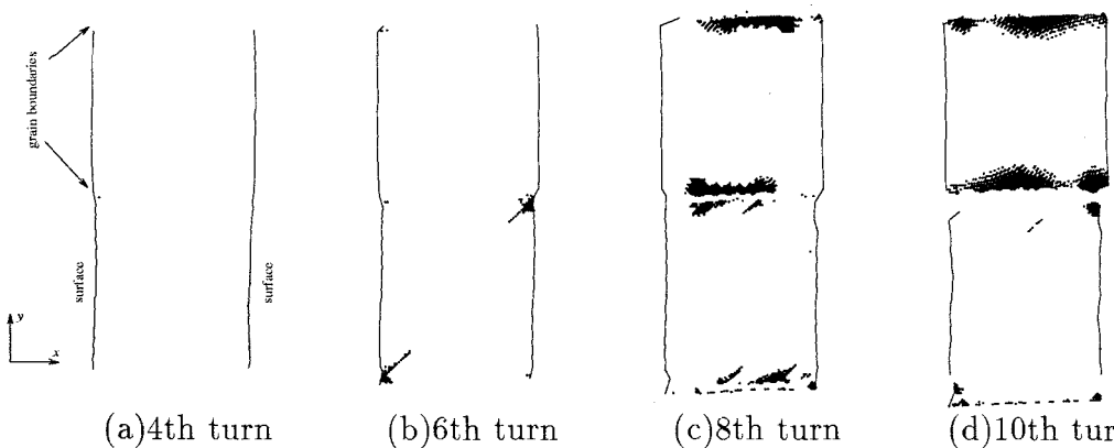
Fig. 6.25 Atoms having square displacement with the magnitude being larger than a specific threshold during one turn (case(VI))
