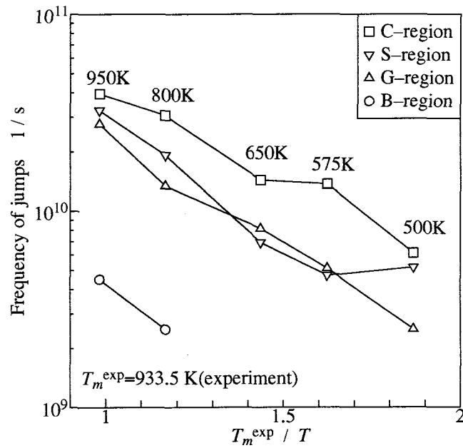
Fig. 5.9 Regional dependence of frequency of jumps
