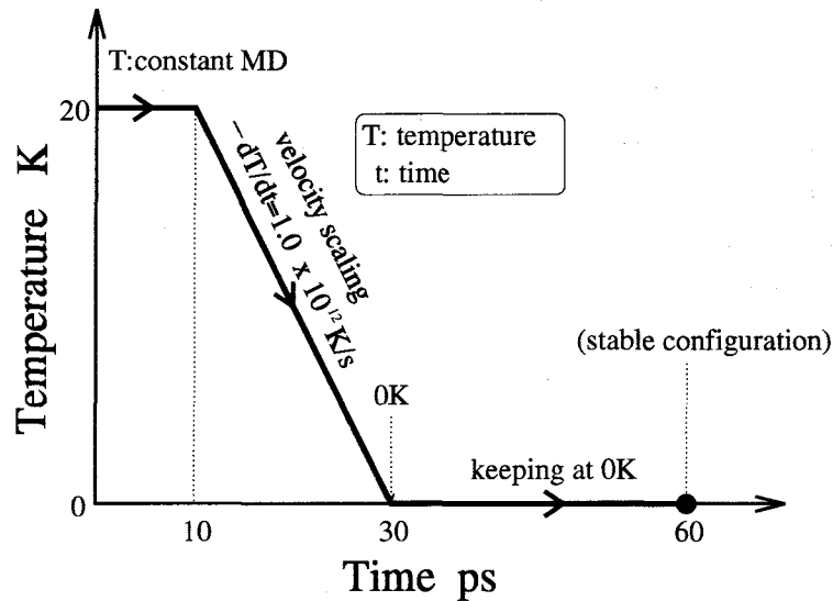
Fig. 2.14 Temperature control diagram to lead to a stable grain boundary structure at 0 K
