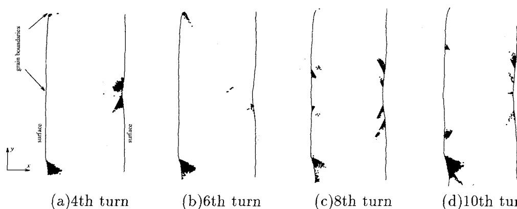
Fig. 6.23 Atoms having square displacement with the magnitude being larger than a specific threshold during one turn (case(II))
