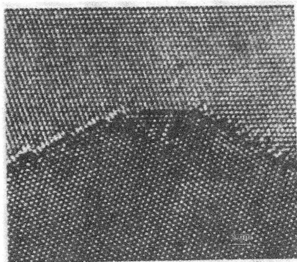
Fig. 1.1 High-resolution microscopy image of Au tilt grain boundary (Merkle, K. and Wolf, D., (1992) (20) )
