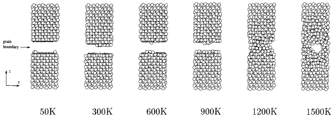
(b)molecular dynamics method (20 ps)
