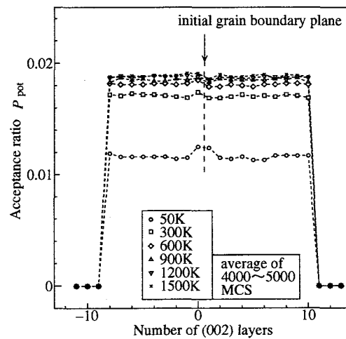
Fig. 4.22 Distribution of acceptance ratio P_{\text{pot}} in Metropolis simulation
