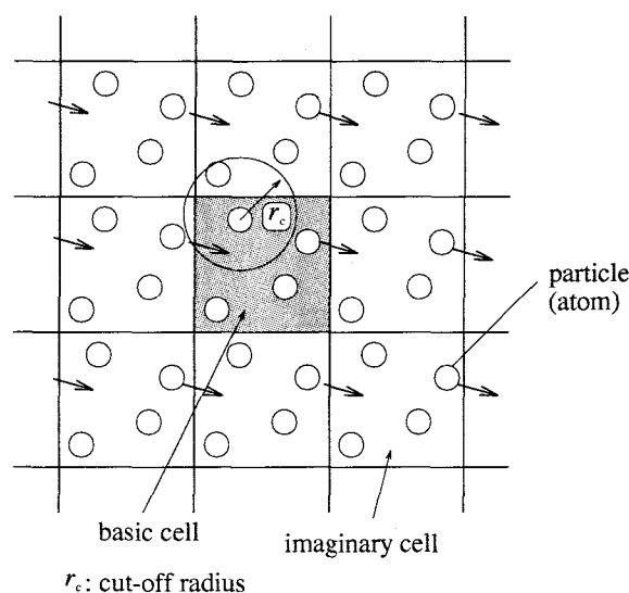
Fig. 2.1 Periodic boundary condition
