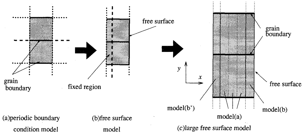
Fig. 6.1 Generation of free surface model
