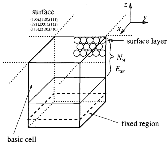
Fig. 2.5 Model used for calculation of surface energy
