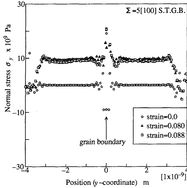
Fig. 3.12 Distribution of \sigma_y along y direction ( \Sigma = 5[100] tilt grain boundary)
