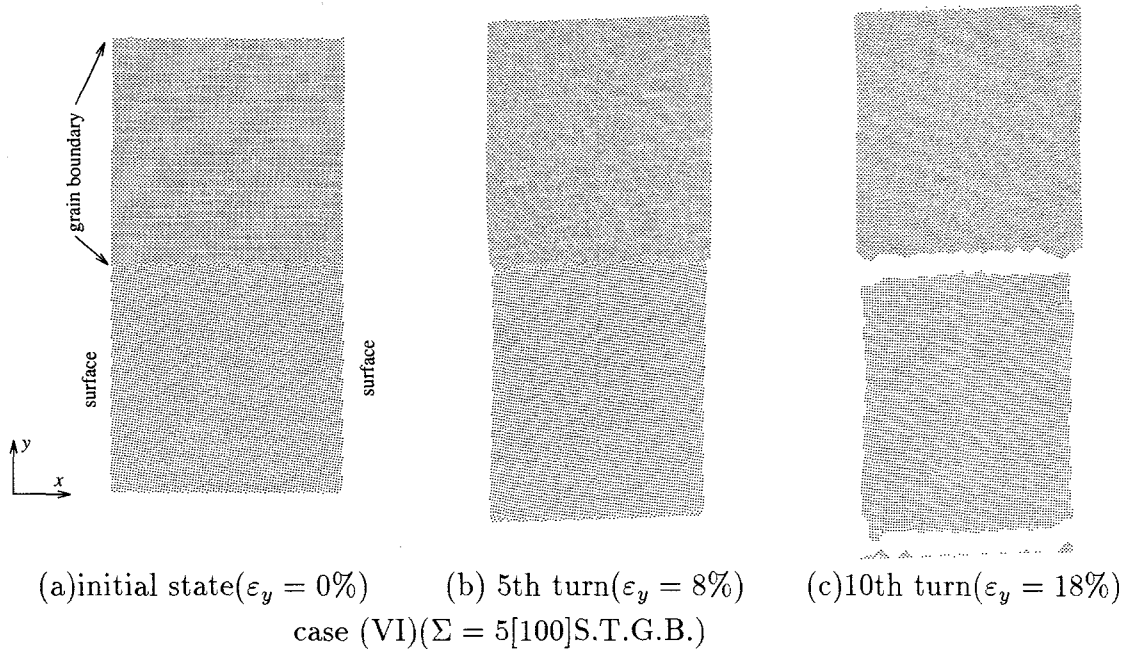
Fig. 6.13 Atomic configuration during loading(case (V),(VI); projection on xy plane)
