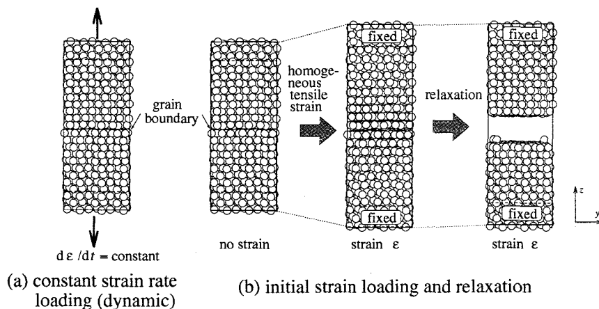
Fig. 4.17 Two tensile loading methods ((b) is used in both MD and Metropolis simulations.)
