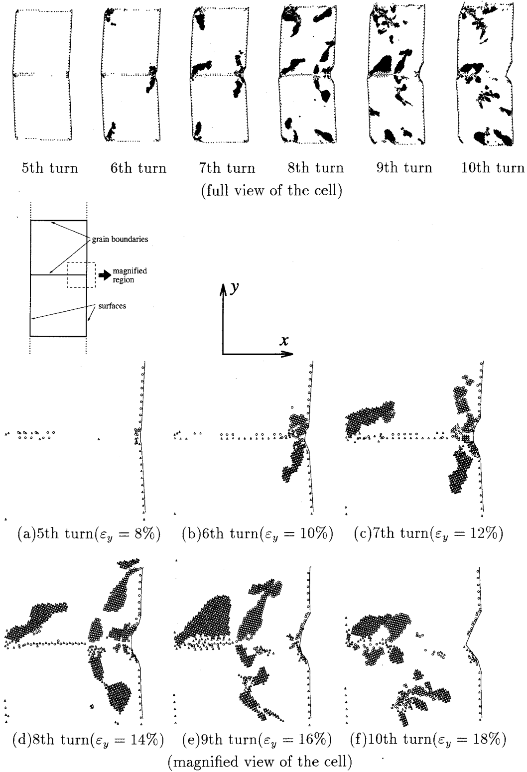
Fig. 6.20 Distribution of atomic shear stress \tau_i^{xy} being larger than a specific value in case (IV) (Only atoms with \tau_i^{xy} > 1\text{GPa} ( \bigcirc ) or with \tau_i^{xy} < -1\text{GPa} ( \triangle ) are displayed.)
