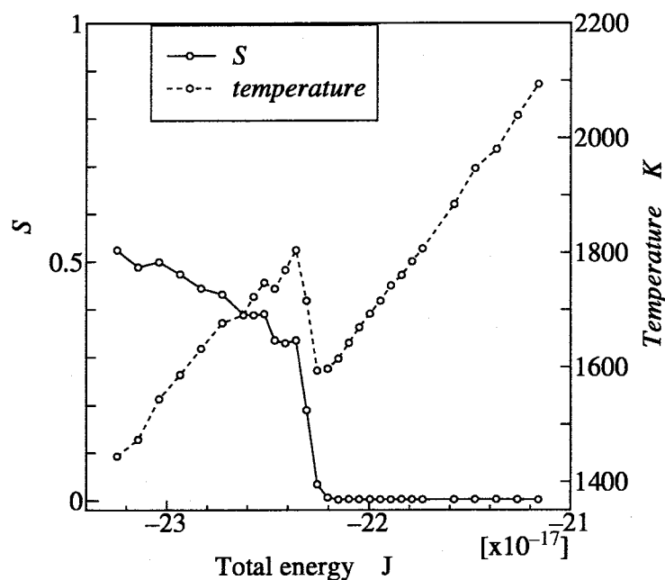
Fig. 5.15 Dependence of S and temperature on total energy ( S and temperature are averaged over 10ps.)
