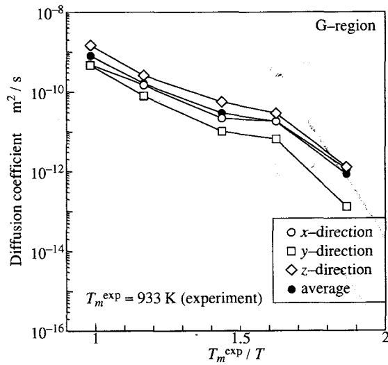
(c)G-region
