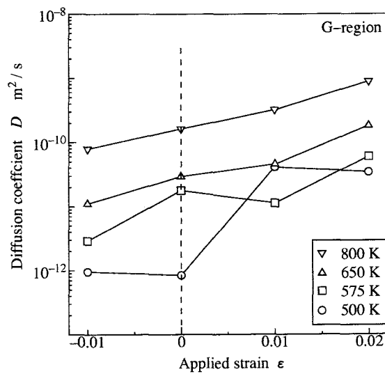
(c) G-region
