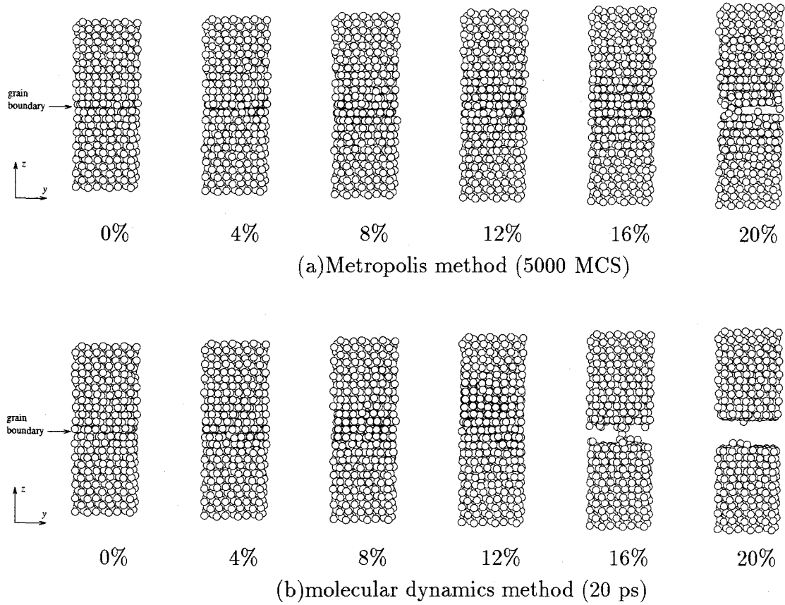
Fig. 4.21 Atomic configurations obtained by Metropolis method and MD method (Temperature of the system is kept at 600K.)
