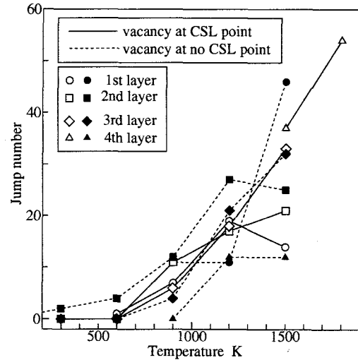
Fig. 4.8 Cumulative jump number during thermal equilibrium calculation (20ps)
