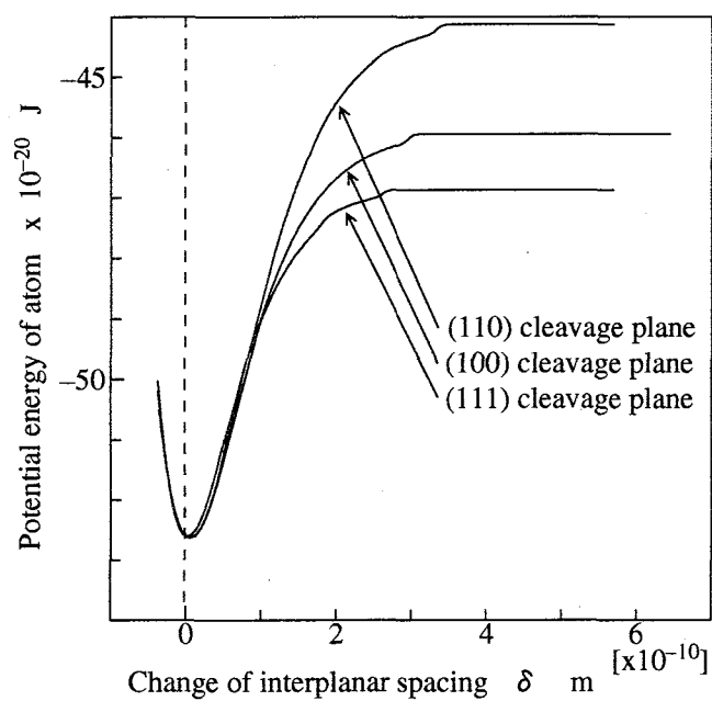
Fig. 3.3 Relation between interplanar spacing and potential energy of atom (for three cleavage planes)
