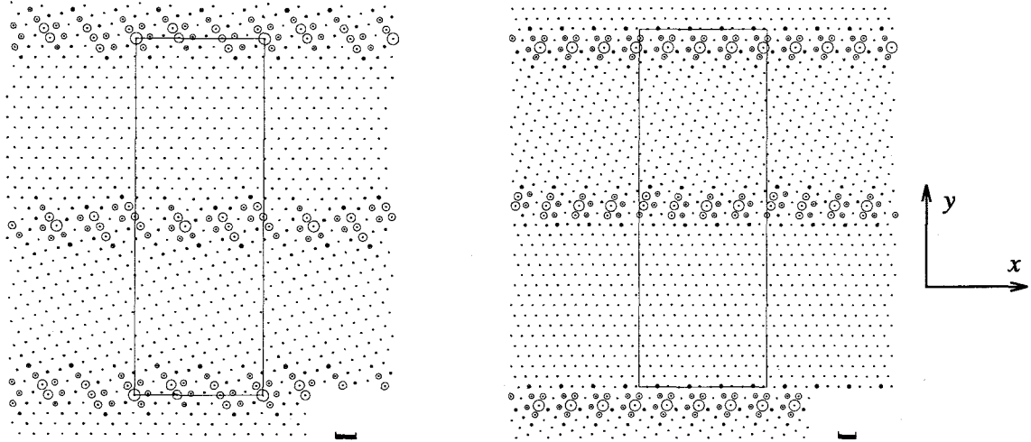
[110]A.T.G.B. (A)
