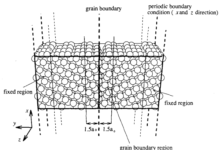
Fig. 5.22 Periodical grain boundary model for estimation of diffusion coefficient of [110] or [100] S.T.G.B.
