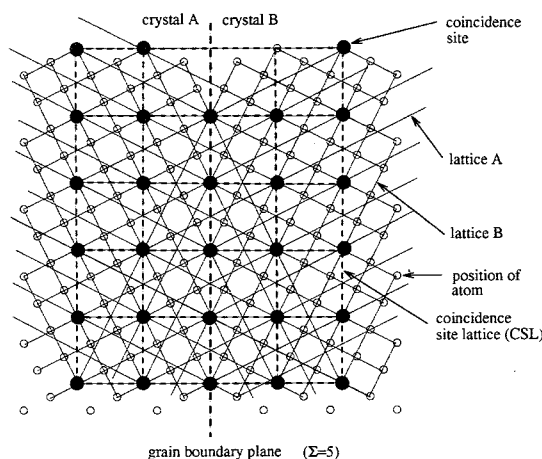
Fig. 2.10 Coincidence site lattice
