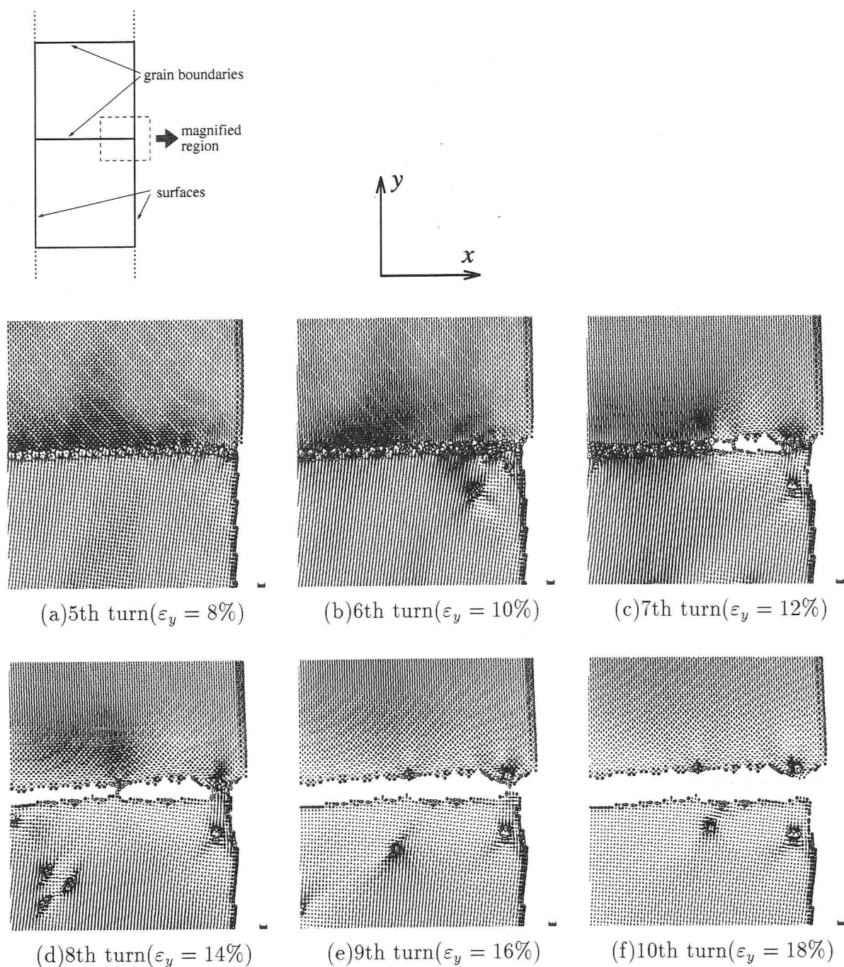
Fig. 6.18 Distribution of principal stress in case (VI) (Region near the junction point is magnified. Length of line segment at the lower right of each figure corresponds to 20GPa.)
