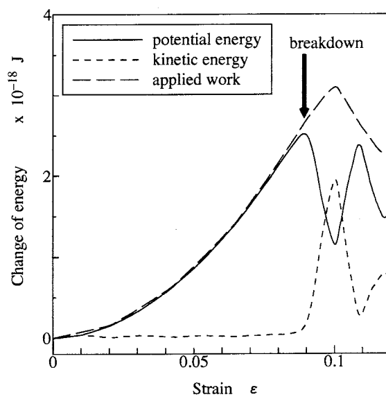
Fig. 3.10 Transition of potential energy, kinetic energy and applied work during loading ( \Sigma = 5[100] tilt grain boundary)
