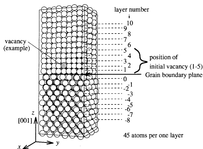
Fig. 4.2 Numbering of (002) layers and initial position of vacancy
