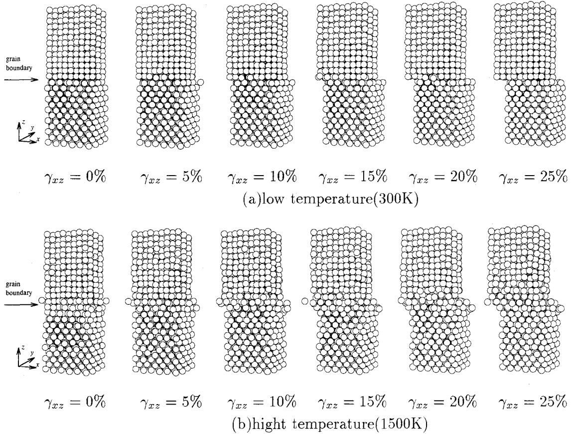
Fig. 4.15 Atomic configuration during shear loading
