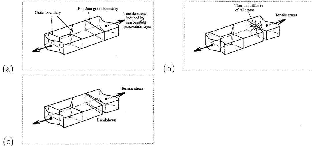
Fig. 5.2 Process of stress migration failure in aluminum lines (Void is nucleated and grows along the bamboo grain boundary ((a)→(b)→(c)).)
