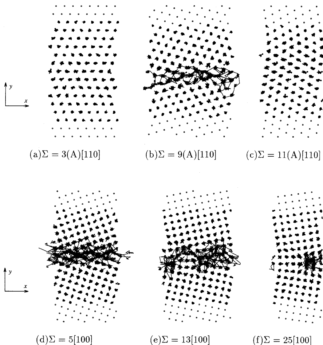
Fig. 5.23 Trajectories of atoms during 0.1ns (projection on xy plane)
