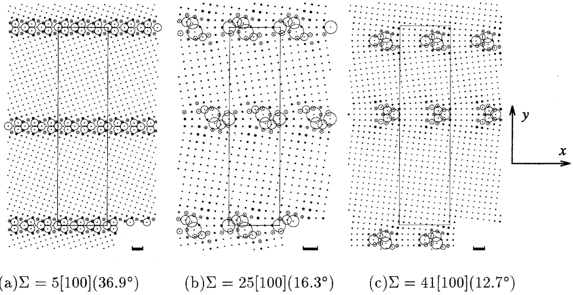
Fig. 2.18 Atomic configuration and energy distribution of [100] tilt grain boundaries (Energy level of each atom is shown by circle centered at its position. Radius of the circle corresponds to the energy level. Length of line segment at the lower right of each figure corresponds to -4.3 \times 10^{-19} \text{J} . See Fig.2.15.)
