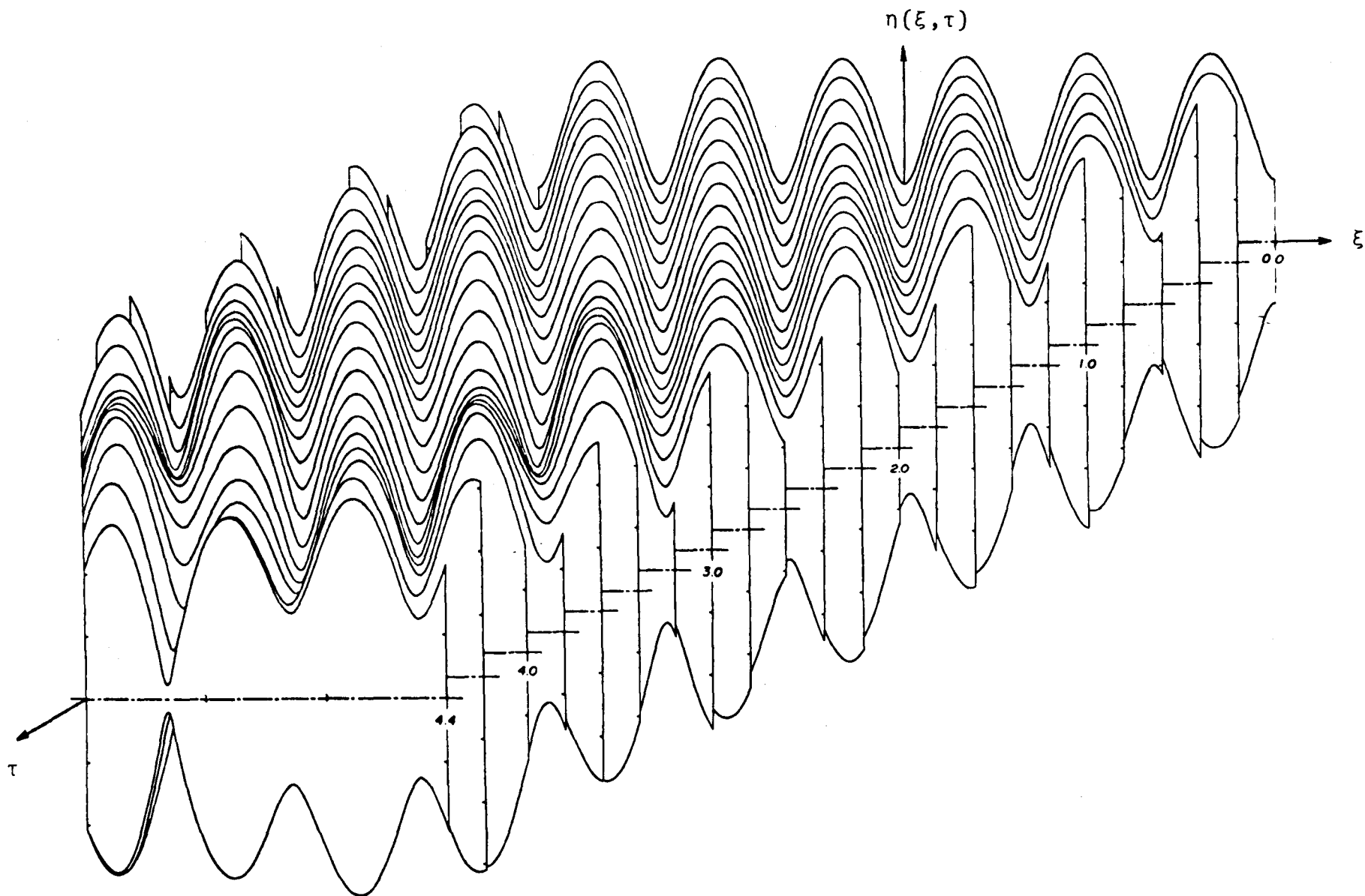
Fig.8. Variations of free surface \eta for Case (II). In the initial stage the minimum trough is placed at \xi = 0 . The wave profiles are drawn over two wavelengths of the disturbance.
