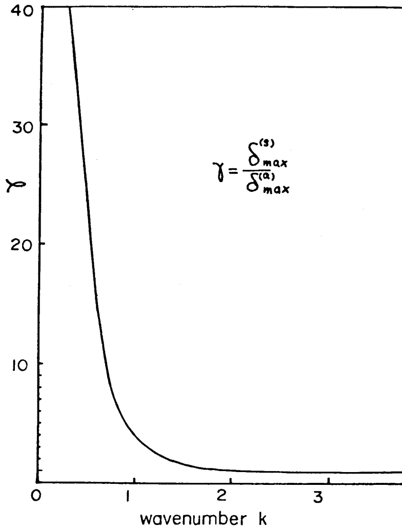
Fig.5. Variation of the ratio \gamma = \delta_{\max}^{(s)} / \delta_{\max}^{(a)} as a function of the wavenumber k . The superscripts (s) and (a) denote the symmetrical and antisymmetrical waves, respectively.
