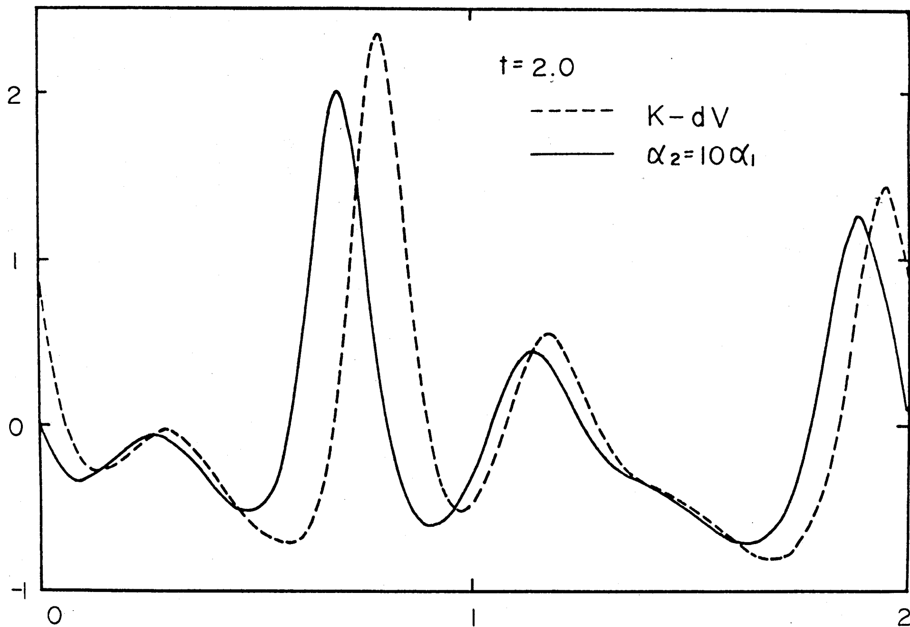
Fig.4. Wave forms at t = 2.0 for Case A_1 and K-dV solution
