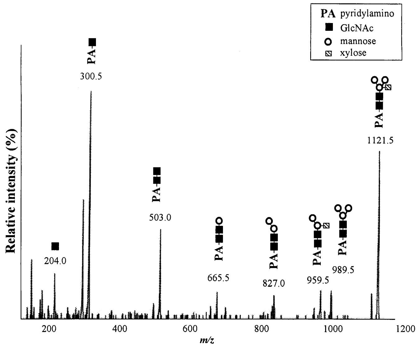
Fig. 10. MS/MS spectrum of PA-sugar chain F-IV-a ( m/z 1121.5).
