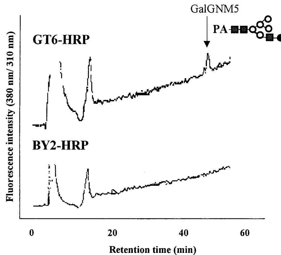
Fig. 29. Reversed-phase HPLC of PA-sugar chains from purified HRP after RCA_{120} affinity chromatography. PA-sugar chains were eluted from Cosmosil 5C18-P column (6 x 250 mm) by increasing the acetonitrile concentration in 0.02% TFA linearly from 0 to 15% for 60 min at a flow rate of 1.2 ml/min. Excitation and emission wavelengths were 310 nm and 380 nm, respectively. Only one major peak was observed from GT6-HRP. The PA-labeled sample corresponded to the expected elution position of Gal_1GlcNAc_1Man_5GlcNAc_2 (GalGNM5).
