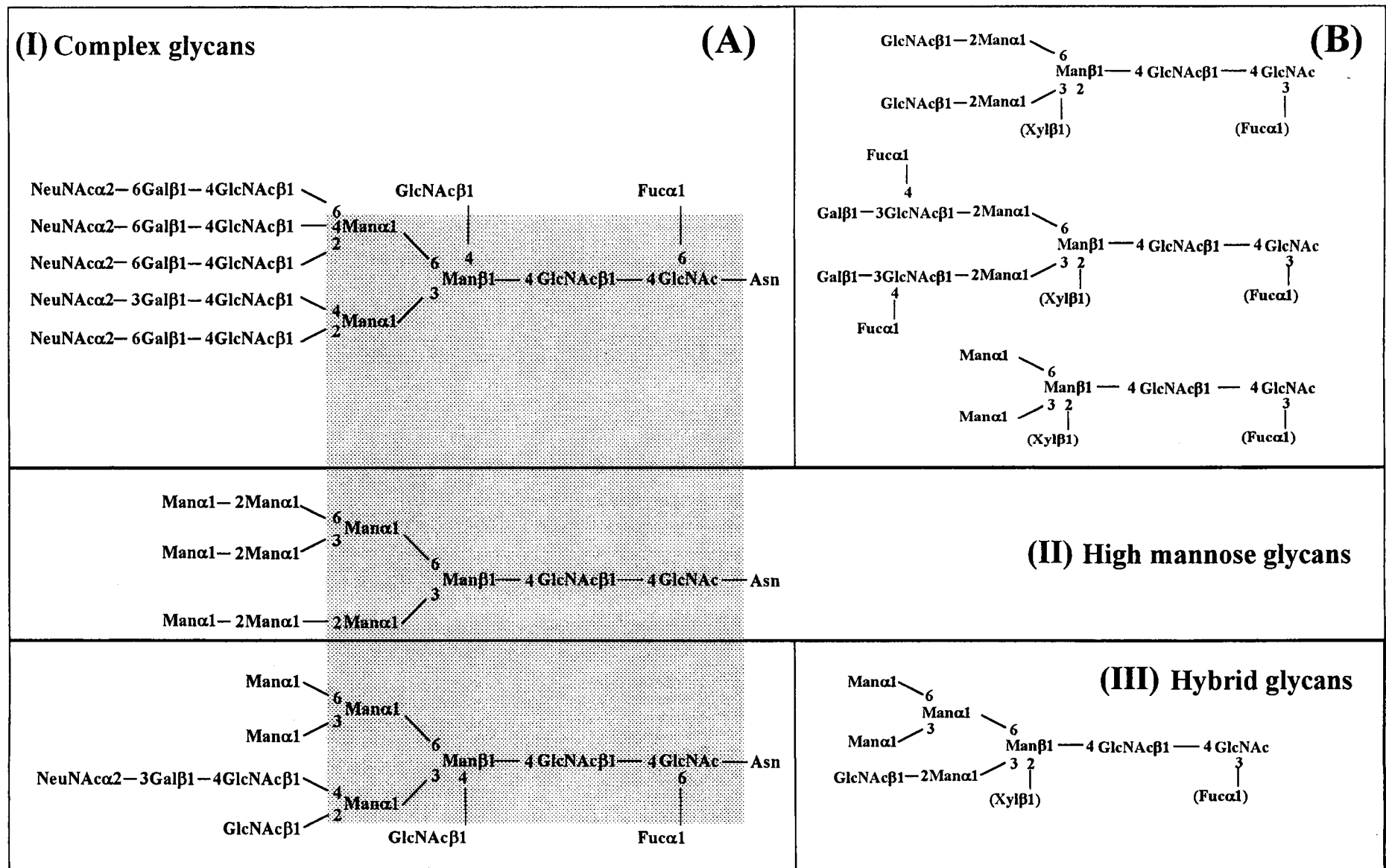
Fig. 2. Sub-groups of N -linked sugar chains. The structure within the shaded box is the trimannosyl core common to all N -linked glycans. (A) Representatives from mammalian glycoproteins; (B) representatives from plant glycoproteins.
