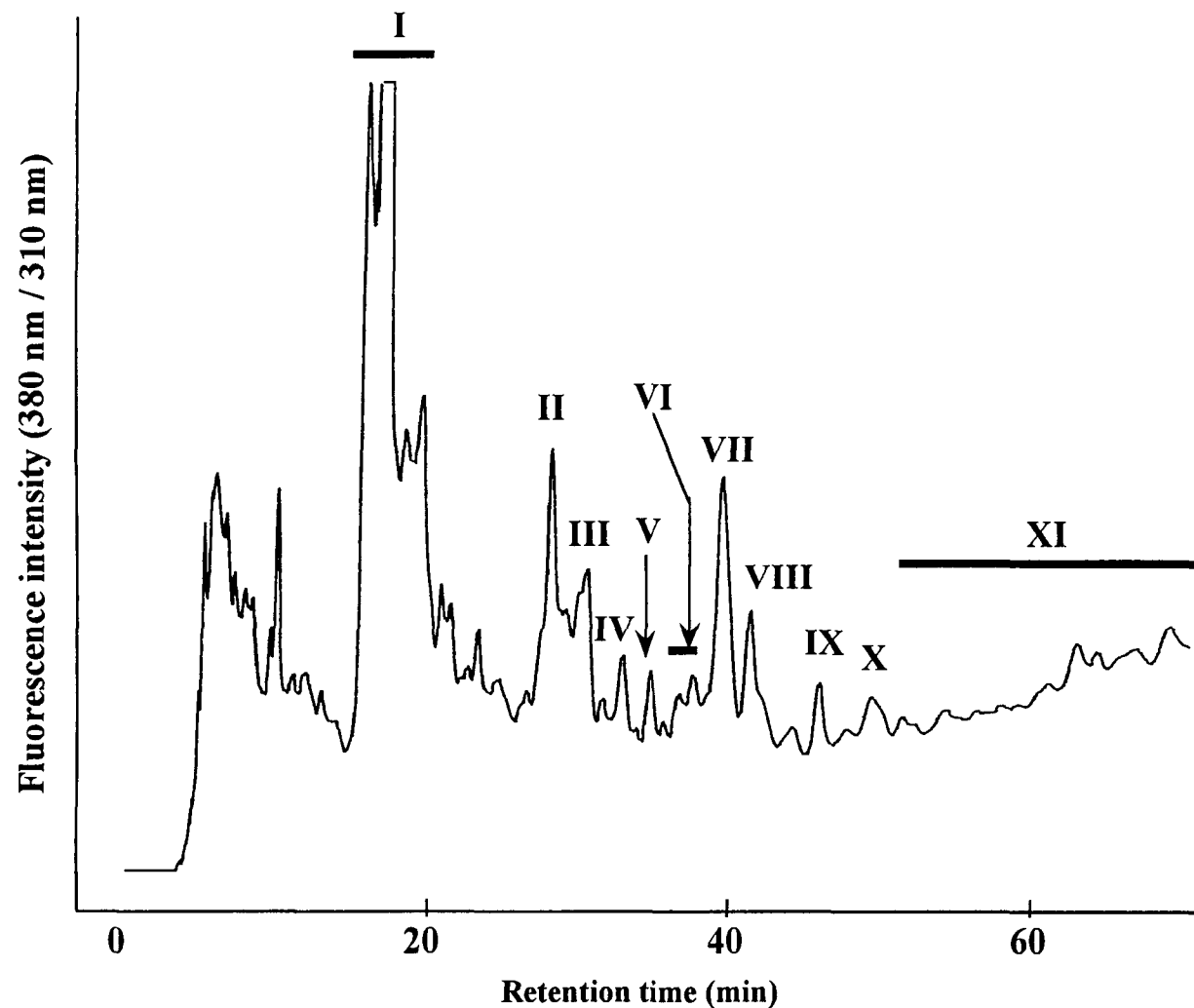
Fig. 16. Reversed-phase HPLC pattern of PA-derivatives prepared from transformed cells. PA-sugar chains were eluted by increasing the acetonitrile concentration in 0.02% TFA linearly from 0 to 15% for 60 min at a flow rate of 1.2 ml/min. I-XI indicate individual fractions collected and purified for size-fractionation HPLC.
