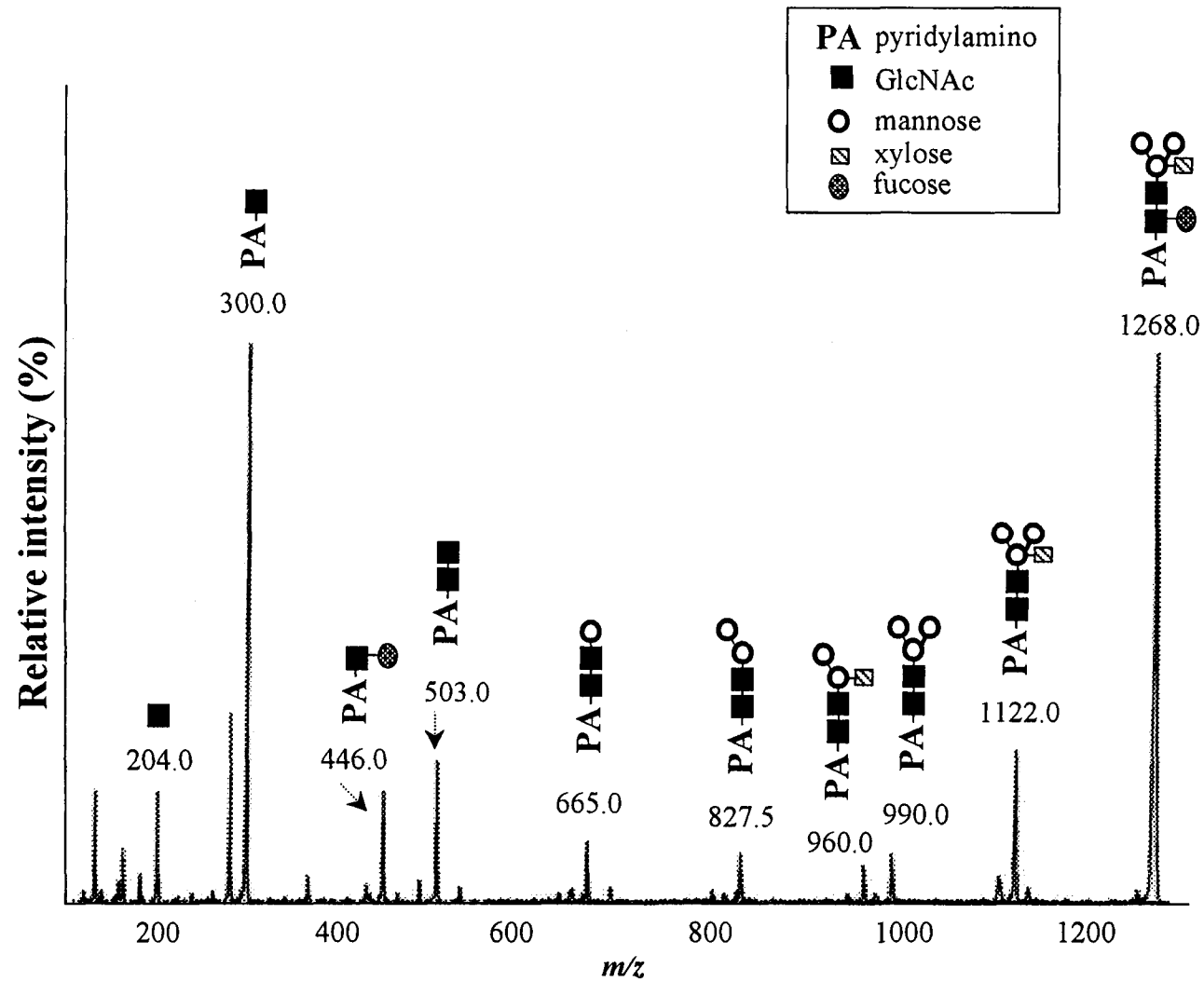
Fig. 6. MS/MS spectrum of PA-sugar chain F-I ( m/z 1268.0).
