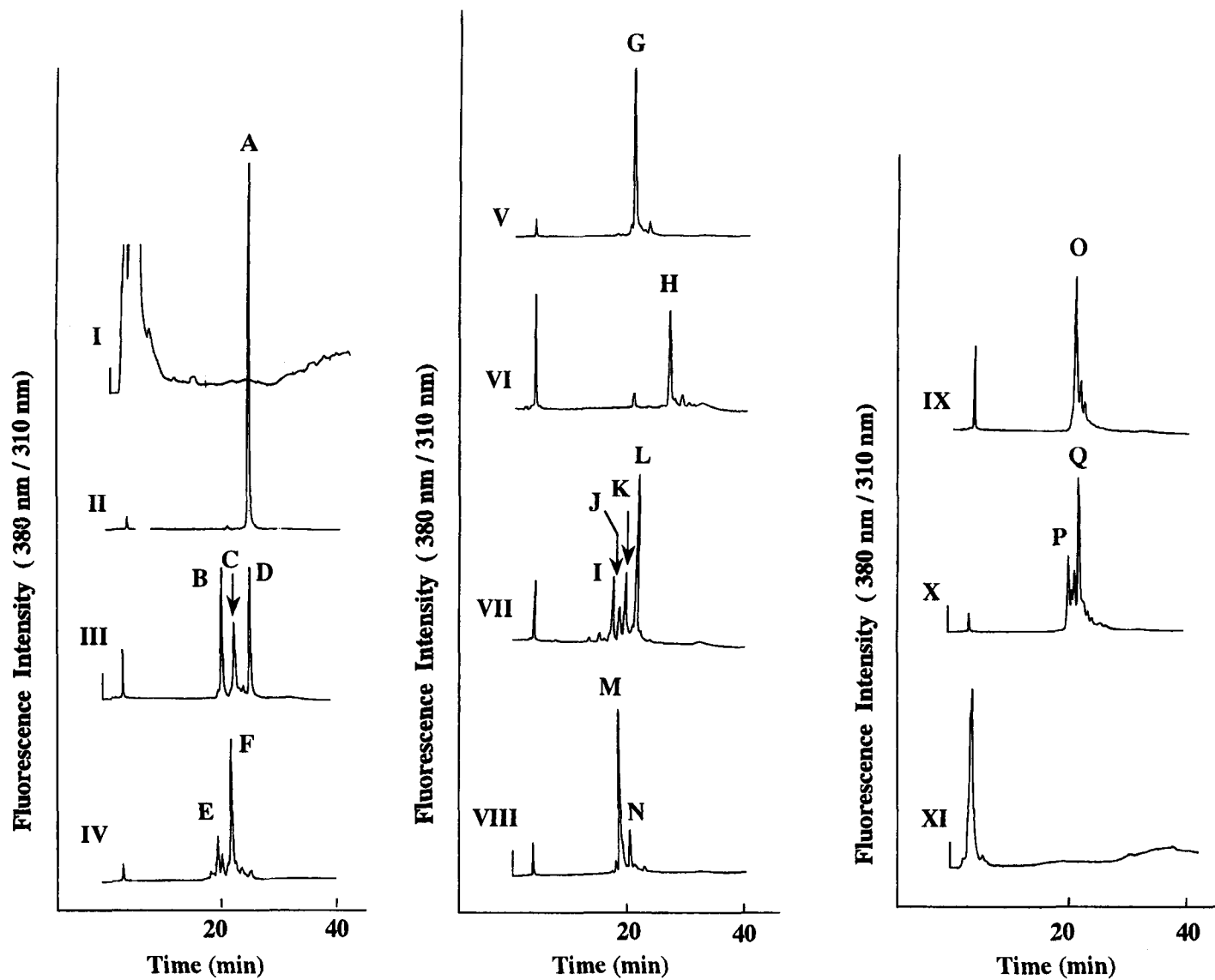
Fig. 17. Size-fractionation HPLC of PA-sugar chains from Fig. 15. PA-sugar chains were eluted by increasing the water content in the water-acetonitrile mixture from 30% to 50% for 40 min at a flow rate of 0.8 ml/min.
