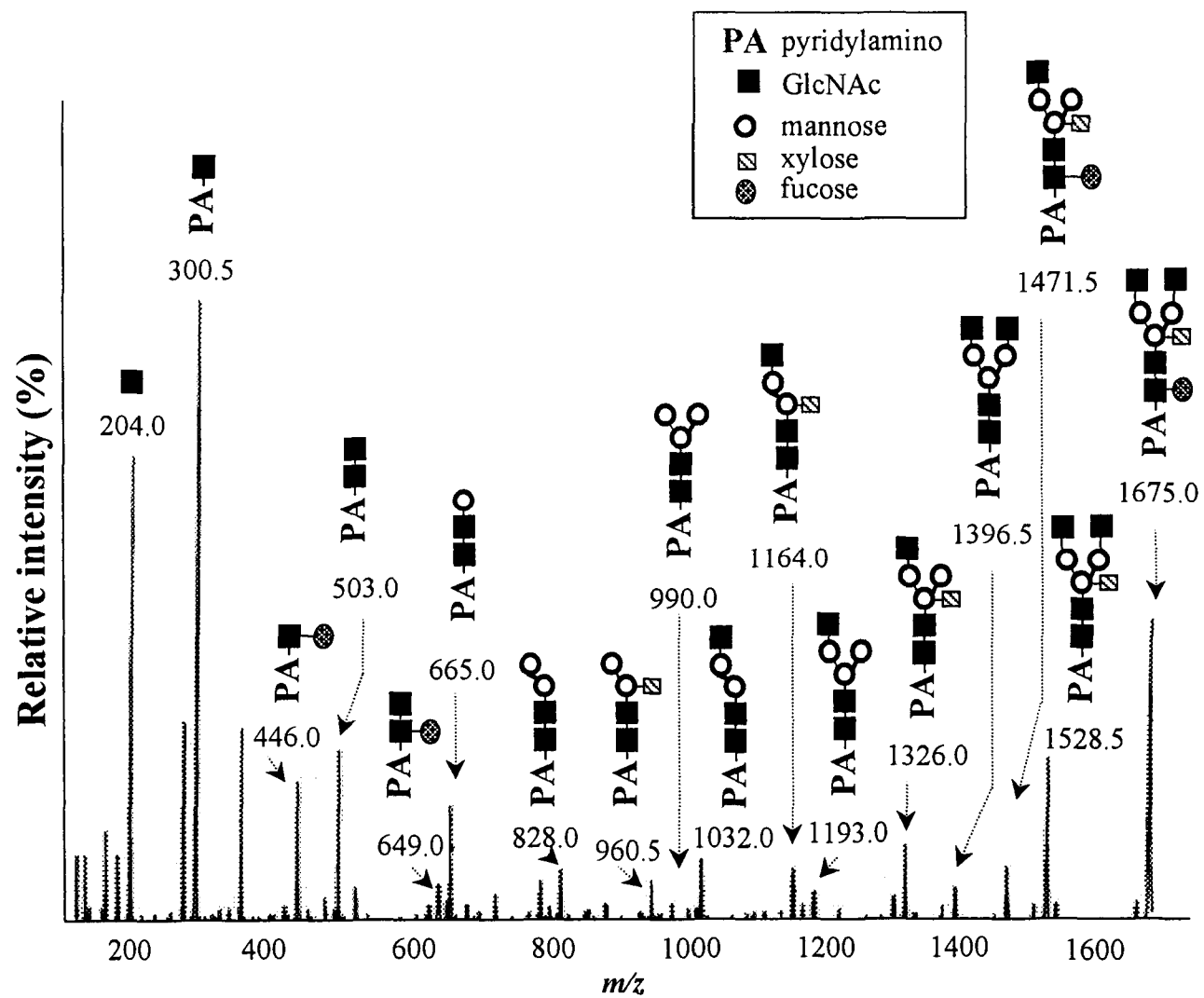
Fig. 8. MS/MS spectrum of PA-sugar chain F-II ( m/z 1675.0).
