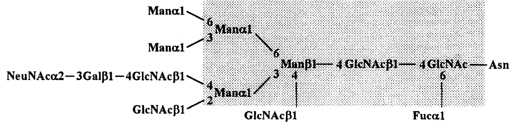
Fig. 2. Sub-groups of N -linked sugar chains. The structure within the shaded box is the trimannosyl core common to all N -linked glycans. (A) Representatives from mammalian glycoproteins; (B) representatives from plant glycoproteins.
