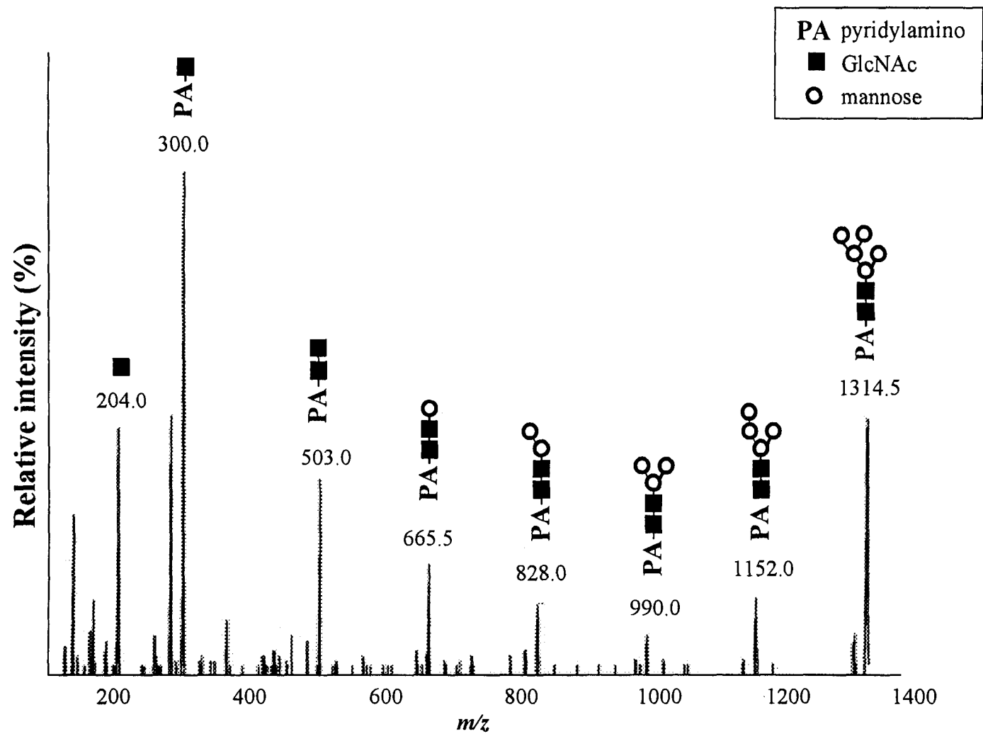
Fig.11. MS/MS spectrum of PA-sugar chain F-IV-b ( m/z 1314.0).
