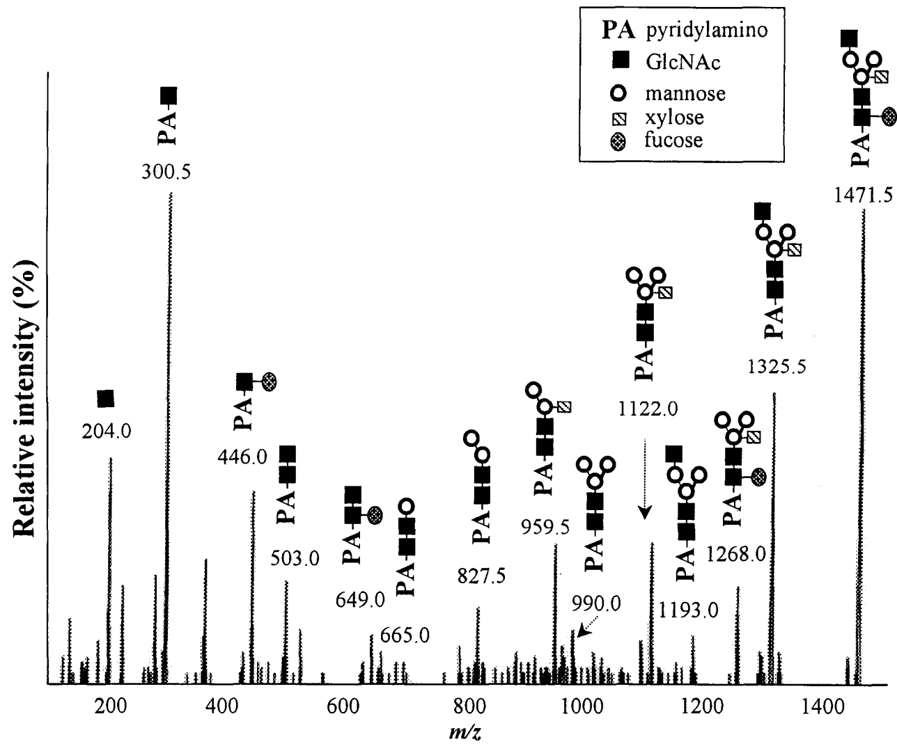
Fig. 9. MS/MS spectrum of PA-sugar chain F-III ( m/z 1471.5).
