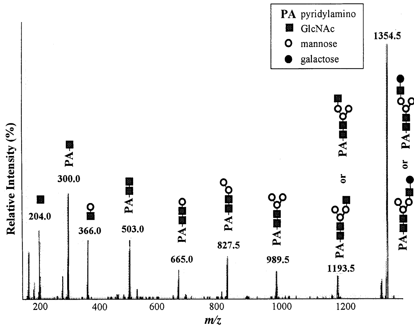
Fig. 18. MS/MS spectrum of PA-sugar chain -K-2 ( m/z 1354.5).
