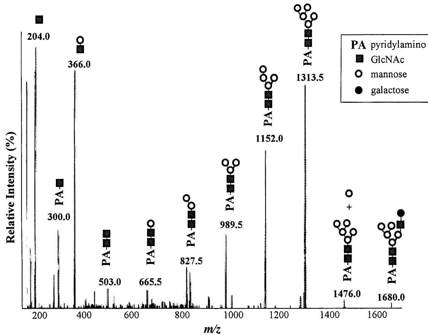
Fig. 22. MS/MS spectrum of PA-sugar chain -L ( m/z 1680.0).
