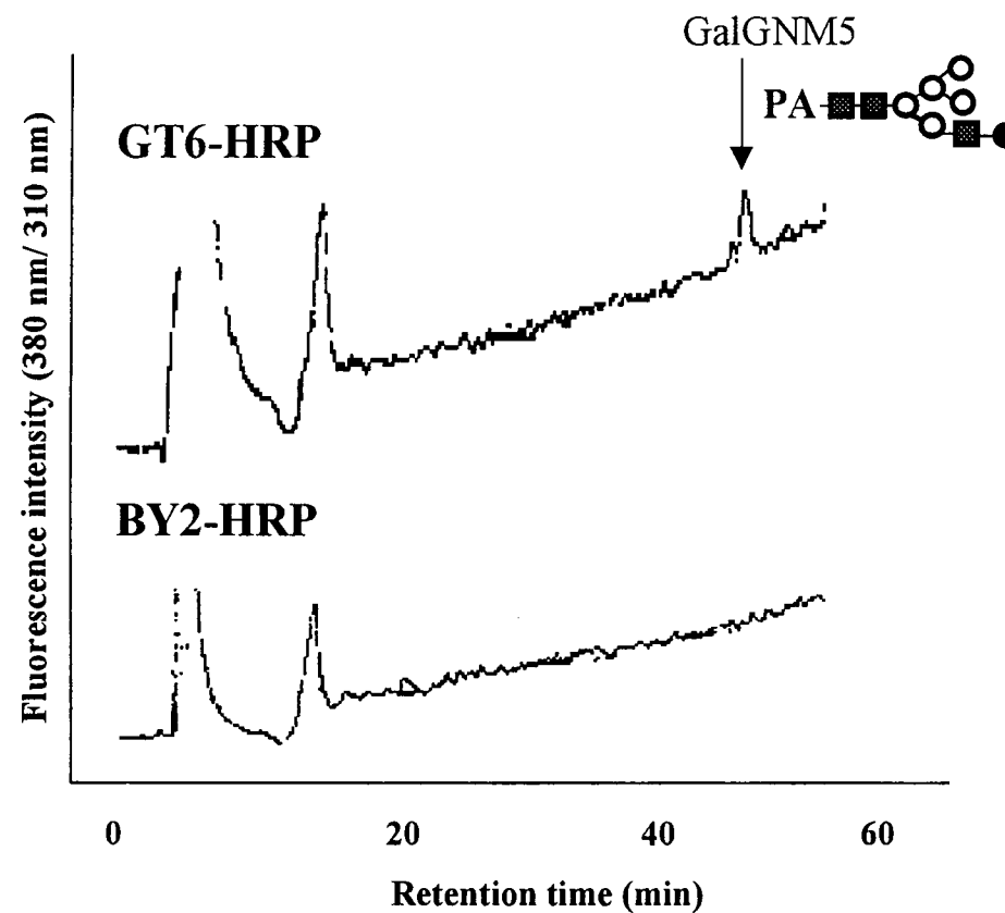
Fig. 29. Reversed-phase HPLC of PA-sugar chains from purified HRP after RCA 120 affinity chromatography. PA-sugar chains were eluted from Cosmosil 5C18-P column (6 x 250 mm) by increasing the acetonitrile concentration in 0.02% TFA linearly from 0 to 15% for 60 min at a flow rate of 1.2 ml/min. Excitation and emission wavelengths were 310 nm and 380 nm, respectively. Only one major peak was observed from GT6-HRP. The PA-labeled sample corresponded to the expected elution position of Gal 1 GlcNAc 1 Man 5 GlcNAc 2 (GalGNM5).
