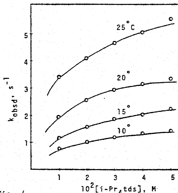
Fig. 4 Plots of k_{obsd} against [i-Pr_4tds] ; [Ag(i-Pr_2dte)]_6 = 5.0 \times 10^{-4} M .
