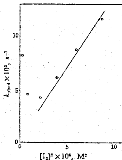
Fig. 5. Plots of the apparent rate constant against the square of the \text{I}_2 concentrations; \text{Me}_2\text{Sn}(\text{dtc})_2 5.1 \times 10^{-5} \text{ M} .
