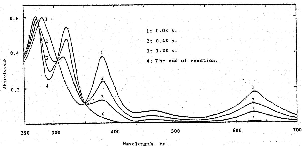
Fig. 1. Rapid scanning spectra of the reaction of [\text{Au}(n\text{-Bu}_2\text{dtc})]_2 ( 2.11 \times 10^{-4} M) with \text{I}_2 ( 2.08 \times 10^{-4} M) in \text{CH}_2\text{Cl}_2 at 25^\circ\text{C} ; scanning speed = 150 nm/5 ms, cell length = 0.2 cm.
