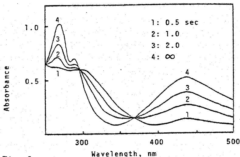
Fig. 1 Spectral changes after mixing of [\text{Cu}(\text{Et}_2\text{dtc})]_4 ( 5.1 \times 10^{-5} \text{ M} ) with \text{Et}_4\text{tds} ( 1.0 \times 10^{-4} \text{ M} ) in \text{CH}_2\text{Cl}_2 at 25^\circ\text{C} .
