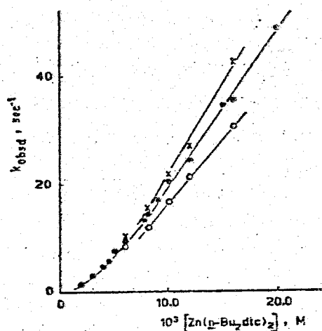
Figure 2. Plots of k_{\text{obsd}} (360 nm) against [\text{Zn}(n\text{-Bu}_2\text{dte})_2] ; \circ 15 °C, \bullet 25 °C, and \times 35 °C.
