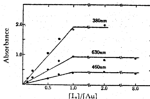
Fig. 2. Mole ratio study of [\text{Au}(n\text{-Bu}_2\text{dtc})]_2\text{-I}_2 system in \text{CH}_2\text{Cl}_2 at -50^\circ\text{C} ; [\text{Au}(n\text{-Bu}_2\text{dtc})]_2 = 5.0 \times 10^{-5} \text{ M} .
