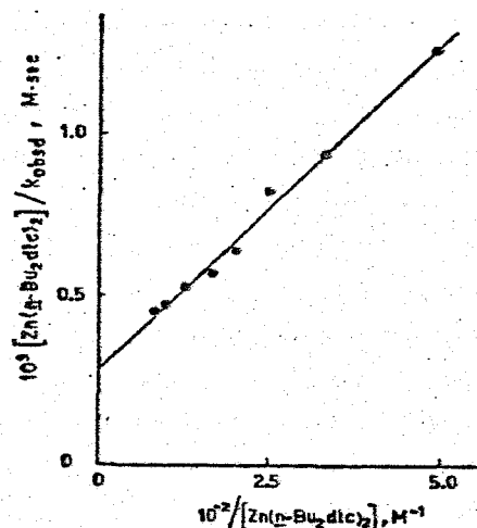
Figure 3. Plots of [Zn(n-Bu_2dtc)_2]/k_{obsd} against 1/[Zn(n-Bu_2dtc)_2] for the reaction of I_2 with excess Zn(n-Bu_2dtc)_2 at 25^\circ C ; [I_2] = 1.0 \times 10^{-4} M .
