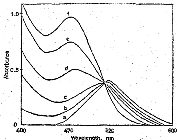
Fig. 2. Absorption spectra of \text{I}_2 in cyclohexane ( 8.0 \times 10^{-4} \text{ M} ) containing varying amounts of \text{Et}_4\text{tds} : (a) 0, (b) 8.0 \times 10^{-4} , (c) 1.6 \times 10^{-3} , (d) 4.0 \times 10^{-3} , (e) 8.0 \times 10^{-3} , (f) 1.6 \times 10^{-2} \text{ M} ( 25^\circ\text{C} ).
