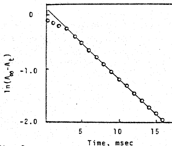
Fig. 2 Plots of \ln(A_\infty - A_t) against time at 25^\circ\text{C} ; [\text{Cu}(\text{Et}_2\text{dtc})]_4 = 1.0 \times 10^{-4} \text{ M} , [\text{Et}_4\text{tds}] = 1.0 \times 10^{-2} \text{ M} .
