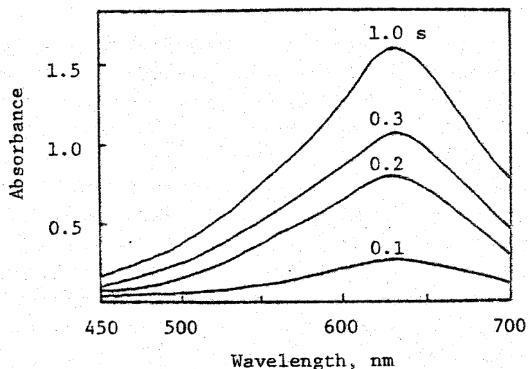
Fig. 3 Spectral changes after mixing of [\text{Ag}(i\text{-Pr}_2\text{dtc})]_6 ( 5.0 \times 10^{-4} M) with i\text{-Pr}_4\text{tds} ( 5.0 \times 10^{-2} M) in \text{CH}_2\text{Cl}_2 at 25^\circ\text{C} .
