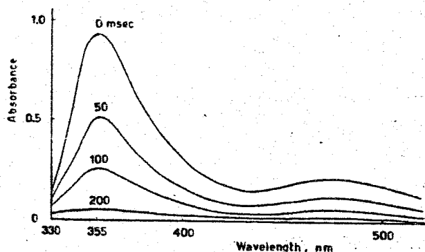
Figure 1. The decay of the electronic spectrum after mixing I_2 ( 3.00 \times 10^{-4} M ) with excess Zn(n-Bu_2dtc)_2 ( 1.00 \times 10^{-2} M ) in cyclohexane; scanning speed = 150 nm/5 msec, cell length = 1.0 cm.
