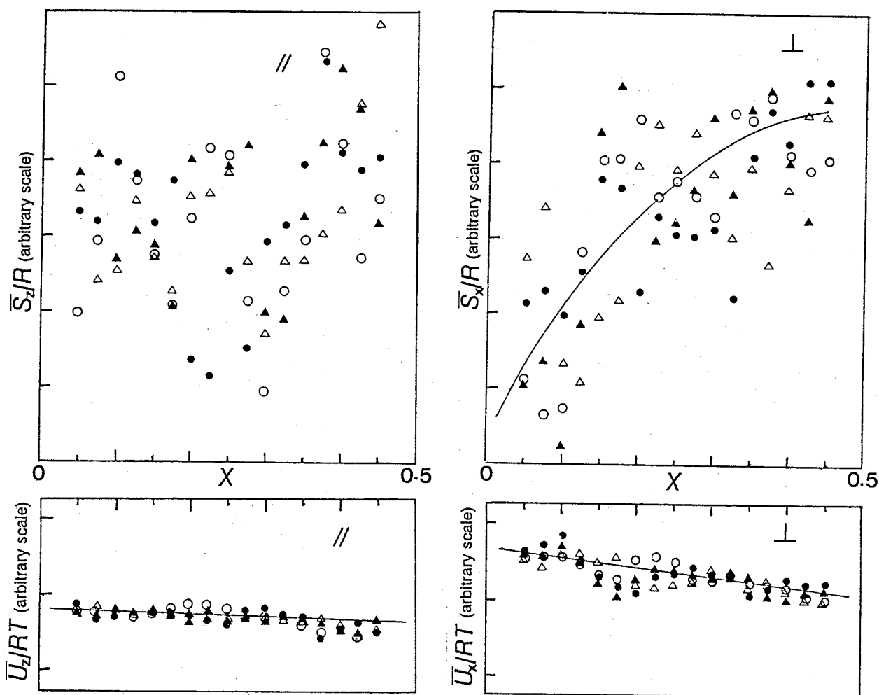
Fig.4.9d Calculated partial molar entropy (top) and partial molar internal energy function (bottom) at various X based on the \mathbf{s} // \mathbf{Z} lattice (left) and \mathbf{s} \perp \mathbf{Z} one (right) of the Model B'. Meaning of marks are same in Fig.4.8d.
