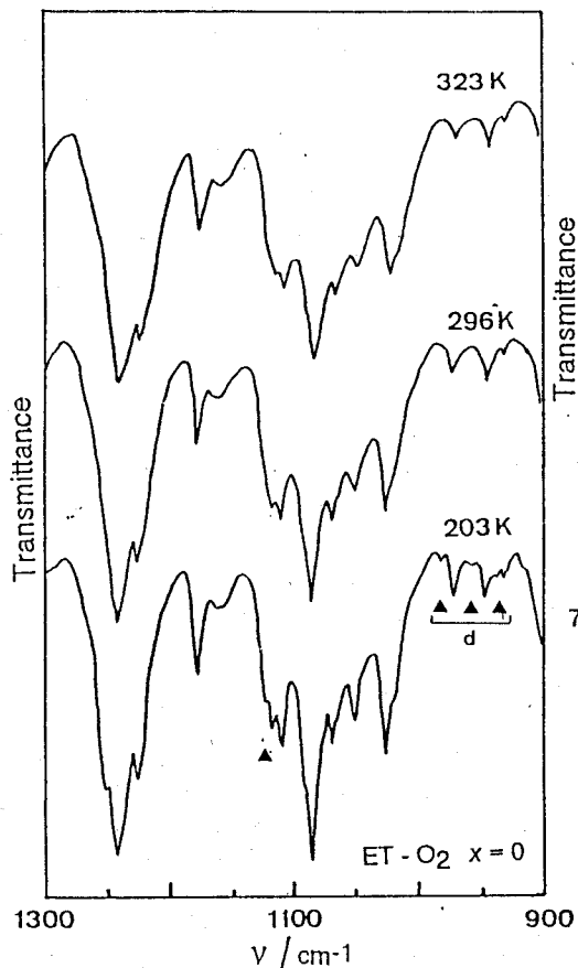
Fig.5.17a Infrared spectra ( 350\text{-}700\text{cm}^{-1} and 900\text{-}1300\text{cm}^{-1} ) of the ET-O 2 system with x=0 at 203K, 296K and 323K. Triangles on the spectra at 323K and 203K indicate the peaks with shapes significantly different from the one at 296K. The peaks with "o" marks are also observed in the spectra of the ME-O 2 system with x=0.45 , and those with "d" marks showed isotope shift in the ME-O 2 system with x=0.45 .
