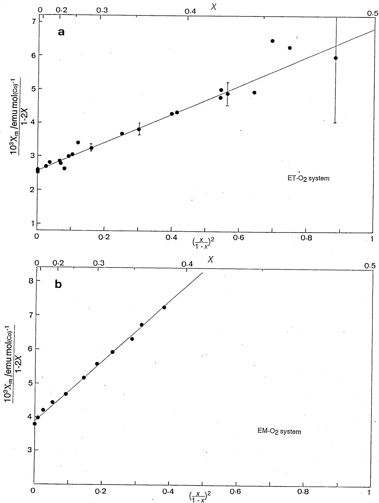
Fig.5.13 Plots of molar magnetic susceptibility of paramagnetic cobalt ions vs. \{x/(1-x)\}^2 ; a, ET-O 2 system at (288.8 \pm 2.0) K; and b, EM-O 2 system at (286.7 \pm 0.7) K. Solid lines indicate the value calculated by eq.5.1 with parameters in Table 5.4.
