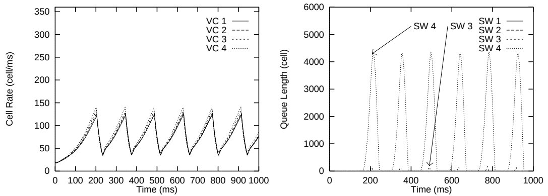
Figure 5.32: WAN Case for RIF = 1/1024 and RDF = 1/64 (Scheme 3).
