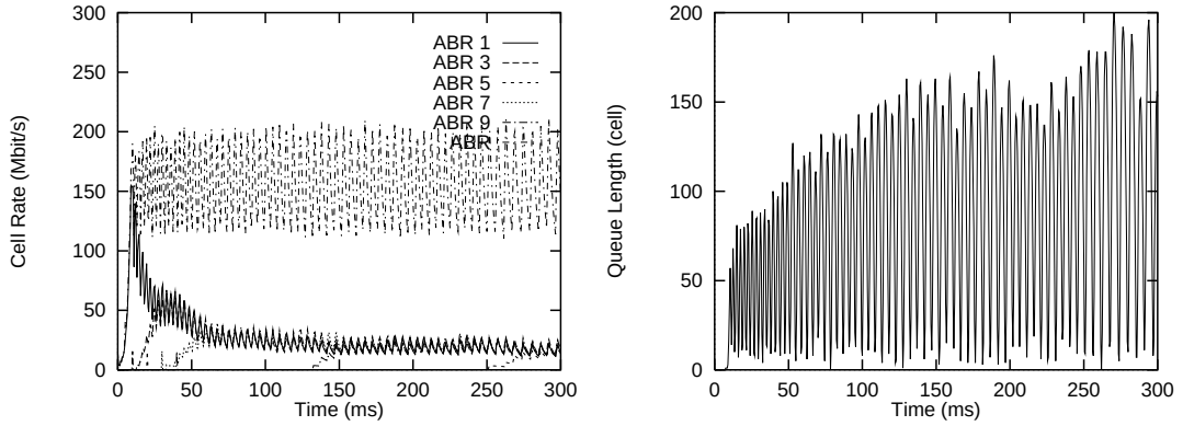
Figure 3.2: EPRCA with an EFCI Switch ( N_{VC} = 10 , \tau = 0.01 ).
