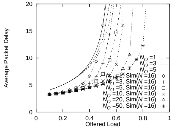
Figure 2.15: Average Packet Delay vs. Offered Load for \overline{BL} = 3 .
