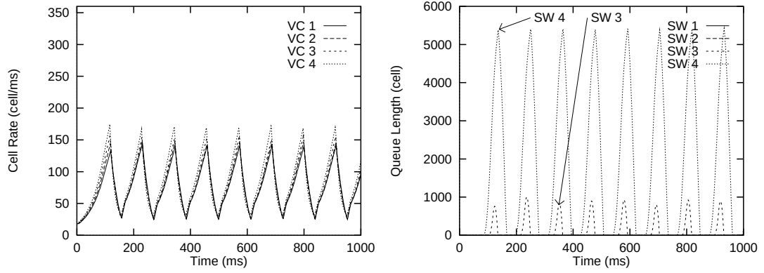
Figure 5.31: WAN Case for RIF = 1/512 and RDF = 1/64 (Schemes 1 and 2).
