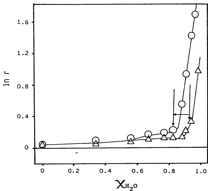
Fig. 6. The relationship between the mole fraction of water in water-dioxane mixture ( X_{H_2O} ) and the \ln r value of the competitive acylation in the presence ( \circ ) or the absence ( \Delta ) of CTAB.
