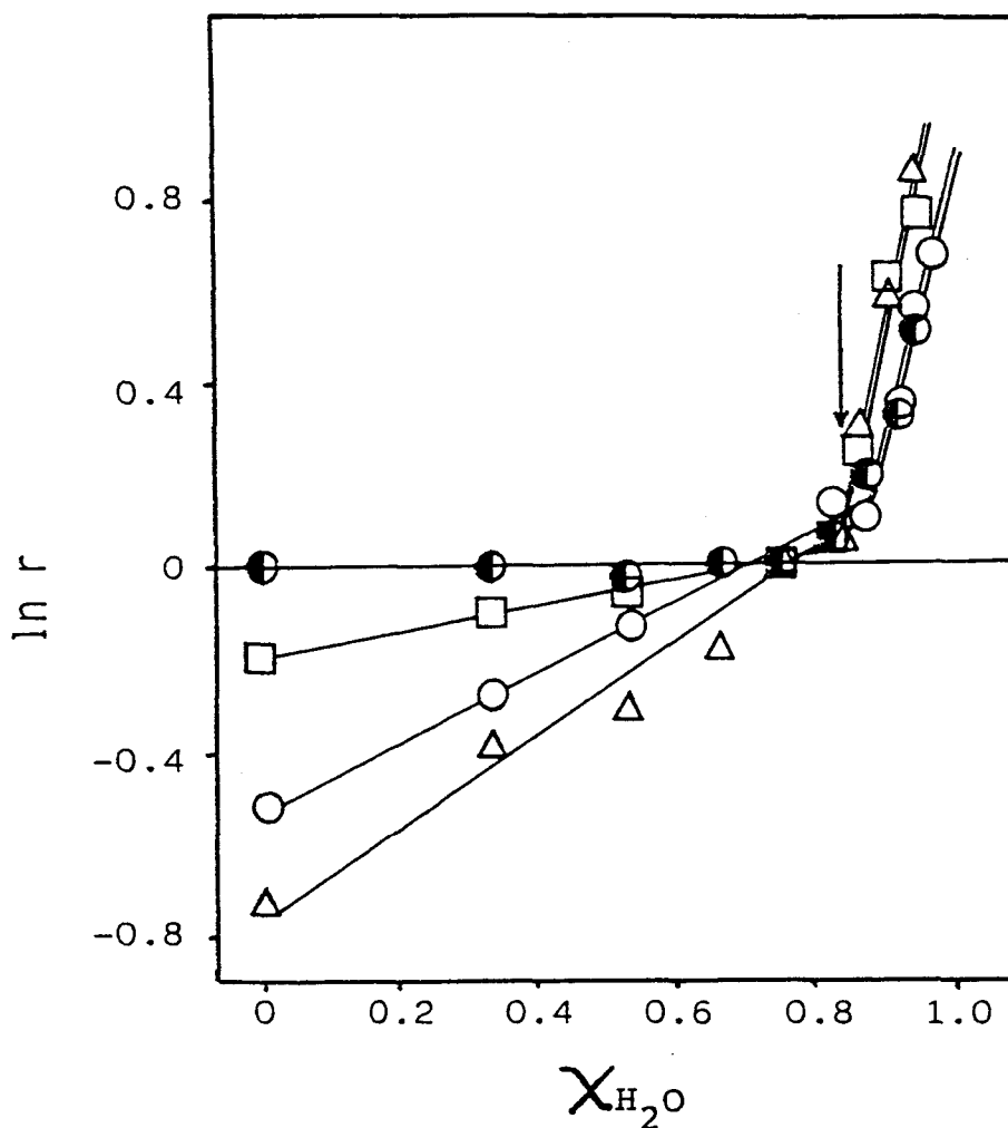
Fig. 7(a). The relationship between the mole fraction of water in water-dioxane mixture ( \chi_{H_2O} ) and the \ln r value of the competitive acylation with isovaleric anhydride. Benzylamine ( \Delta ), phenethylamine ( \circ ), 3-phenylpropylamine ( \square ), and pentylamine ( \bullet ) were employed as R^1-NH_2 . Butylamine was employed as R^2-NH_2 in every case. The concentration of a reagent was 50 mM.
