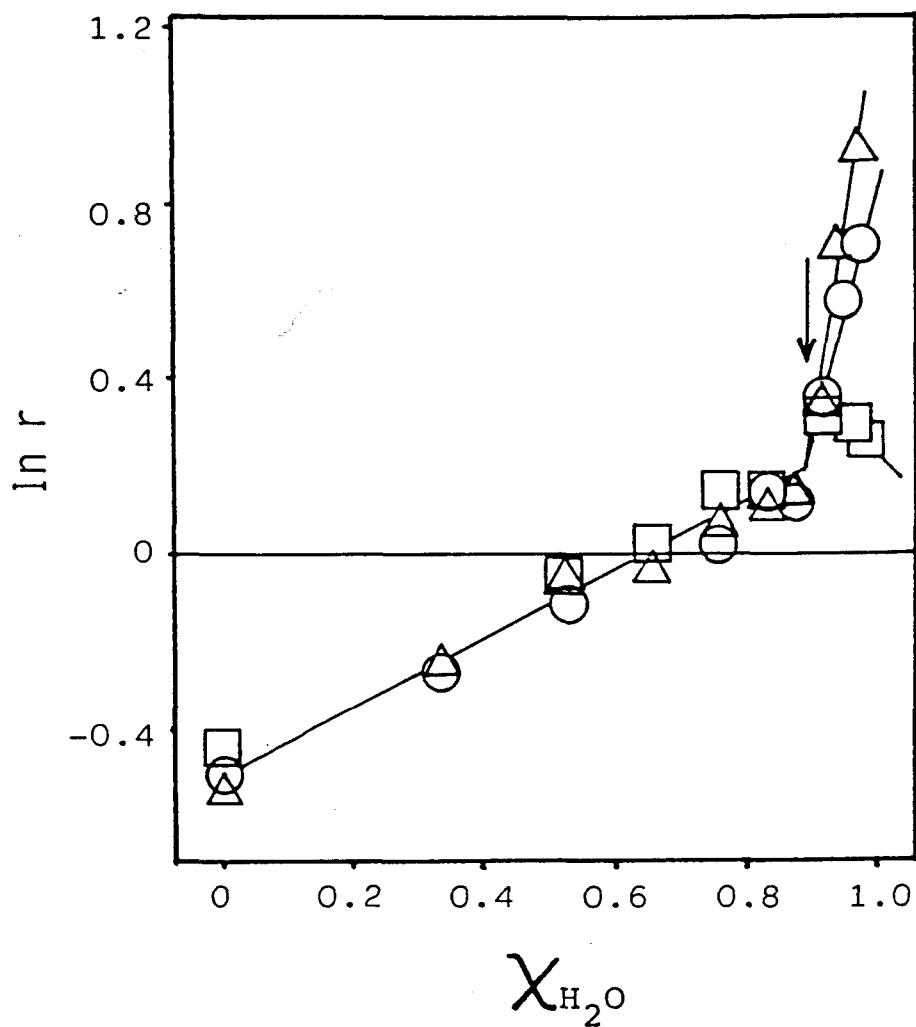
Fig. 7(b). The relationship between the mole fraction of water in water-dioxane mixture ( X_{H_2O} ) and the \ln r value of the competitive acylation with isovaleric anhydride. Phenethylamine was employed as R^1-NH_2 . As R^2-NH_2 , propylamine ( \Delta ), butylamine ( \circ ), and hexylamine ( \square ) were employed. The concentration of a reagent was 6.25 mM.
