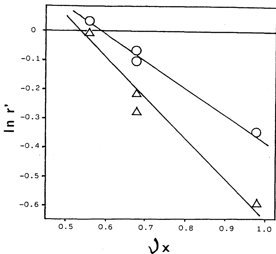
Fig. 18. The relationship between the \ln r' value and v_x value of carbon chains in the substrates. The reaction was carried out in dioxane (O) or benzene ( \Delta ).
