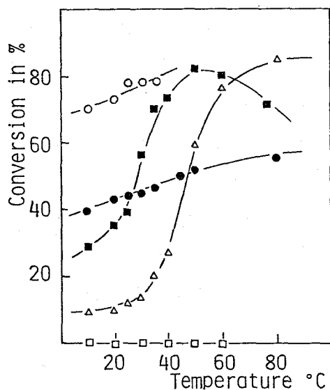
Figure II-21, Effect of temperature on the polycondensation of 5u ; relationship between the conversion and the temperature. ( \Delta ):cyclohexane; ( \blacksquare ): carbon tetrachloride; ( \bullet ):benzene; ( \circ ):diethyl ether; ( \square ):methanol, DMF, DMSO; [ 5u ]=20mmole/l, [Triethylamine]=20mmole/l; reaction time 24h
