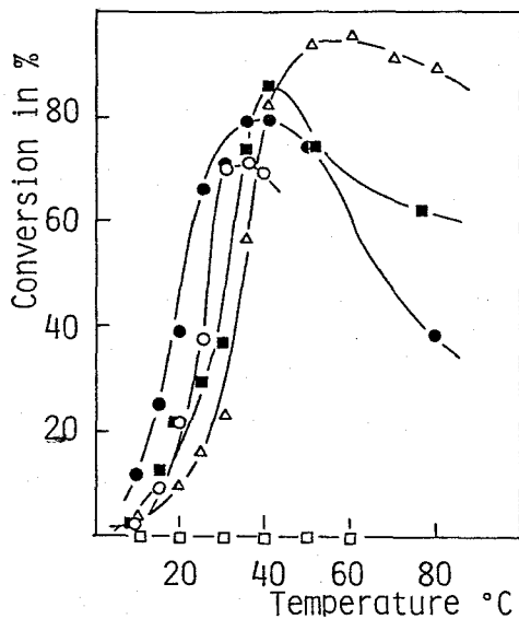
Figure II-9, Effect of temperature on the polycondensation of 5i ; relationship between the conversion and the temperature. ( \Delta ):cyclohexane; ( \blacksquare ): carbon tetrachloride; ( \bullet ):benzene; ( \circ ):diethyl ether; ( \square ):methanol, DMF, DMSO; [5i]=20\text{mmole/l} , [\text{Triethylamine}]=20\text{mmole/l} ; reaction time 24h
