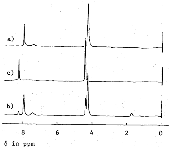
Figure IV-1 1 H NMR spectra of poly(glycyglycine) obtained from 19a in carbon tetrachloride at 30°C (measured in trifluoroacetic acid). a) Water insoluble part, b) Chloroform insoluble part, c) Authentic 2,5-piperazinedione.
