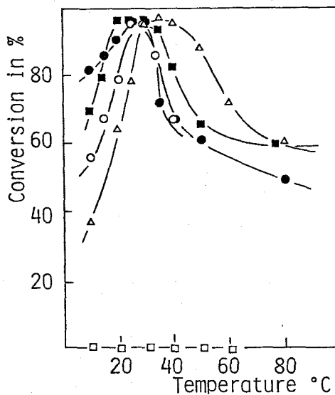
Figure II-6, Effect of temperature on the polycondensation of 5f; relationship between the conversion and the temperature. ( \Delta ):cyclohexane; ( \blacksquare ): carbon tetrachloride; ( \bullet ):benzene; ( \circ ):diethyl ether; ( \square ):methanol, DMF, DMSO; [5f]=20mmole/l, [Triethylamine]=20mmole/l; reaction time 24h
