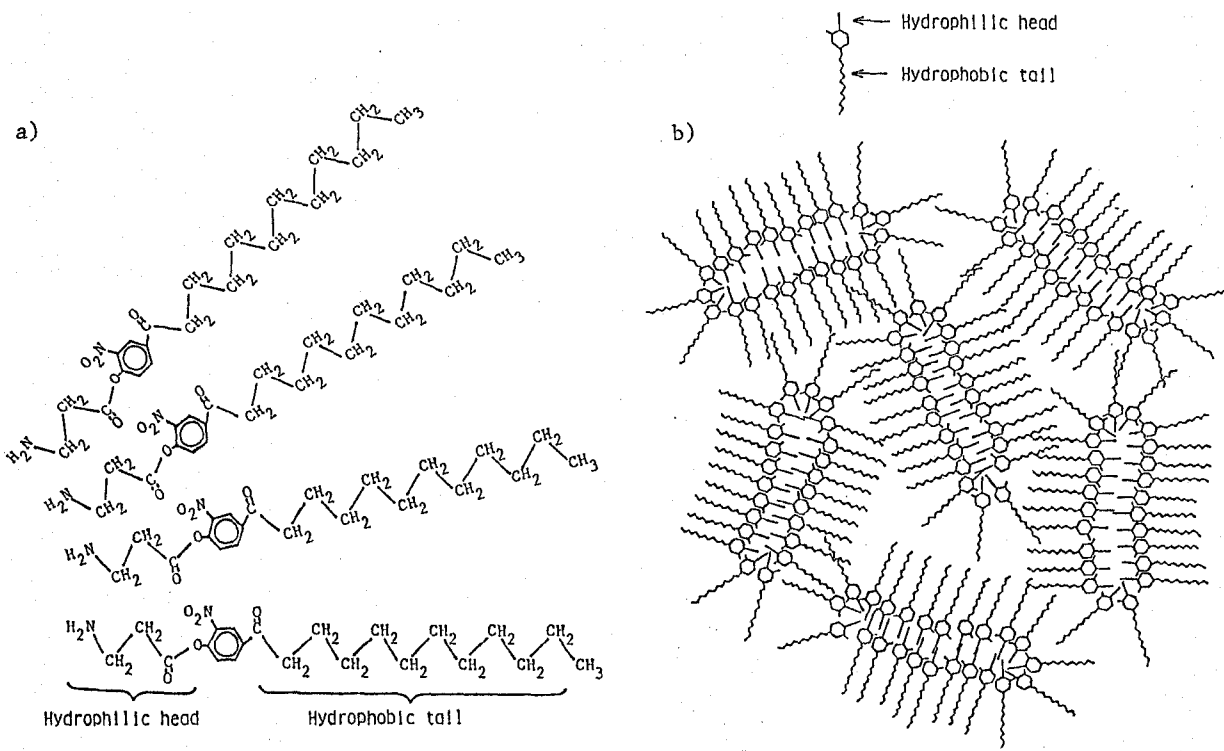
Figure II-22 Schematic illustration of polycondensation field formed by reversed micellar surface a) Microscopic presentation b) Macroscopic presentation
