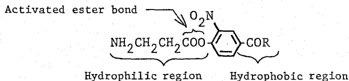
\beta -Alanine 4-Acyl-2-nitrophenyl Ester
