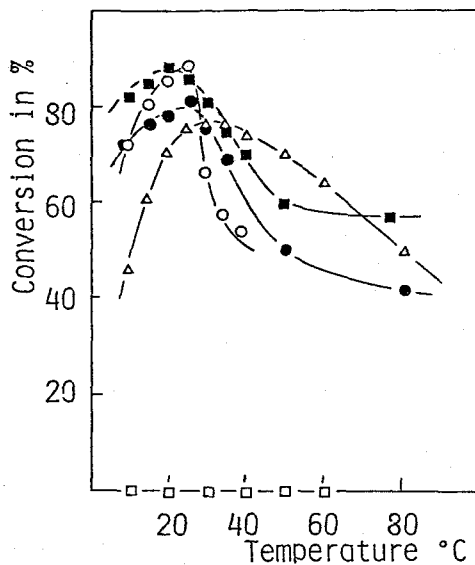
Figure II-5, Effect of temperature on the polycondensation of 5e; relationship between the conversion and the temperature. ( \Delta ):cyclohexane; ( \blacksquare ): carbon tetrachloride; ( \bullet ):benzene; ( \circ ):diethyl ether; ( \square ):methanol, DMF, DMSO; [5e]=20mmole/l, [Triethylamine]=20mmole/l; reaction time 24h
