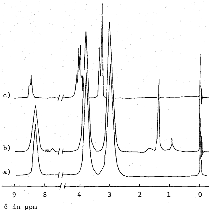
Figure IV-4. ^1\text{H} NMR spectra for poly( \beta -alanine) from the polycondensation of 22b in carbon tetrachloride at 30^\circ\text{C} (measured in trifluoroacetic acid).
