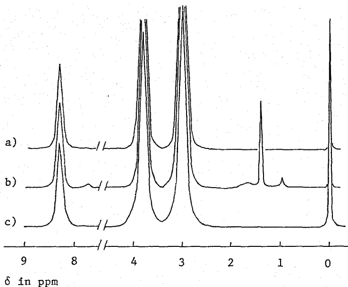
Figure II-23. ^1\text{H} NMR spectra for poly( \beta -alanine) from the polycondensation of 5g in diethyl ether at 30^\circ\text{C} (measured in trifluoroacetic acid).
