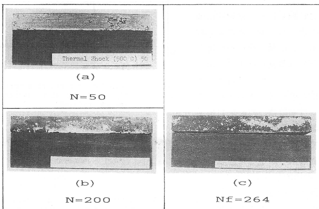
Fig. 5-19 Deformation of copper explosive clad steel after thermal cycling (500°C) [(a), (b), (c) longitudinal side]
