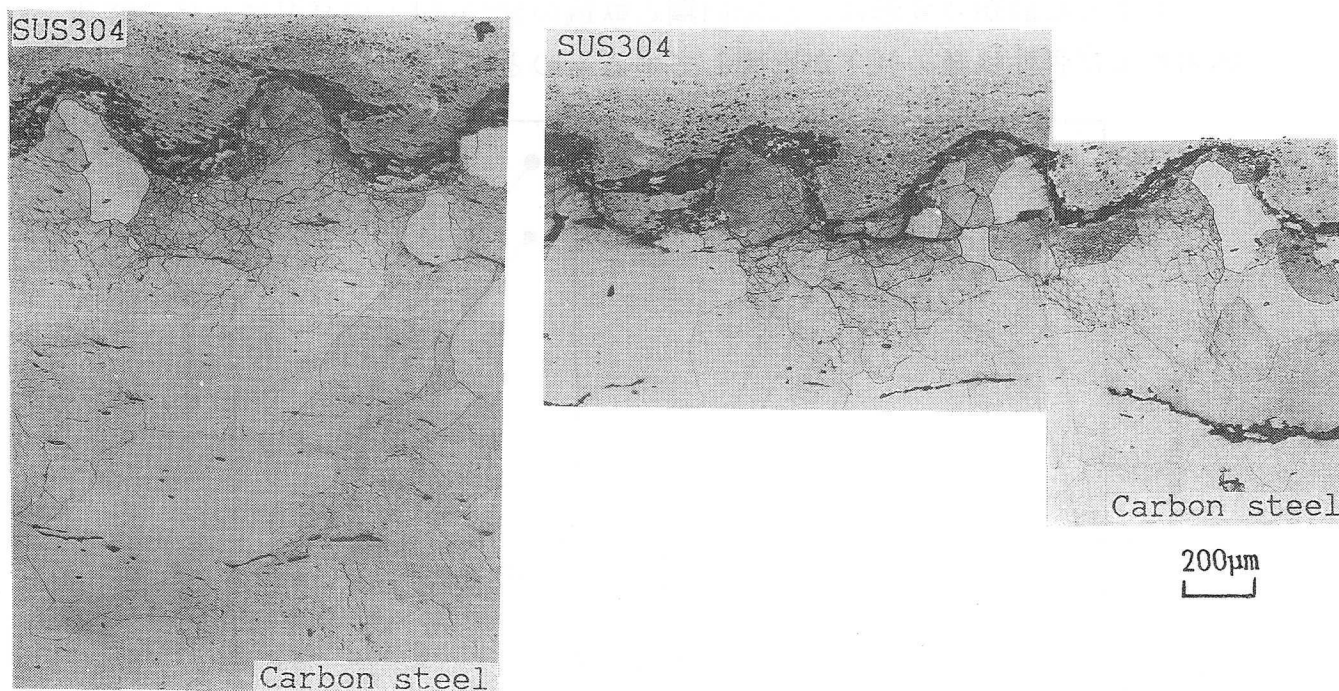
Fig. 5-29 Microstructures of SUS304 explosive clad steel after 200 thermal cycles(700℃)
