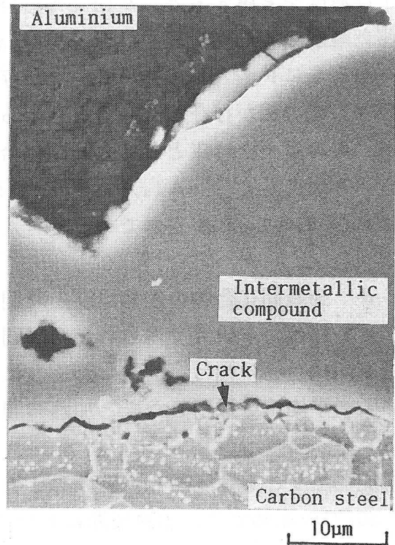
Fig. 3-15 Current photograph of diffusion band (exposed 10hr at 600^{\circ}\text{C} )
