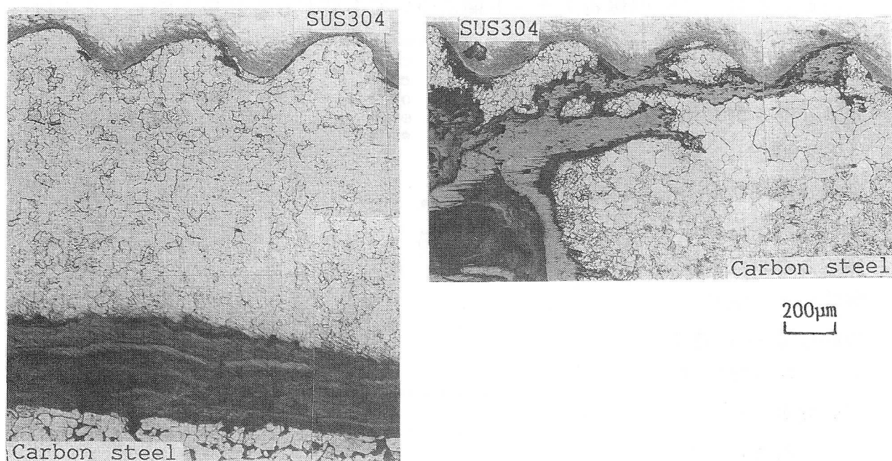
Fig. 5-28 Microstructures of SUS304 explosive clad steel after 2000 thermal cycles(500℃)
