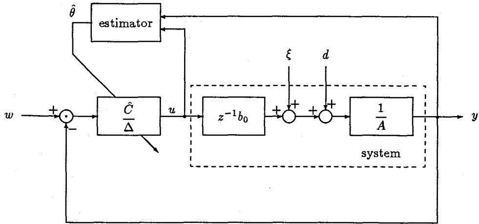
Fig.4.1 Block diagram of the proposed self-tuning PID control system based on pole-assignment method.
