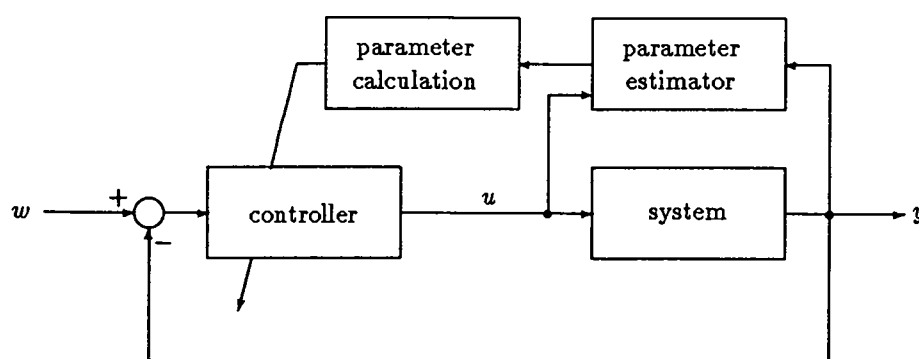
Fig.1.1 Block diagram of the usual self-tuning control system.
