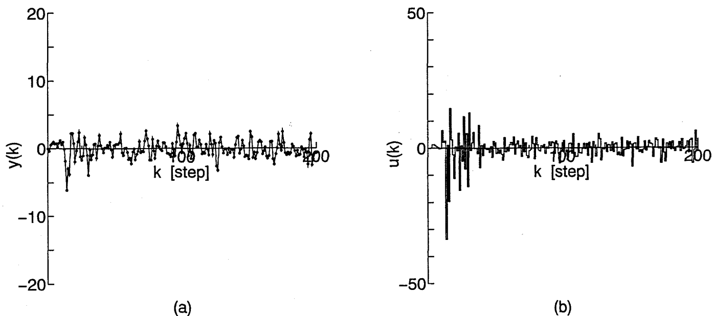
Fig.3.2 Simulation results using the pole-assignment control algorithm with the term of -\hat{p}_0 \cdot \hat{C}(z^{-1})\eta(k) where (a) and (b) show output y(k) and input u(k) .
