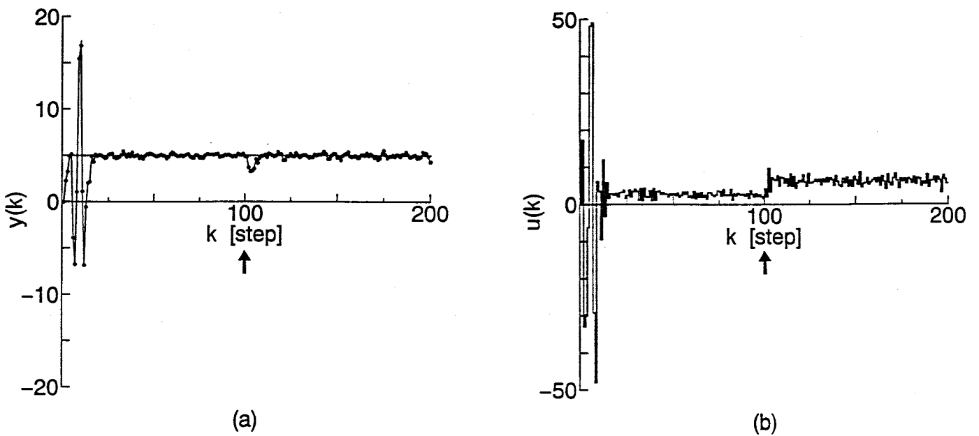
Fig.2.6 Simulation results in the case where d(k) changes at 100[step], using the proposed least squares algorithm of (2.3.3)-(2.3.9).
