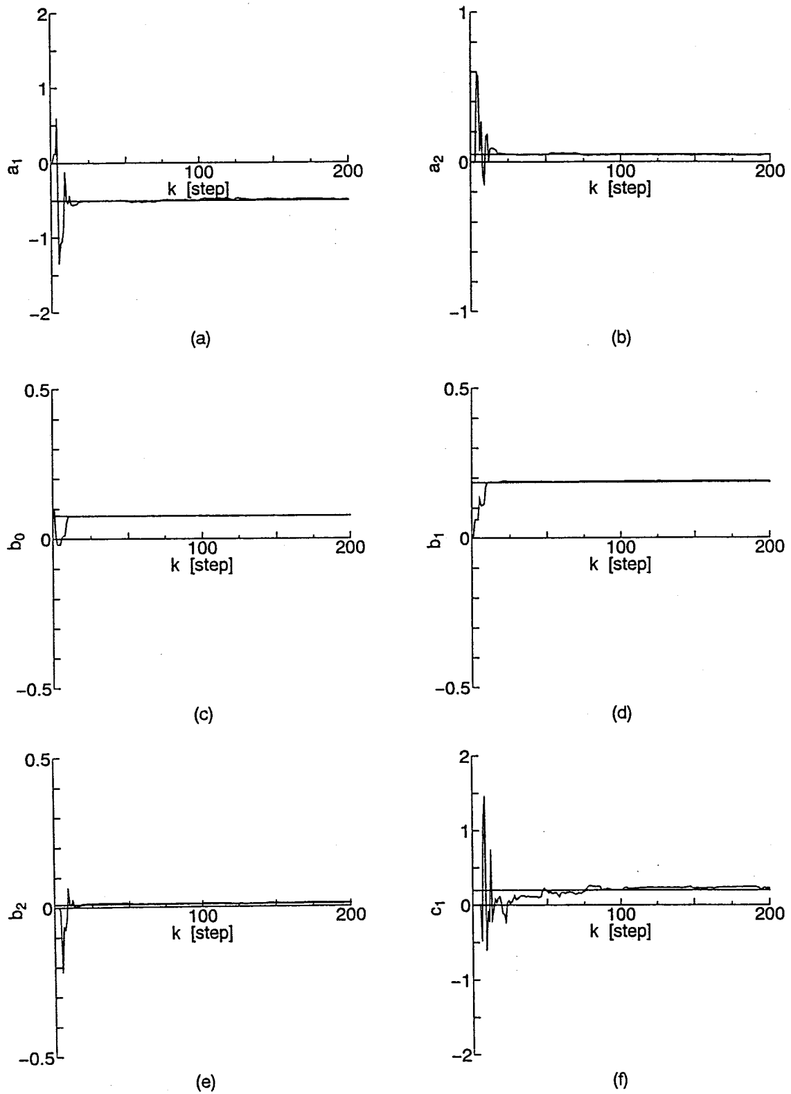
Fig.3.5 Identified parameters using the least squares algorithm of (3.2.25)-(3.2.30).
