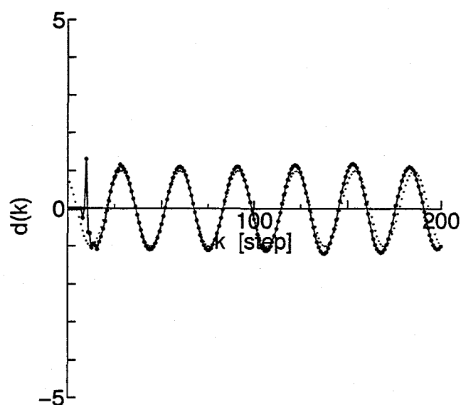
Fig.2.4 The calculated result of a deterministic disturbance \hat{d}(k) using (2.3.10).
