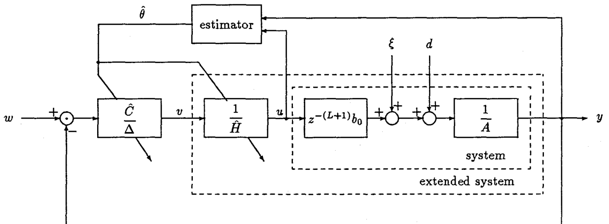
Fig.4.5 Block diagram of the proposed self-tunign PID control system with pre-compensator.
