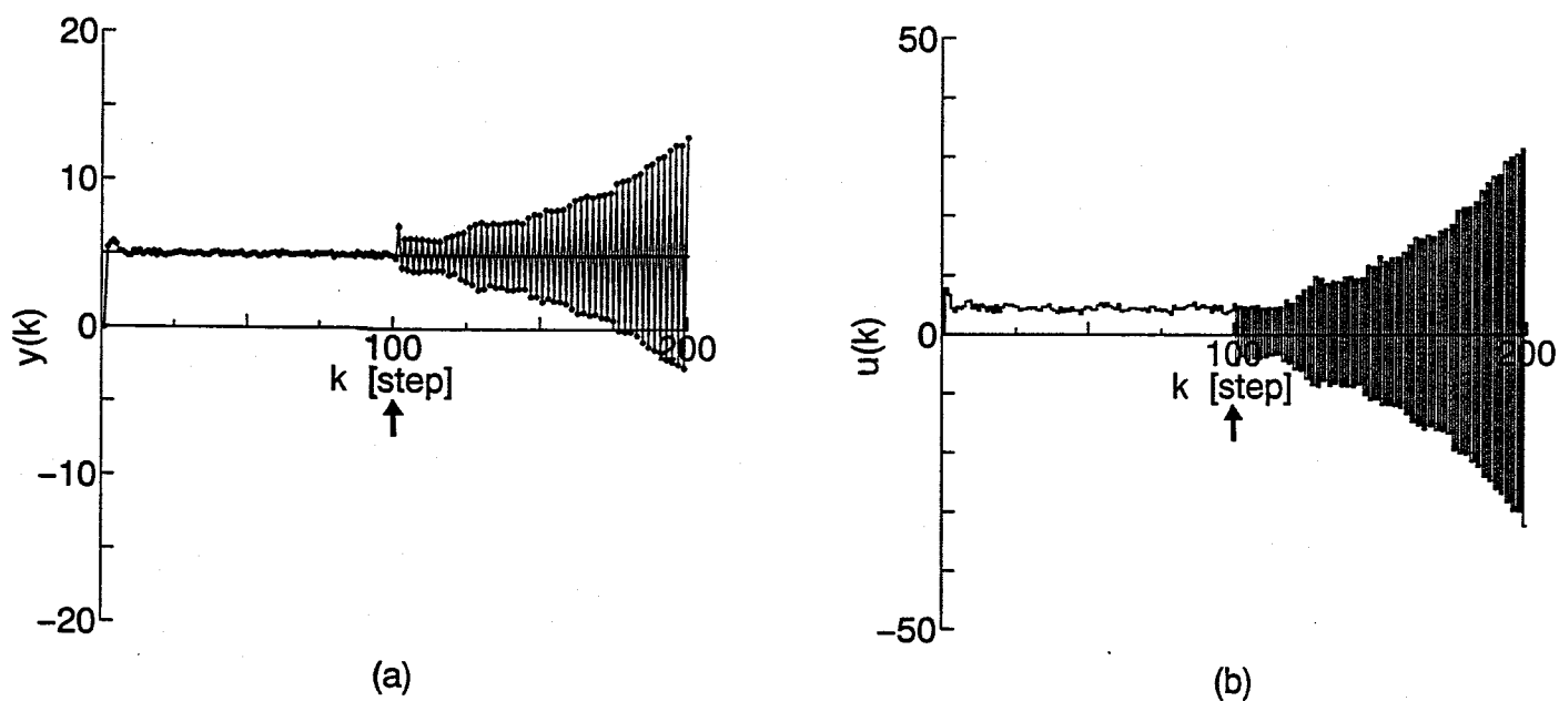
Fig.4.2 Simulation results using the PID control with fixed PID gains where (a) and (b) show output y(k) and input u(k) .
