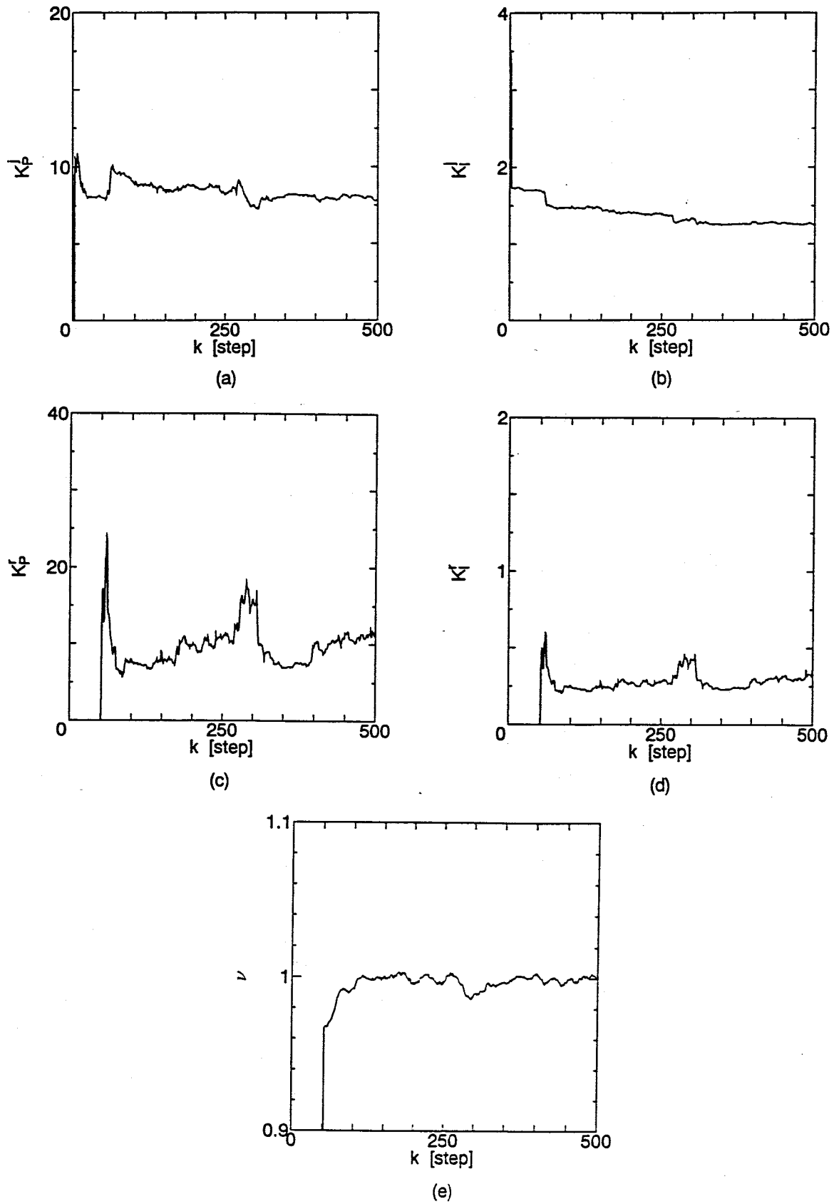
Fig.4.20 Identified PID gains and \hat{v}(k) .
