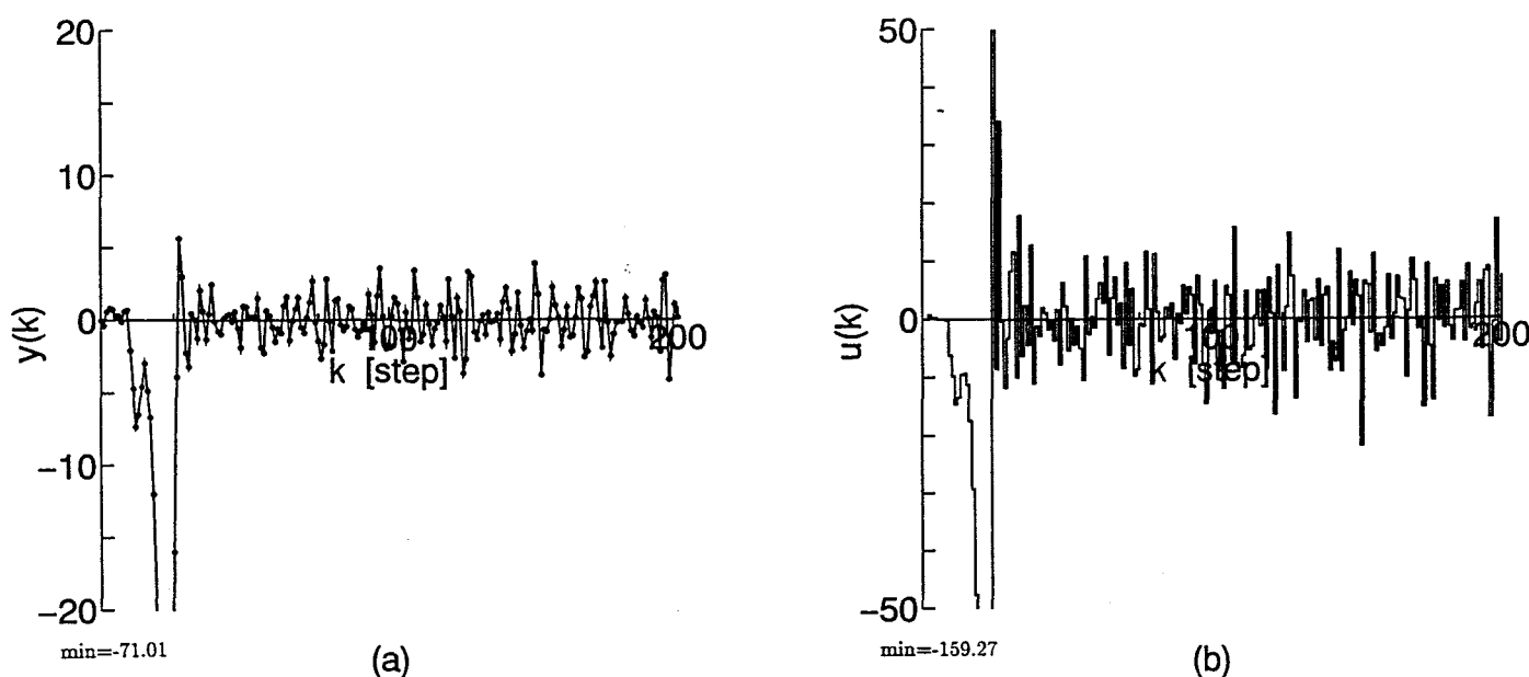
Fig.3.3 Simulation results using the pole-assignment control algorithm without the term of -\hat{p}_0 \cdot \hat{C}(z^{-1})\eta(k) where (a) and (b) show output y(k) and input u(k) .
