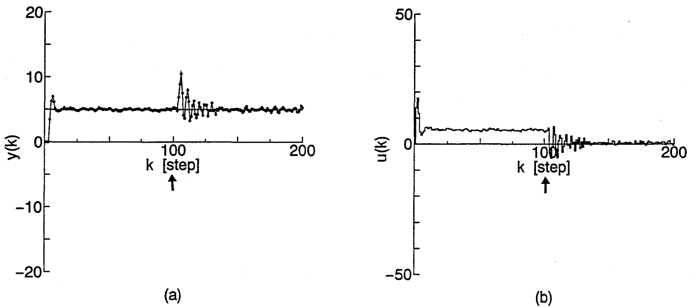
Fig.4.10 Simulation results for the time-varying system using the self-tuning PID control algorithm with Smith-type time-lag compensator where (a) and (b) show output y(k) and input u(k) .
