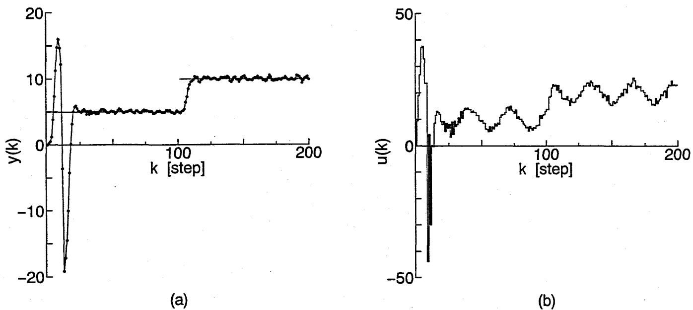
Fig.2.2 Simulation results using the proposed self-tuning pole-assignment control algorithm of (2.3.14) where (a) and (b) show output y(k) and input u(k) .
