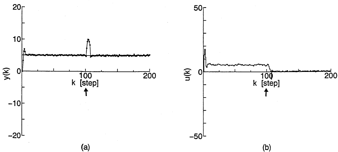
Fig.4.3 Simulation results for the time-varying system using the proposed self-tuning PID control algorithm where (a) and (b) show output y(k) and input u(k) .
