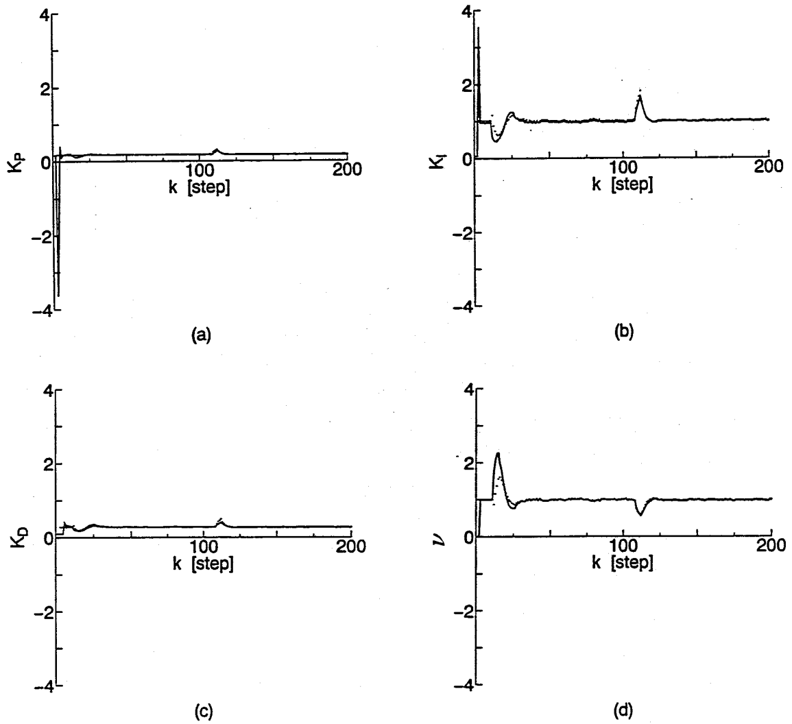
Fig.4.13 Identified PID gains and \hat{v}(k) for Fig.4.12.
