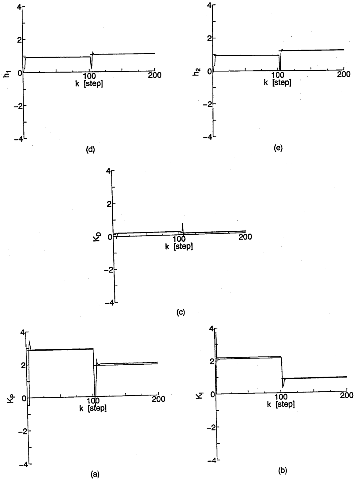
Fig.4.9 Identified PID gains and parameters of pre-compensator for Fig.4.8
