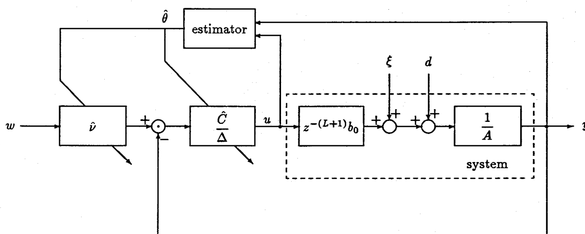
Fig.4.11 Block diagram of the proposed self-tuning controller based on predictive model.
