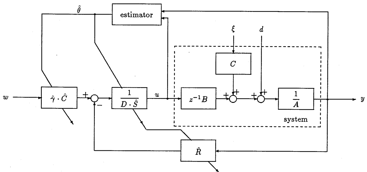
Fig.2.1 Block diagram of the proposed self-tuning pole-assignment control system.
