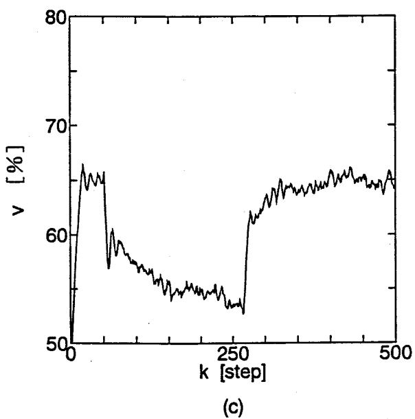
Fig.4.18 Simulation results by using the usual PID control method with fixed PID gains of (4.5.14) and (4.5.15).
