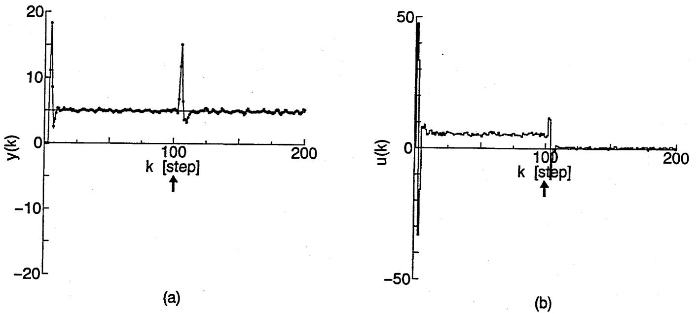
Fig.4.8 Simulation results for the time-varying system using the self-tuning PID control algorithm with pre-compensator where (a) and (b) show output y(k) and input u(k) .
