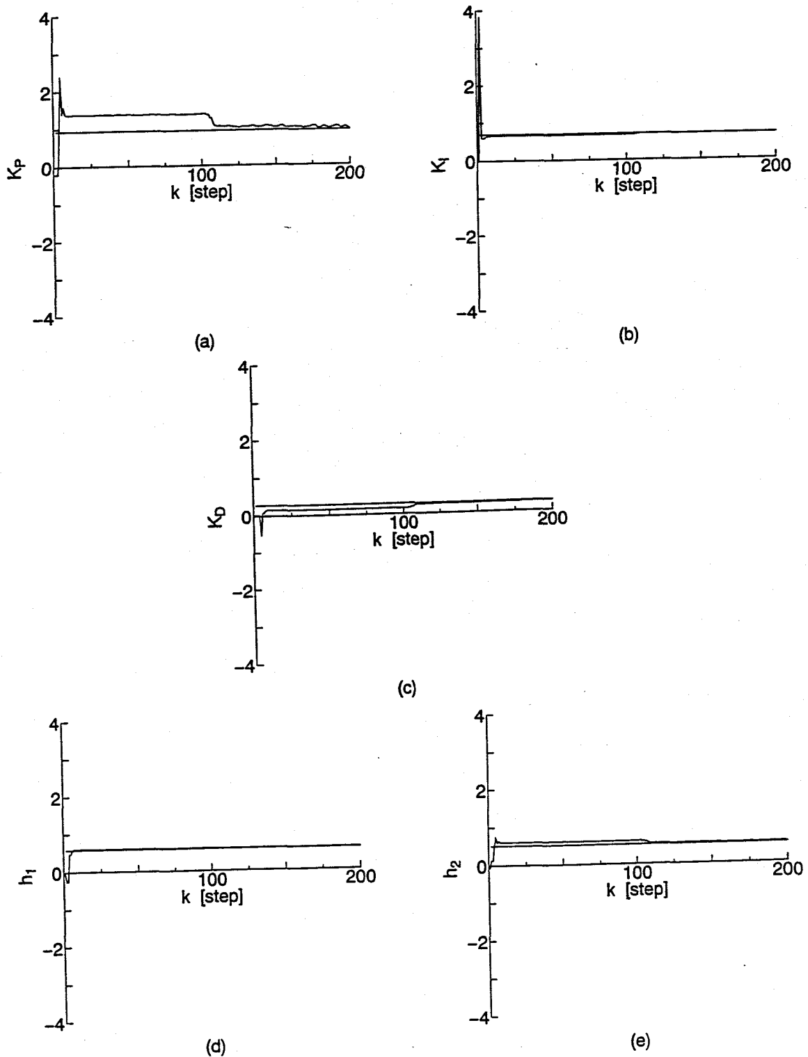
Fig.4.7 Identified PID gains and parameters of pre-compensator for Fig.4.6.
