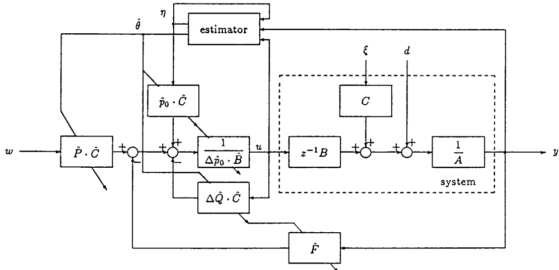
Fig.3.1 Block diagram of the proposed pole-assignment control system with minimum variance property.
