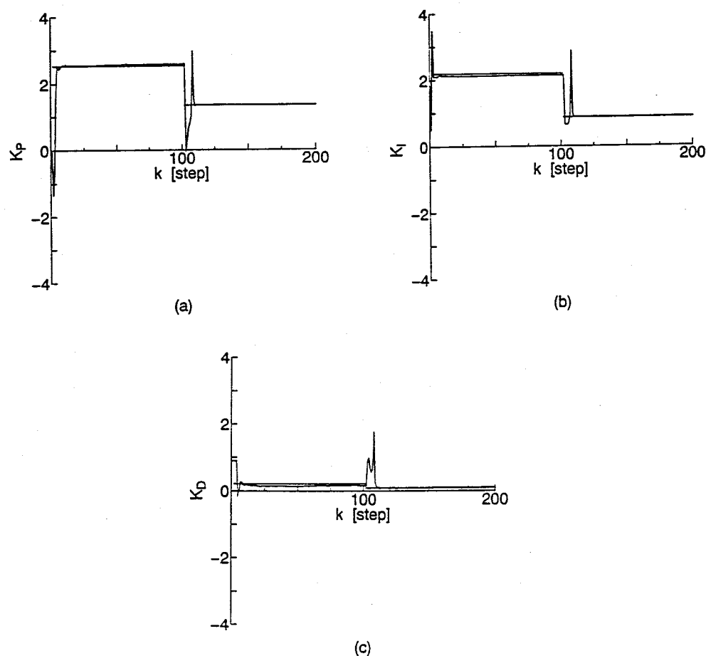
Fig.4.4 Identified PID gains for Fig.4.3.
