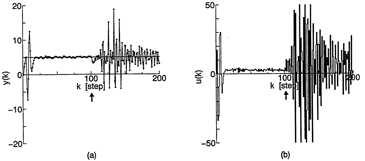
Fig.2.5 Simulation results in the case where d(k) changes at 100[step], using the usual least squares algorithm of (2.3.20)-(2.3.25).
