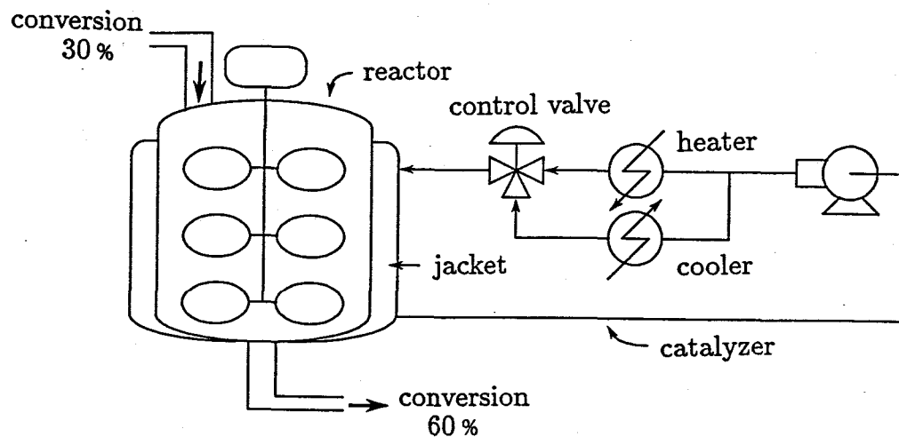
Fig.4.15 The schematic figure of the polystyrene reactor.
