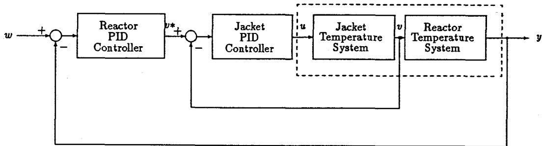
Fig.4.17 The schematic diagram of the control system.
