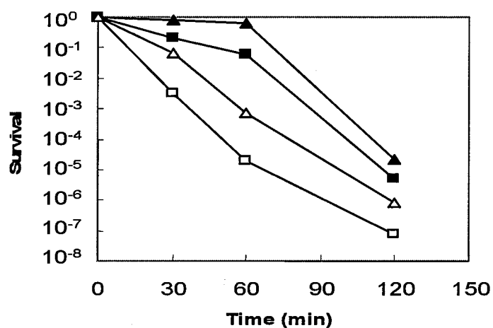
FIG. 4.4 Timecourse of survival of Lb. casei cells in the simulated gastrointestinal conditions.
