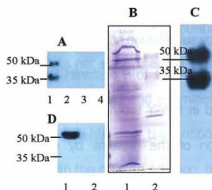
FIG. 3.3 Expression, purification, and binding of CPHM produced in P. pastoris . (A) Western blot of CPHM expressed in P. pastoris . Lane 1, supernatant of GS115/pPIaCPHM; lane 2, supernatant
