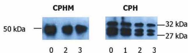
FIG. 3.5 Stable binding of CPHM and CPH to cells of Lb. casei . Cells bound to CPH or CPHM were incubated in PBS buffer at 4°C. The samples were taken at the time (h) indicated in the figure and were analyzed for the amount of the bound protein by western blotting using the anti-histidine tag antibody. The dissociation rate constant ( k_{off} ), estimated as described in materials and methods, was 2 \times 10^{-5} \text{ s}^{-1} for CPHM, and 7 \times 10^{-5} \text{ s}^{-1} for CPH.
