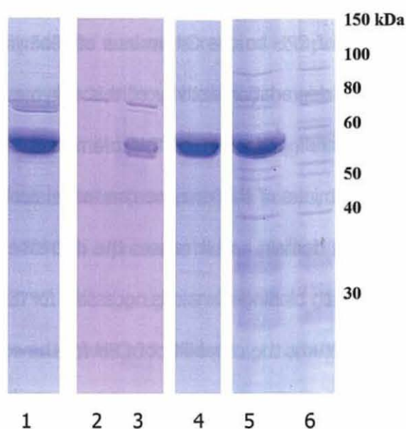
FIG. 4.2 Purification of CPH-SBD, its binding to starch, and to Lb. casei cells. Lane 1, nickel chelate column purified protein preparation; lane 2, supernatant after starch binding assay; lane 3, control without starch; lane 4, ion exchange chromatography purified CPH-SBD; lane 5, cells
