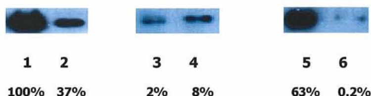
FIG. 2.3 Binding of CPH-AMY to LAB strains. Lane 1, Lc. lactis ATCC 19435; lane 2, Lb. plantarum NRRL B-531; lane 3, Lc. lactis IL 1403; lane 4, Lb. casei NRRL B-441; lane 5, Lb. delbrueckii ATCC 9649; lane 6, Lb. casei NRRL B-445. The estimated number of bound molecules of CPH-AMY to one cell of Lc. Lactis ATCC 19435 is 1 \times 10^3 which was considered as 100% and the relative percentages for other cells were shown in the figure. No signal was detected for the cells incubated with citrate buffer or free \alpha -amylase.
