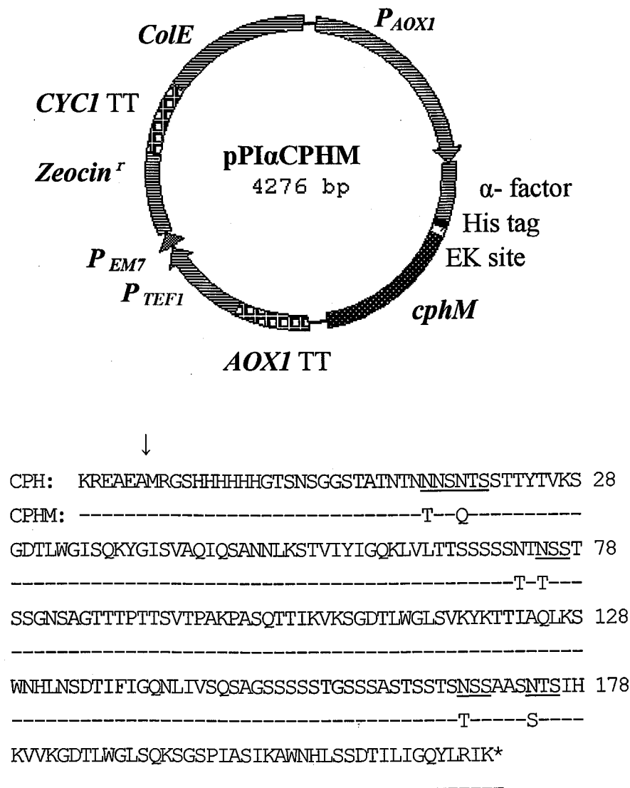
FIG 3.1 Structure of pPIaCPHM and amino acid sequences of CPHM and CPH.
