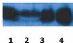
FIG. 3.4 Binding of CPHM produced in P. pastoris to cells. CPHM bound to cells was detected using the anti-histidine tag antibody and no signal was detected for the cells incubated with elution buffer instead of CPHM. Lane 1, B. subtilis 168; lane 2, E. coli XL1-Blue; lane 3, Lb. casei B-441; lane 4, S.cerevsiae IFO0216.
