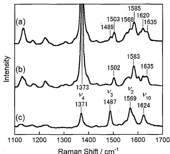
Figure 4-5. Resonance Raman spectra of ferric P450cams in 1100–1700 \text{cm}^{-1} region in 50 mM potassium phosphate buffer (pH 7.4) containing 1 mM d -camphor (except (b)) and 100 mM KCl at room temperature; (a) rP450cam(2) spectrum in the presence of 1 mM d -camphor and 100 mM KCl, (b) camphor-free wild-type P450cam spectrum, and (c) camphor-bound wild-type P450cam spectrum. The excitation wavelength was 413.1 nm and the laser power was 3 mW.
