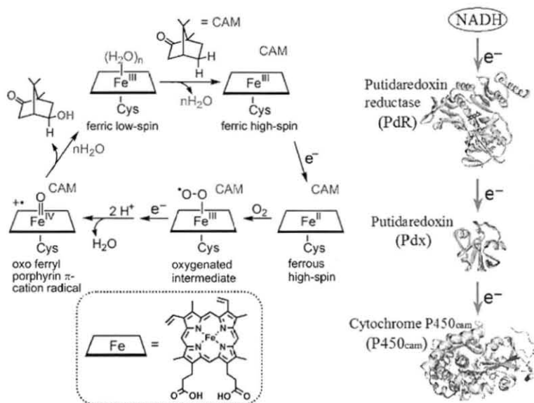
Figure 9. Catalytic cycle of d -camphor hydroxylation by P450cam.
