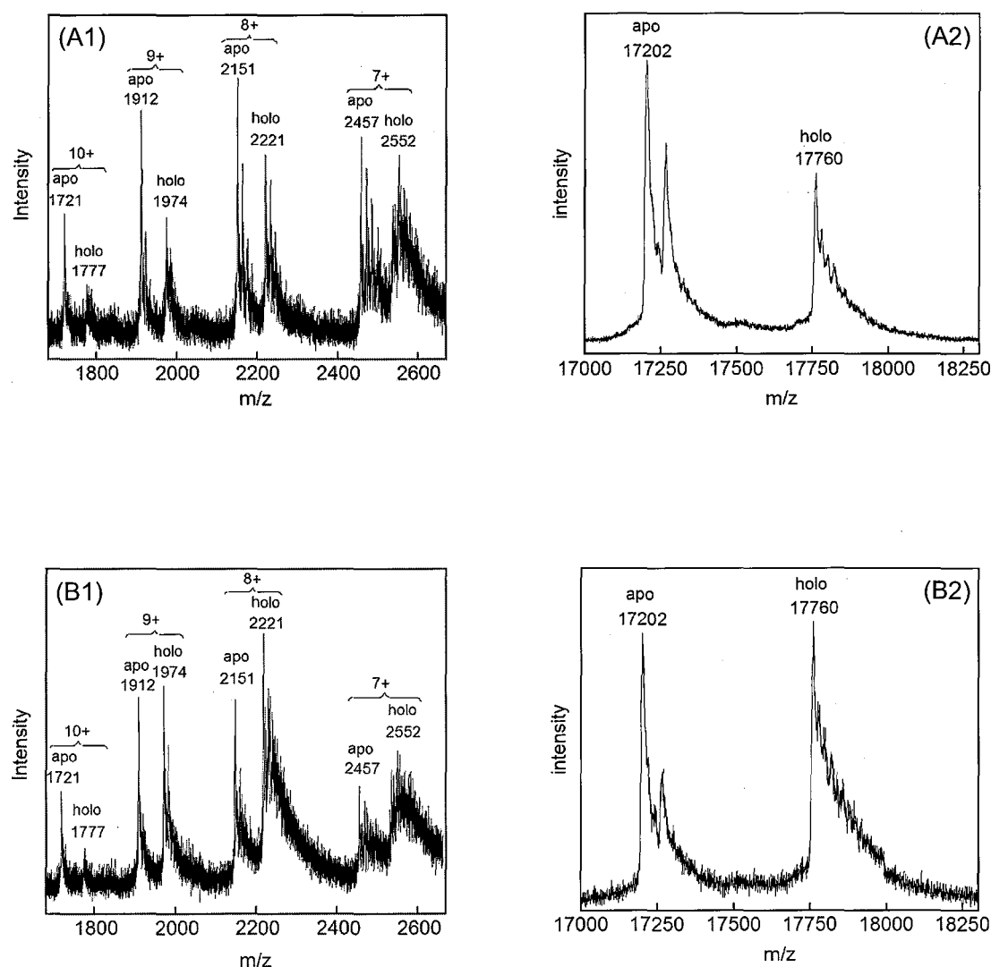
Figure 1-1. ESI-TOF mass spectra of met-rMb in 10 mM ammonium acetate buffer containing 50% methanol and 0.1% formic acid. (A1) rMb(1), (B1) rMb(2), deconvoluted mass spectra of met-rMb (A2) rMb(1), (B2) rMb(2). The nozzle potential was 160 V for rMb(1) and 90 V for rMb(2).
