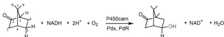
Scheme 1. Hydroxylation of d -camphor catalyzed by cytochrome P450cam.
