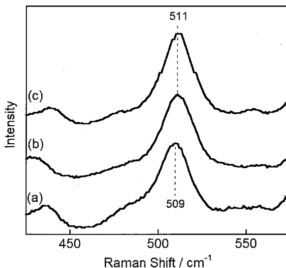
Figure 2-16. Resonance Raman spectra of CO-myoglobins in the 425\text{--}575\text{ cm}^{-1} region in 100 mM potassium phosphate buffer (pH 7.0) at room temperature: (a) rMb(1), (b) rMb(2), (c) rMb(3). The excitation wavelength was 413.1 nm and a laser power was 10 mW.
