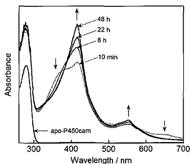
Figure 3-2. UV-vis spectral changes at various time during the reconstitution reaction in 0.1 M His buffer (pH 8.0) containing 20% glycerol (v/v), 0.4 mM d -camphor, and 20 mM DTT at room temperature in a glove box (O 2 < 1 ppm).
