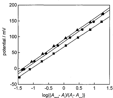
Figure 2-5. Nernst plot obtained from the spectral changes at 433 nm of rMb(1) ( \blacktriangle ), rMb(2) ( \bullet ), and rMb(3) ( \blacksquare ).
