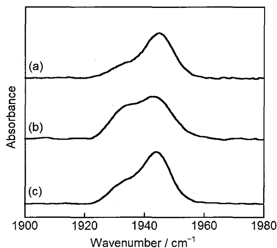
Figure 2-17. IR spectra of CO-bound myoglobins in the 1900\text{--}1980\text{ cm}^{-1} region in 100 mM potassium phosphate buffer (pH 7.0) at room temperature: (a) rMb(1), (b) rMb(2), and (c) rMb(3).
