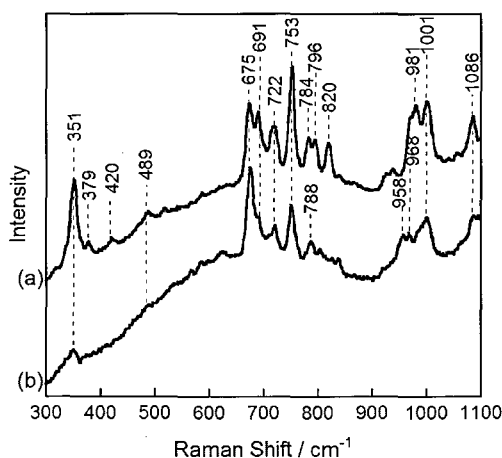
Figure 4-9. Resonance Raman spectra of ferric P450cams excited at 363.8 nm in 300–1100 \text{cm}^{-1} and 1100–1650 \text{cm}^{-1} regions in 50 mM potassium phosphate buffer (pH 7.4) containing 1 mM d -camphor and 100 mM KCl at room temperature; (a) camphor-bound wild-type P450cam and (b) rP450cam(2) spectrum. The excitation wavelength was 363.8 nm and the laser power was 6 mW.
