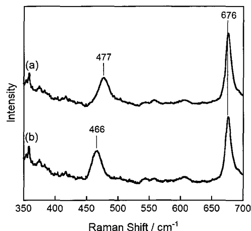
Figure 4-8. Resonance Raman spectra of CO-rP450cam(2) in 350–700 \text{cm}^{-1} region in 50 mM potassium phosphate buffer (pH 7.4) containing 1 mM d -camphor and 100 mM KCl at room temperature; (a) ^{12}\text{C}^{16}\text{O} -rP450cam(2) spectrum and (b) ^{13}\text{C}^{18}\text{O} -rP450cam(2) spectrum. The excitation wavelength was 441.6 nm and the laser power was 3 mW.
