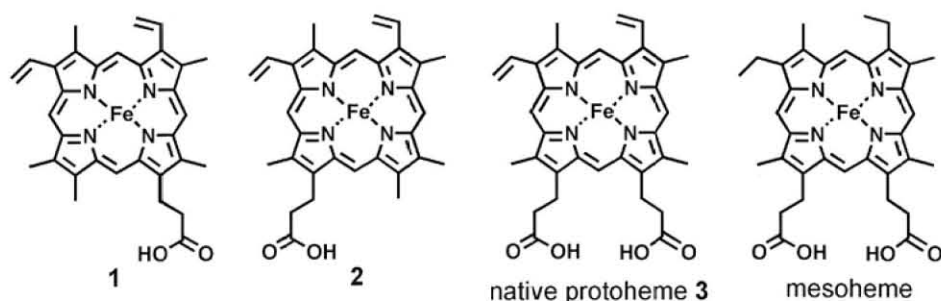
Figure 2-2. Structures of one-legged hemes 1 and 2, protoheme IX 3, and mesoheme.
