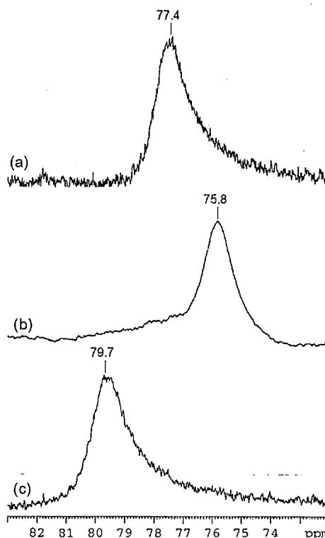
Figure 2-7. ^1\text{H} NMR spectra of deoxymyoglobins in the 72–83 ppm region in 10 mM potassium phosphate buffer ( \text{H}_2\text{O}/\text{D}_2\text{O} = 95/5 , pH 7.0) at 298 K: (a) rMb(3), (b) rMb(2), (c) rMb(1). The sample concentration was about 1 mM.
