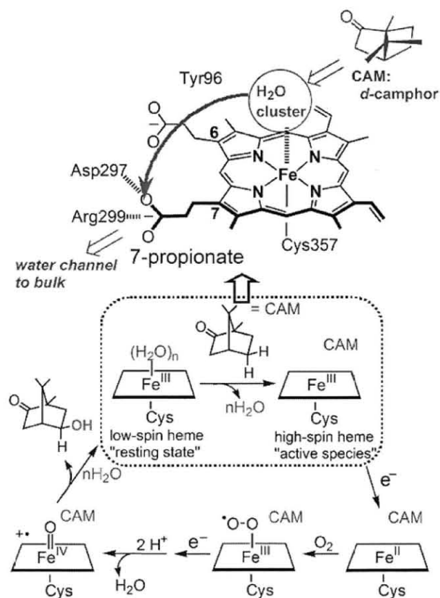
Figure 4-2. Catalytic mechanism of d -camphor hydroxylation by cytochrome P450cam and water cluster exclusion upon binding of d -camphor.
