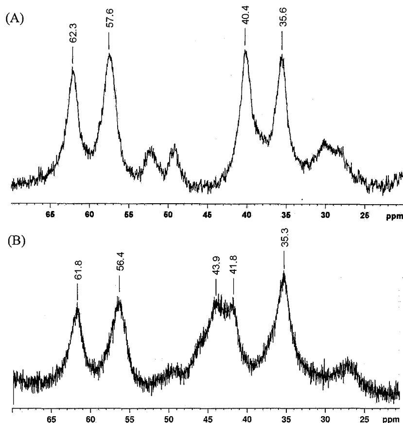
Figure 3-12. ^1\text{H} NMR spectra of the ferric high-spin form for (A) wild-type P450cam and (B) rP450cam(1) in 50 mM KPi (pD 7.4) containing 100 mM KCl and 1 mM d -camphor at 296 K.
