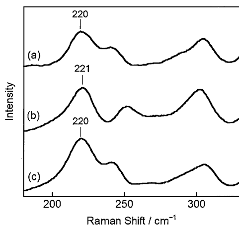
Figure 2-6. Resonance Raman spectra of deoxymyoglobins in the 180–330 \text{cm}^{-1} region in 100 mM potassium phosphate buffer (pH 7.0) at room temperature: (a) rMb(1), (b) rMb(2), (c) rMb(3). The excitation wavelength was 441.6 nm and a laser power was 12 mW.
