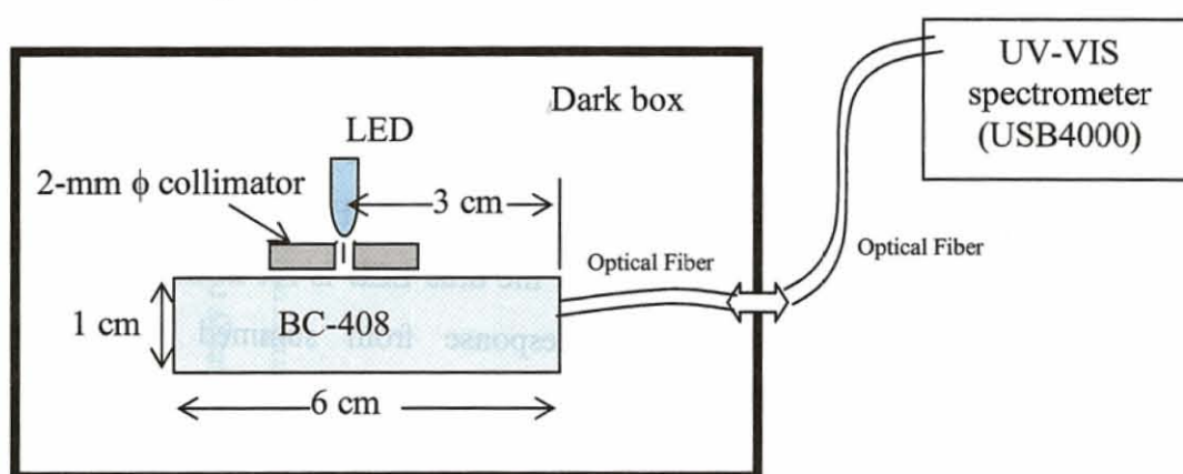
Fig. C.2 Experimental arrangement for measuring the emission spectrum of the plastic scintillator BC-408 by the UV-light LED.
