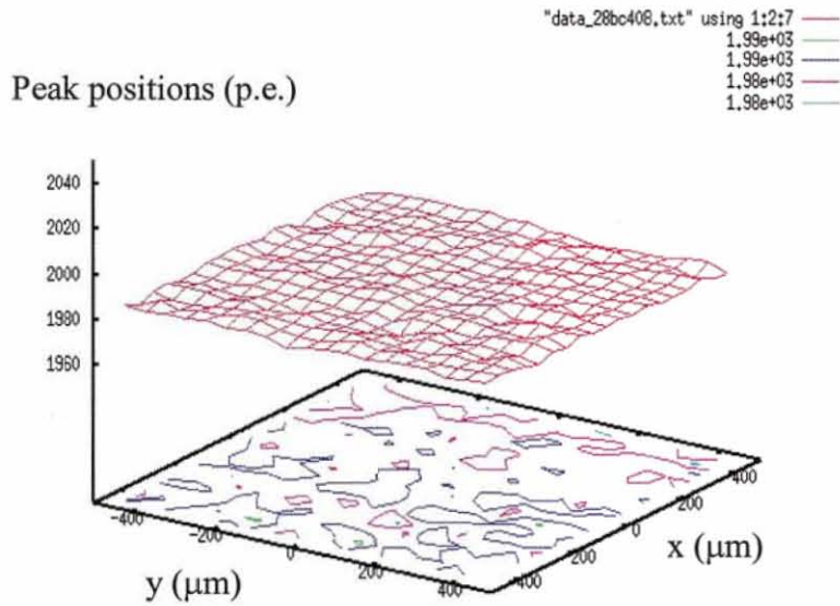
Fig. 3.5.1 Peak positions (unit: photoelectrons) plotted against the two-dimensional (2D) scanned area (x-y, unit: \mu\text{m} ).
