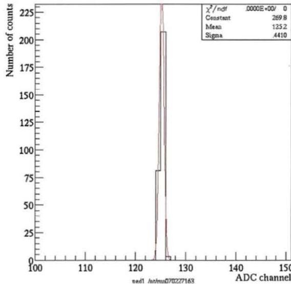
Fig. 2.1.7 Pedestal signal. The fluctuation of pedestal signal is less than 1 ADC channel.
