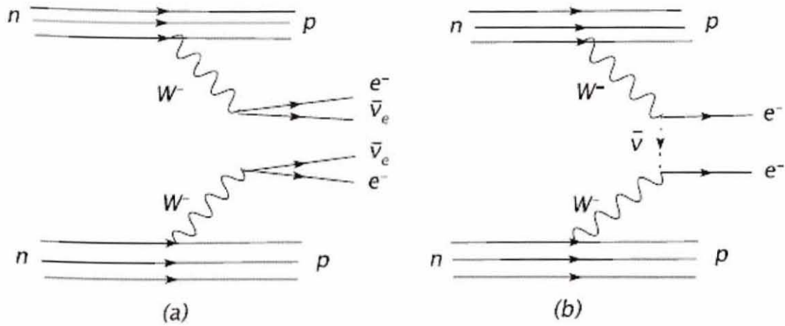
Fig. 1.2.3 Diagrams for double beta decay processes. a. Two-neutrino double beta decay. b. neutrinoless double beta decay.
