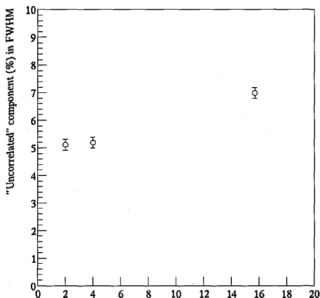
Fig. 2.2.10 Dependence of the uncorrelated component in FWHM versus electron-beam sizes. The 15.7-mm diameter beam size is equivalent a beam without use of the collimator.
