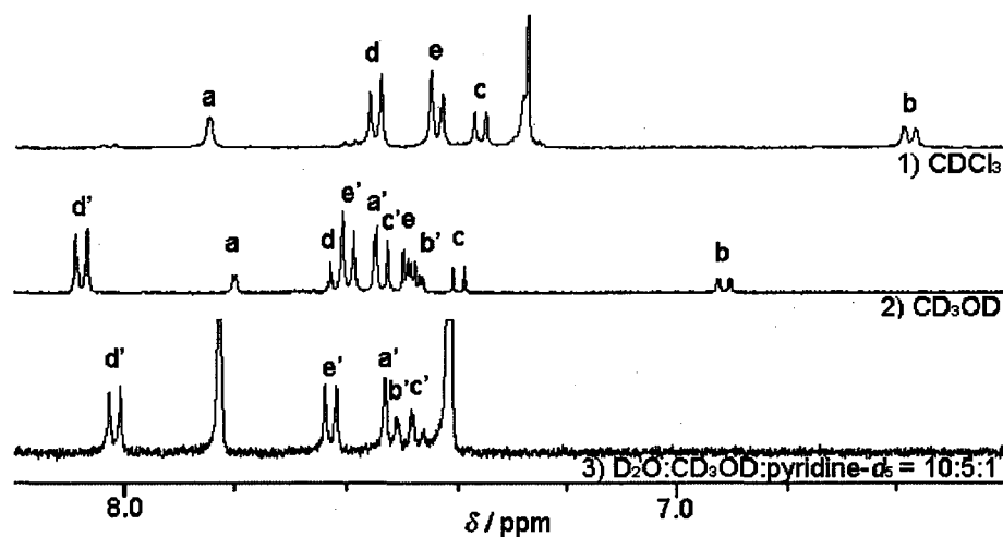
Figure 1. The aromatic region of 400 MHz ^1\text{H} NMR Spectra of 2 in several solvents. 1) \text{CDCl}_3 at rt; 2) \text{CD}_3\text{OD} at rt; 3) \text{D}_2\text{O}:\text{CD}_3\text{OD}:\text{pyridine-}d_5 = 10:5:1 at 50 °C.
