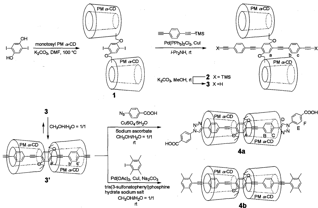
Scheme 2. Synthesis of \pi -conjugated guest bearing two PM \alpha -CDs.
